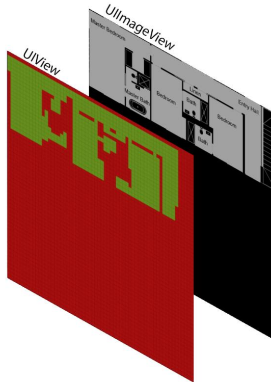
Figure 39: UIView elements of the navigation App.
