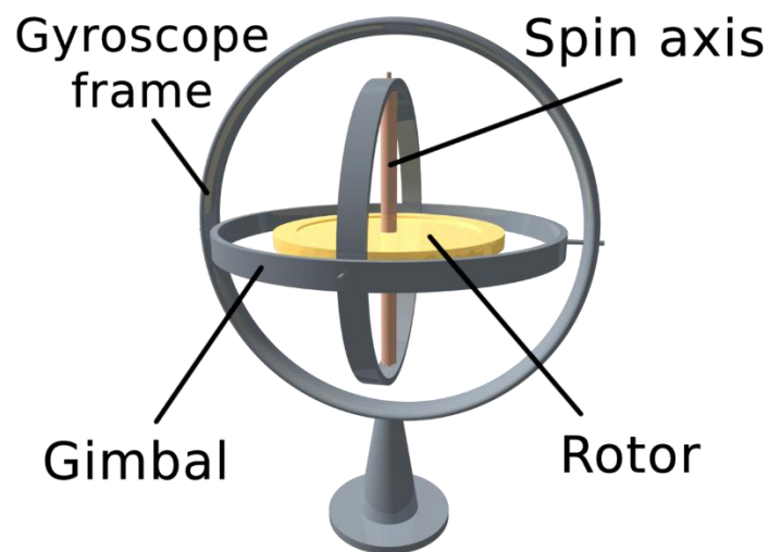
Figure 15: Gyroscope schematic structure (Gyroscope 2018).
