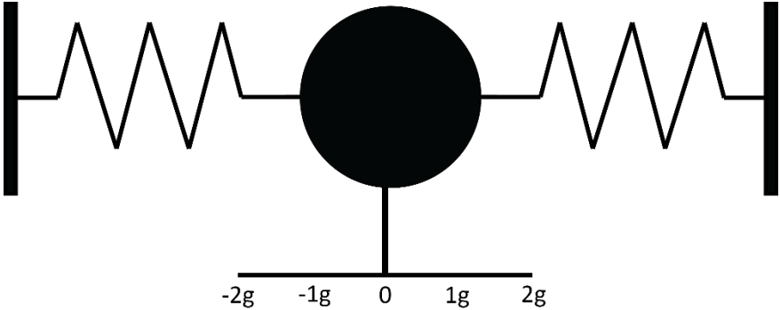
Figure 13: Schematic structure of accelerometer.
