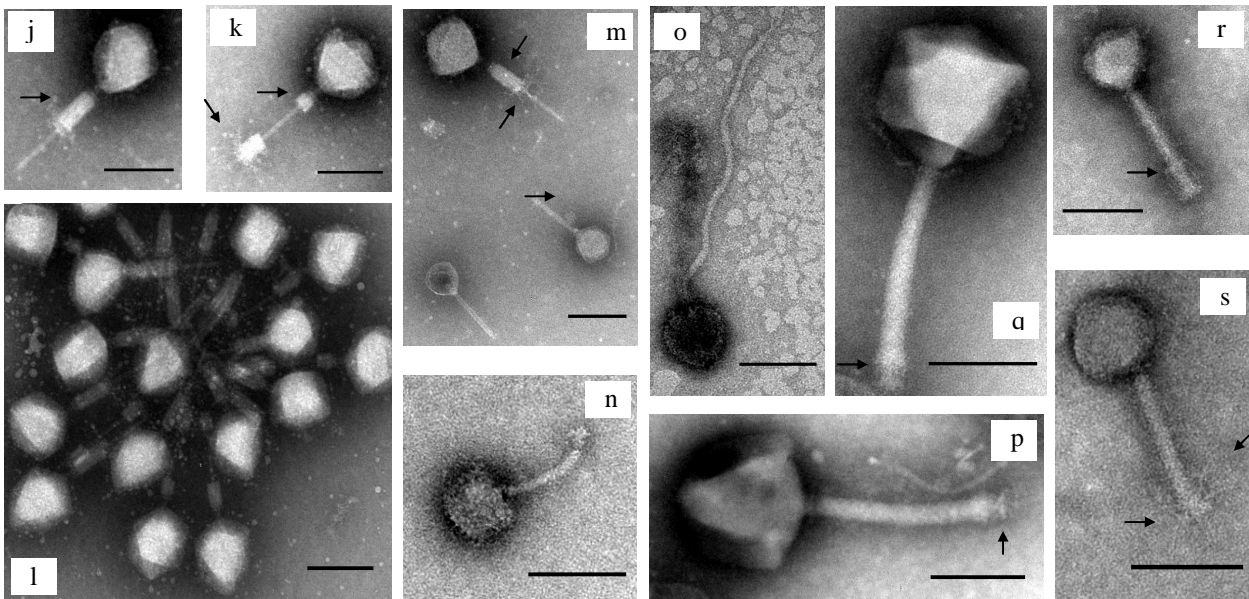
Figure 6.1 Selected transmission electron microscope micrographs of virus-like particles in the reactors VLPs in the daily-fed reactor (a-i) and the hourly-fed reactor (j-s). VLPs morphologically similar to Siphoviridae (a, b, c, e, g, i and o) and to Myoviridae (j, p, q, r, and s) were observed. Scale bar represents 100 nm.
