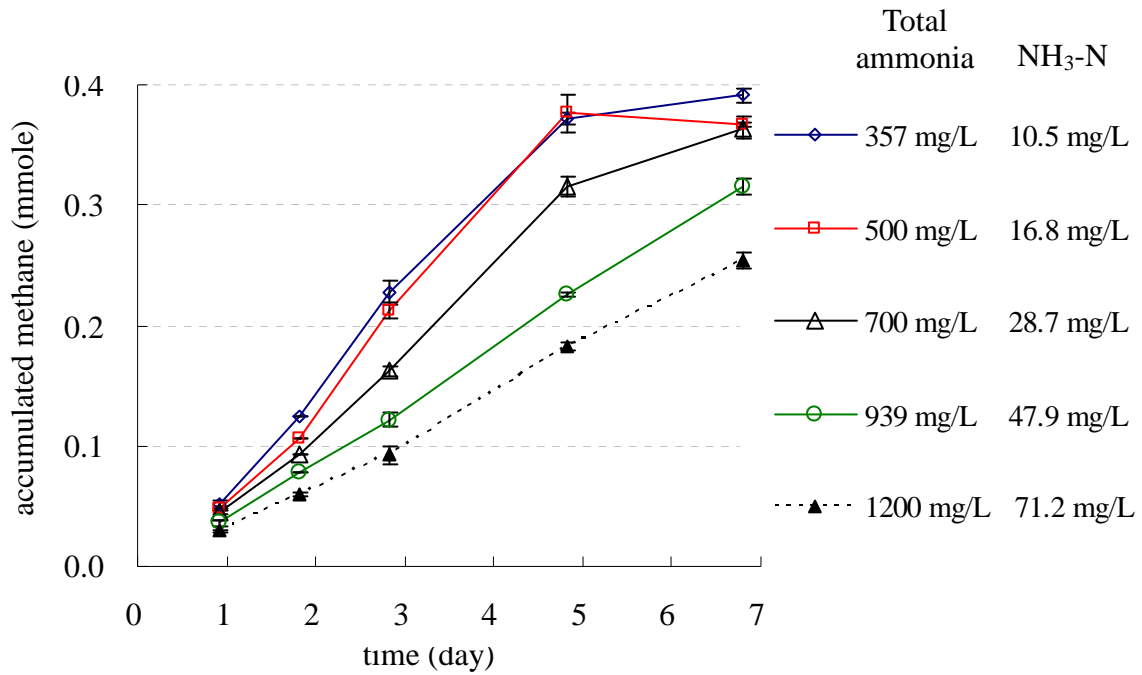
Figure 5.14 Influence of ammonia toxicity on methane yield of Methanosaeta concilii DSM 6752
