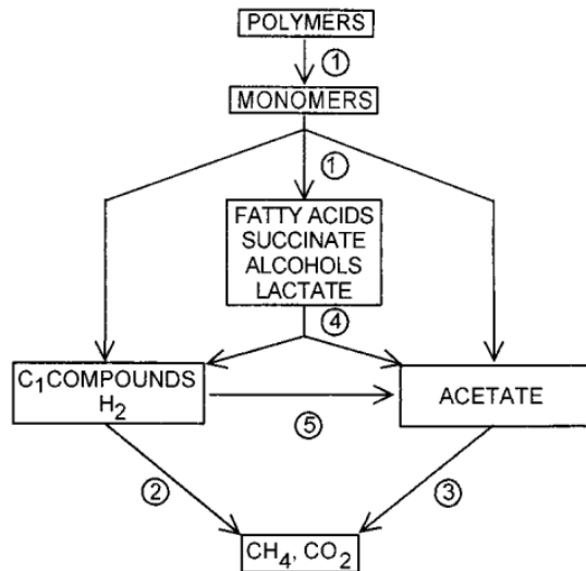
Figure 2.1 Trophic groups of microorganisms involved in anaerobic sludge digestion. Groups of organisms involved: 1) Hydrolytic and primary fermenting bacteria, 2) Hydrogenotrophic methanogens, 3) Acetoclastic methanogens, 4) Secondary fermenting (“syntrophic”) bacteria, 5) Homoacetogenic bacteria. (Schink 1997).
