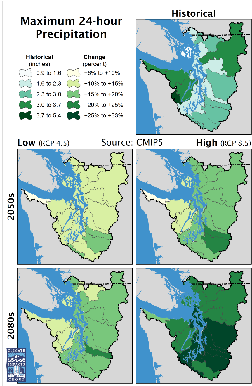
Figure 8b. Maximum 24-hour precipitation, newer projections. As in Figure 8a, except showing results from the current generation of climate model projections. Instead of the 2040s, mid-century projections are shown for the 2050s (2040-2069), and projections are included for two greenhouse gas scenarios: one low (RCP 4.5) and one high (RCP 8.5). Figure created by Rob Norheim, Climate Impacts Group, based on the CMIP5 projections used in the IPCC 2013 2 report. Data source: Mote et al. 2015. 1
