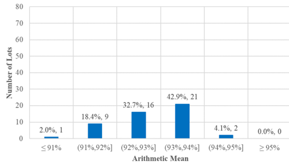
C7445, 1/2-inch NMA, Coarse-Graded, Density: 92.4%, Asphalt Content: 5.07%, PSC: 47.2, PRC: 79.1
