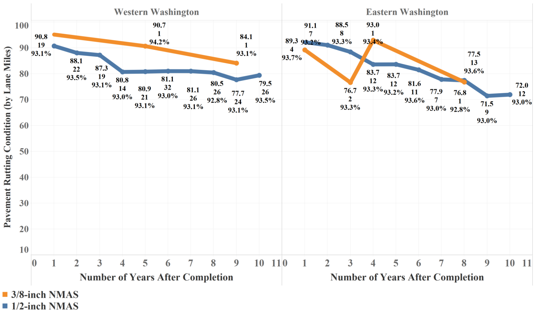
Figure 52. Average Weighted Pavement Rutting Condition by Tons of Mix, Location, Number of Contracts, and Average Weighted Density for 3/8-inch and 1/2-inch NMAS WSDOT Asphalt Pavement Mixtures, 2007 to 2016 [Data Labels: PRC (Top), Number of Contracts (Middle), Density (Bottom)]
