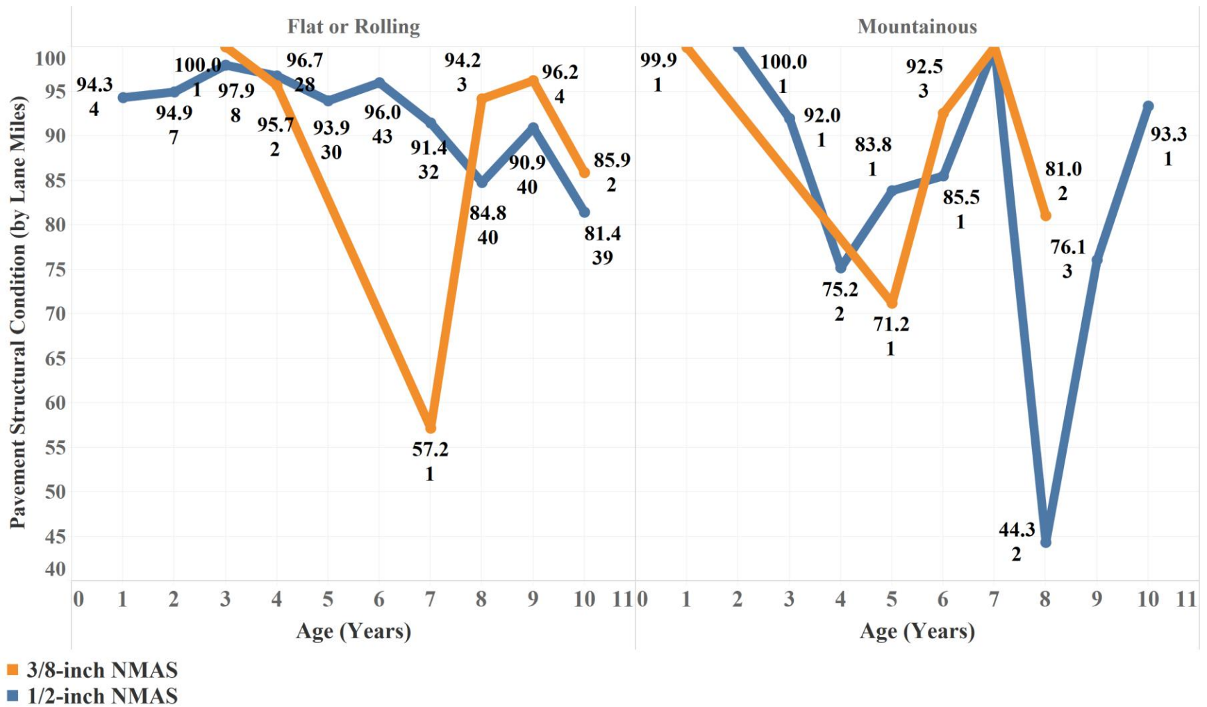
Figure 24. Average Weighted Pavement Structural Condition by Tons of Mix, Terrain, and Number of Contracts for 3/8-inch and 1/2-inch NMAAS WSDOT Asphalt Pavement Mixtures, 2007 to 2016 [Data Labels: PSC (Top), Number of Contracts (Bottom)]
