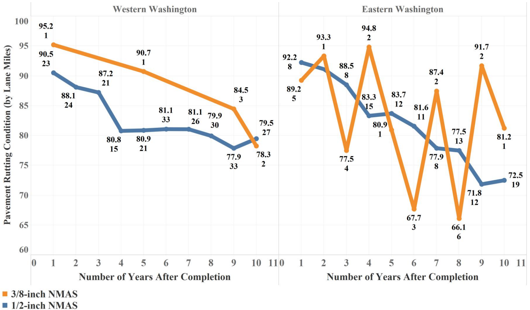
Figure 25. Average Weighted Pavement Rutting Condition by Tons of Mix, Location, and Number of Contracts for 3/8-inch and 1/2-inch NMAAS WSDOT Asphalt Pavement Mixtures, 2007 to 2016 [Data Labels: PRC (Top), Number of Contracts (Bottom)]
