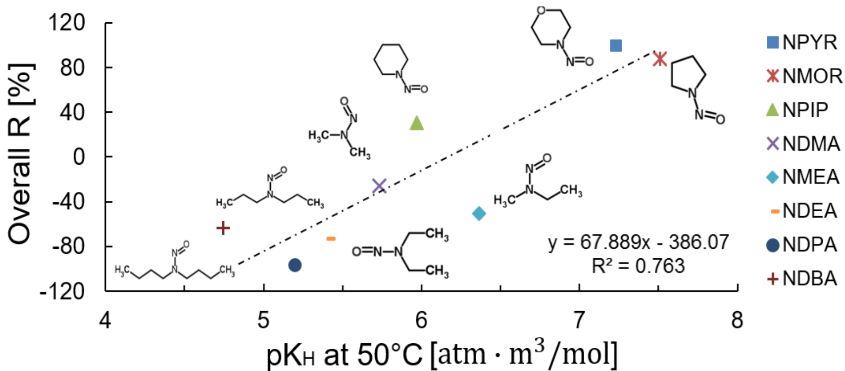
Figure 10. Overall rejections [%] of 8 nitrosamines with increasing Henry's law constants values shown as p K H at 50°C. Abbreviations for compounds represent N-nitrosopyrrolidine (NPYR), N-nitrosomorpholine (NMOR), N-nitrosopiperidine (NPIP), N-nitrosodimethylamine (NDMA), N-nitrosomethylethylamine (NMEA), N-nitrosodiethylamine (NDEA), N-nitrosodipropylamine (NDPA), and N-nitrosodibutylamine (NDBA).
