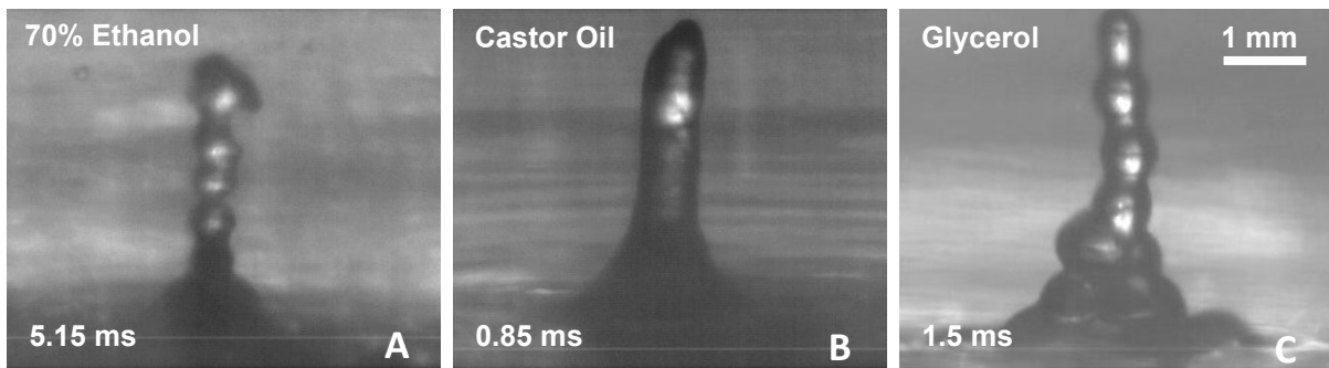
FIGURE 4.8: Frames taken from the high speed videos of A) 70% ethanol at a 180 W/cm 2 acoustic intensity, B) castor oil at a 24,000 W/cm 2 intensity, and C) glycerol at a 24,000 W/cm 2 intensity. In ethanol (A), the intensity was just above its atomization threshold; on the upper left just under the “70% ethanol” label, you can see a droplet that was ejected from the fountain. In both castor oil (B) and glycerol (C), the intensity was at the maximum output of the transducer and atomization did not occur ( i.e. no droplets were emitted from the fountain).
