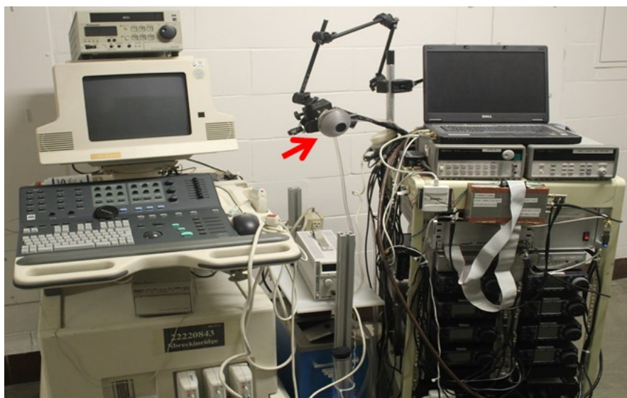
FIGURE 5.1: Image showing the first generation array device used in the threshold study. On the left is the HDI 5000, which collects an image of the kidney with a coaxially aligned P4-2 transducer. In the middle is the water cooling and circulation system, and on the right is the custom-built array device. The red arrow indicates the 2 MHz array transducer with the water-coupling cone.
