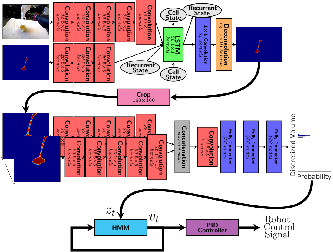
Figure 5.2: The entire robot control system using the recurrent neural network for detections and the multi-frame network for volume estimation. The recurrent detection network (top) takes both the color image and its own detections from the previous time step and produces a liquid detection heatmap. The multi-frame network (center) takes a sequence of detections cropped around the target container and outputs a distribution over volumes in the container. The output of this network is fed into a HMM, which estimates the volume of the container. This is passed into a PID controller, which computes the robot's control signal.
