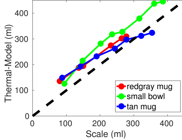
Figure 5.5: The plot shows the scale reading compared to the thermal camera with the model based method for each of the target containers.
