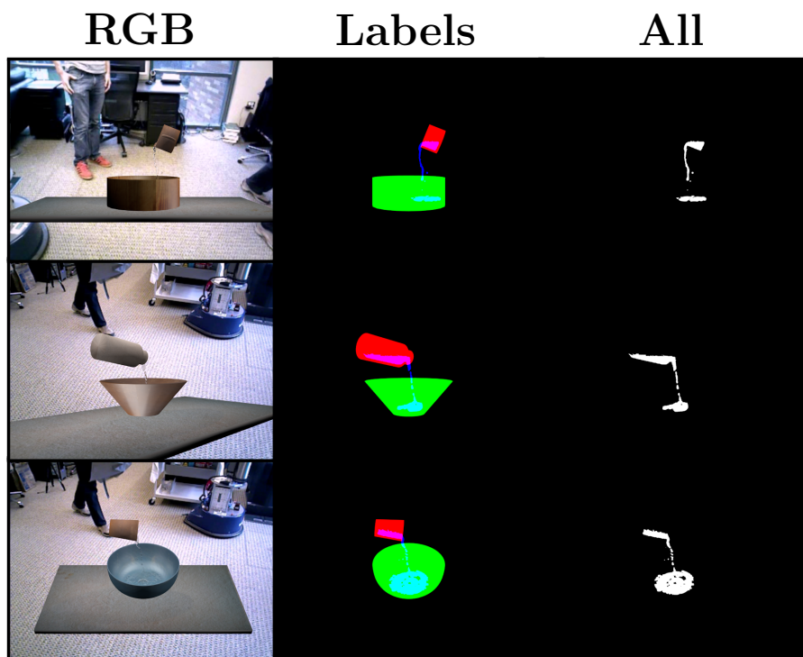
Figure 6.1: Examples of frames from the simulated dataset. The left column is the raw RGB images generated by the renderer (for reference); the center column shows the ground truth labeling output by the simulator; the right column shows the ground truth liquid location for all liquid in the scene.
