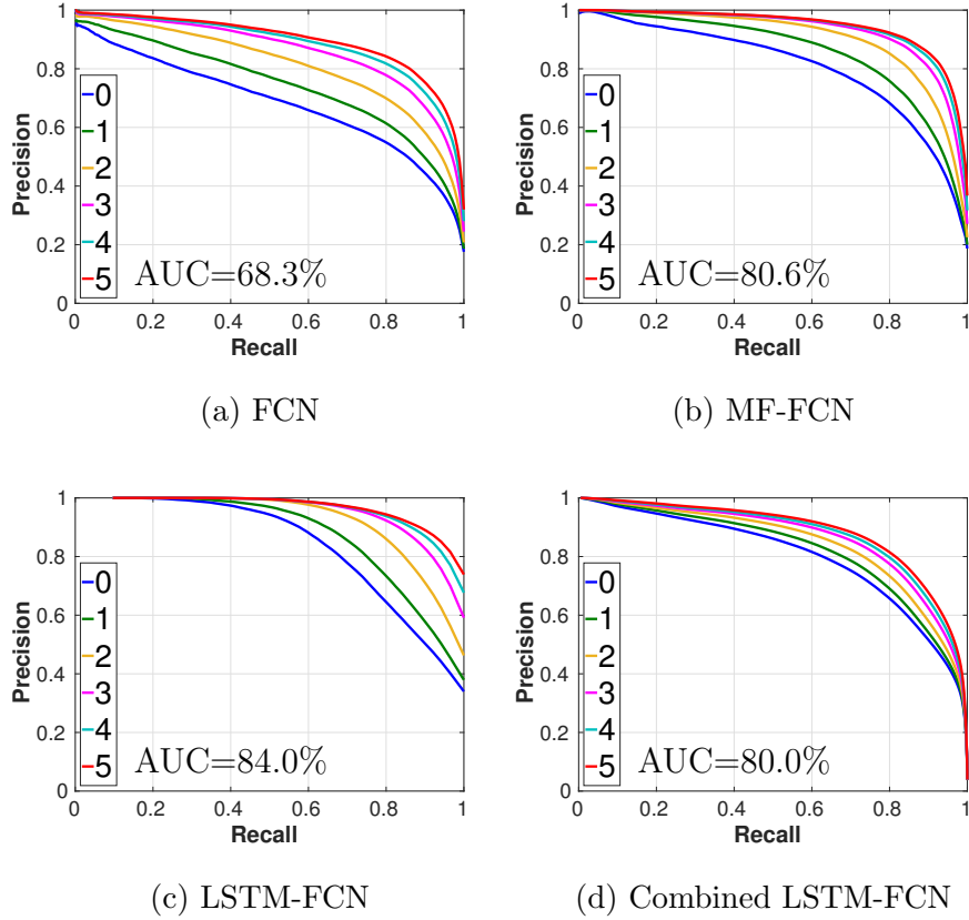
Figure 6.3: The precision-recall curves for the tracking task on the simulated dataset. The first 3 show the performance of the three network types on the tracking task alone. The last graph shows the performance of the LSTM-FCN on the combined detection & tracking task using the standard RGB format as input. The different lines show the different amounts of slack, i.e., how far a positive classification can be from a true positive to still count as correct. The area under the curve (AUC) is shown for the 0 slack curve.
