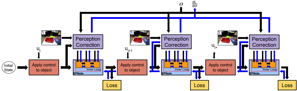
Figure 8.9: Diagram of the rollout procedure for optimizing the parameters of the perception network \theta . This is very similar to the procedures shown in Figures 8.5 and 8.7. The dynamics are computed forward (black arrows) for a fixed number of timesteps into the future (shown here are 3). In this case the controls u are fixed. The gradients of the loss are computed with respect to \theta backwards (blue arrows) through the rollout using backpropagation. The box “Perception Correction” corresponds to the network shown in Figure 8.8 and \theta are its parameters. Note that here the inner loop of the PBF algorithm in SPNets is shown (with 3 iterations) since this is how the perception correction is integrated into the dynamics.
