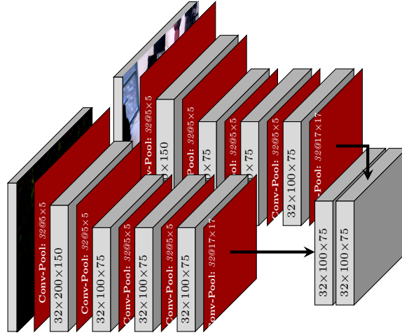
(c) Late Fusion Input Block
