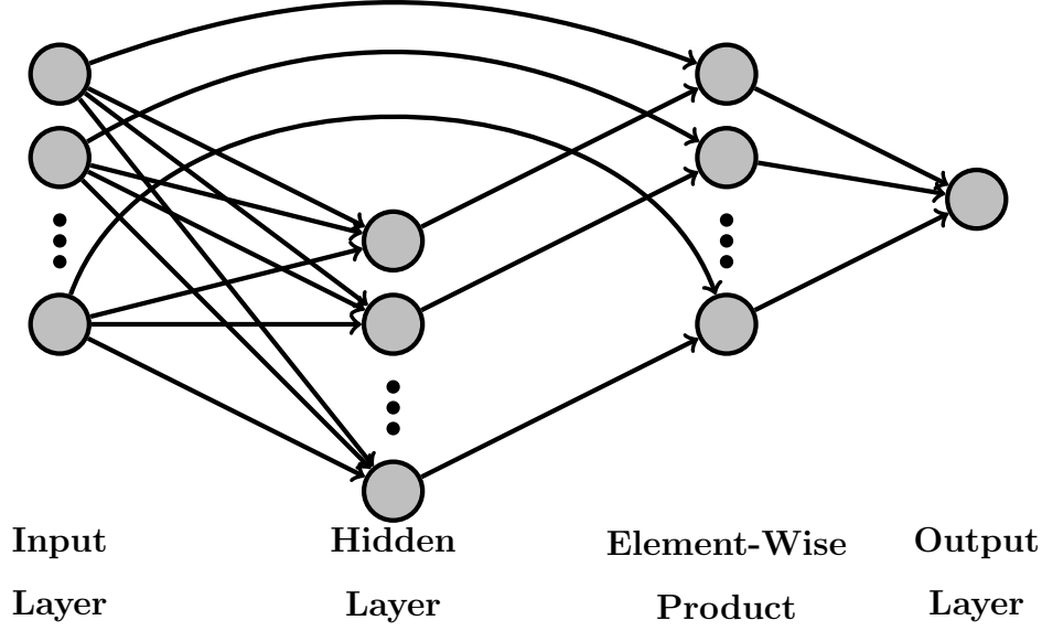
Figure 3.2: The neural network used to learn the policy. The input layer is fed into a fully-connected hidden layer, and then the output of the hidden layer is element-wise multiplied by the input layer, which is finally fed into the output layer.
