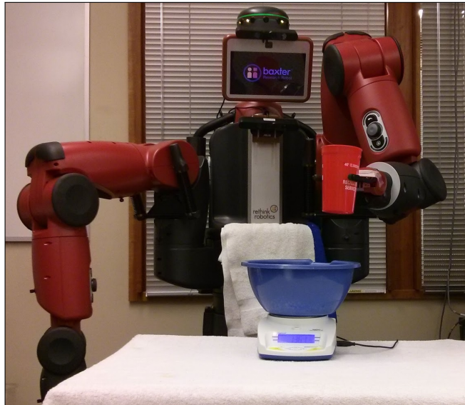
Figure 3.1: The robot used in these experiments. It is a Rethink Robotics Baxter Research Robot, equipped with two 7-DOF arms. Also shown is the experimental setup with the cup in the robot’s gripper positioned above the table, with the bowl resting on top of the scale.
