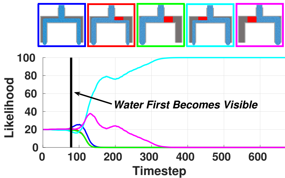
Figure 7.7: Probability distribution over the blockage location over time for a single interaction. The 5 diagrams across the top correspond to the five different simulations the robot ran, each color-coded to the corresponding line in the plot. The true blockage was placed in the left leg and only partially blocked the leg (in the keys in the top row, second from right). Best viewed in color.
