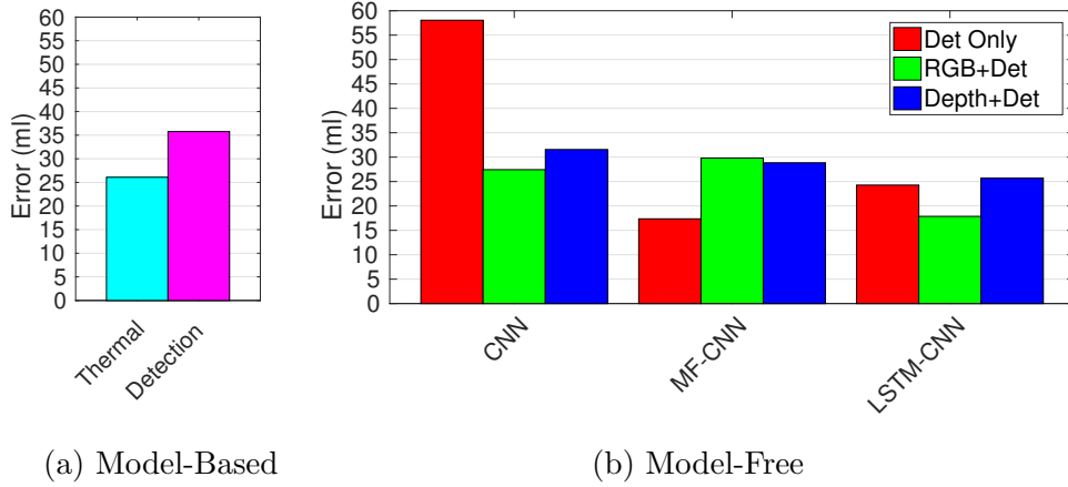
Figure 5.6: Root mean squared error in milliliters of each of the methods for volume estimation. The left plot shows the error for the model-based method using either the thermal image or the output of the detection network as pixel labels. The right plot shows the error for the model-free methods when the networks take as input only the liquid detections (red), the liquid detections plus the color image (green), and the liquid detections plus the depth image (blue).
