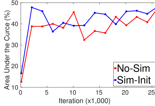
Figure 4.15: The area under the curve on the test set at each iteration of training. The red line shows the performance of the LSTM-FCN trained solely on the robot dataset; the blue line shows the performance of the LSTM-FCN initialized from the simulated dataset.
