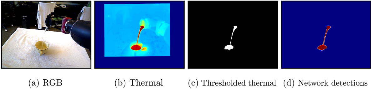
Figure 5.3: An example frame from a pouring sequence. The left image shows the color camera from the robot’s perspective, the left-middle image shows a heatmap of the thermal camera after it has been registered to the color camera, the right-middle image shows the water labeled by thresholding the thermal image, and the right image shows the output of the detection network based on the RGB input.
