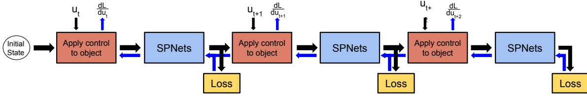
Figure 8.5: Diagram of the rollout procedure for optimizing the controls u . The dynamics are computed forward (black arrows) for a fixed number of timesteps into the future (shown here are 3). Then gradients of the loss are computed with respect to the controls backwards (blue arrows) through the rollout using backpropagation.
