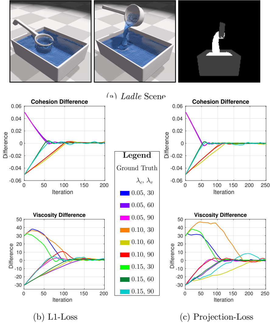
Figure 8.3: (Top) The ladle scene. The left two images are before and after snapshots, the right image shows the particles projected onto a virtual camera image (with the objects shown in dark gray for reference). (Bottom) The difference between the estimated and ground truth fluid parameter values for cohesion \lambda_c and viscosity \lambda_v after each iteration of training for both the L1 loss and the projection loss. The color of the lines indicates the ground truth \lambda_c and \lambda_v values. The cohesion parameter \lambda_c was initialized to 0.1 in all cases except when the ground truth was 0.1, in which case it was initialized to 0.05. The viscosity parameter \lambda_v was initialized to 60 in all cases except when the ground truth was 60, in which case it was initialized to 30.
