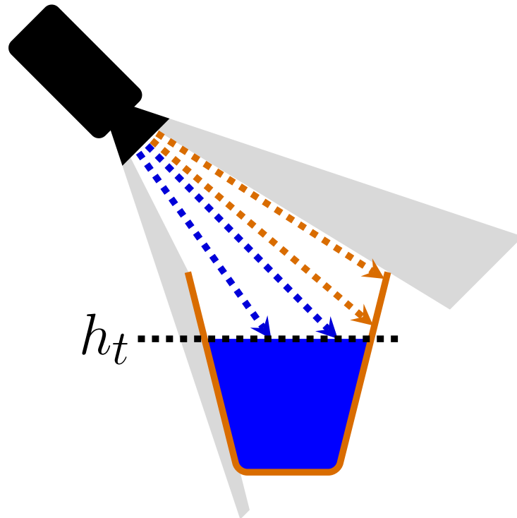
Figure 5.4: Diagram of the camera looking into the target container. The blue shows where the liquid is expected to be, given a volume and the corresponding fill height, h_t . The blue lines show pixels expected to be classified as liquid and the orange lines show pixels that are expected to be classified as not-liquid . The gray shows pixels outside the container and not used by our algorithm.
