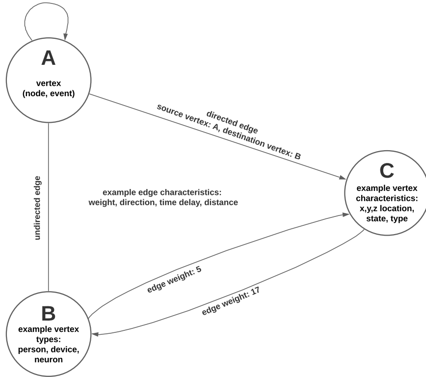
Figure 1.1: In this example, A, B, and C are vertices connected by edges. The relationship between A and B is shown with an undirected edge, which means either could be the source or destination vertex; it is a two-way path. The directed edges, conversely, show that there is a path from A to B through vertex C, but not a path from B to A through vertex C. When C is the source vertex, B and C (itself) are the only destination vertices.
