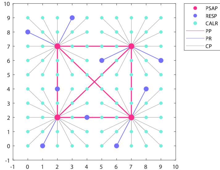
Figure 5.3: 10 \times 10 grid of vertices displaying connections between PSAPs, responders, and callers
