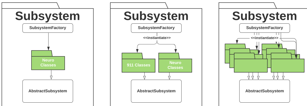
Figure 4.4: Graphitti was designed to have a uniform structure within each subsystem regardless of how many domains are added. Prior to implementing the NG-911 domain, only the Neuro domain existed. This topology allows for new domains to be added without affecting the greater system functionality, increasing configurability.
