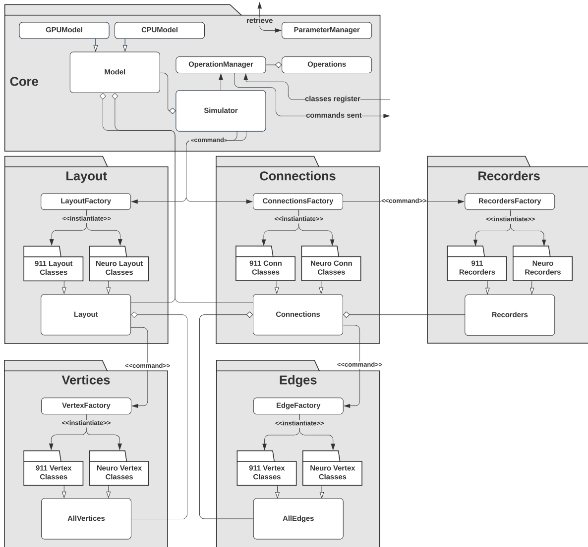
Figure 4.1: Graphitti UML diagram showing (1) the six main subsystems: Core , Layouts , Connections , Vertices , Edges , and Recorders ; and (2) the discipline-specific subsystems
