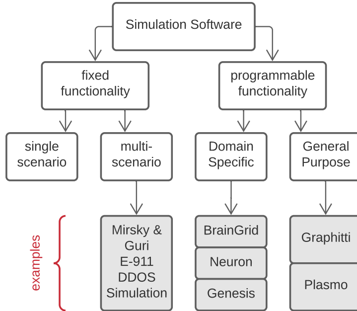
Figure 2.1: A type-map for simulators relevant to this paper, with examples.
