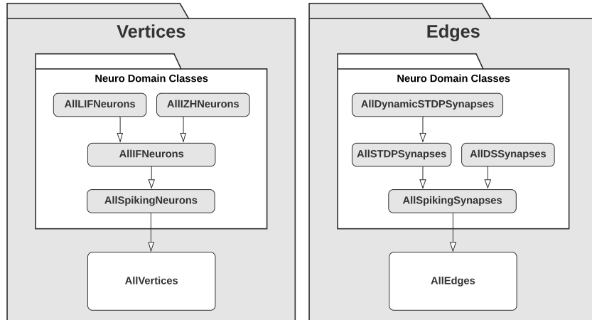
Figure 4.2: This diagram illustrates the relegation of neurospecific classes within the vertices and edges subsystems. No new classes or domains are represented.
