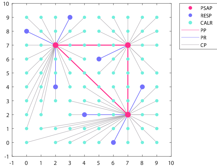
Figure 5.5: 10 \times 10 grid of vertices displaying connections between PSAPs, responders, and callers
