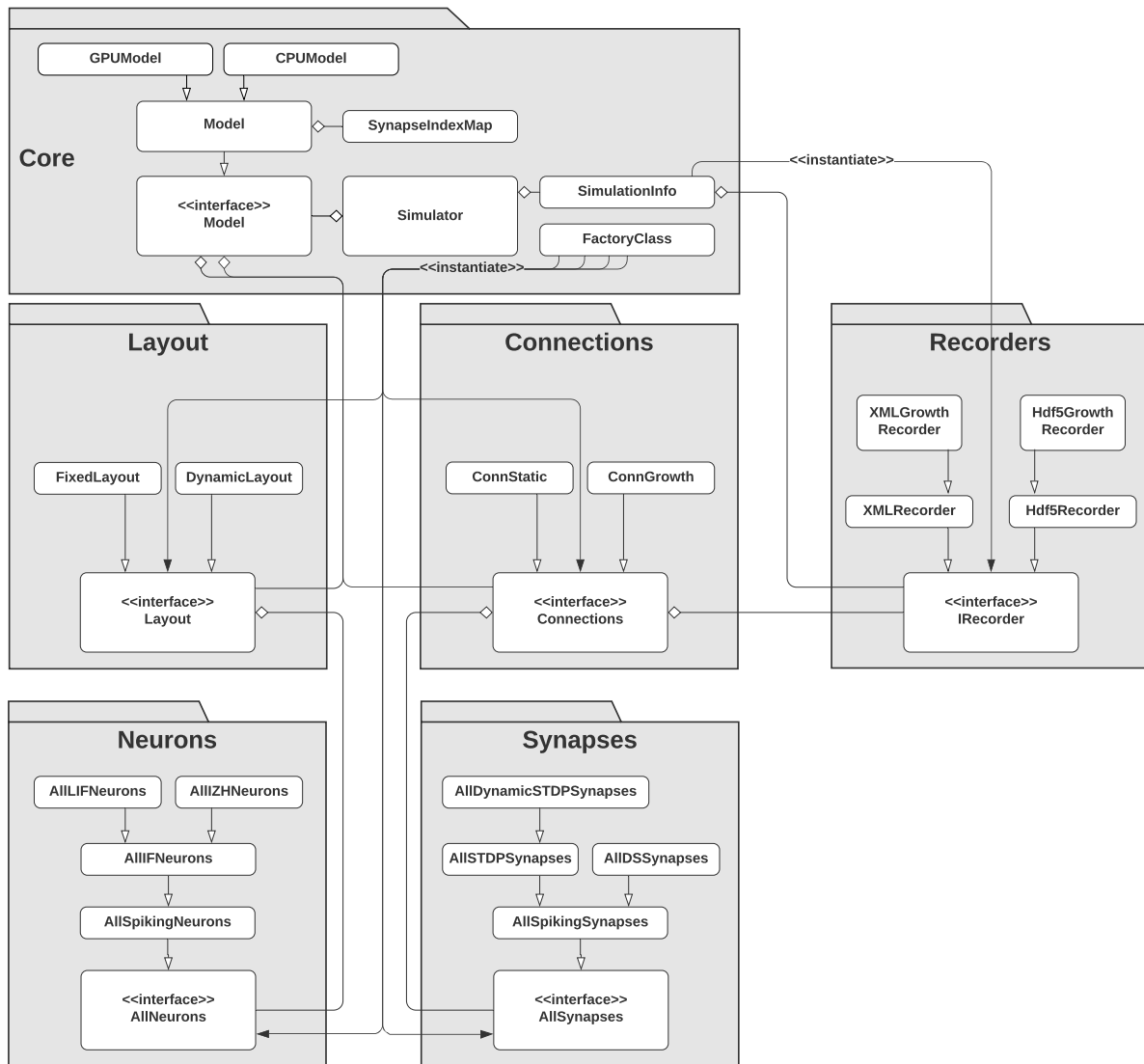
Figure 3.1: BrainGrid UML Diagram showing the six main subsystems: Core , Layouts , Connections , Neurons , Synapses , and Recorders
