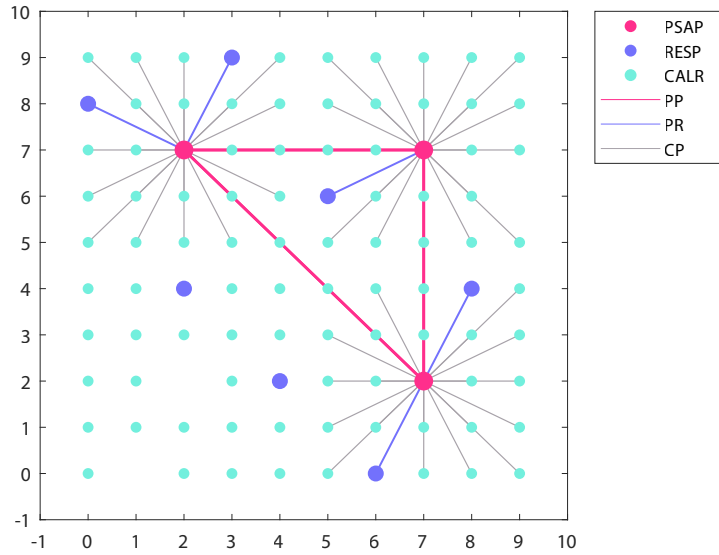
Figure 5.4: 10 \times 10 grid of vertices displaying connections between PSAPs, responders, and callers
