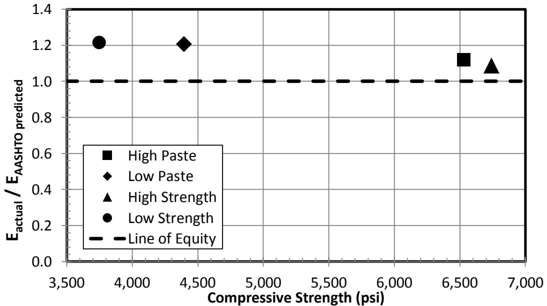
Figure 6.3: Day 28 Elastic Modulus Ratio: DuPont (3/4-in.) Mixtures
