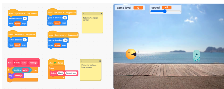
Figure 7.5: A “Game micro-world”. Available blocks(left) and the game controlled by the program(right).
