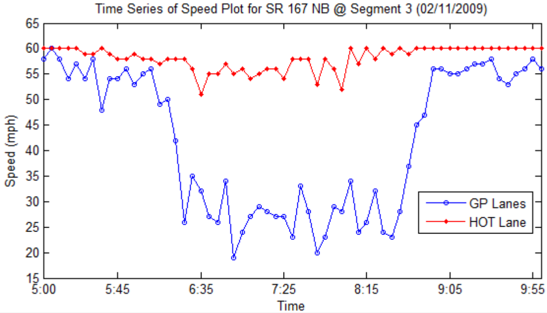
FIGURE 5.3 Time Series of Speed Plot for SR 167 NB @ Segment 3
