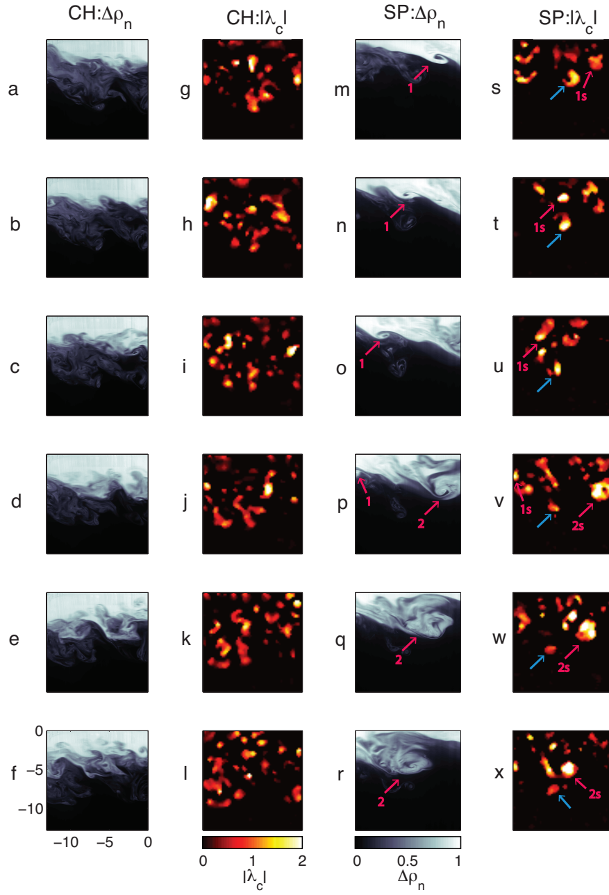
Figure A.2: Same as Figure A.1 but for a later time when plume turns into steady-state region
