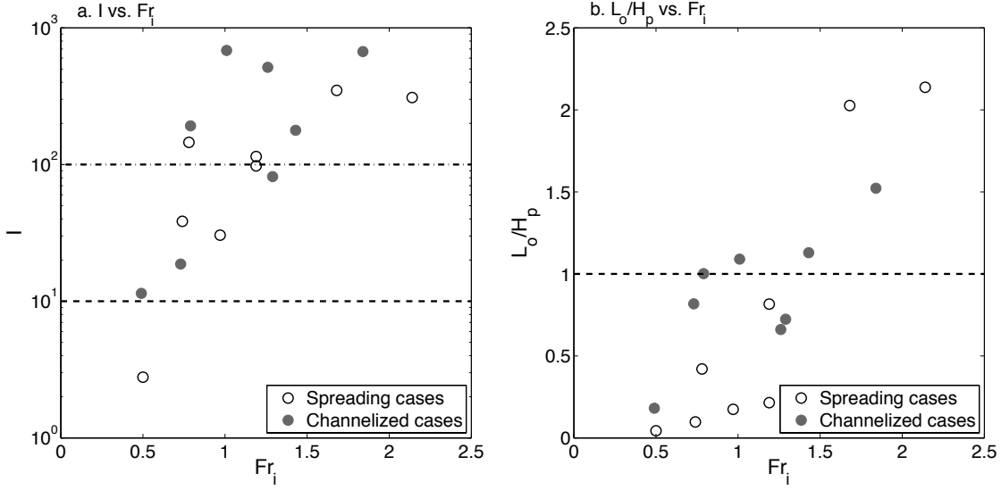
Figure 3.12: Plots of a) I = \varepsilon / \nu N^2 vs. Fr_i , dash line and dash-dot lines are two thresholds for turbulent regime, I = 10 and I = 100 . b) Ozmidov scale L_o normalized by plume thickness H_p vs. Fr_i , dash line is the reference for L_o = H_p
