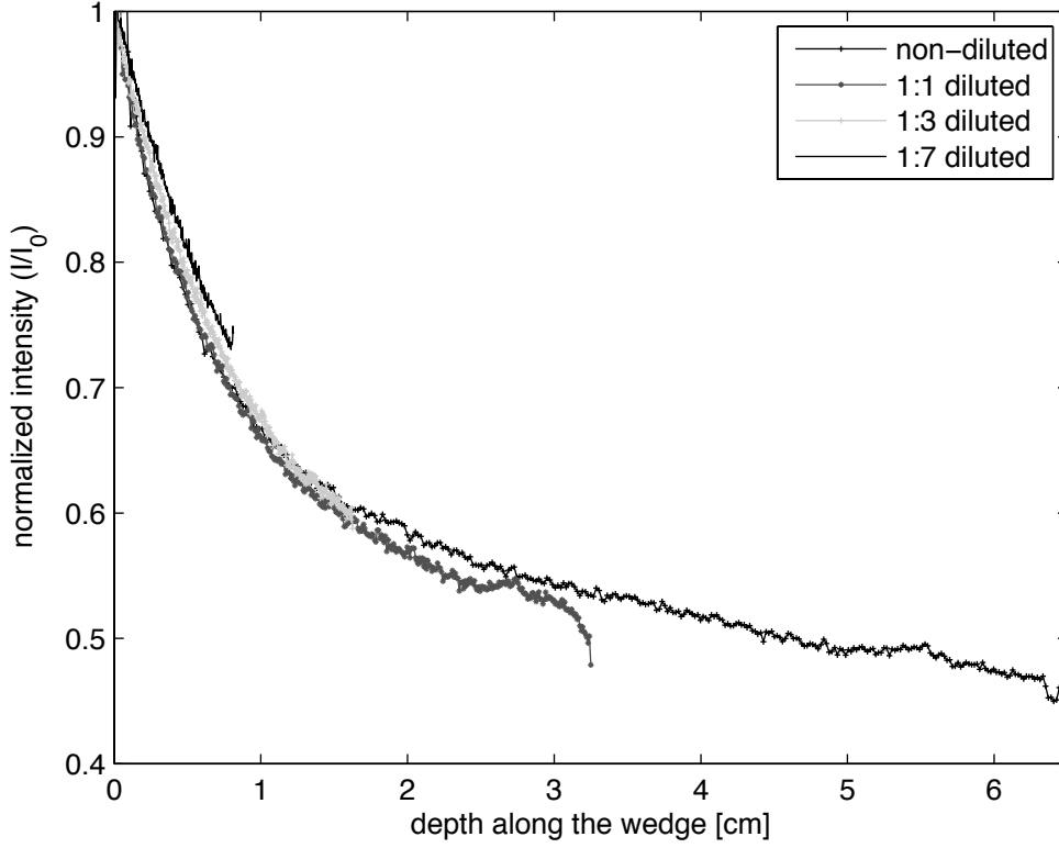
Figure 2.5: Red dye dilution test comparing non-diluted dye water to 1:1, 1:3, 1:7 DI water dilution. The normalized intensities I/I_0 are along the calibration wedge and depths for different dilutions are scaled by their corresponding dilution ratios.
