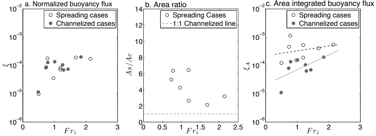
Figure 3.11: Plots of a) normalized buoyancy flux \xi = \frac{\bar{B}}{\Delta \rho g l} , b) ratio of Plume area in spreading cases ( A_S ) to channelized cases ( A_C ), and c) area integrated turbulent buoyancy flux \xi_A = \xi \frac{A_S}{A_C} vs. Fr_i for spreading (open circles) and channelized (filled circles) runs. Linear fits in c) are applied separately for spreading (dash line) and for channelized runs (solid line).
