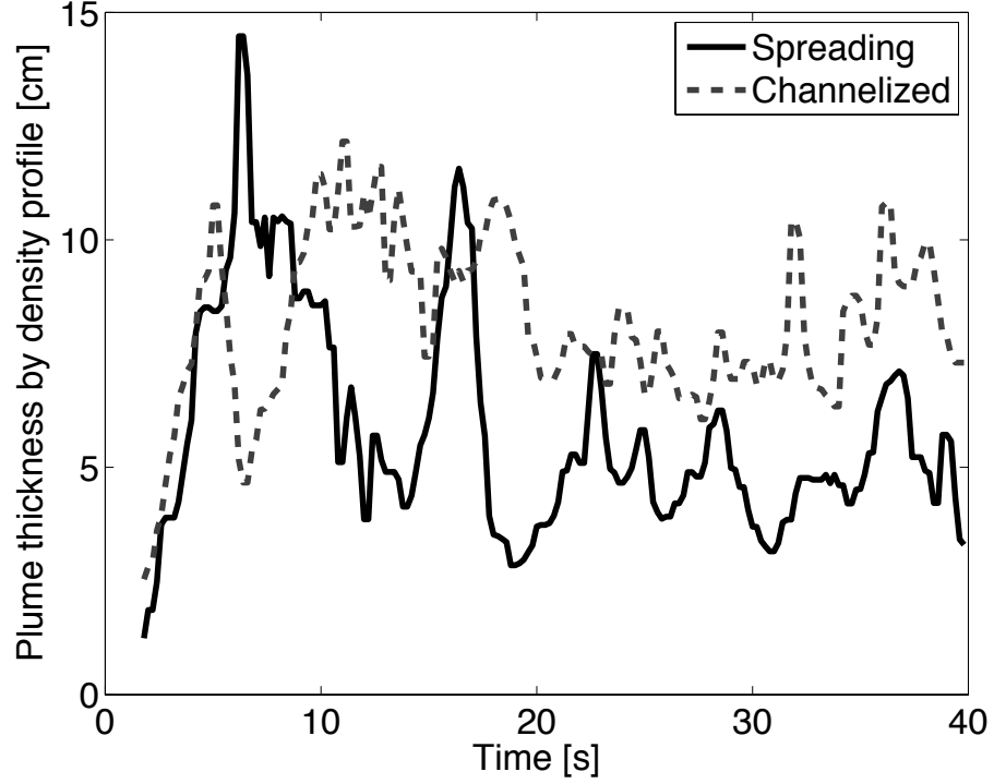
Figure 4.9: Plume thickness, \delta_\rho vs. time t .
