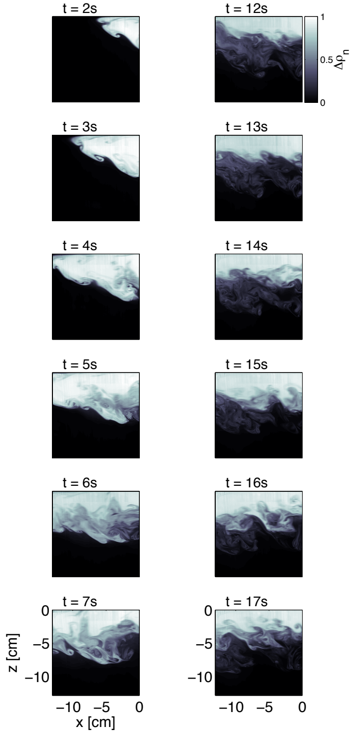
Figure 4.6: Normalized density anomaly field sequence at the plume front region (left-hand column) and steady-state region (right-hand column) for channelized case (CH 4 ). Time increases downward at each column, time interval between two frames is 1 s. Physical dimension of this field of view is labeled at the lower-left corner.
