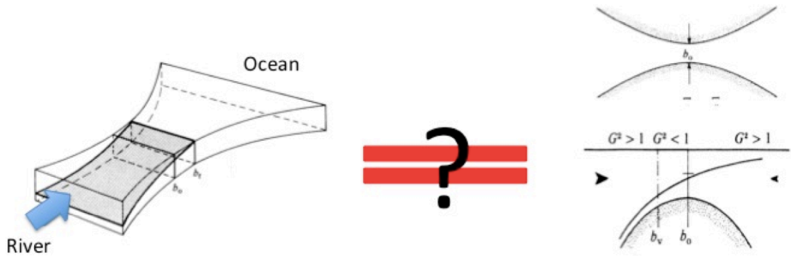
Figure 4.2: Schematic comparison between 'inverted box flows' ( left ) and classical two-way exchange flow over sill and contraction ( right ). 'Inverted box flows' is modified from the definition of 'box flows' model described by Armi and Farmer (1986) Figure 10: perspective view of intermediate box flow in which the interface meets the surface upstream of the narrowest section. The classical two-way exchange flow model is after Farmer and Armi (1986) Figure 12: the sketch of plan view and side view of two-way exchange past a coincident sill and contraction with strong barotropic component.
