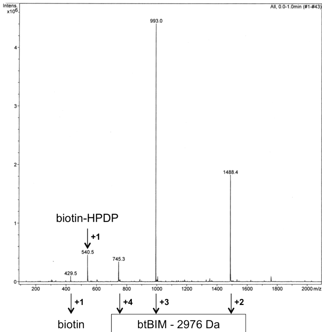
Figure 3.10: The crude btBIM product was analyzed by mass spectrometry to confirm sufficient conjugation. No free peptide was observed in the crude sample suggesting near 100% conjugation with an excess of biotin-HPDP
