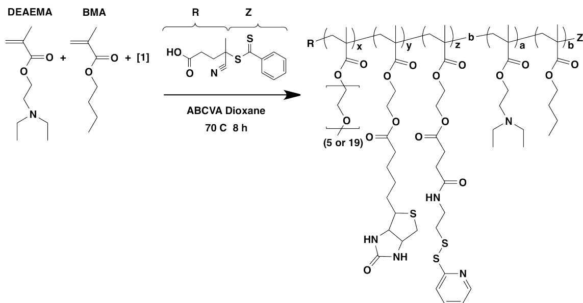
Figure 5.2: RAFT synthesis was used to make two diblock copolymers by incorporating the multifunctional O950 and O300 polymers as the macroCTAs with ABVCA as the radical initiator. To make the second block, the monomer feed ratio was 60% diethylaminoethyl methacrylate (DEAEMA) and 40% butyl methacrylate (BMA).
