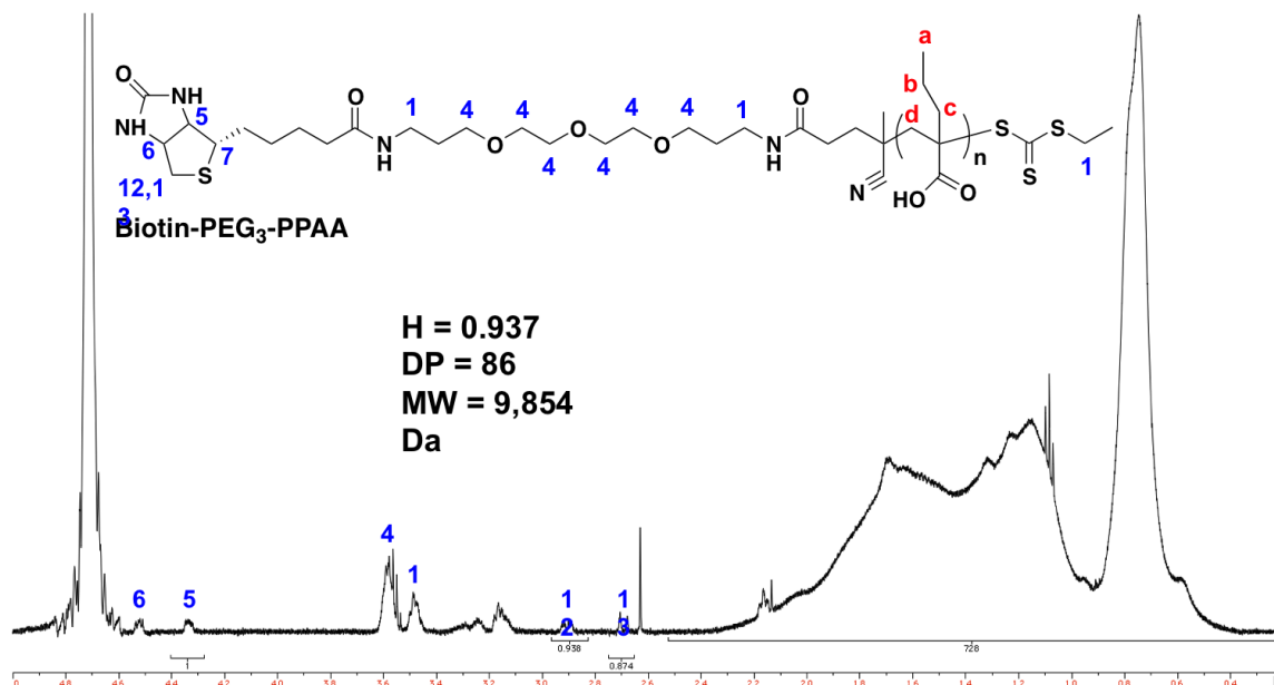
Figure 3.13: NMR spectrum of the btPEG-PPAA polymer
