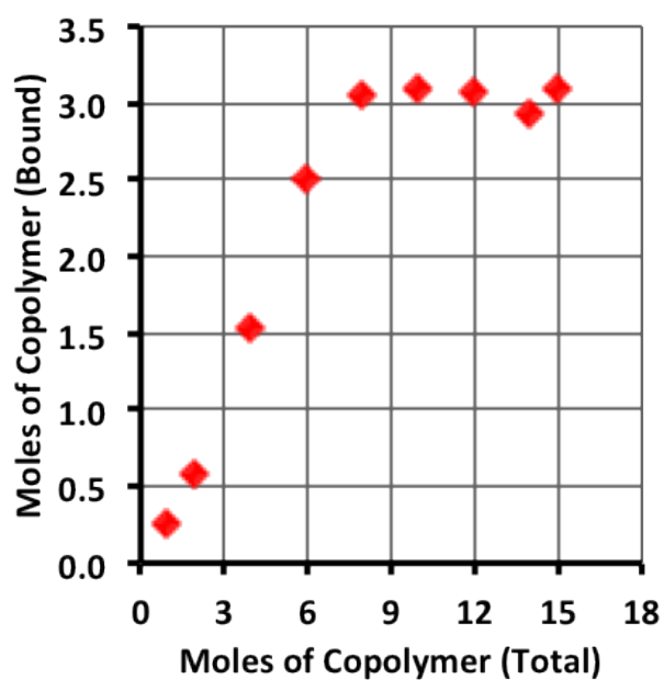
Figure 3.5: A HABA binding curve was used to measure the number of accessible biotin per diblock copolymer and demonstrate saturation of the streptavidin protein with biotinylated polymer
