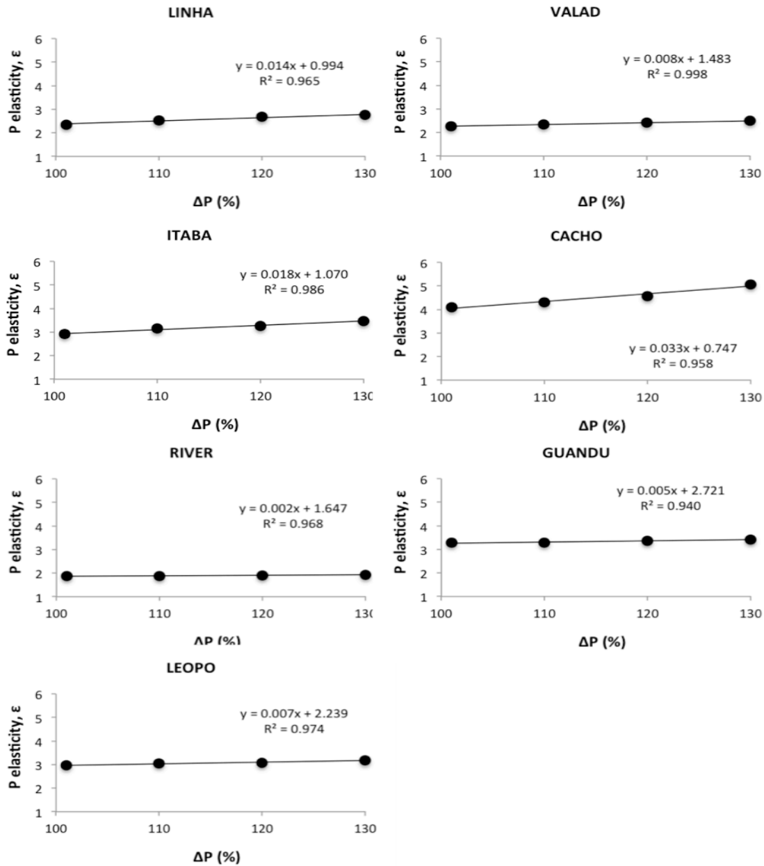
Figure 2.7. Precipitation elasticity ( \epsilon ) for the seven gauging stations from VIC simulations.
