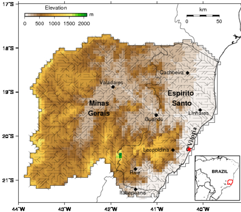
Figure 2.1: DEM and domain of Espírito Santo and Minas Gerais with station locations and flow directions.
