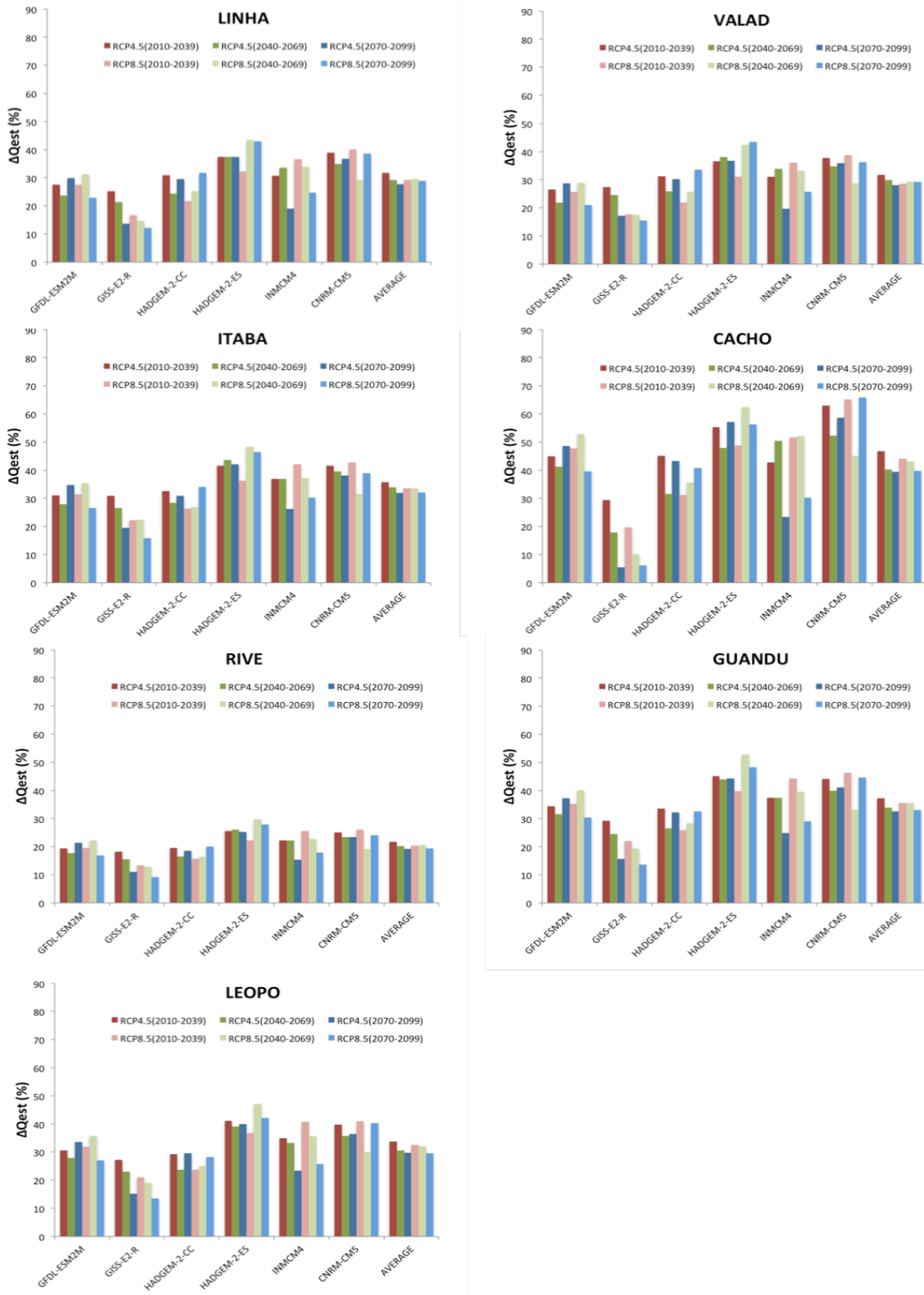
Figure 2.9. Predicted rate of change of streamflow, \Delta Q_{est} for the seven basins by the different selected AOGCMs for RCP4.5 and RCP8.5 for each corresponding 30-year interval (2010 – 2039, 2040 – 2069 and 2070 – 2099)
