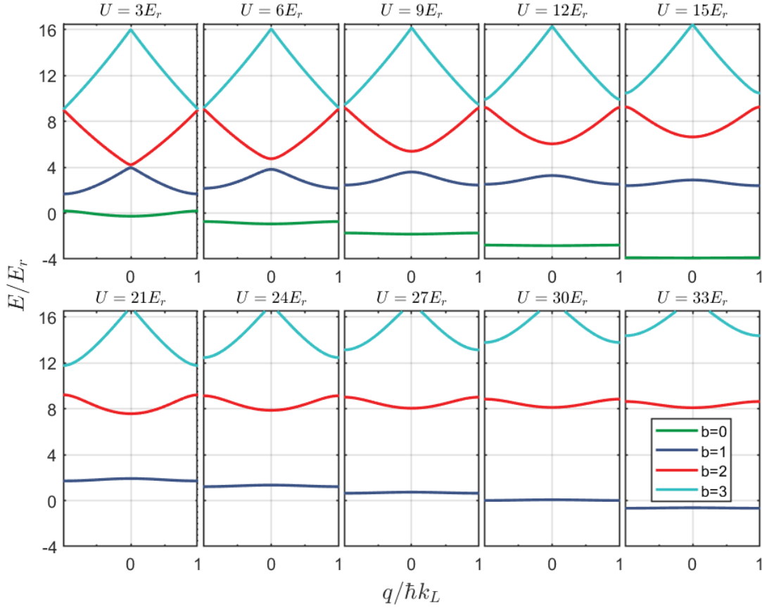
Figure 4.1: The ground ( b=0 ) and three excited ( b=1,2,3 ) Bloch bands shown for a range of lattice depths. Top row: Bloch bands around the first magic depth U_M^{(1)} = 9.2E_r . Bottom row: Bloch bands around the 2nd magic depth U_M^{(1)} = 27.3E_r .
