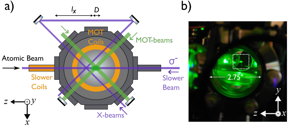
Figure 2.2: MOT chamber with fields. (a) Birds-eye schematic. An increasing field Zeeman slower is followed by the X-beam slower before the MOT. (b) Side view roughly coinciding with side imaging (see Section 2.7). A dashed rectangular region highlights a MOT fluorescing with > 10^8 ytterbium atoms.
