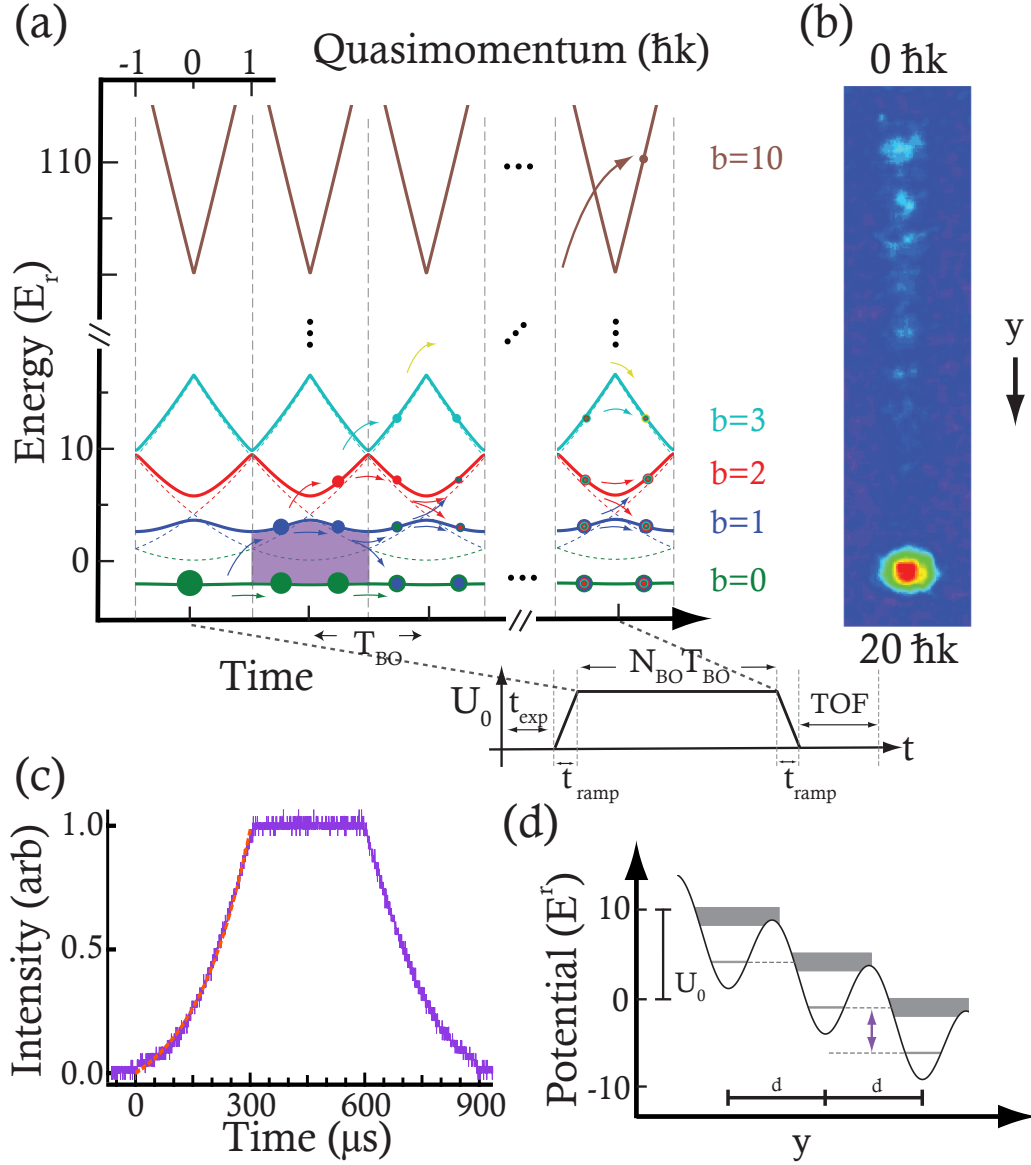
Figure 3.1: Multi-path Stückelberg interferometer sequence. (a) Atomic passage due to BOs in a periodic zone scheme with avoided band crossings acting as beamsplitters, shown for U_0/E_r = 10 and N_{\text{BO}} = 10 . The shaded region highlights the energy difference between b = 0 and b = 1 within one Brillouin zone. Inset: A sketch of the lattice intensity during a typical MPSI sequence. (b) Averaged absorption image ( t_{\text{exp}} = 3 \text{ ms} , \text{TOF} = 12 \text{ ms} ) showing MPSI output ports for N_{\text{BO}} = 10 , U_0/E_r = 6 , T_{\text{BO}} = 0.33(h/E_r) . Gravity points against the y direction. (c) A representative intensity profile with T_{\text{BO}} = 0.11(h/E_r) , N_{\text{BO}} = 10 , U_0/E_r = 6 . (d) Washboard potential for U_0/E_r = 10 and T_{\text{BO}} = 0.2(h/E_r) with shading for the bandwidth.
