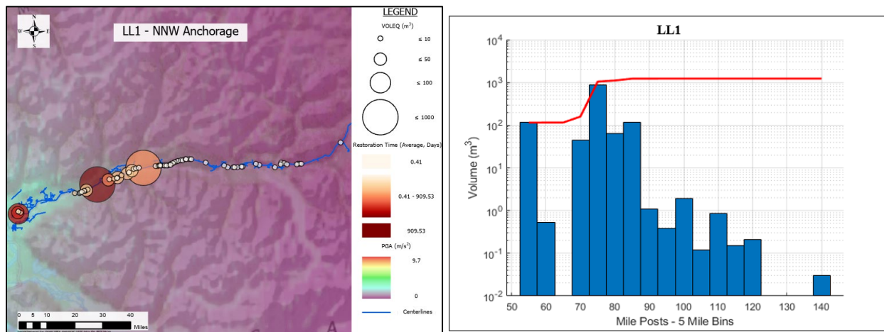
Figure 4.19 Long Lake Scenario LL1 results (accumulated volume in red in the panel to the right)
