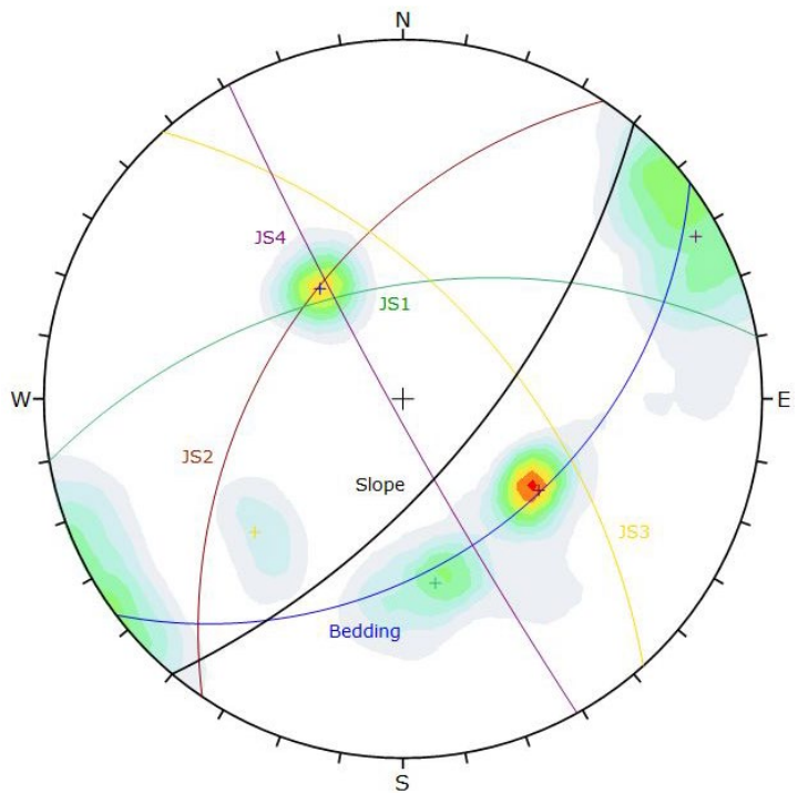
Figure 2.6 Stereonet for Long Lake 75.5 sandstone.
