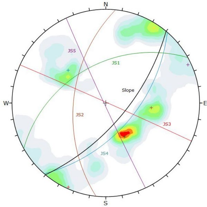
Figure 2.5 Stereonet for Long Lake 75.5 rhyodacite.
