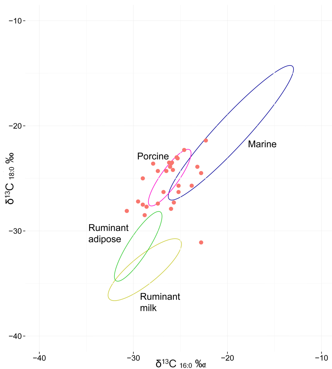
Figure 5.16: The results of CSIA by GC-C-IRMS of the samples from the Sosa-Dong site using the reference from Craig et al. (2011)
