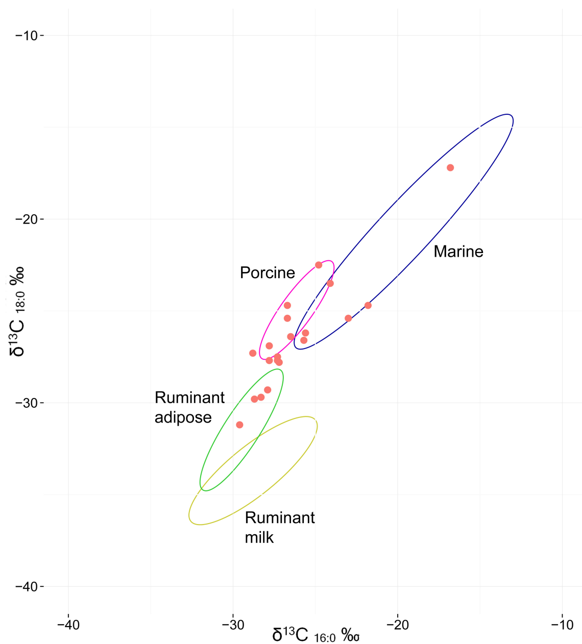
Figure 5.7: The results of CSIA by GC-C-IRMS of the samples from the Kimpo-Yangchon site using the reference from Craig et al. (2011)
