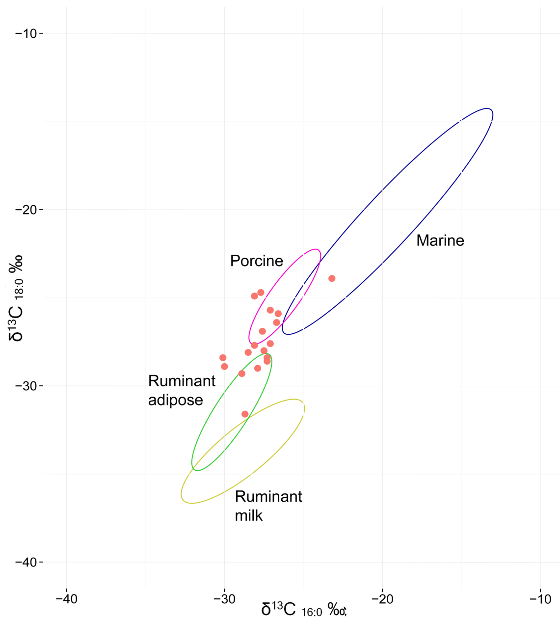
Figure 5.22: The results of CSIA by GC-C-IRMS of the samples from the Songguk-Ri site using the reference from Craig et al. (2011)
