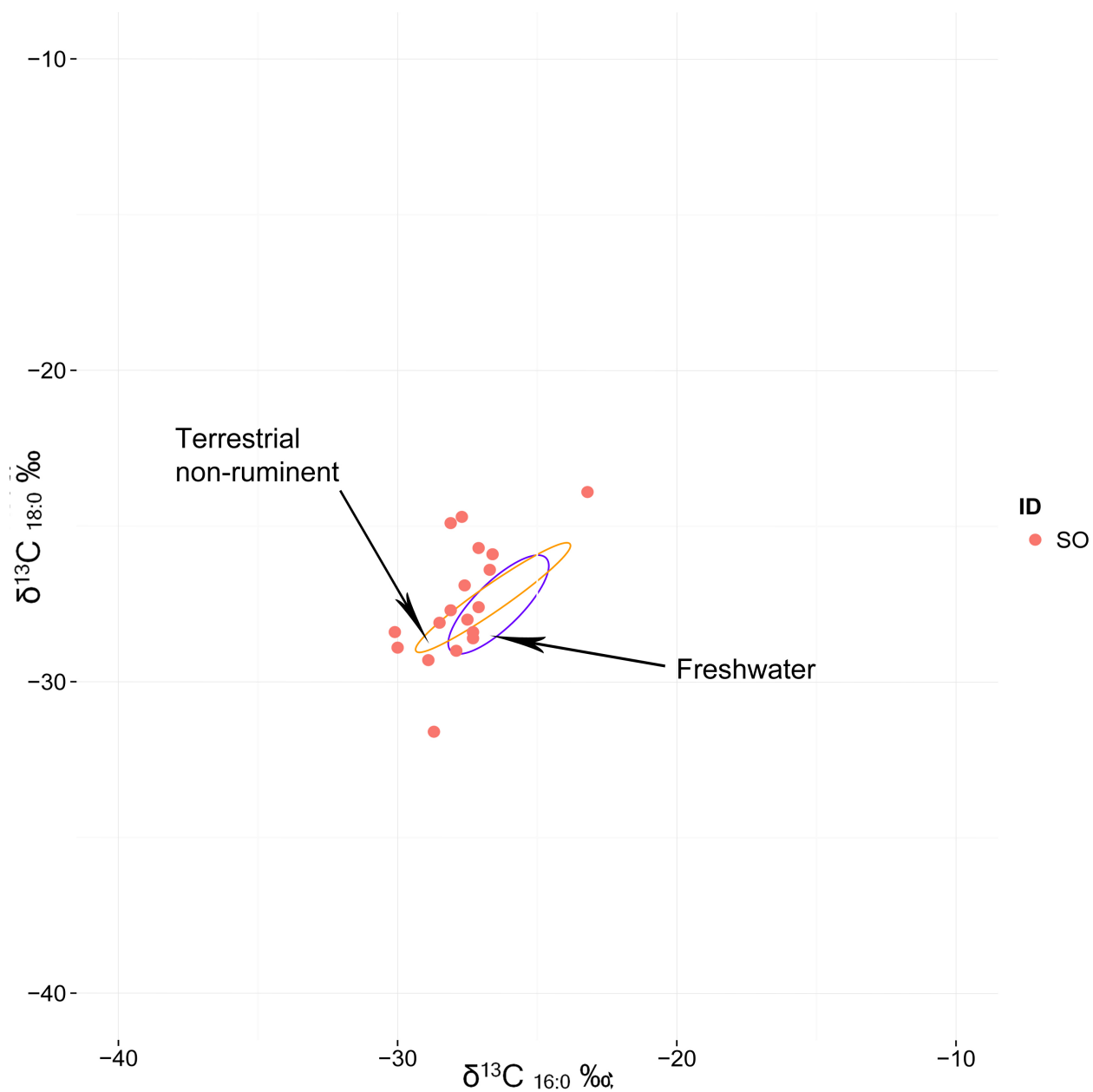
Figure 5.23: The results of CSIA by GC-C-IRMS of the samples from the Songguk-Ri site using the reference from Craig et al. (2013)
