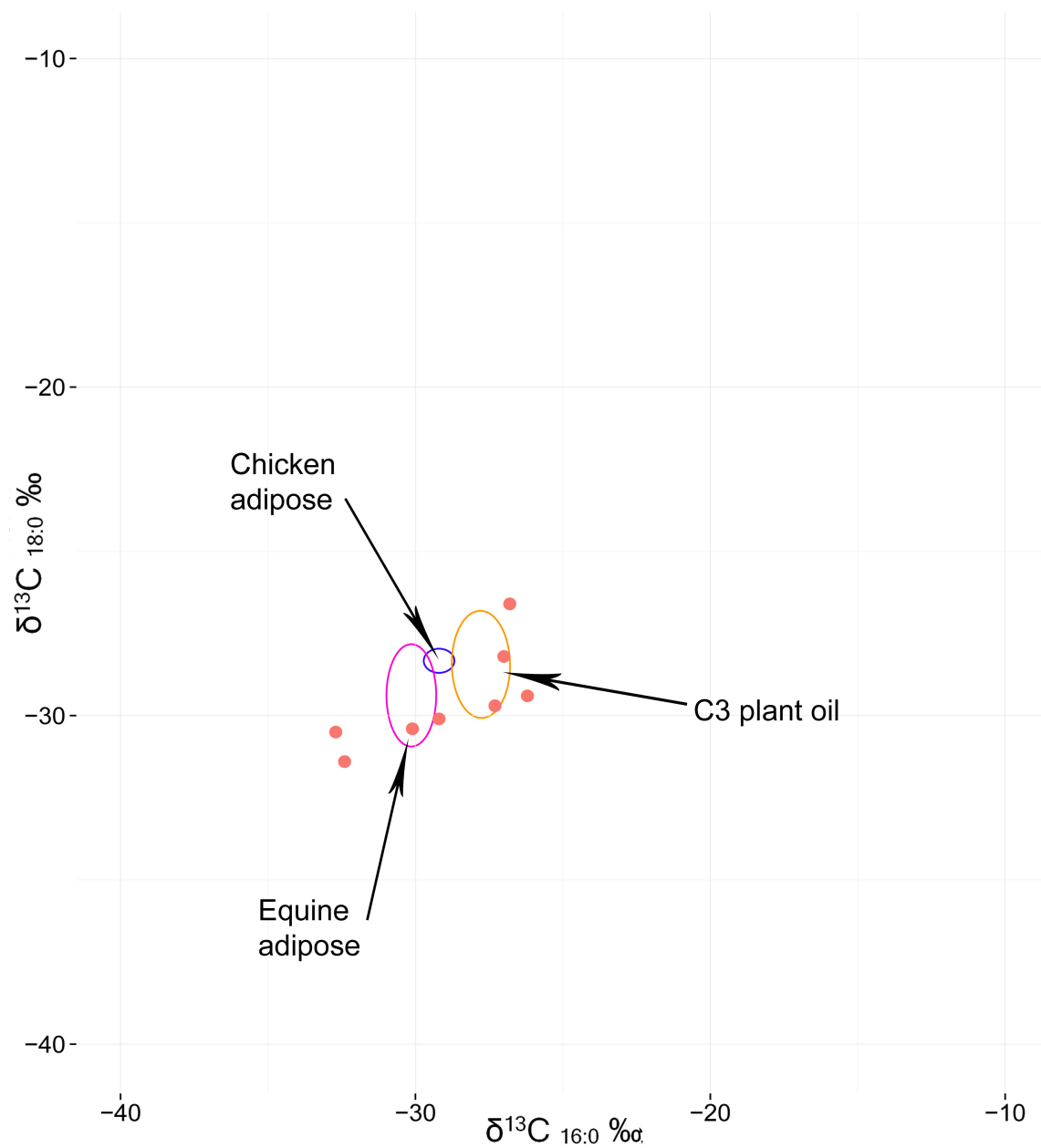
Figure 5.28: The results of CSIA by GC-C-IRMS of the samples from the Eupha-Ri site using the available references (cf. Dudd & Evershed, 1998; Dudd et al., 1999; Steele et al., 2010)
