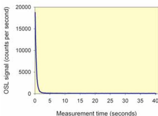
Figure 3.2: A typical optically stimulated luminescence signal from quartz grains (Duller, 2008)
