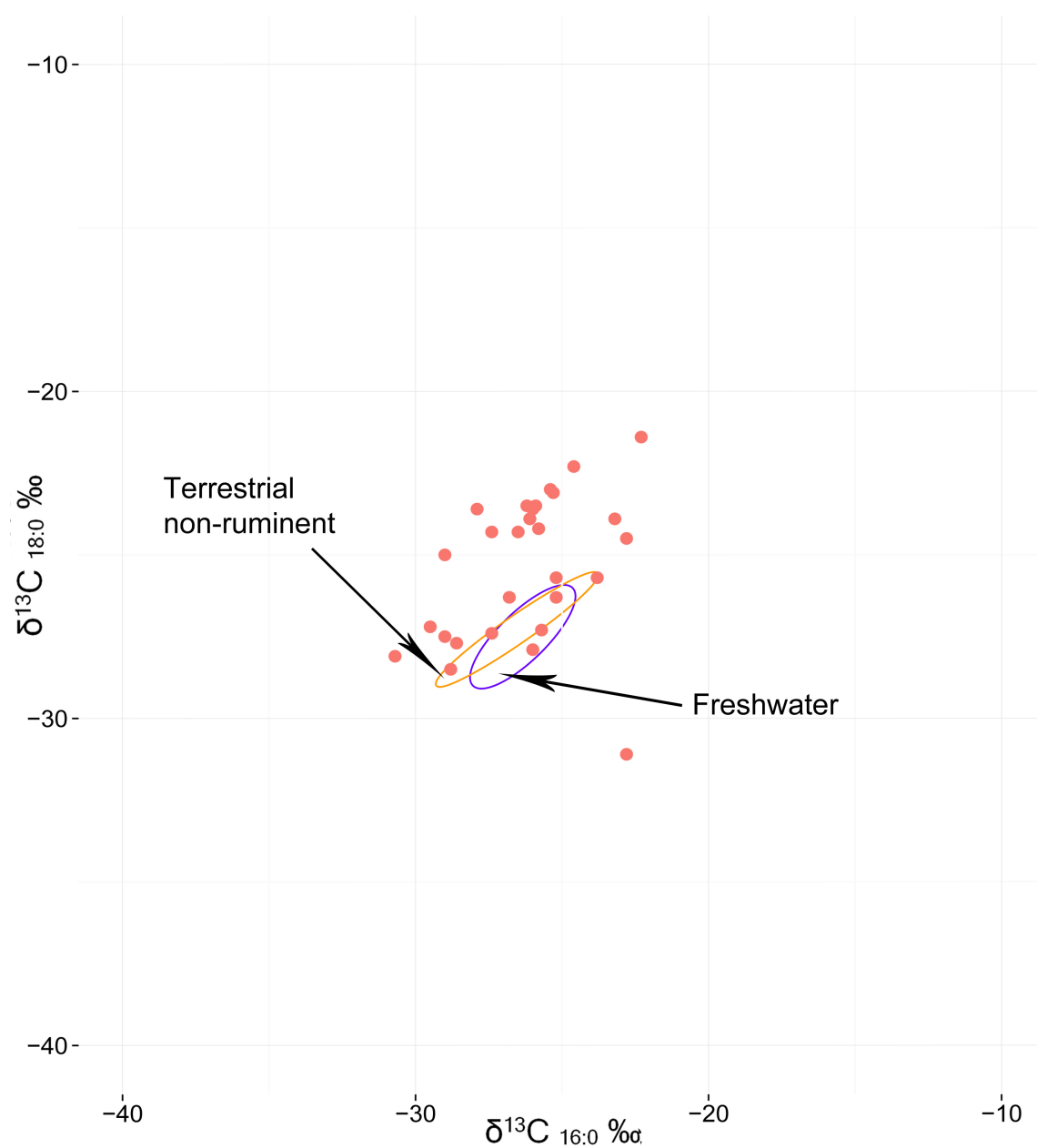
Figure 5.17: The results of CSIA by GC-C-IRMS of the samples from the Sosa-Dong site using the reference from Craig et al. (2013)
