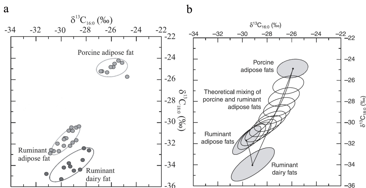
Figure 4.5: Interpretation of the results of CSIA (a): \delta^{13}\text{C} values acquired from the \text{C}_{16:0} and \text{C}_{18:0} fatty acids in archaeological potsherds are plotted along with the reference animal fat ellipses (Evershed, 2007) (b): The theoretical mixing curves between the porcine adipose fat, ruminant adipose fat and ruminant dairy fat are shown (Evershed et al., 2008)
