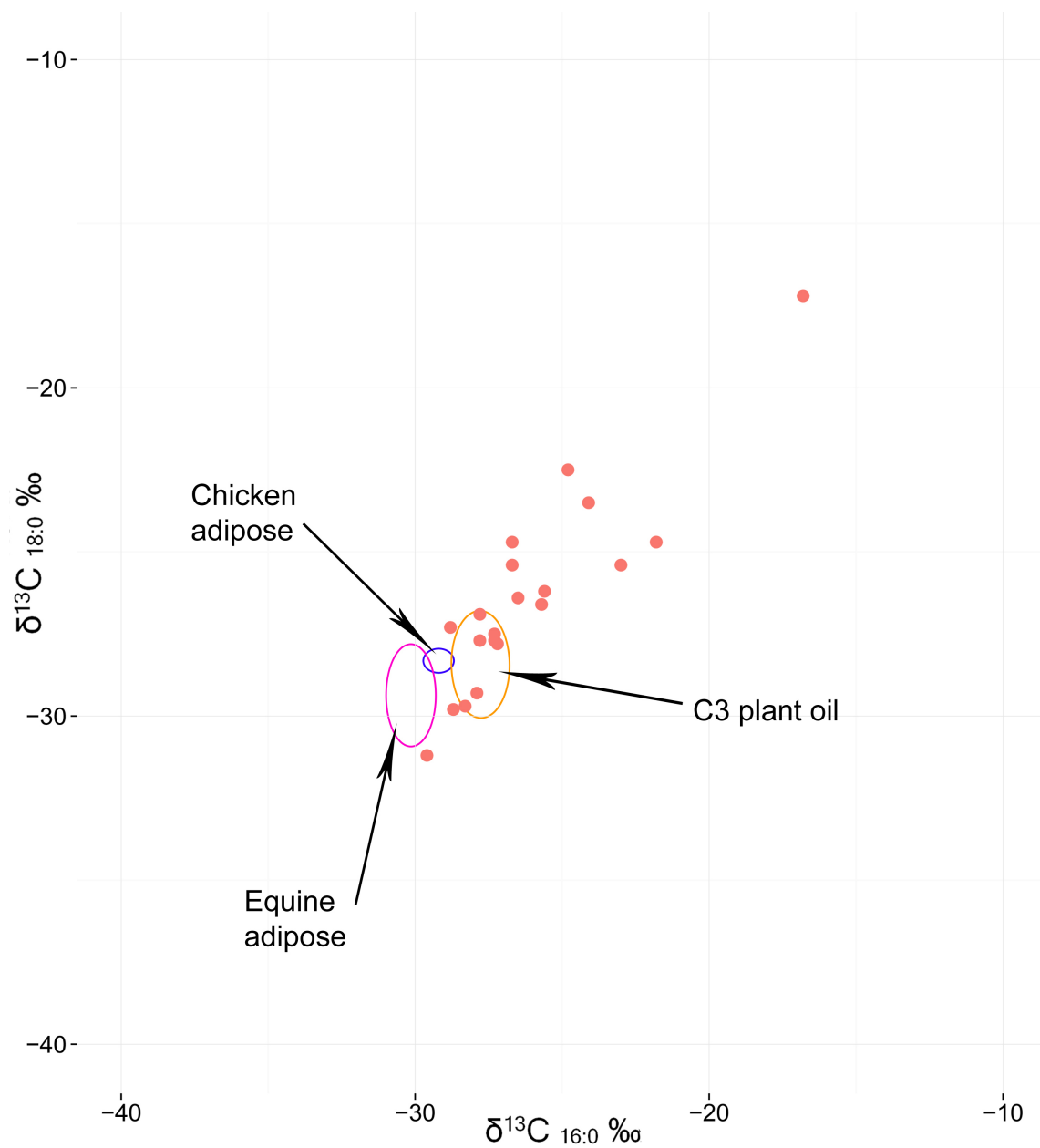
Figure 5.6: The results of CSIA by GC-C-IRMS of the samples from the Kimpo-Yangchon site using the available references (cf. Dudd & Evershed, 1998; Dudd et al., 1999; Steele et al., 2010)
