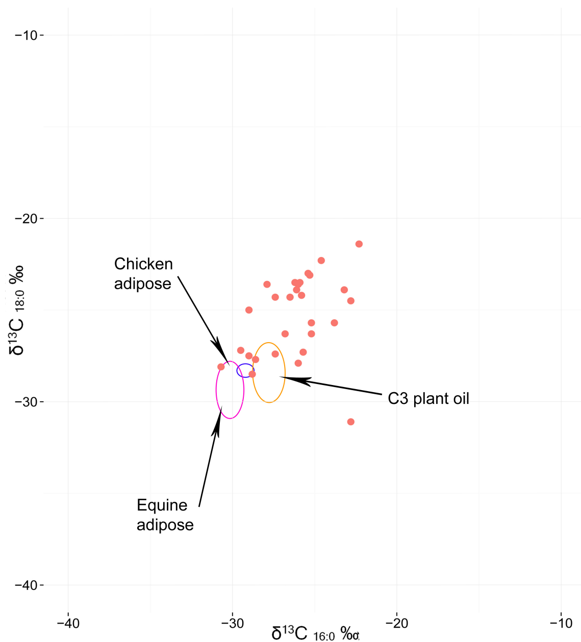
Figure 5.15: The results of CSIA by GC-C-IRMS of the samples from the Sosa-Dong site using the available references (cf. Dudd & Evershed, 1998; Dudd et al., 1999; Steele et al., 2010)
