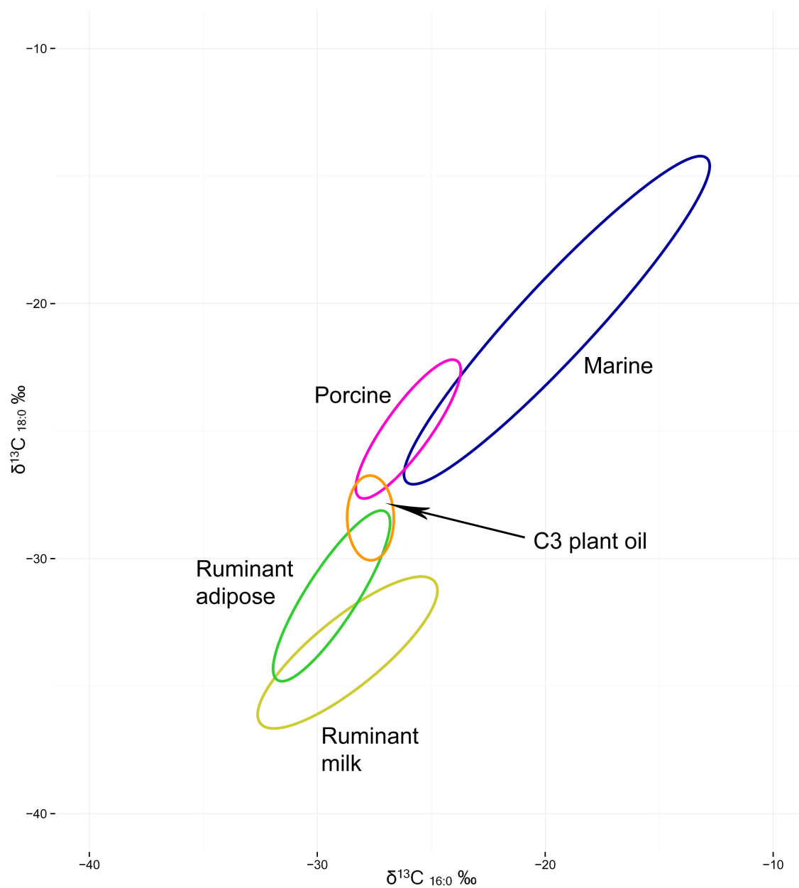
Figure 6.5: The ellipses of C 3 plant oil, pork adipose and ruminant adipose showing they overlap one another (cf. Craig et al., 2011; Steele et al., 2010)
