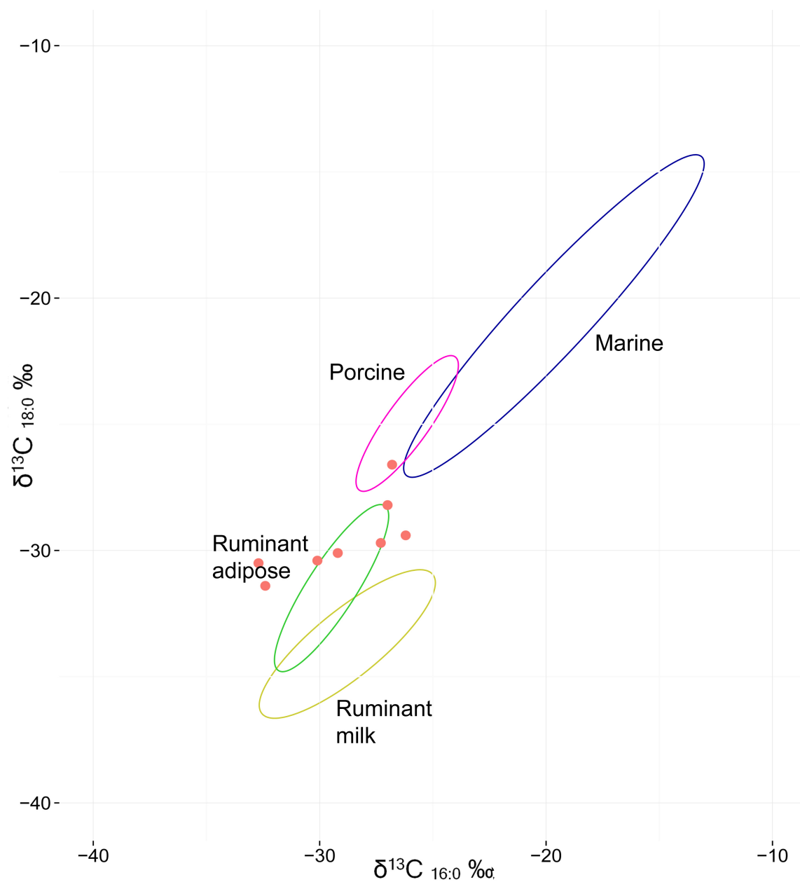
Figure 5.29: The results of CSIA by GC-C-IRMS of the samples from the Eupha-Ri site using the reference from Craig et al. (2011)
