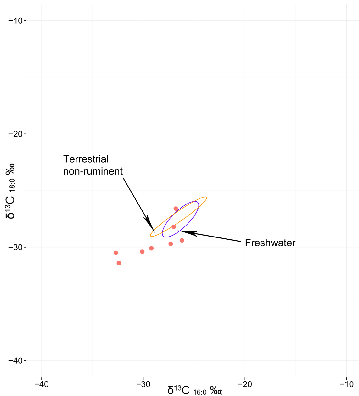
Figure 5.30: The results of CSIA by GC-C-IRMS of the samples from the Eupha-Ri site using the reference from Craig et al. (2013)
