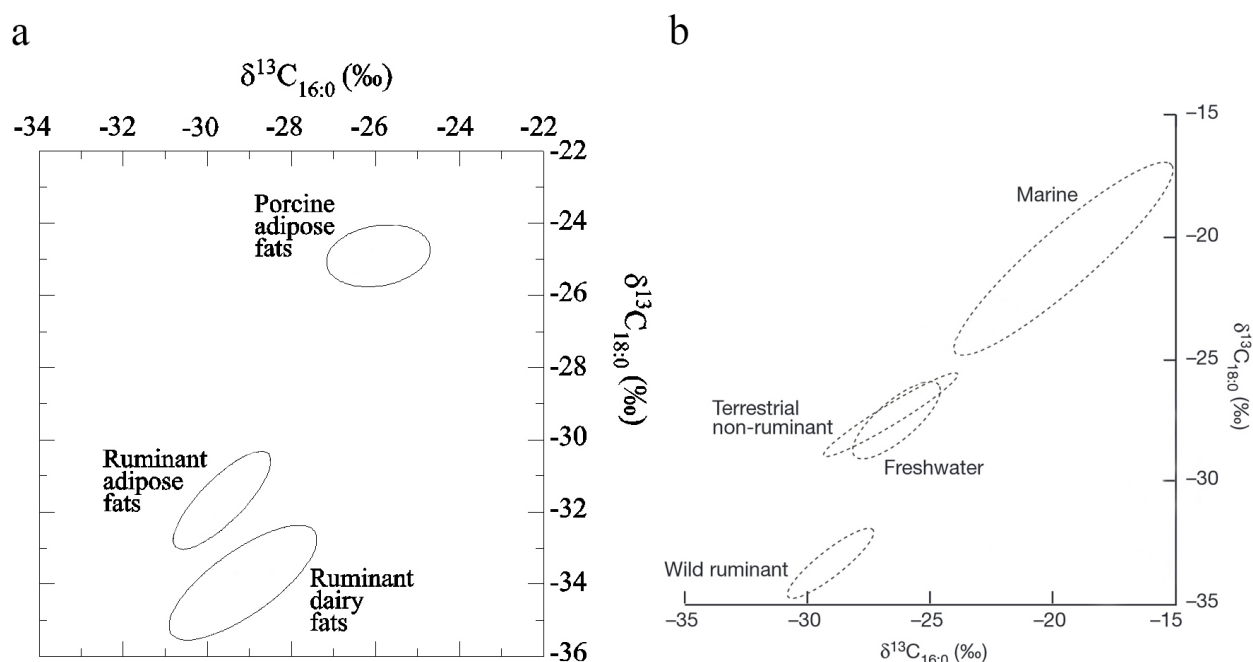
Figure 4.4: Reference database created based on modern fats for CSIA. (a): Only the animals having been reared on known diets were sampled (e.g. \text{C}_3 plant diet in order to mimic the prehistoric condition, absence of \text{C}_4 plants) (Copley et al., 2003; Dudd et al., 1998). (b): The modern reference samples were collected from authentic wild animals to avoid the effects of commercial farming and selective breeding (Craig et al., 2013). The \delta^{13}\text{C} values obtained from all modern reference animals were adjusted by the addition of 1.2 permil, considering post-Industrial Revolution effects of fossil fuel burning (Friedli et al., 1986).
