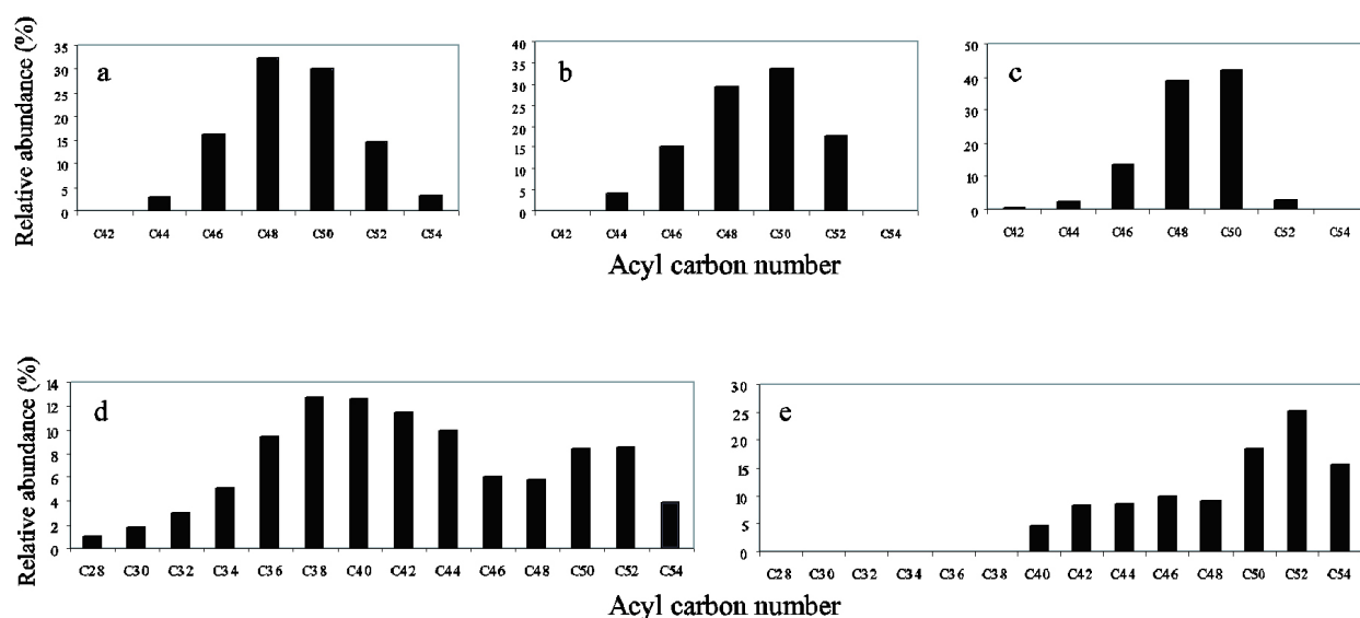
Figure 4.2: The distributions of TAGs in different kinds of animal fats (modified from Mukherjee, 2004: p. 20). (a): cow adipose fat (b): sheep adipose fat (c): pig adipose fat (d): fresh milk (e): milk degraded for 90 days
