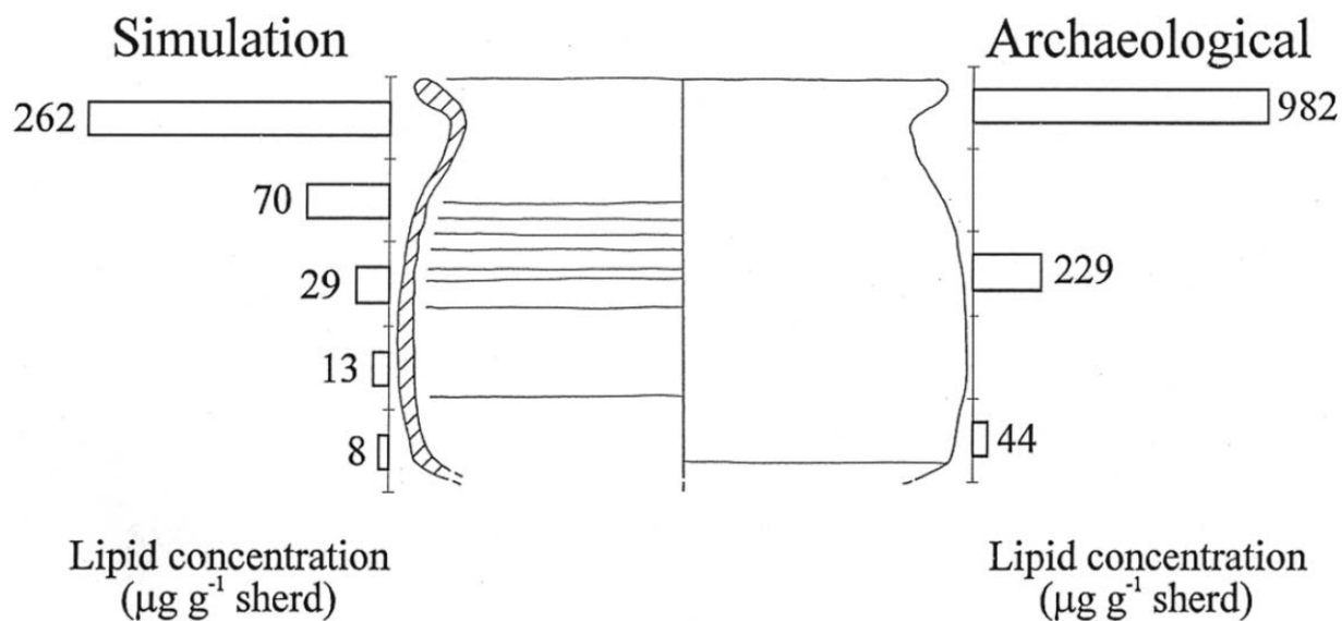
Figure 5.12: Diagram showing the lipid concentration of each body part from the both experimental and archaeological sherd samples (adapted from Evershed, 2008a)
