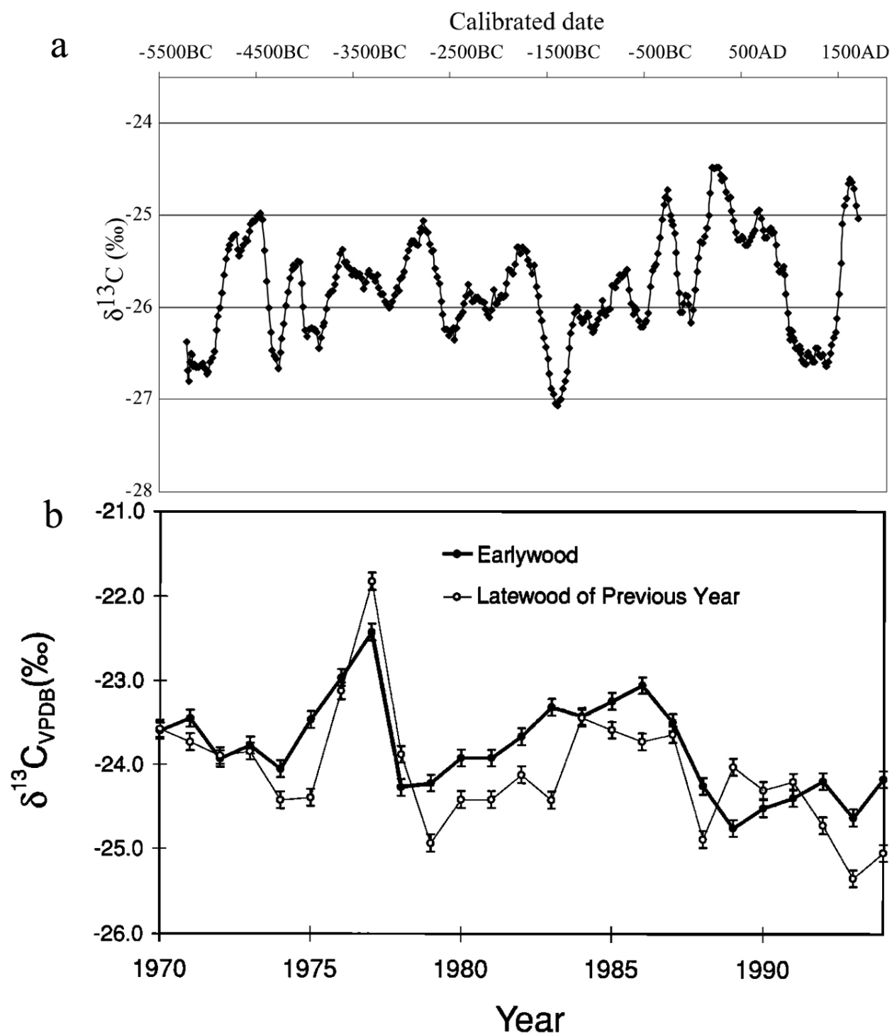
Figure 4.7: \delta^{13}\text{C} values of the cellulose from the oak tree-ring sequence (a): 11-year running mean from ancient Irish oaks (data obtained from McCormac, Baillie, Pilcher, Brown, & Hoper, 1994; Mukherjee, 2004) (b): Yearly measurement from 1970 to 1995 of modern oaks in east England (Robertson et al., 1997)
