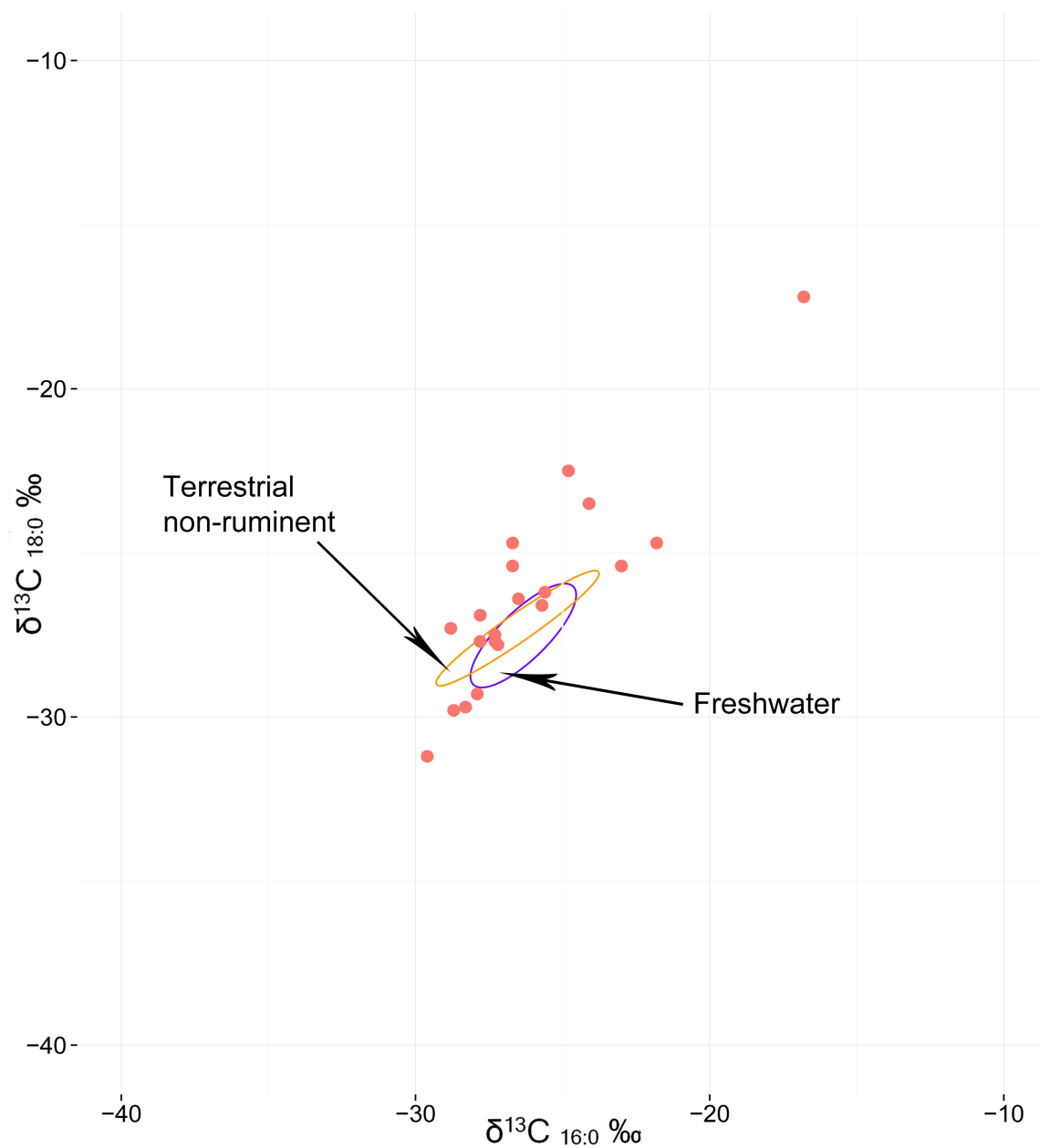
Figure 5.8: The results of CSIA by GC-C-IRMS of the samples from the Kimpo-Yangchon site using the reference from Craig et al. (2013)
