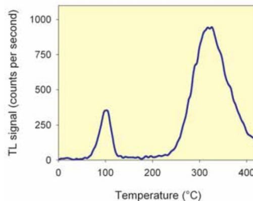
Figure 3.1: A typical thermoluminescence signal (commonly referred to as “glow curve”) that shows multiple traps (Duller, 2008; cf. Feathers, 2003: p. 1495)
