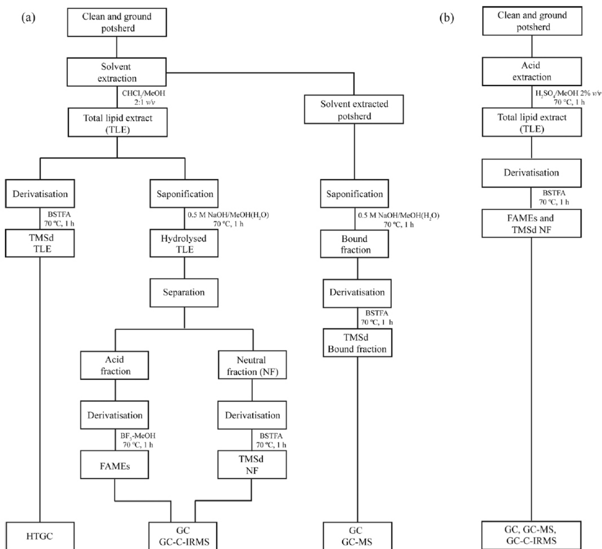
Figure 4.8: The comparison between (a) the solvent extraction protocol and (b) the acid extraction protocol (Correa-Ascencio & Evershed, 2014)
