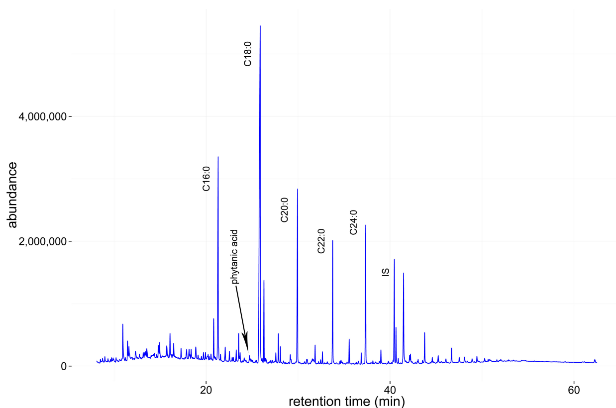
Figure 5.14: The result chromatogram of the GC-MS analysis of one of the samples from the Sosa-Dong site (SOSo49), using R version 3.2.0. Due to degradation, we usually observe medium- and long-chain saturated fatty acids. 5- \alpha Cholestane was added as an internal standard (IS = 132 ng / microliter)
