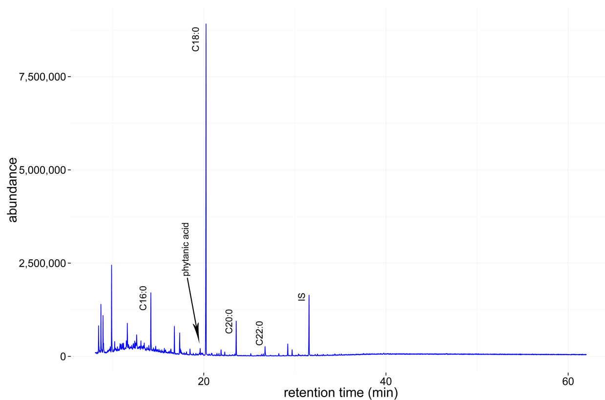
Figure 5.5: The result chromatogram of the GC-MS analysis of one of the samples from the Kimpo-Yangchon site (KIMo61), using R version 3.2.0. Due to degradation, we usually observe medium- and long-chain saturated fatty acids. \gamma -Cholestane was added as an internal standard (IS = 132 ng / microliter)
