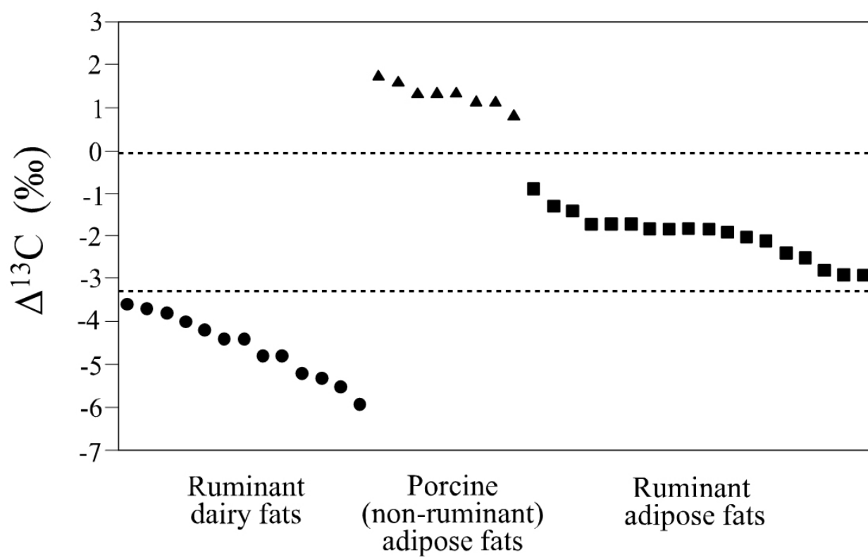
Figure 4.6: Plots showing the difference in \delta^{13}\text{C} values of the C18:o and C16:o fatty acids ( \Delta^{13}\text{C} = \delta^{13}\text{C}_{\text{C18:o}} - \delta^{13}\text{C}_{\text{C16:o}} ) obtained from the modern reference fats (Copley et al., 2003)
