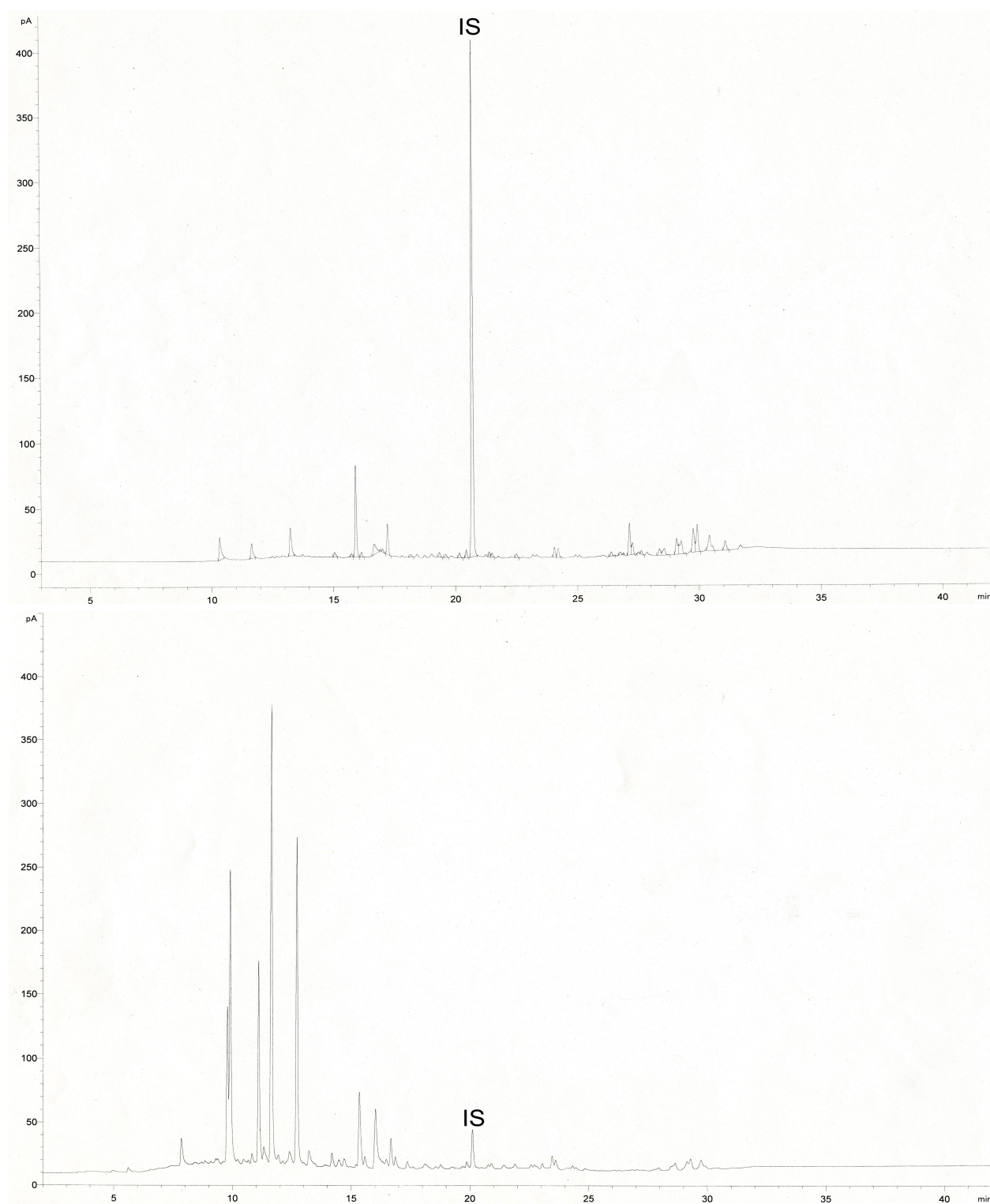
Figure 4.9: The GC chromatograms of the same archaeological sherd sample (KIMo14) showing different recovery rates. (a) chloroform : methanol solvent extraction (b): acidified methanol extraction (IS = Internal Standard). In both extractions, the same amount of internal standard was injected. The acidified extraction method showed a much higher recovery rate (more than 20 times) compared with the prevailing chloroform/methanol solvent extraction protocol.
