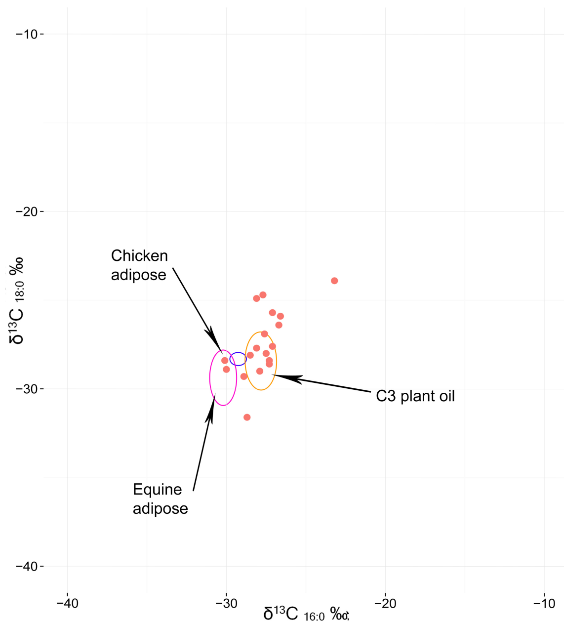
Figure 5.21: The results of CSIA by GC-C-IRMS of the samples from the Songguk-Ri site using the available references (cf. Dudd & Evershed, 1998; Dudd et al., 1999; Steele et al., 2010)
