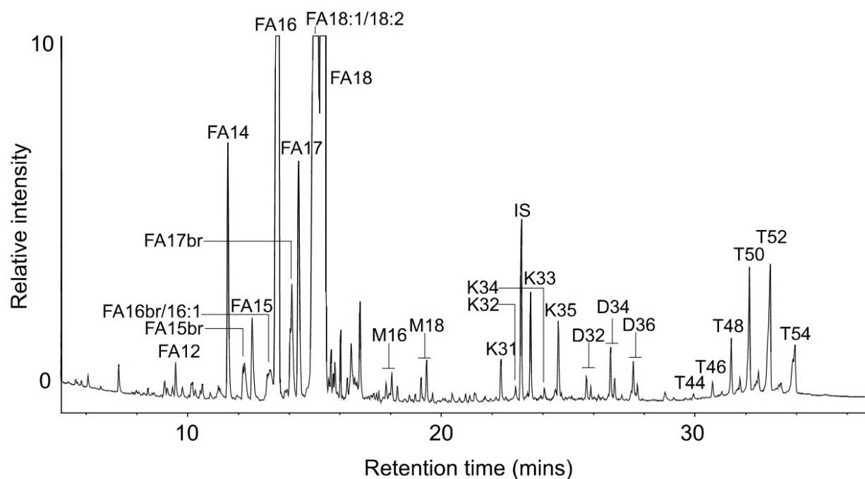
Figure 4.1: partial HTGC profile of the lipid extract from a Romano-British sherd from Stanwick, Northamptonshire (Evershed et al., 2002). A low abundance of intact TAGs are observed at retention times above 30 min. The majority of them was hydrolyzed during vessel use or burial, resulting in the formation of DAGs, MAGs, and free fatty acids. Key: IS = internal standard (n-tetratriacontane). IS was added to the sample at the extraction stage for quantification of lipid. The extracts are trimethylsilylated.
