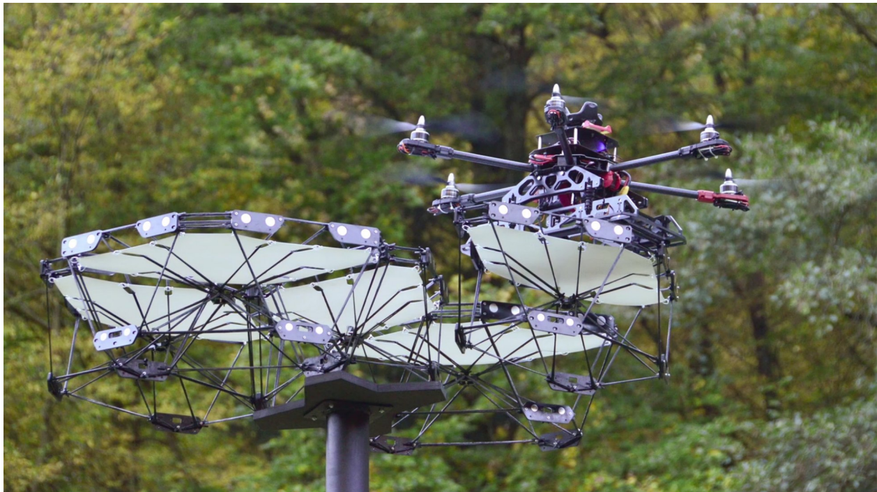
Figure 12 Reconfigurable architectural system - Source: University of Stuttgart
