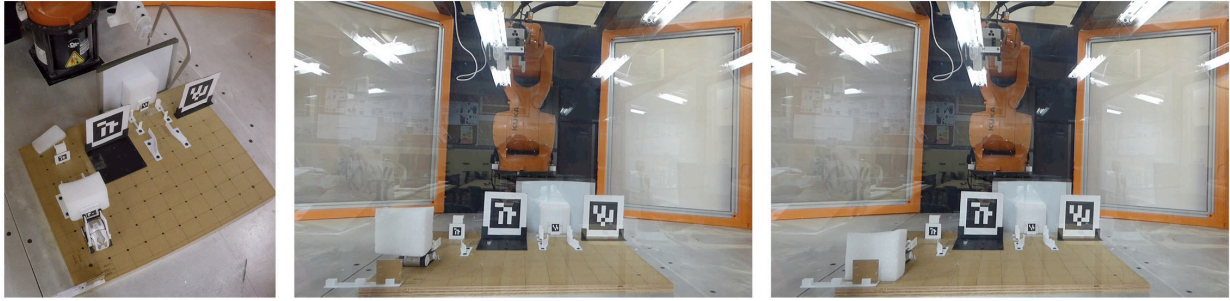
Figure 29 Putting down the block
