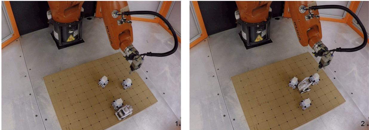
Figure 30 Obstacle avoidance of recognized objects
