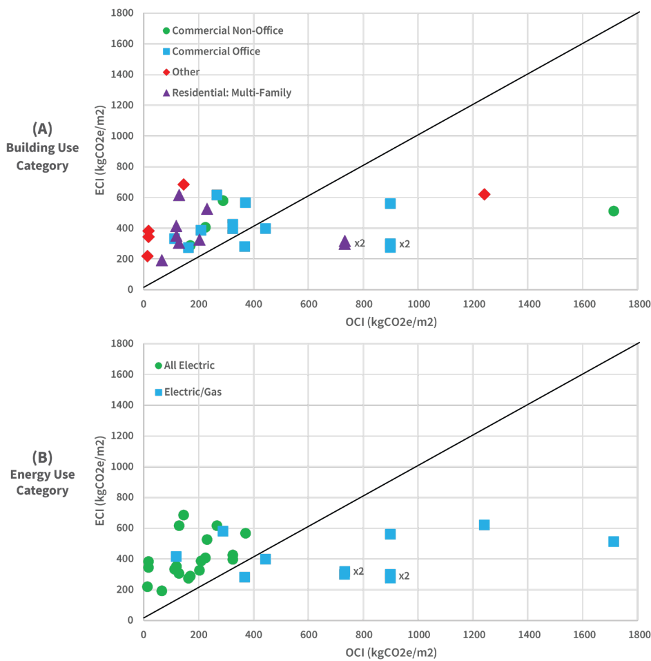
Figure B1. Embodied carbon intensity (ECI) and operational carbon intensity (OCI) under different building categorizations. Results are shown for all buildings by building use category (A) and energy use category (B) as symbols. Points above the diagonal line indicate projects whose ECIs were larger than OCIs at and, below the line, projects whose OCIs were greater.
