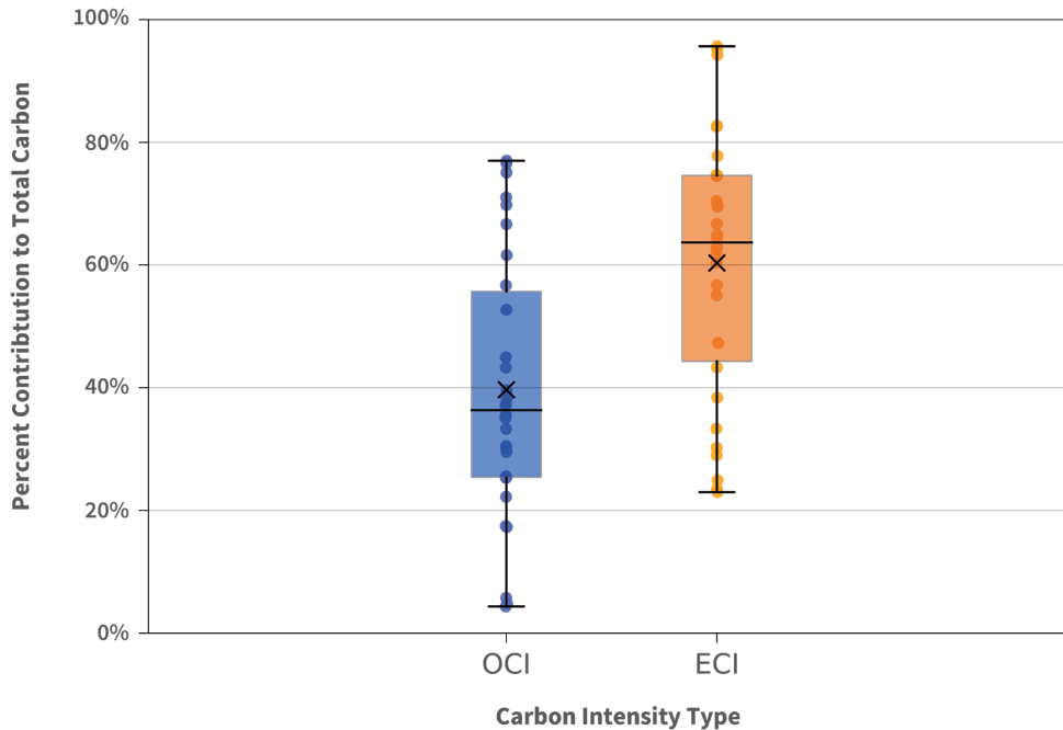
Figure 10. Percentage contribution of operational and embodied carbon to whole life carbon impacts for all buildings. Buildings assessed over a 60-year reference study period. Mean values are shown with a cross (x) and median values with a horizontal solid line within the box plots.
