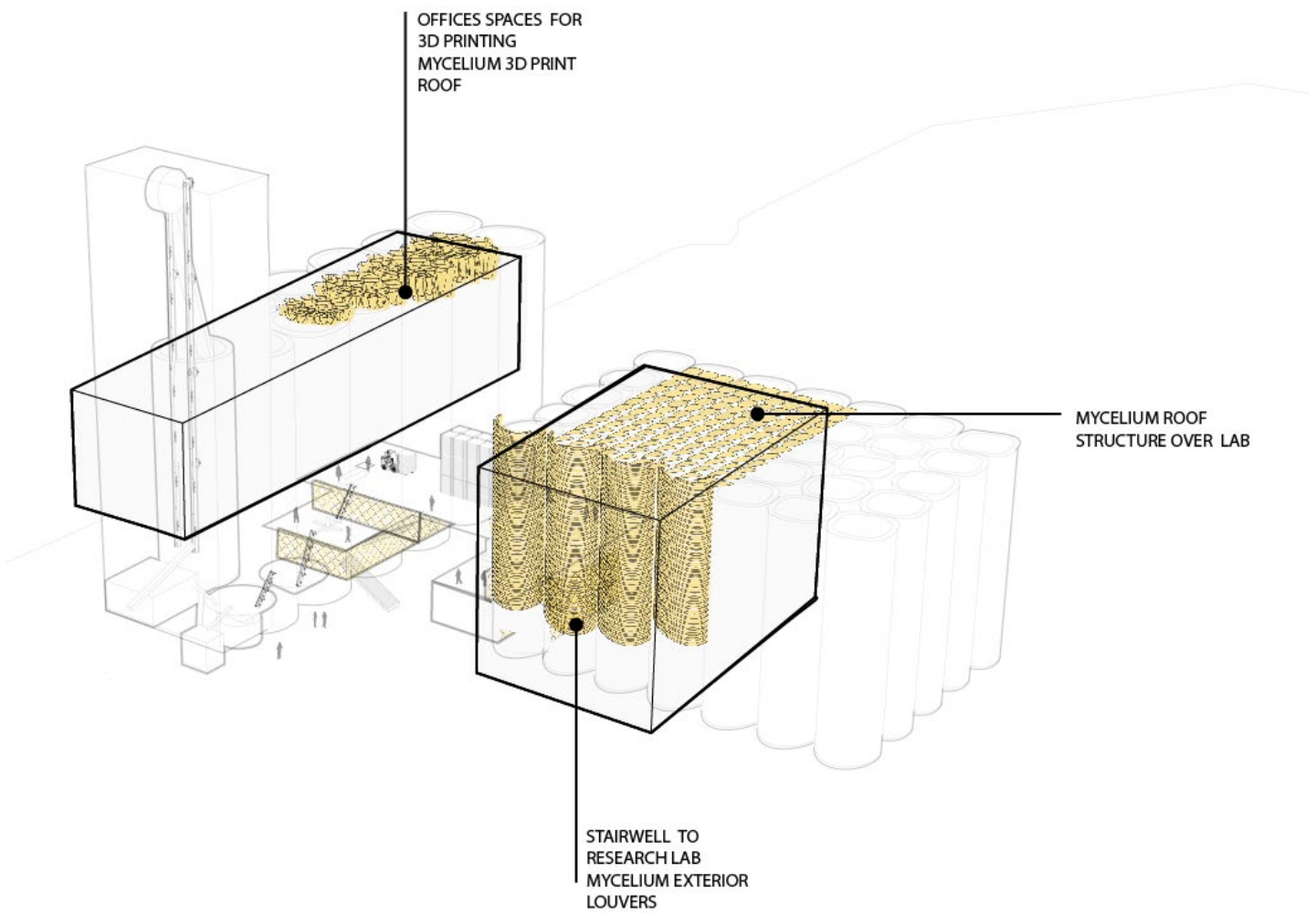
Figure 62: Phase 2 enlarged building axon
