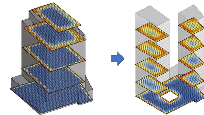
Figure 34 - Comparison of daylight availability in two massing designs. In the new massing proposal, better daylighting scheme is achieved at all floors of the building.
