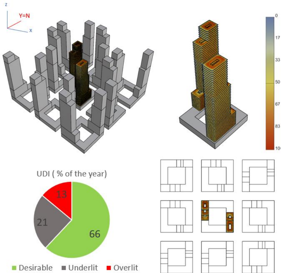
Figure 65 - Step 5 - Simulation result for the informed design phase (changing parameter is removing circulation area)
