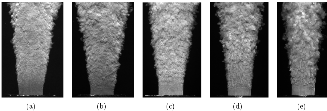
Figure 3.31: Images of jets issuing from a 4 mm convergent nozzle at 12.6 m/s; the jet viscosity is (left to right) 0.5 cP, 1 cP, 2 cP, 10 cP, 100 cP
