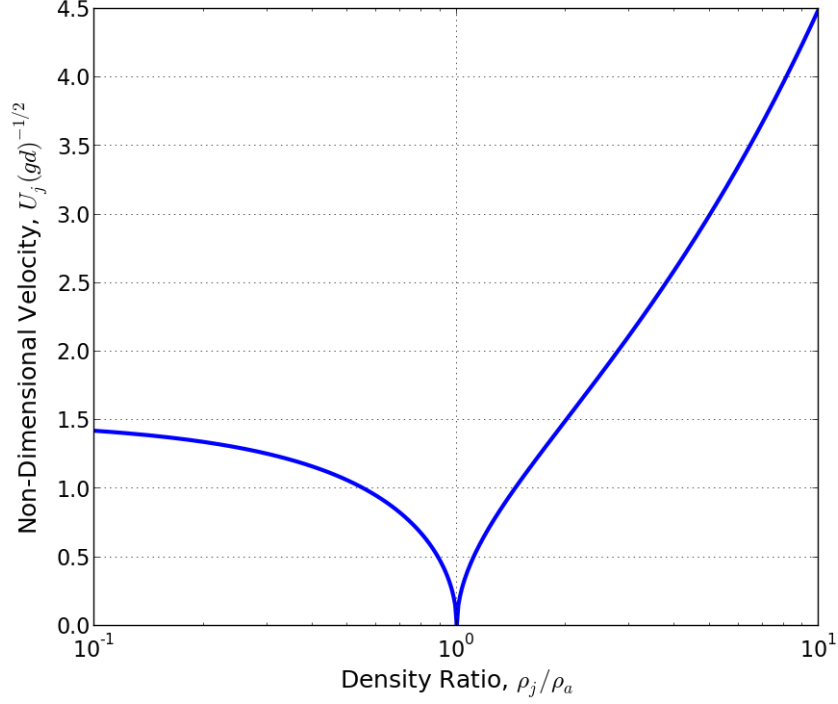
Figure 3.30: Plots the minimum non-dimensional velocity ( U_j(gd)^{-1/2} ) required for P > 1 as a function of the jet density ratio ( \rho_j/\rho_a )
