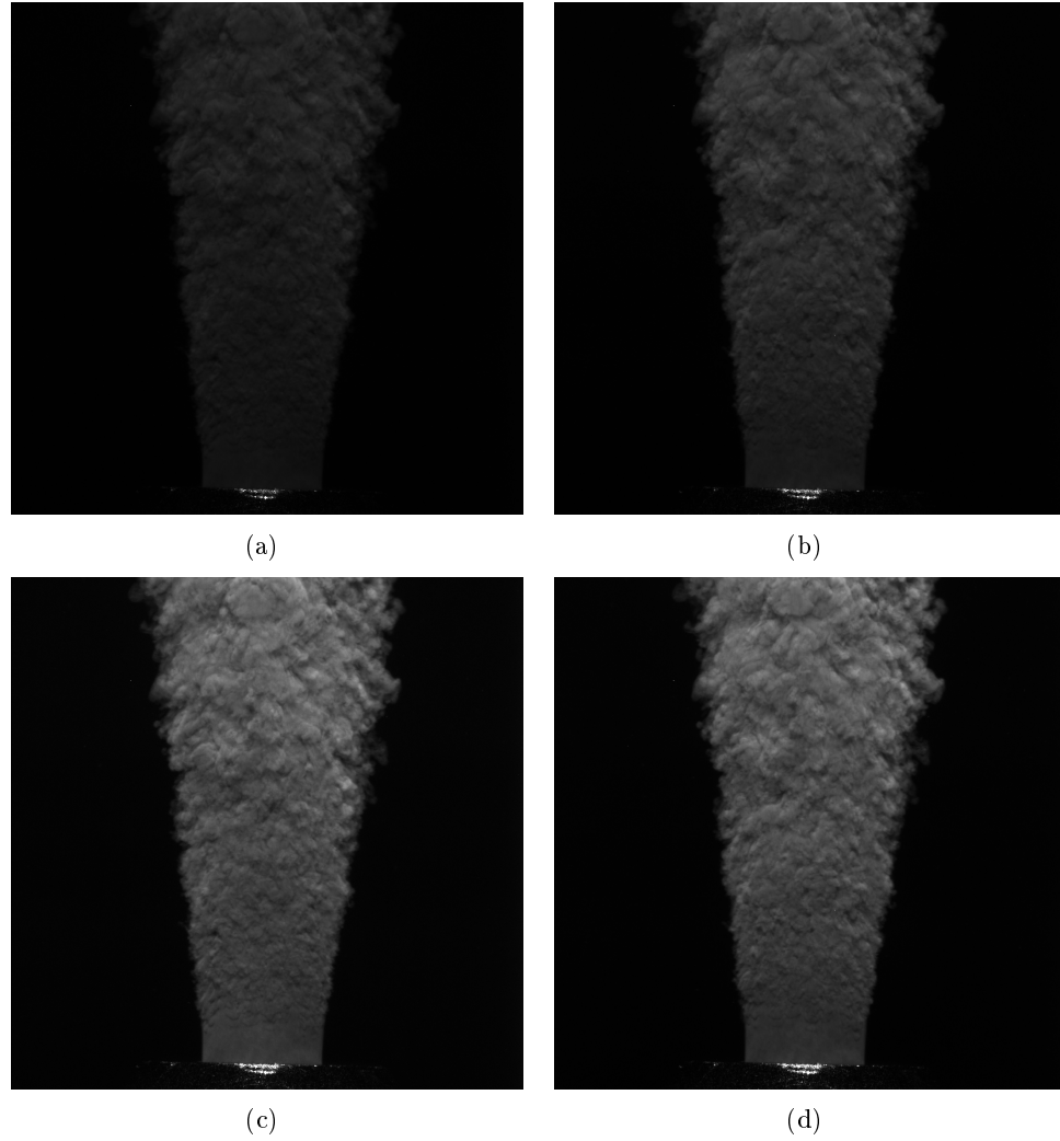
Figure 3.23: Image pairs ( \delta t = 120 \mu s ) of an illuminated Rhodamine-dyed water jet ( Re = 50,000 ) interface both before (top) and after (bottom) contrast normalization via ImageJ
