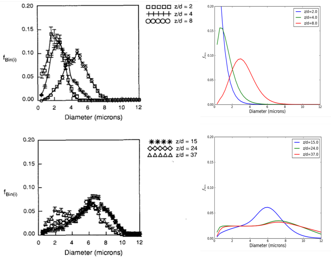
Figure 5.9: Comparison of experimental and model results of droplet diameter distribution at the jet centerline for various downstream positions for a saturated 85 °C jet
