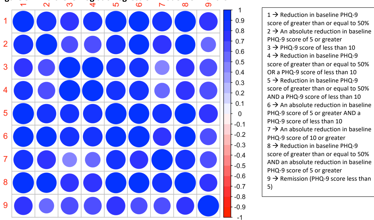
Figure S1: Multilevel Logistic Regression Model - 3 Months
