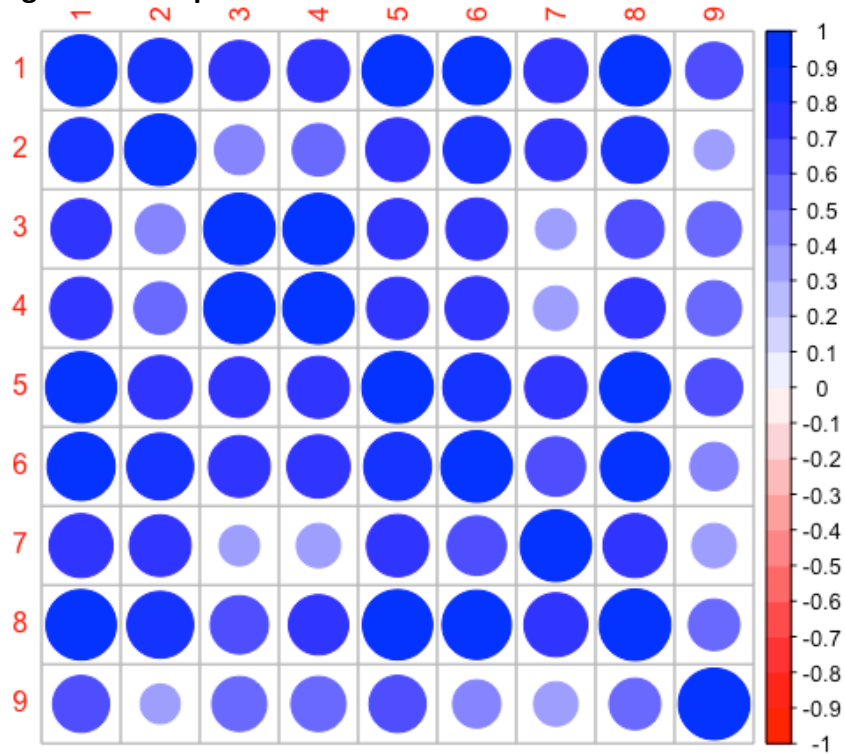
Figure S3: Sample Means - 3 Months
