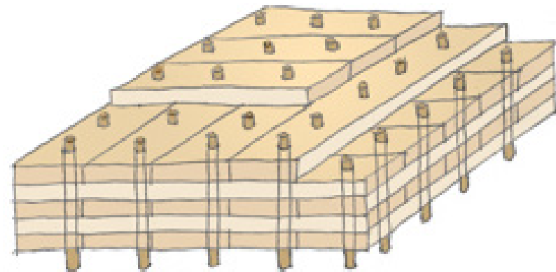
Figure 35 Brettstapel Construction
