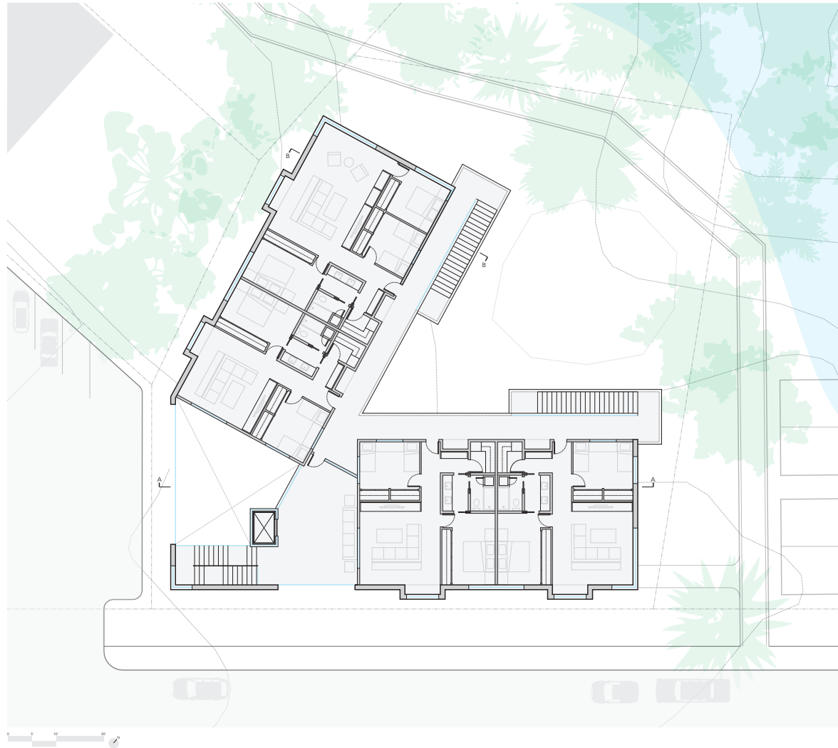
Figure 46 Third, Fifth Floor Plan
