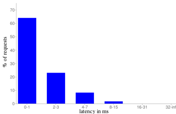
Figure 3.11: Latency without client certificates
