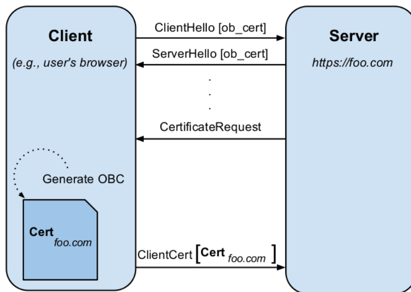
Figure 3.1: TLS-OBC extension handshake flow.
