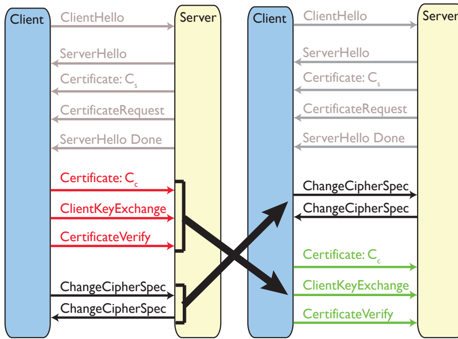
Figure 3.15: TLS encrypted client certificates
