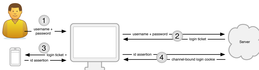
Figure 4.1: PhoneAuth overview
