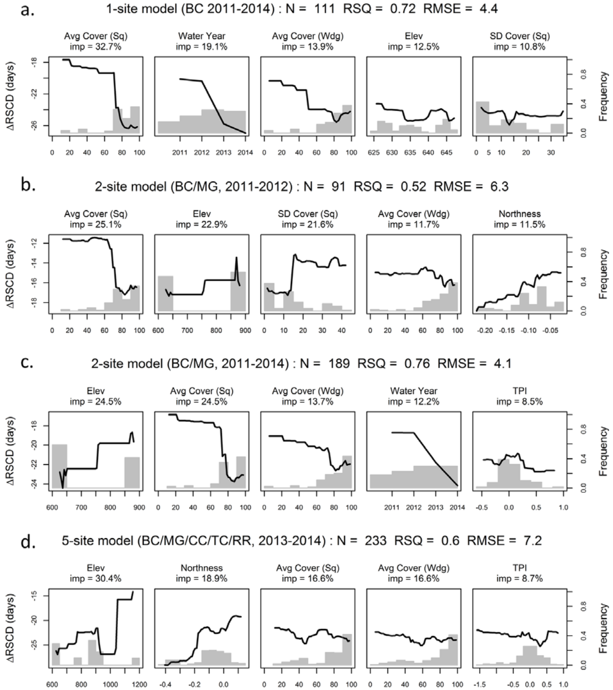
Figure 7.7 Partial plots from Random Forest model fitted to a suite of canopy and topographic predictor variables for snow duration observations ( \Delta\text{RSCD} , computed as snow duration in a reference open location minus snow duration at a sample location), where the black line shows the snow duration response to an individual predictor variable across the range of predictor values with all other predictors held constant at their mean values. The gray histogram indicates the frequency distribution of predictor values in the dataset. The subplots display the results for
