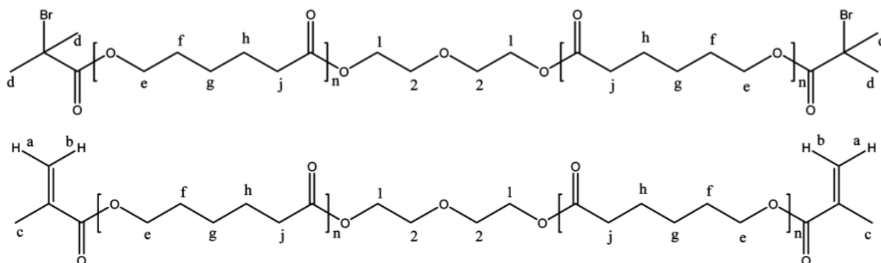
Fig. 4. Designed caprolactone-based degradable ATRP initiator (top) and crosslinker (bottom). (Atzet et al., 2008)
