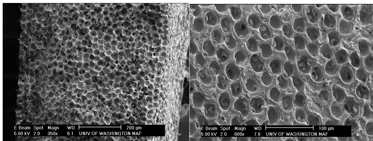
Fig. 7. Scanning electron microscope images of porous caprolactone-based pHEMA.
