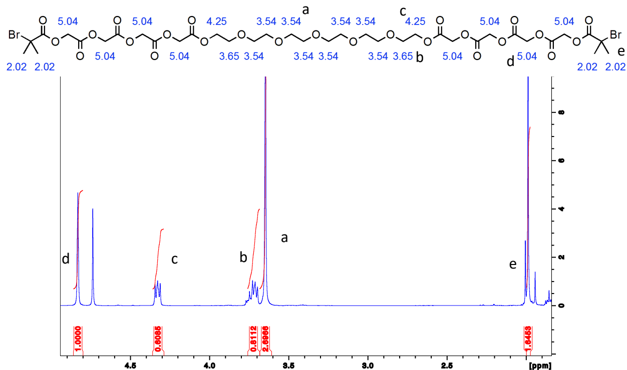
Fig. 9. NMR of glycolide-based degradable ATRP initiator.
