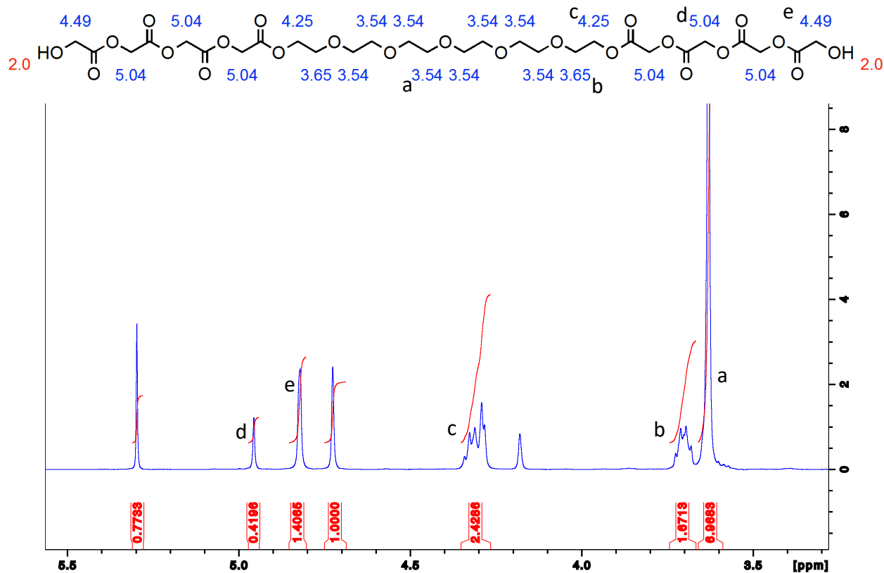
Fig. 11. NMR of glycolide-based degradable diol.
