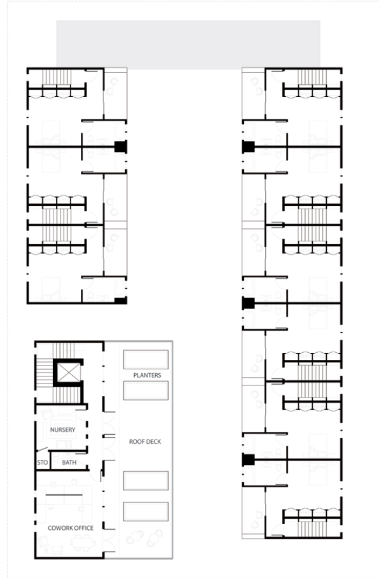
LEVEL 3 PLAN
