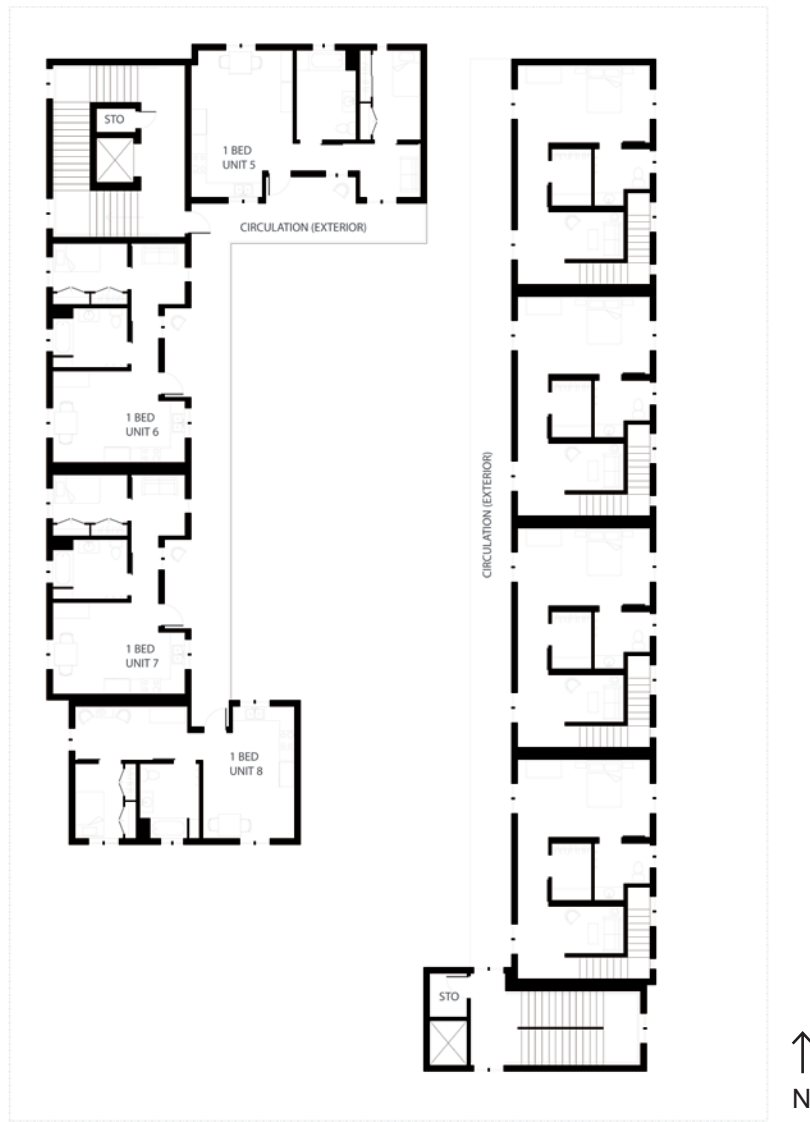
LEVEL 2 PLAN
