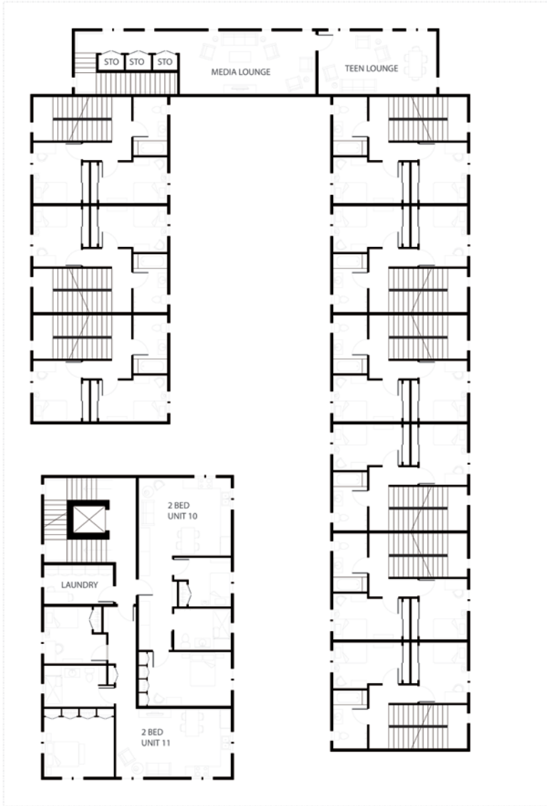
LEVEL 2 PLAN
