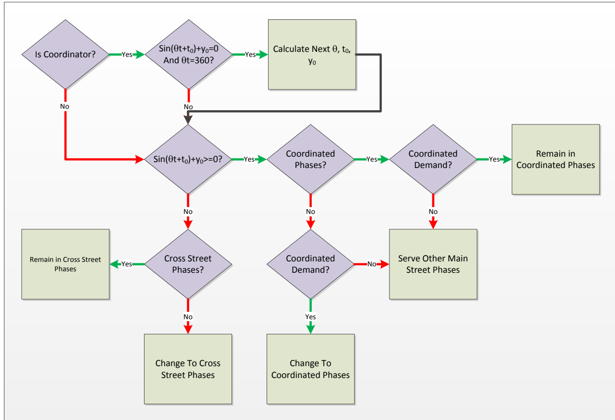
Figure 7-5: Coordinator and Corridor Control Logic
