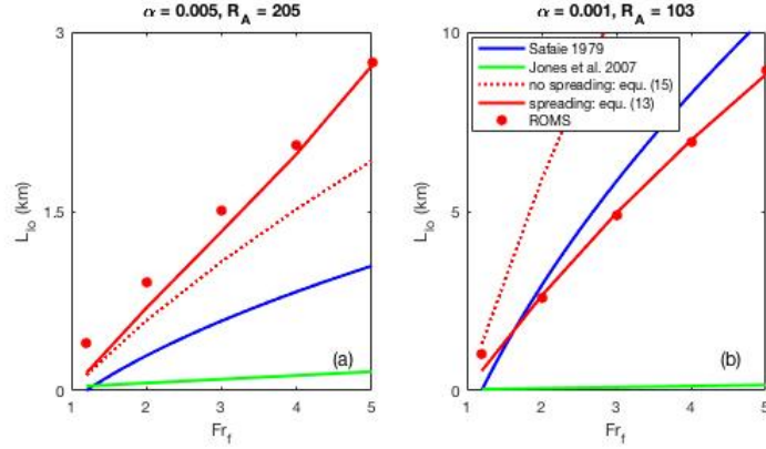
Figure 3.10: Liftoff length comparison of equation predictions to ROMS estimates for (a) \alpha = 0.005 and R_A = 205 and (b) \alpha = 0.001 and R_A = 103
