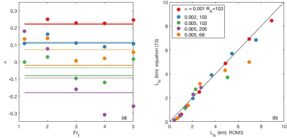
Figure 3.12: Estimations of the spreading parameter and its effect on L_{lo} calculations (a) \kappa as a function of \alpha , R_A , and Fr_f . Solid lines are the \kappa values determined by minimizing the difference between the liftoff lengths calculated with (3.13) and the ROMS estimates of L_{lo} . Circles are calculated from the freshwater flux, dashed lines are averages of the circle values over Fr_f . (b) Liftoff lengths calculated with equation (3.13) and \kappa from the freshwater flux calculation vs. liftoff lengths estimated from the ROMS output.
