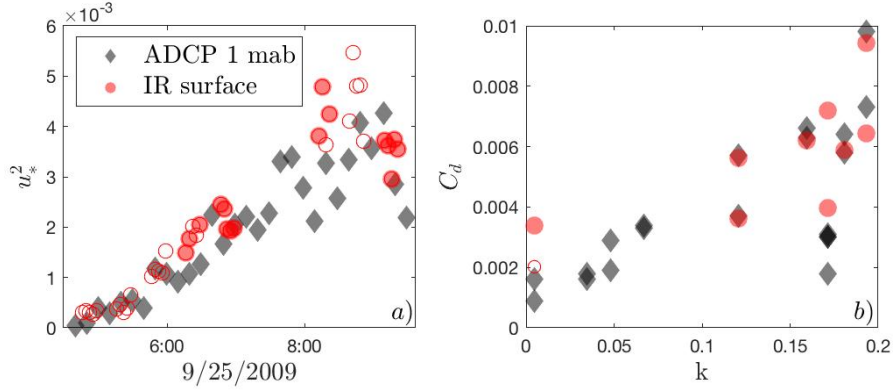
Figure 4.9: (a) Friction velocity calculated using ADCP data 1 mab (equation 4.6) and IR surface TKE data (equation 4.18) for a sample tide. Open circles indicate the R^2 of a fit of the IR velocity spectra to f^{-5/3} was below 0.9 and filled circles indicate R^2 was greater than 0.9. b) C_d calculated as the slope of u'w' vs. u(u^2 + v^2)^{1/2} for all 20 tides with the ADCP 1 mab and C_d calculated with IR TKE data using equation (4.19). The open circle indicates the R^2 of a fit of the IR velocity spectra to f^{-5/3} was above 0.88 and the filled circles indicate R^2 > 0.9 .
