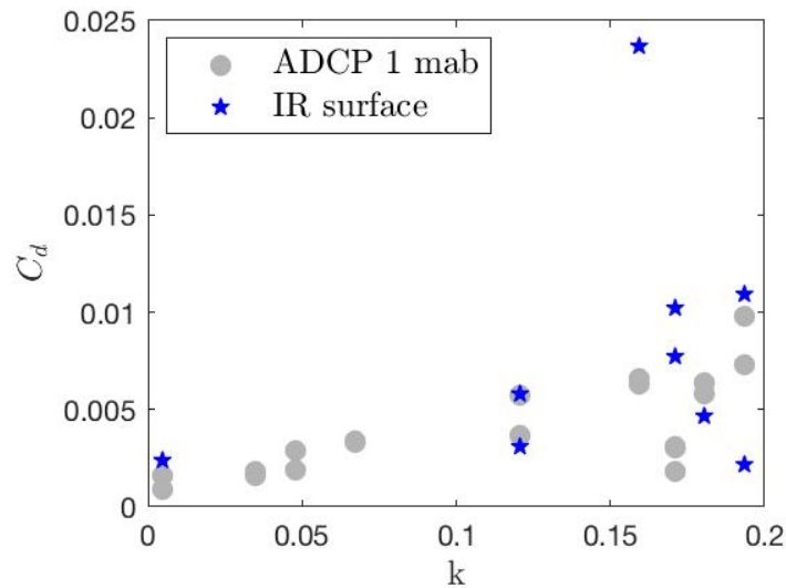
Figure 4.13: Comparison of C_d calculated with remotely sensed IR surface \overline{u'v'} data (equation 4.13) and ADCP \overline{u'w'} data measured 1 mab (equation 4.8).
