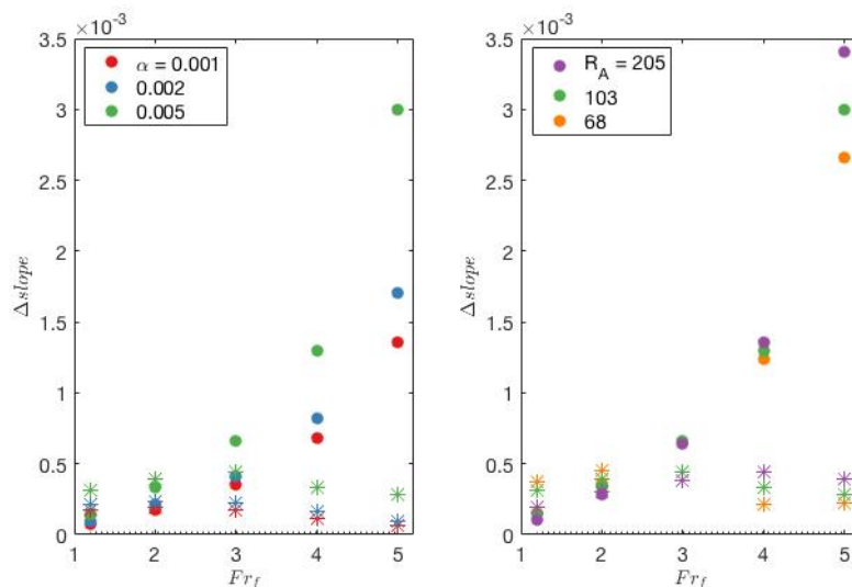
Figure 3.14: Water surface slope changes at the river mouth (filled circles) and at the ridge peak (stars) for (a) three shelf slopes and (b) three river mouth aspect ratios. The predicted SWOT slope accuracy of 1.7 \times 10^{-5} is plotted as a dotted line.
