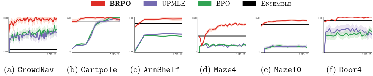
Figure 7.5: Training curves. BRPO dramatically outperforms agents that do not leverage expert knowledge (BPO, UP-MLE), and significantly improves the ensemble of experts.
