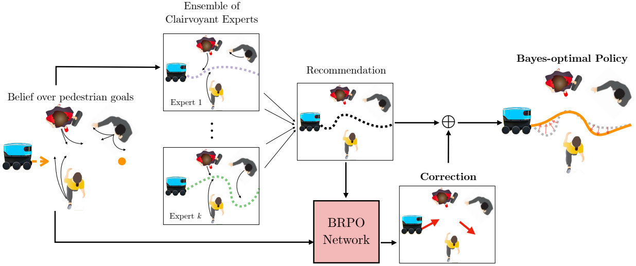
Figure 7.1: An overview of Bayesian Residual Policy Optimization. (a) Pedestrian goals are latent and tracked as a belief distribution. (b) Experts propose their solutions for a scenario, which are combined into a mixture of experts. (c) Residual policy takes in the belief and ensemble’s proposal and returns a correction to the proposal. (d) The combined BRPO and ensemble policy is Bayes-optimal.
