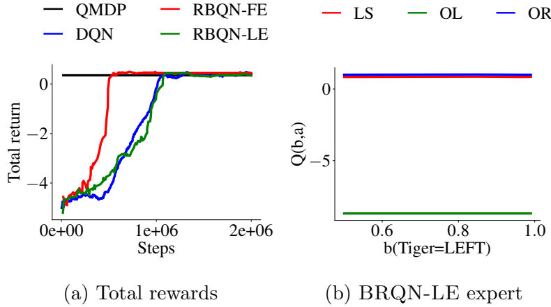
Figure 6.2: Tiger. (a) BRQN-FE converges quickly to the optimum. (b) BRQN-LE produces experts specialized in one MDP, which opens one of the doors deterministically.
