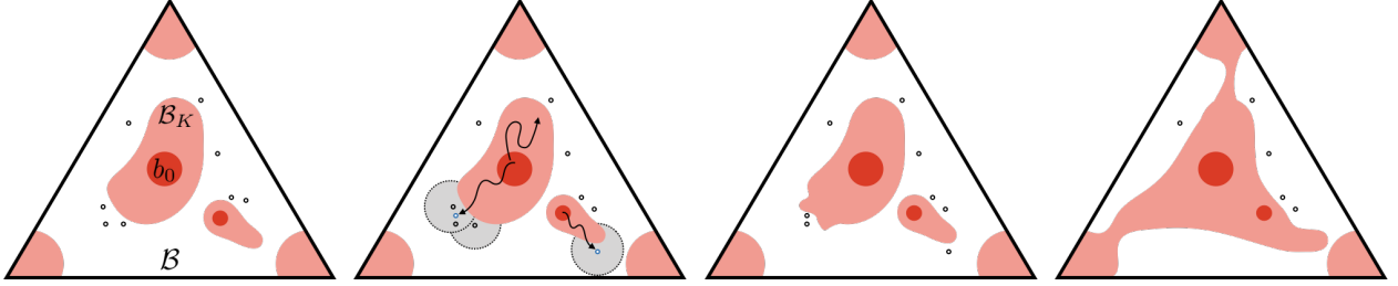
Figure 5.1: The BCPACE algorithm for BAMDPs. The vertices of the belief simplex correspond to the latent MDPs constituting the BAMDP model, for which we can precompute the optimal Q-values. During an iteration of BCPACE, it executes its greedy policy from initial belief b_0 , which either never escapes the known belief MDP \text{BELIEF MDP}_K or leads to an unknown sample. Adding the unknown sample to the sample set may expand the known set K and the known belief MDP \text{BELIEF MDP}_K . The algorithm terminates when the optimally reachable belief space is sufficiently covered.
