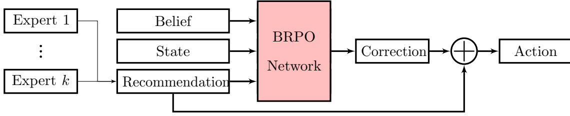
Figure 7.2: Bayesian residual policy network architecture.
