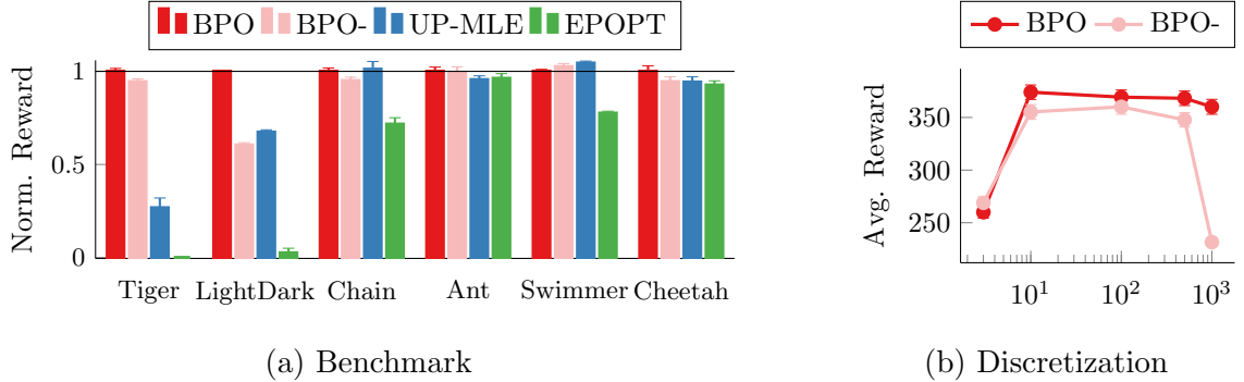
Figure 4.2: (a) Comparison of BPO with belief-agnostic, robust RL algorithms. BPO significantly outperforms benchmarks when belief-awareness and explicit information gathering are necessary ( Tiger , LightDark ). It is competitive with UP-MLE when passive estimation or universal robustness is sufficient ( Chain , MuJoCo ). (b) Scalability of BPO with respect to latent state space discretization for the Chain problem.
