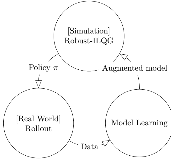
Figure 3.1: GP-ILQG overview
