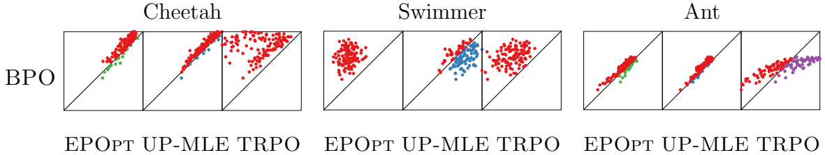
Figure 4.5: Pairwise performance comparison of algorithms on MuJoCo BAMDPs. Each point represents an MDP, and its (x, y) -coordinates correspond to the long-term reward by (baseline, BPO). The farther a point is above the line y = x , the more BPO outperforms that baseline. Colors indicate which algorithm achieved higher reward: BPO (red), EPOPT (green), UP-MLE (blue), or TRPO (purple).
