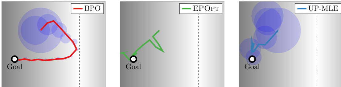
Figure 4.3: Visualization of different algorithms on the LightDark environment. The dashed line indicates the light source. Blue circles are one standard deviation for per-step estimates. The BPO policy moves toward the light to obtain a better state estimate before moving toward the goal.
