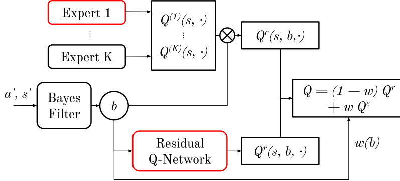
Figure 6.1: Network overview. State s is an input to every module, and s', a' are the state and action from the previous step. Red is one example of trained modules per sample batch. Samples from \mathcal{M}^k are only used to train expert k , while the Residual Q-network is trained with samples from all MDPs.
