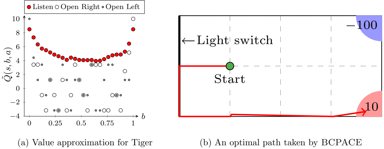
Figure 5.2: With greedy exploration, only best actions are tightly approximated (Figure 5.2a). BCPACE takes optimal actions for a continuous BAMDP (Figure 5.2b).
