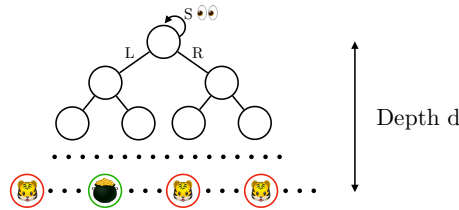
Figure 2.1: A tree-like MDP that highlights the distinction between BRL and PSRL.
