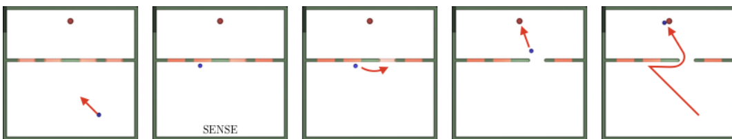
(c) Door4 . The agent senses only when it is near the wall with doors, where sensing is most accurate. The transparency of the red bars indicates the posterior probability that the door is blocked. With sensing, the agent notices that the third door is open.
