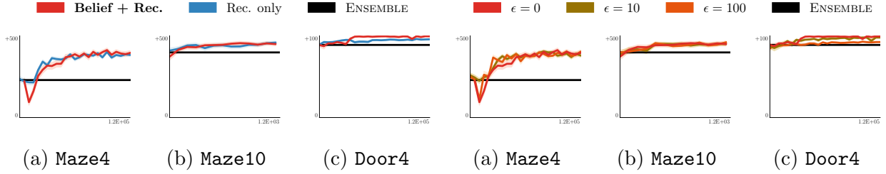
Figure 7.7: Ablation study on input features. Including both belief and recommendation results in faster learning in Door4.
