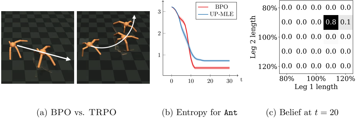
Figure 4.4: (a) Comparison of BPO and TRPO trained on the nominal environment for a different environment. The task is to move to the right along the x-axis. However, the model at test time differs from the one TRPO trained with: one leg is 20% longer, another is 20% shorter. (b) Comparison of average entropy per timestep by BPO and UP-MLE. The belief distribution collapses more quickly under the BPO policy. (c) Belief distribution at t = 20 during a BPO rollout.
