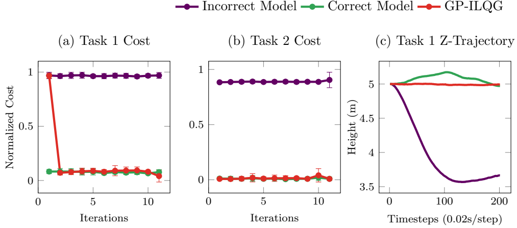
Figure 3.3: Quadrotor control
