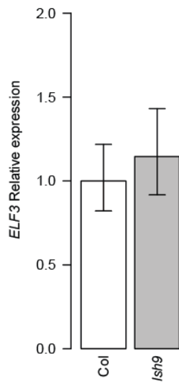
Figure D.8: ELF3 expression is not substantially affected by lsh9 T-DNA insertion. ELF3 expression was measured by PCR and normalized to UBC21 expression (Col set to 1.0). Error bars are standard error of the mean from three technical replicates. This experiment was repeated with similar results.
