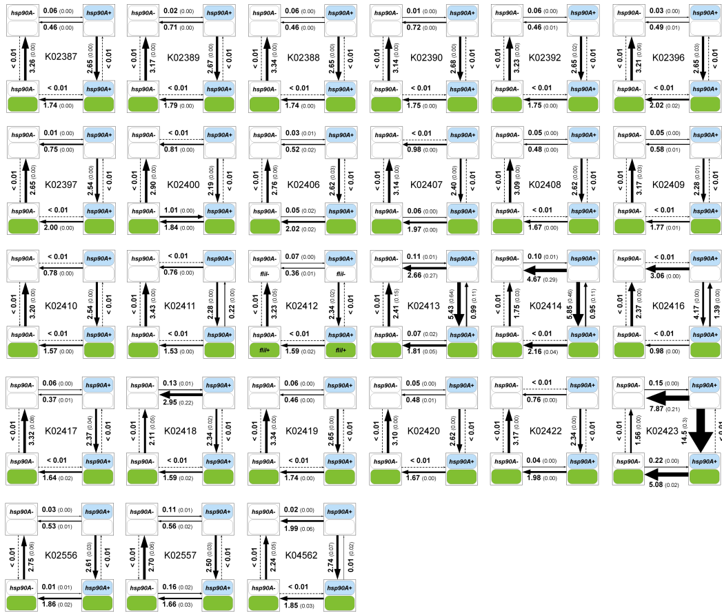
Figure F.2: Co-evolutionary gain and loss rates of all hsp90A - associated flagellar genes. The layout of each diagram is similar to that used in Figure 7.2.
