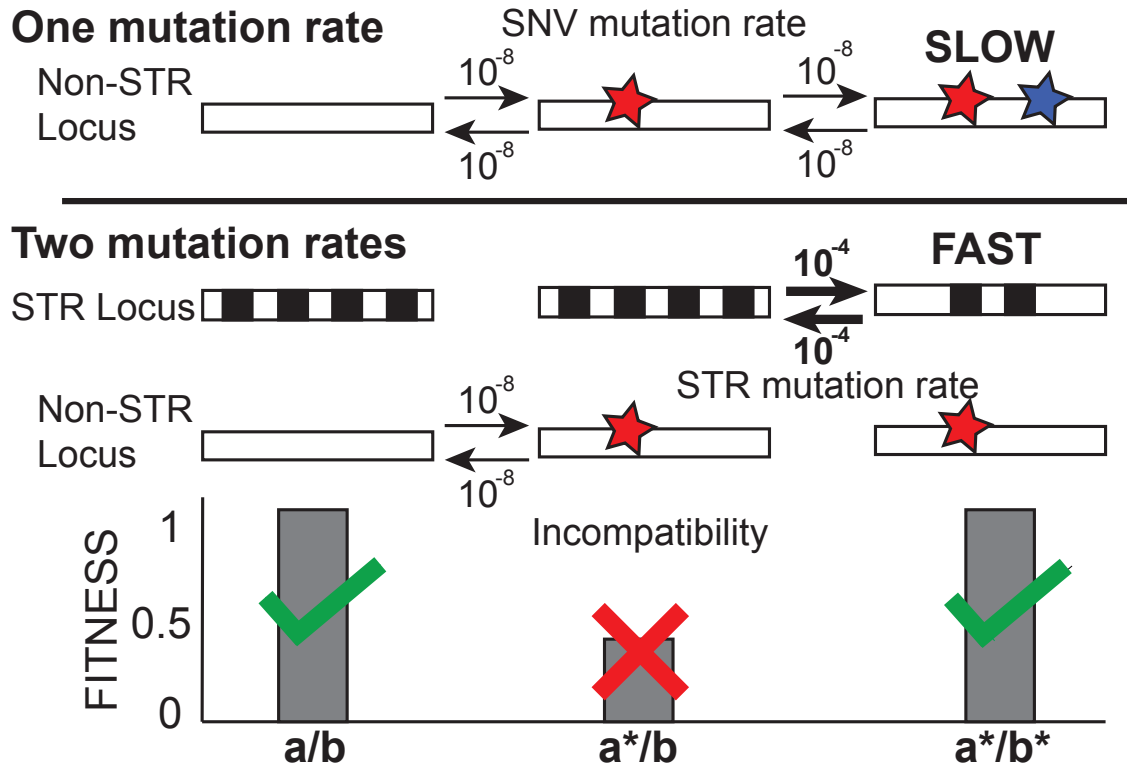
Figure 4.2: A locus with higher mutation rates allows genetic modification of unfavorable genotypes at interacting loci. Top, a model of evolution under epistasis with only one slow mutation rate. Middle, a model of evolution under epistasis with a slow and a fast mutation rate. Boxes represent loci, stars represent SNV-type mutations, black and white checkering indicates an STR locus (a/b, a*/b, and a*/b* signify different genotypes). Arrows with numbers represent possible mutations and their respective rates. Bottom, fitness of each genotype under both models. We expect that the model with two mutation rates will occupy the fully derived state (a*/b*) more quickly.
