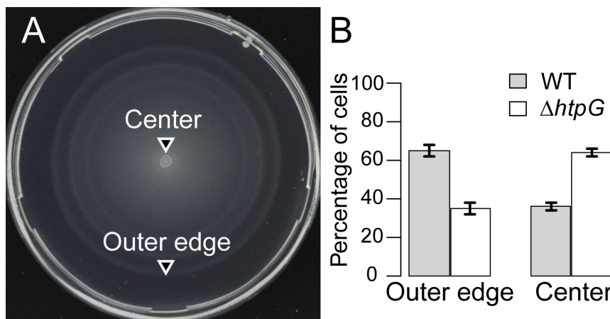
Figure 7.4: \Delta htpG E. coli cells spread less efficiently on soft-agar plates. Upon equal mixing, WT and \Delta htpG cells were competed for 8 hours at 34° on the same soft-agar plates, where bacteria spread in a motility- and chemotaxis-dependent fashion. Samples from the outer edge of the plate are thus enriched in cells with optimal chemotaxis and motility, whereas cells from the center are less chemotactic and/or motile. (A) A representative image of assay plate. (B) Quantitation of different genotypes as determined by percentage of the YFP-labeled WT vs. CFP-labeled \Delta htpG cells at the indicated locations. YFP and CFP expression was induced by 1 \mu M IPTG. An essentially identical result was obtained for the CFP-labeled WT vs. YFP-labeled \Delta htpG cells (data not shown), confirming that it is label-independent. Error bars indicate standard errors from four replicates. Results were similar at 42°C (Table F.3).
