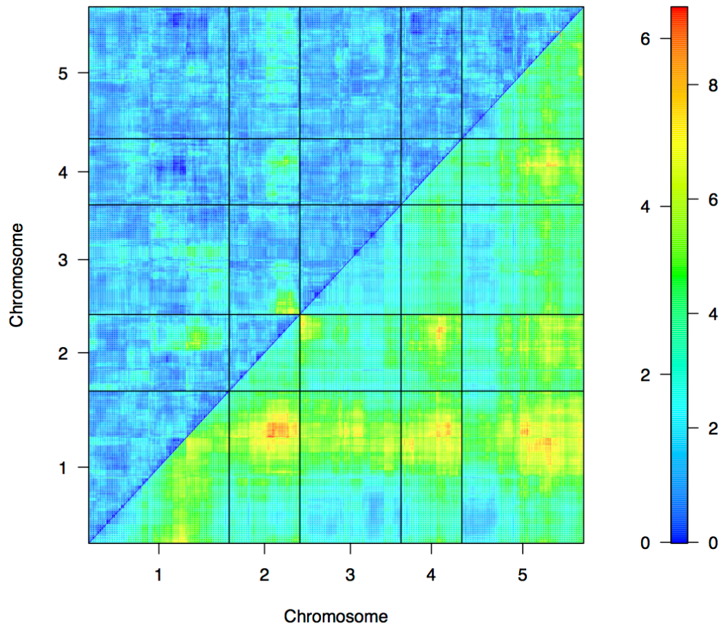
Figure D.4: 2-locus QTL scan indicates potential genetic interactions between ELF3 and other loci. Lower triangle indicates LOD for full model, upper triangle indicates LOD for interaction terms alone. ELF3 corresponds to the locus on chromosome 2.
