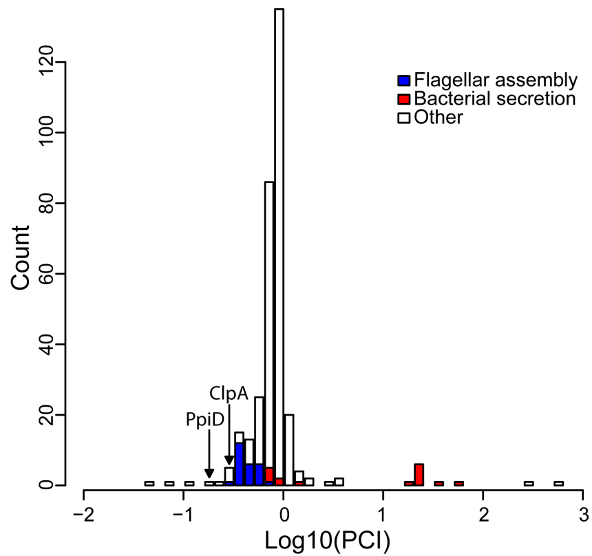
Figure 7.3: The distribution of the Putative Client Index, PCI, among hsp90A -associated genes. Lower values indicate behavior closer to that expected of a client. The 18 genes most likely to be clients are listed in Table 7.2. Prominent functional groups are highlighted, as well as two chaperone-encoding genes.
