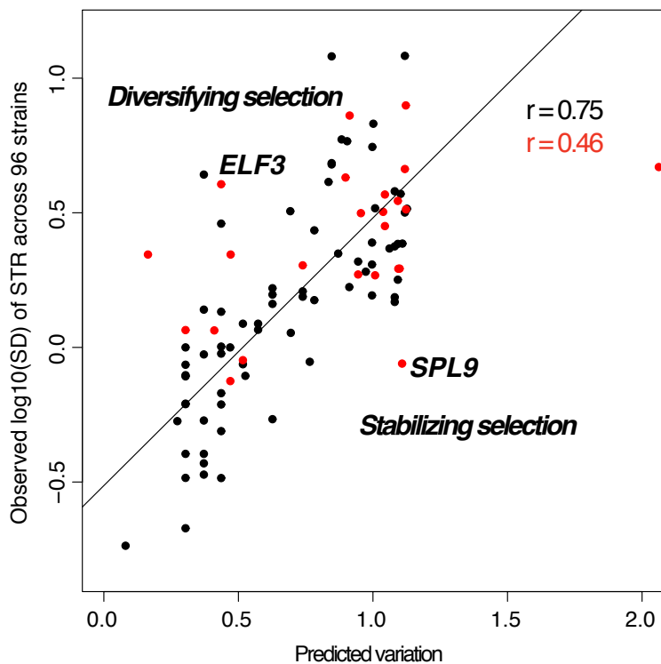
Figure 4.3: Observed and predicted STR variation showed greater correlation for non-coding STRs than coding STRs. The correlation between the observed log 10 of the standard deviation of STR unit number across strains (y-axis) and the VARscore (x-axis), which predicts STR variation from sequence characteristics. Black points are non-coding STRs, red points are coding STRs. Outliers may indicate functional importance ( ELF3 STR is indicated).
