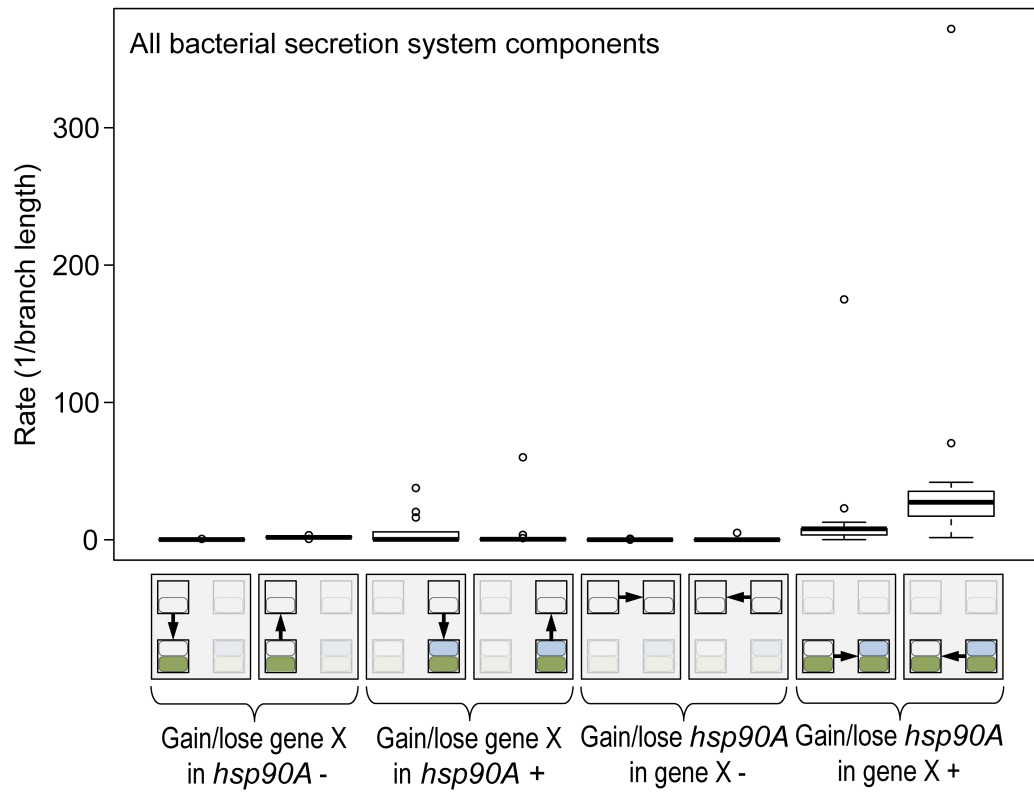
Figure F.4: Box plots of the rates of gain and loss of all hsp90A - associated secretion genes ( n = 16 ). See also Figure 7.2D.
