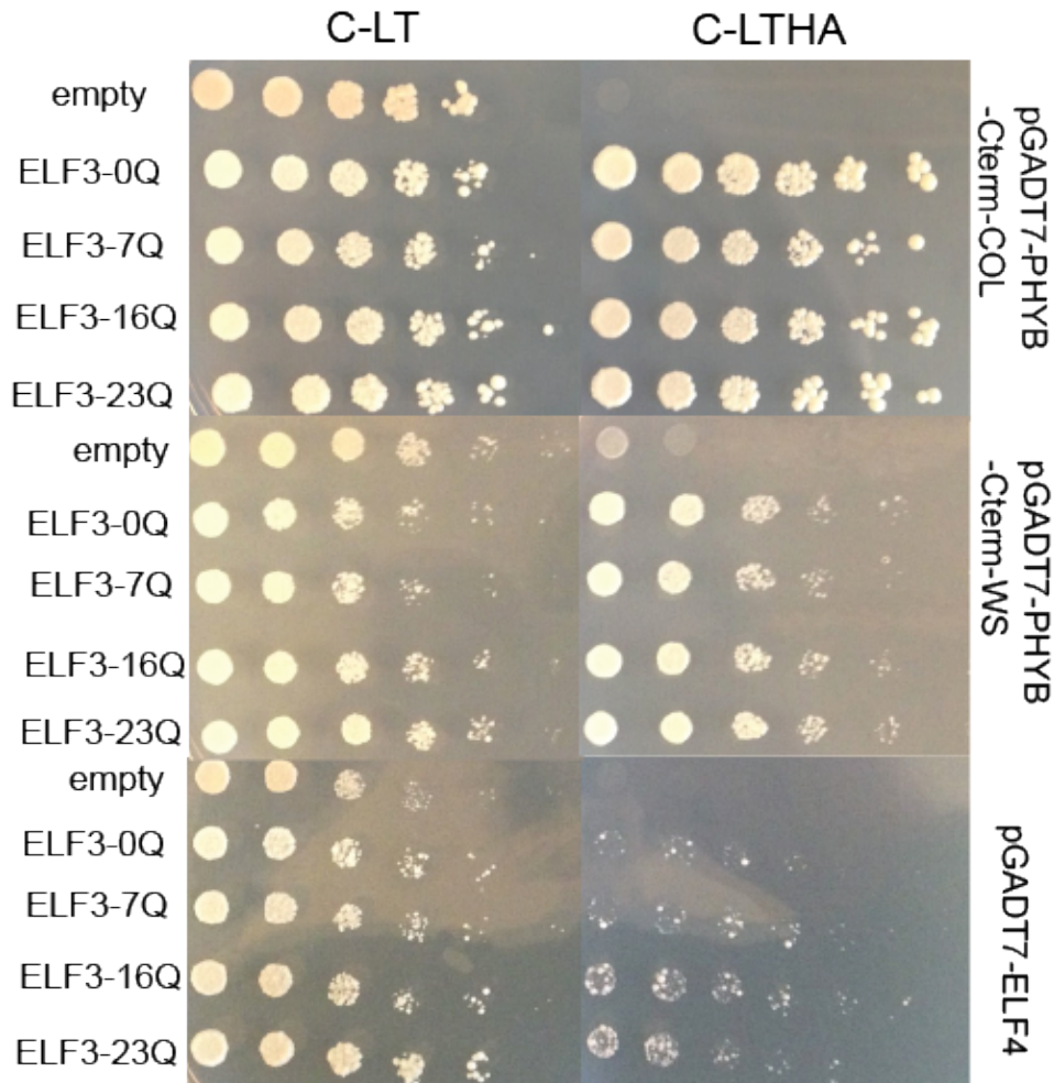
Figure 5.4: Y2H interaction of ELF3 with known protein interactors can be modulated by polyQ variation. Yeast carrying indicated vectors were spotted in five-fold dilutions onto C-leu-trp (C-LT) or C-leu-trp-his-ade (C-LTHA) media. PHYB-Cterm: previously-defined C-terminal truncations of PHYB sufficient for ELF3 interaction [213] from the Col and Ws backgrounds. For each protein X, experiments were repeated with independent PJ69-4 \alpha + pGADT7-X transformants with similar results.
