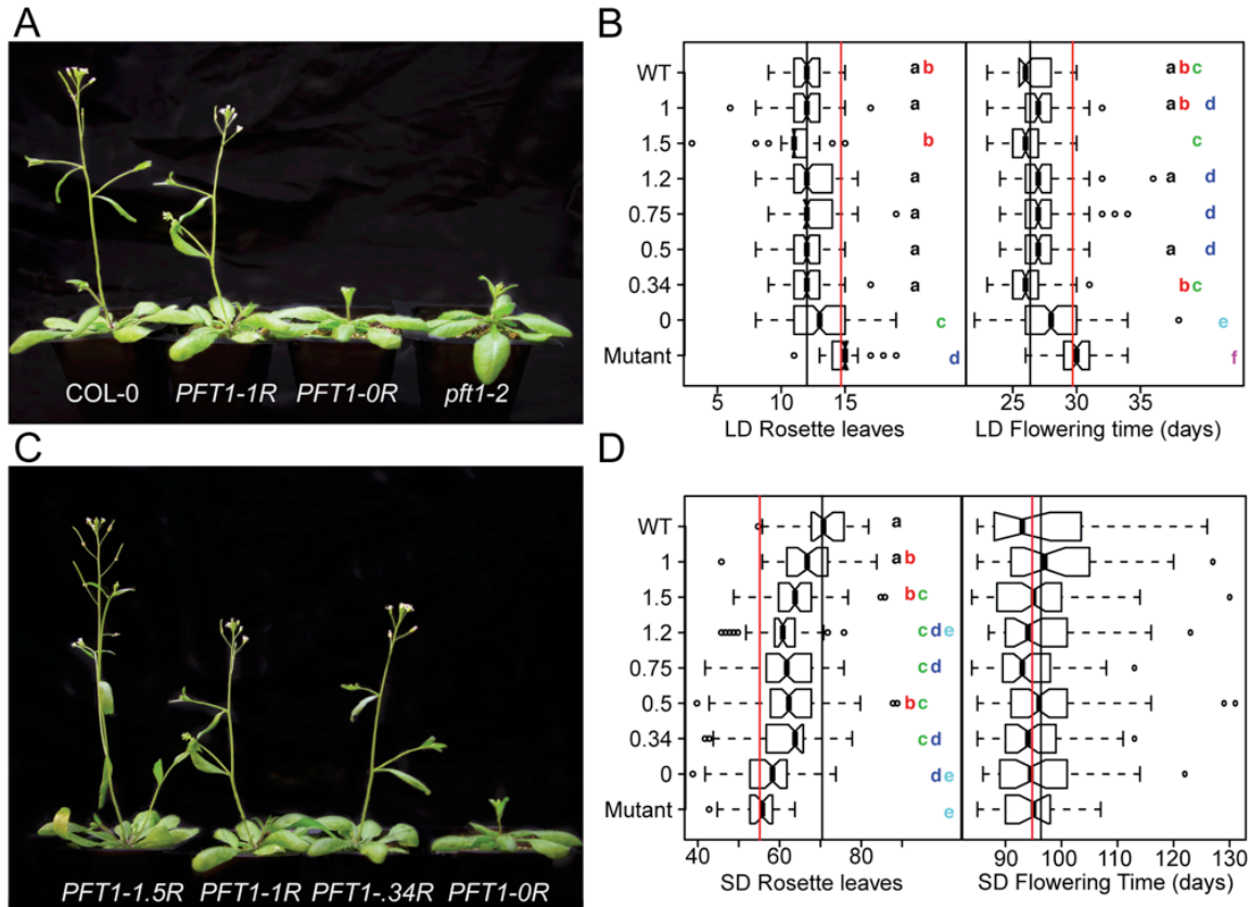
Figure 3.1: PFT1 STR alleles differ in their ability to rescue a pft1 loss-of-function mutant for flowering phenotypes. (A), (C) Transgenic plants carrying different PFT1 STR alleles. Plants were grown under LD for 31 days and photographed. Background was removed in Adobe Photoshop CS 6.0. (B), (D) Strains sharing letters are not significantly different by Tukey's HSD test. Black lines represent WT means, red lines represents pft1-2 means for each phenotype. Each STR allele is represented by at least two independent transgenic lines (Table B.3), with N > 20 for SD phenotypes and N > 35 for LD phenotypes, \alpha = 0.05 . LD=long days, SD=short days. In SD flowering time (days), no groups are significantly different.
