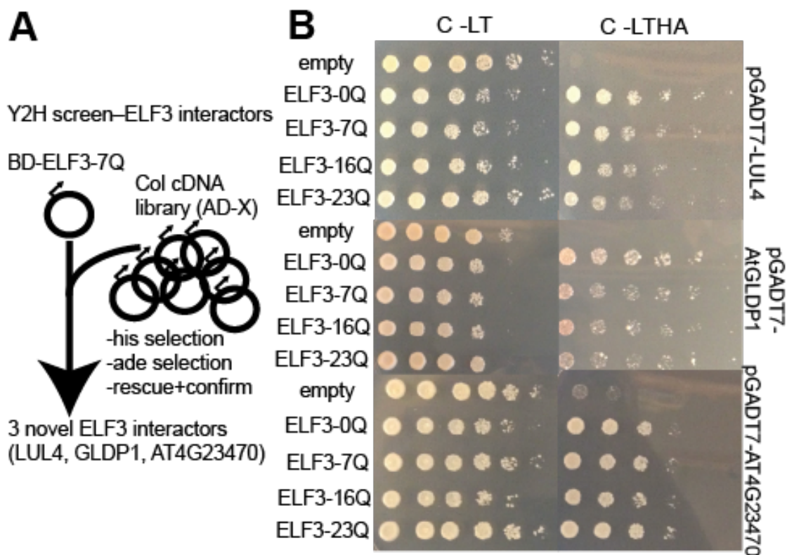
Figure 5.5: Y2H screen identifies new interactors of ELF3. (A): ELF3 Y2H screen design. (B): Yeast carrying indicated vectors were spotted in five-fold dilutions onto C-leu-trp (C-LT) or C-leu-trp-his-ade (C-LTHA) media. For each protein X, experiments were repeated with at least two independent PJ69-4 \alpha + pGADT7-X transformants with similar results.
