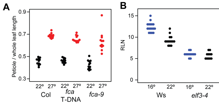
Figure E.2: Regulation of adult thermoresponsive traits by ELF3 and FCA is independent of PIF4 and modulated by genetic background. Flowering temperature response of indicated genotypes under indicated conditions, measured by rosette leaf number (RLN) at flowering. For each experiment, n > 10 plants for each genotype in each treatment. Regression analysis of data in Tables E.4, E.5.
