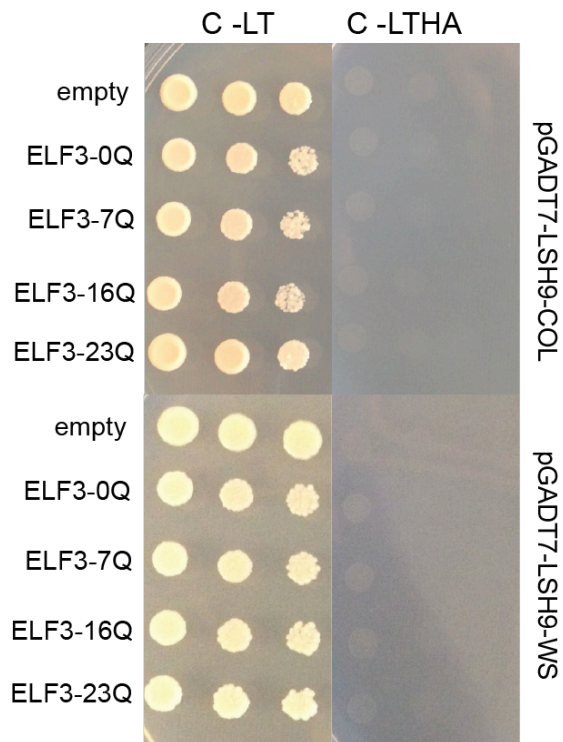
Figure D.7: GAL4 DBD-ELF3 fusions do not lead to Y2H activation in combination with GAL4 AD-LSH9 fusions carrying either the Col or Ws variant of LSH9. Yeast carrying indicated vectors were spotted in five-fold dilutions onto C-leu-trp (C-LT) or C-leu-trp-his-ade (C-LTHA) media. For each protein X, experiments were repeated with independent PJ69-4 \alpha + pGADT7-X transformants with similar results.
