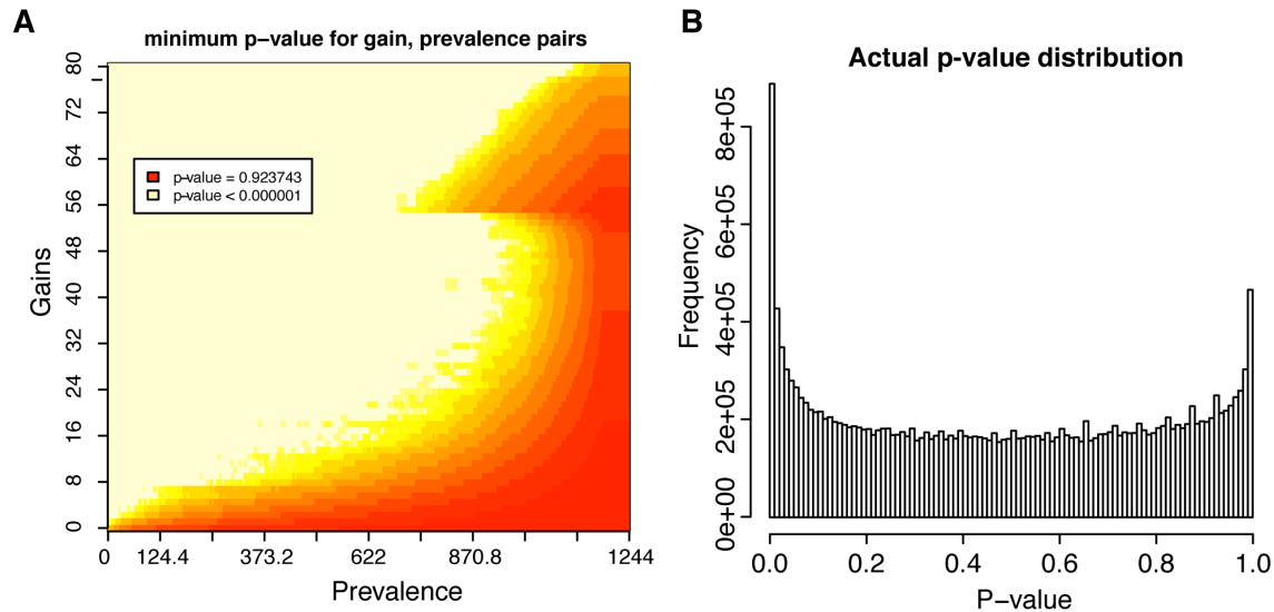
Figure G.3: Some regions of the parameter space are underpowered to detect PGCEs. (A) Power analysis of the parametric bootstrapping hypothesis test for detecting PGCEs. X and Y axes represent, respectively, total prevalence and total gains for a hypothetical pair of genes with a strong PGCE (maximum observable test statistic). Colors represent the (log 10 -scaled) minimum possible p-value that can be attained for such a gene pair using the relevant null distribution of simulated genes. Areas that are not white/pale yellow are underpowered for detecting PGCEs. (B) The distribution of empirical p-values observed for testing hypotheses of no PGCE in the evolution of pairs of genes, according to parametric bootstrapping. The spike at p = 1.0 in (B) indicates that sparsity in the data detracts from power, as predicted in (A), even after filtering pairs of genes with C_{ij} \leq 1 .
