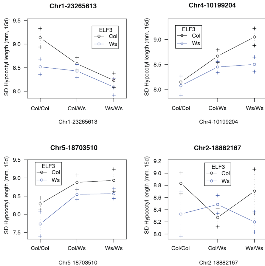
Figure D.5: Effect on hypocotyl length of various QTLs interacting with the ELF 3 locus. X-axis is non-ELF 3 locus, different lines indicate effects of other locus in different ELF 3 backgrounds. Error bars represent standard error of the mean.
