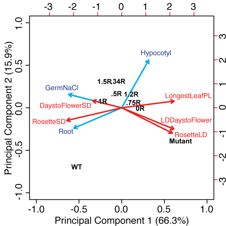
Figure 3.4: Distribution of PFT1 STR allele performance across all phenotypes, relative to wild-type and pft1-2 mutants. Biplot representation of PCA on all phenotypes across all tested PFT1 STR alleles. Percentages on axes are the % variance in the overall data contributed by that principal component. Contributions of specific phenotypes to these axes are shown by size and direction of arrows. Red arrows represent adult phenotypes, blue arrows represent early seedling phenotypes; adult phenotypes are in red, whereas early seedling phenotypes are in blue. 'RosetteSD': number of rosette leaves under SD, 'RosetteLD': number of rosette leaves under LD, 'LongestLeafPL': petiole length of the longest leaf of rosette, 'GermNaCl': proportion of germinants on 200 mM NaCl, 'Hypocotyl' and 'Root' refer to lengths of the specified organs in dark-grown seedlings. Transgenic STR alleles are indicated by their proportion of the wild-type (WT) repeat, i.e. '1.5R'. Top and right axes provide a relative scale for the magnitude of phenotype vectors (blue and red arrows).
