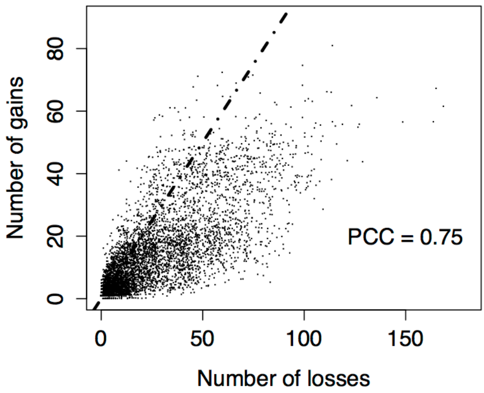
Figure G.1: Gene losses outnumber gene gains. Each of the 5801 genes in the ancestral reconstruction is plotted according to its number of losses and gains. Dashed line indicates expected values if gains and losses were equally frequent. “Gain” and “loss” counts represent the expected number of branches experiencing gain and loss, respectively, for the gene in question. PCC: Pearson correlation coefficient.
