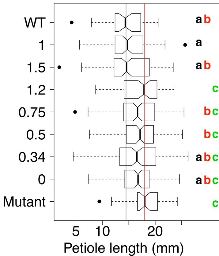
Figure 3.2: PFT1 STR alleles differ in their ability to rescue a pft1 loss-of-function mutant for petiole length in long days. Strains sharing letters are not significantly different by ANOVA with Tukey's HSD test. Black lines represent WT means, red lines represent pft1-2 means for each phenotype. Each allele is represented by at least two independent transgenic lines, N > 35 for each allele, \alpha = 0.05 .
