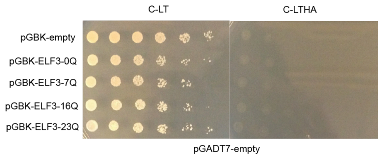
Figure D.9: The GAL4 DBD-ELF3 fusion does not autoactivate in combination with a GAL4 AD-empty vector (pGADT7). Yeast carrying indicated vectors were spotted in five-fold dilutions onto C-leu-trp (C-LT) or C-leu-trp-his-ade (C-LTHA) media. This experiment was repeated with an independent PJ69-4 \alpha + pGADT7 transformant with similar results.
