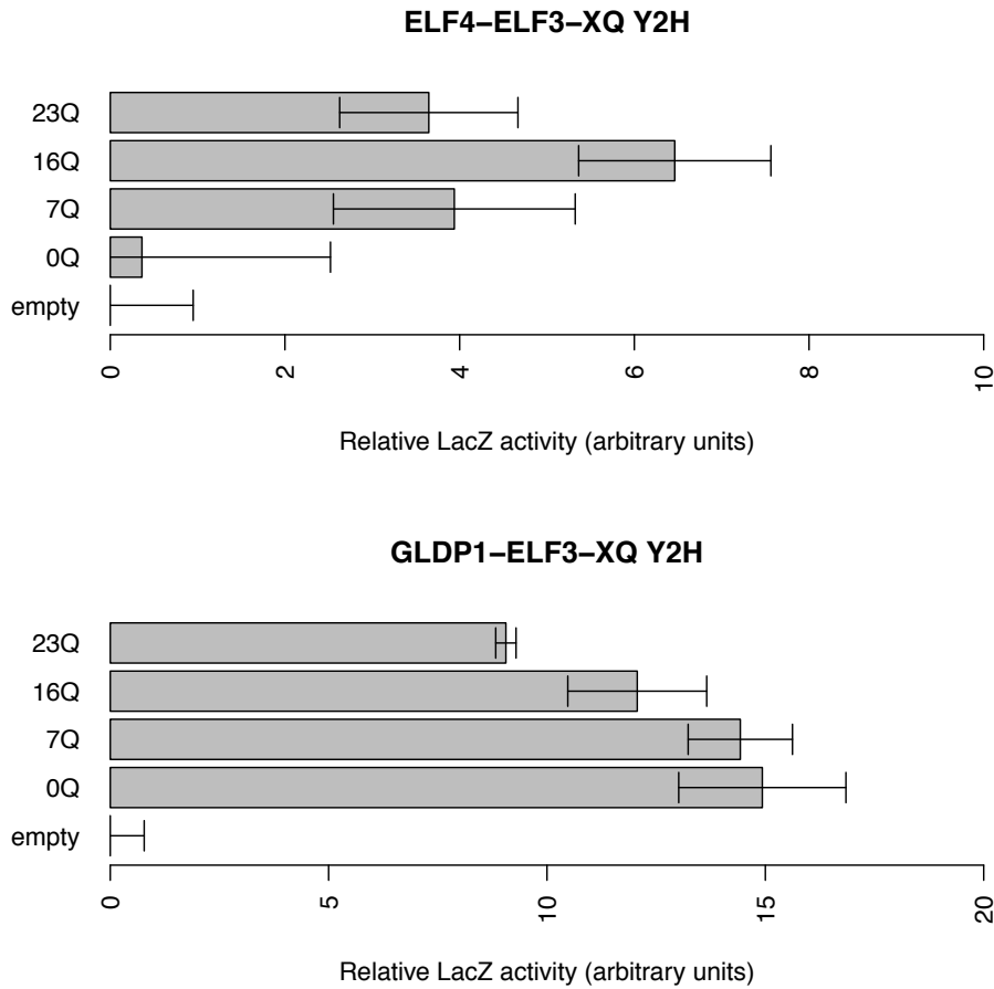
Figure D.11: X-gal cleavage assay confirms modest differences in affinity between ELF3 -polyQ variants for various proteins in Y2H. Bar labels indicate the GAL4 DNA binding domain construct, either empty or containing ELF3 with various polyQ-expressing lengths. In each assay, all observations are expressed relative to the activity of the empty vector, whose mean is set to 0. Error bars indicate standard deviation across three technical replicates. This experiment was repeated with similar results.
