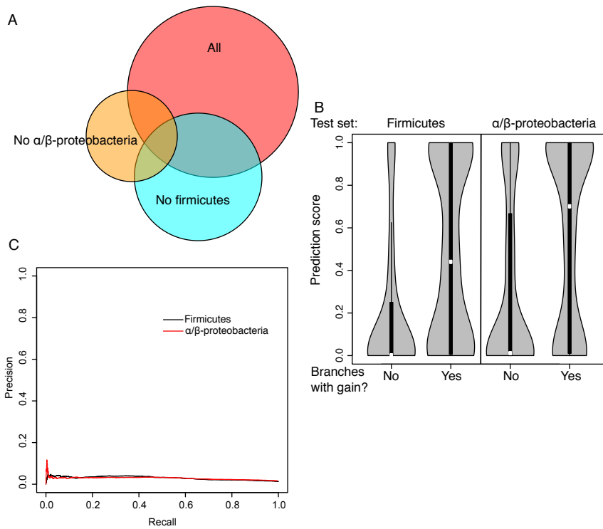
Figure G.9: Performance of models predicting the acquisition of genes between clades. (A) Overlap of edges in PGCE networks inferred from different subsets of the data. See also Table G.4. All overlaps are highly statistically significant ( p < 10^{-15} , hypergeometric test). (B) Distribution of prediction scores for gene acquisition on each branch in the test set clades. Branches with a gain ( \text{Pr}(\text{gain}) > 0.5 ) have a higher score than branches without a gain ( \text{Pr}(\text{gain}) < 0.5 ) for predictable genes ( p < 10^{-15} for each, U-test). Predictable genes are the affected genes in at least one PGCE, i.e. they have at least one in-edge in the trained PGCE model. Violin plots show density of each distribution. Each violin plot shows the distribution of prediction scores for branches in one test set for one category (gene gained/gene not gained). (C) Precision/recall plot of PGCE predictions. Notably, the precision by which any particular gain event is predicted is relatively low due to the rarity of true gain events for any particular gene, yet, as demonstrated in Figure 8.5B and in panel B here, ancestral genome content was overall informative about where along the tree such true gain events occur.
