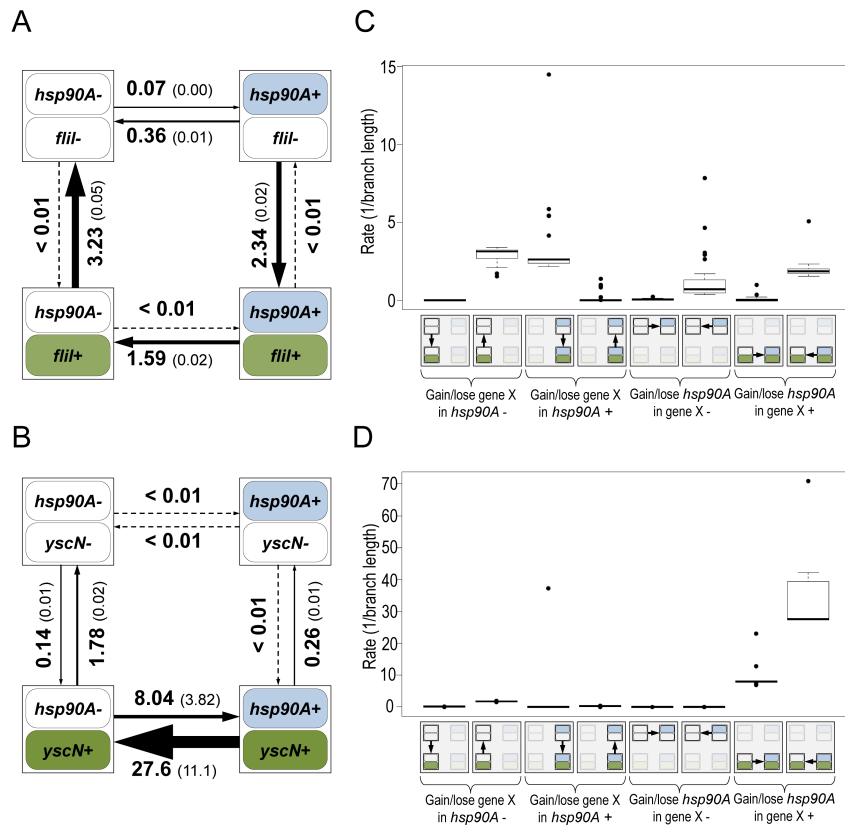
Figure 7.2: Flagellar genes and secretion system genes show distinct signatures of co-evolution with hsp90A . Schematic diagrams of the models describing the co-evolution of hsp90A with the flagellar gene fliI (A) and the non-flagellar Type III secretion gene yscN (B). The four boxes represent the four possible states of presence and absence in each model, and arrows represent transitions between them (gain or loss events). Arrow widths in each diagram are scaled to represent the rate of each transition. The average transition rate and standard deviation across multiple BayesTraits runs are displayed (see Methods). Box plots of the rates of gain and loss of all hsp90A -associated flagellar genes (n = 27; C) and all hsp90A -associated Type III secretion genes (n = 10; D) further demonstrate consistent co-evolutionary dynamics of genes in these categories. A box plot of all hsp90A -associated secretion genes (including all types) is available in the supporting information (Figure F.4).
