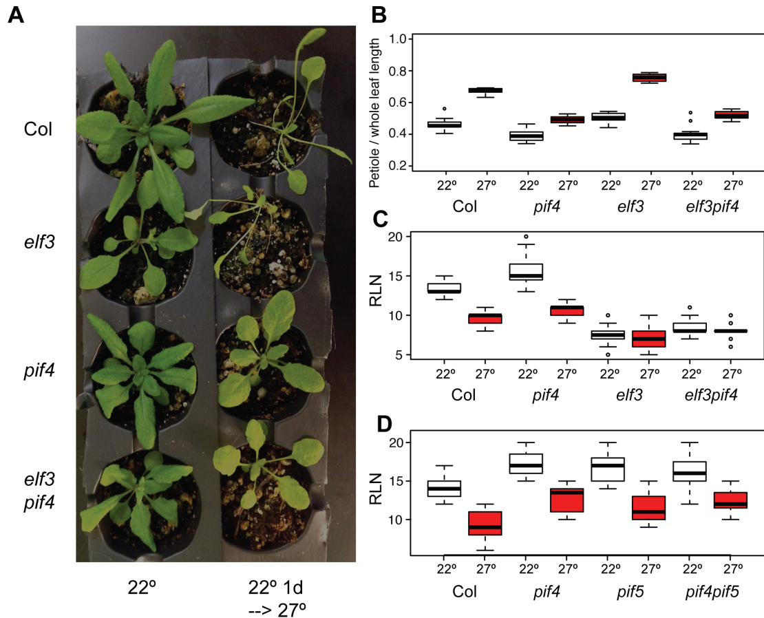
Figure 6.4: Double mutant analysis confirms PIF 4 and ELF 3 independence in adult temperature responses and non-redundancy of PIF 4 with PIF 5 . (A): Col, elf3-200 , pif4-2 , and elf3-200 pif4-2 plants grown under long days with two different temperature regimes were photographed at 25 days post germination. (B): Petiole elongation responses of the indicated genotypes, measured by ratio of petiole to whole leaf length at 25 days post germination. (C): Flowering temperature response of indicated genotypes, measured by rosette leaf number (RLN) at flowering. (B) and (C): n > 8 plants for each genotype in each treatment. All “27°” plants were seeded and incubated one day at 22° before transfer to 27°. Experiments were repeated with similar results. Regression analysis of data reported in Tables E.6 and E.7.
