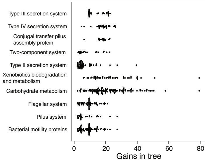
Figure G.7: Differences in gain counts do not explain differential sorting of genes in different functional groups. (A): Variation in ranks of the sort across functional categories. (B): Total branches in which gains have occurred (“gains in tree”) across genes in various functional categories that are differentially ranked in a topological sort of the PGCE network. Note that the categories with the highest average gain (Carbohydrate and Xenobiotics metabolism) are ranked in the middle of the sort. See Table 8.1.
