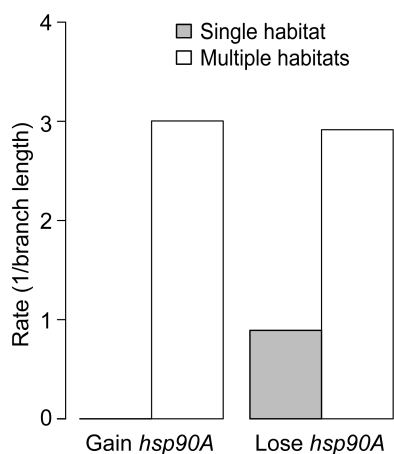
Figure 7.6: Habitat preference affects the gain and loss of hsp90A in bacteria. Rates of gain and loss of hsp90A throughout bacterial evolution with relation to multiple habitat preference. Standard deviation across 100 runs was smaller than 0.001 in all cases.
