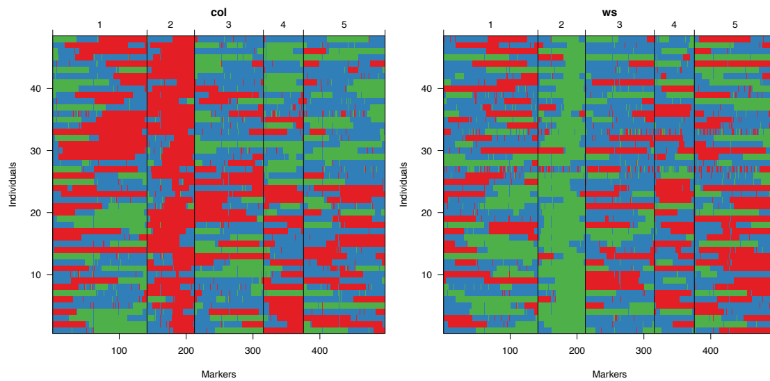
Figure D.3: Genotypes of the 96 extreme F_2 s used for sequencing. Sorted vertically by descending phenotype (longer hypocotyls above, shorter hypocotyls at bottom), chromosomes are displayed along the X axis. ELF_3 - Col homozygotes at left, ELF_3 - Ws homozygotes at right. Red indicates homozygosity for Col allele, blue indicates heterozygosity, and green indicates homozygosity for Ws allele.
