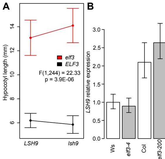
Figure 5.3: ELF3 shows a genetic interaction with LSH9 and modulates its expression in a background-specific fashion. (A): Double mutant analysis of elf3 and lsh9 seedlings grown 15d under SD. Statistics shown are from ANOVA analysis of the interaction between the mutant effects on phenotype. Error bars indicate standard deviation, n > 35 for each genotype. (B): Reverse-transcriptase PCR (RT-PCR) analysis of LSH9 expression across genotypes. Seedlings were grown short days and harvested for RNA at ZT8 (dusk). LSH9 expression is expressed as a proportion of Ws expression, normalized relative to UBC21 , error bars are standard error from three technical replicates. Experiments were repeated with similar results.
