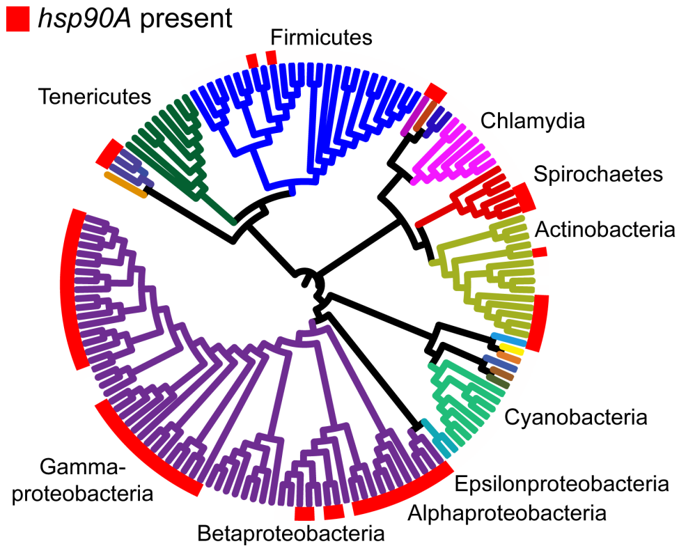
Figure 7.1: The distribution of hsp90A across a bacterial phylogeny. Branches are colored according to phyla. Large taxonomic groups are labeled. Branch lengths are ignored for ease of display. The phylogeny constructed by Ciccarelli et al. [50] is used (see Methods). For distribution of other bacterial Hsp90 paralogs, see Figure F.1C. hsp90B and hsp90C are not displayed, and are ignored throughout the analysis.
