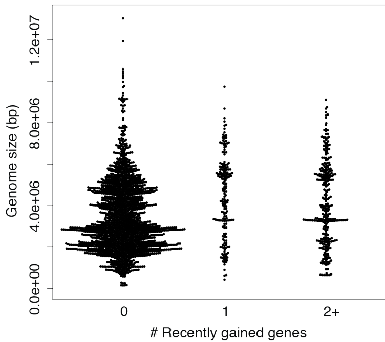
Figure 9.3: Prevalence of recently horizontally acquired genes is weakly correlated with genome size in bacteria. HGT data from [342], sequences were filtered to contain only those genes likely to be inherited horizontally ( \geq 99\% identity between sequences from genomes with < 97\% 16S rRNA identity), and then counted within genomes. Spearman's \rho = 0.17 ( p < 10^{-15} ); when correcting for higher gene content of large genomes (HGT/bp), Spearman's \rho = 0.11 ( p < 10^{-10} ).
