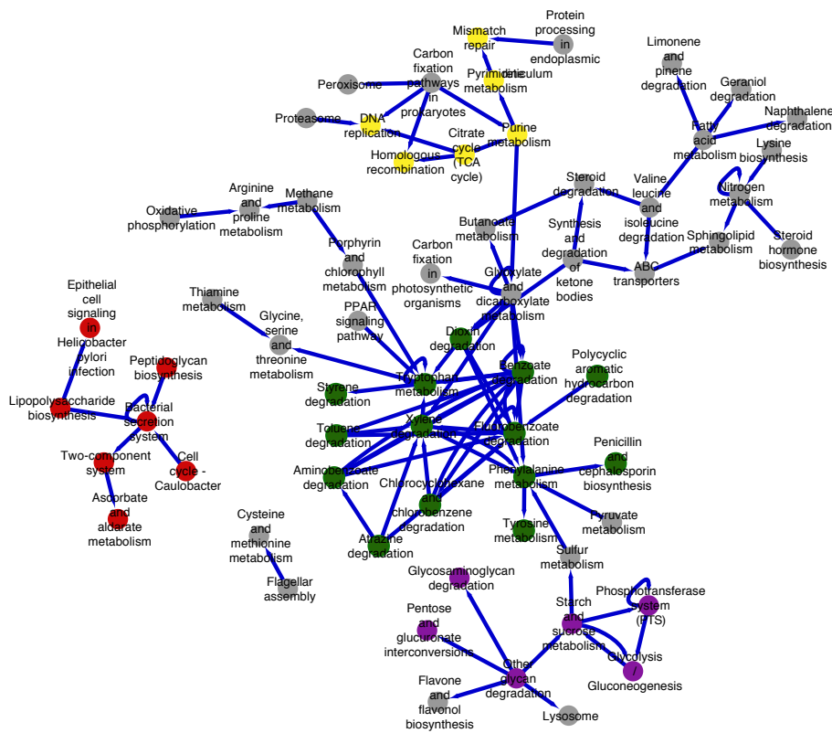
Figure G.6: A network of evolutionary dependencies between functional pathways. Overall structure of the evolutionary pathway-pathway dependency network. Directed edges indicate that the source pathway and the sink pathway are connected by more PGCEs between individual genes in those pathways than expected from a rewired null distribution ( p < 0.001 ). Colors indicate selected pathway clusters of similar functions (green: aromatic compound secondary metabolism; red: pathogenesis; purple: carbohydrate metabolism; yellow: DNA metabolism).
