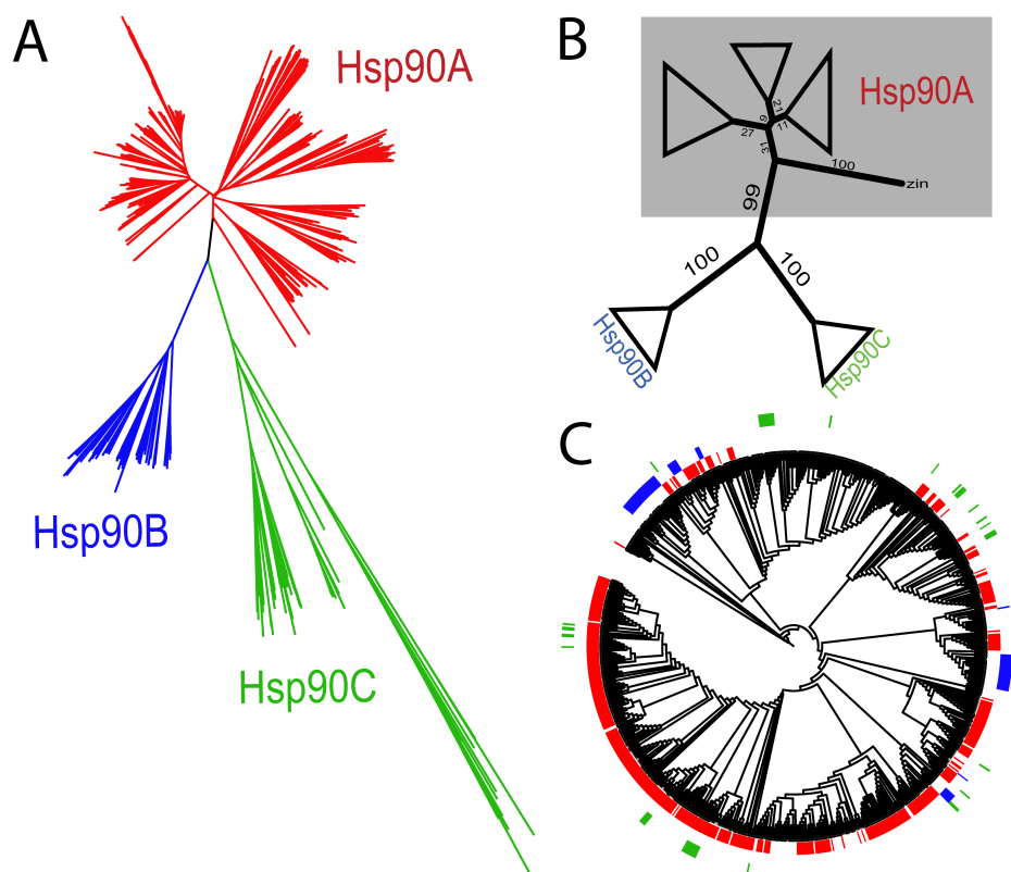
Figure F.1: Phylogenetic clustering of bacterial hsp90 paralogs. (A) Neighbor-joining phylogeny of 897 bacterial Hsp90 amino acid sequences. Groups Hsp90A, Hsp90B, and Hsp90C as defined by Chen et al. [42] are illustrated. (B) Consensus neighbor-joining tree for 100 bootstraps with clades collapsed to highlight deep branch structure. Bootstrap support for each branch is displayed and is also reflected by the branch lengths. One species (ZIN, representing Hsp90 from the organism Candidatus Zinderia insecticola CARI), never grouped within the other divisions shown, and was excluded from our analysis. The branch separating Hsp90B and Hsp90C from the Hsp90A clades is present in 99/100 bootstrap trees. (C) Hsp90A, B, and C presence/absence patterns mapped onto a 16S/23S rRNA phylogeny of 797 bacterial species [252] (see Appendix F Text). Branch lengths are ignored for ease of display.
