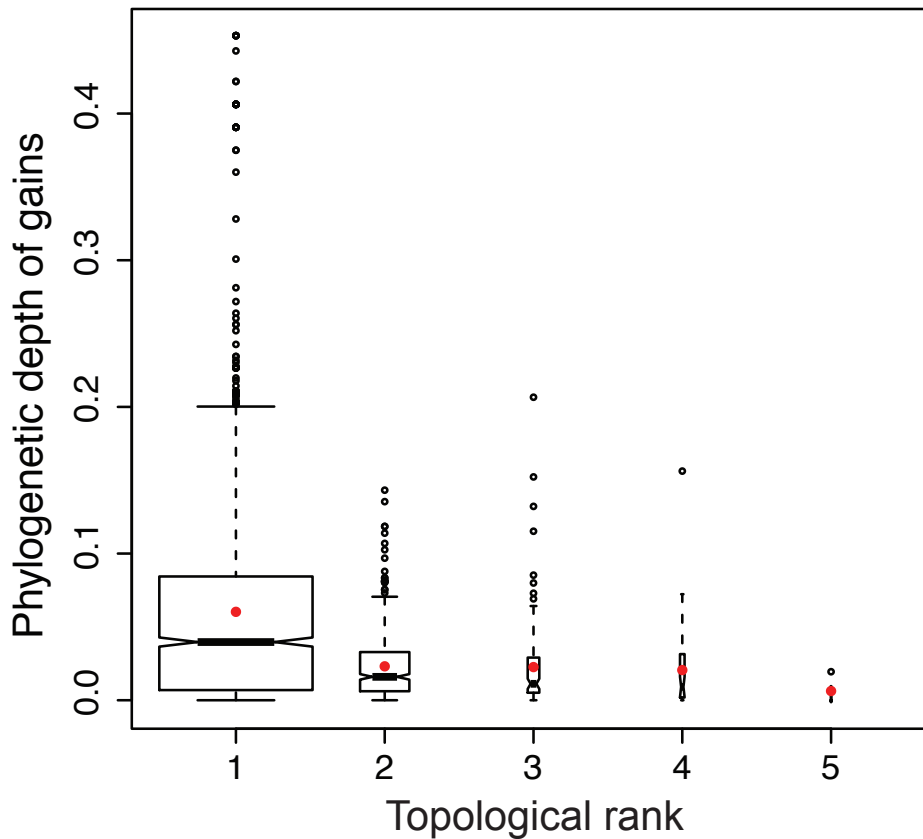
Figure G.8: Phylogenetic depth of gene gains in bacteria decreases with rank in the topological sort. Phylogenetic depth of the gains of genes are weakly negatively correlated with their ranks in the sort (Spearman's r = -0.24 , p < 10^{-15} ). For each rank, we plot the distribution of the phylogenetic depths (distance of gain branch from root) of the average depth of confident gains ( \text{Pr}(\text{gain}) > 0.6 ) of each gene in that rank. The mean of each distribution is plotted as a red point. Branches leading to Archaea and archaeal genomes are omitted from the analysis. Boxplot widths are scaled to the number of genes in each rank of the sort. The tree was converted to an ultrametric tree for the purpose of this analysis (the root is separated from all tips by a total branch length of 1.0).
