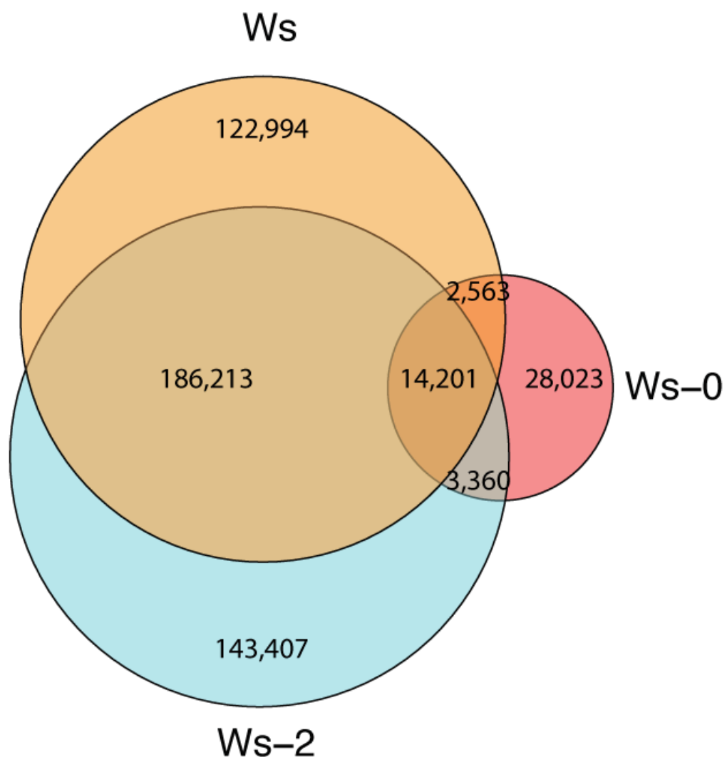
Figure D.2: Overlap of high-confidence ( Q \geq 40 ) single nucleotide variants (SNVs) observed in the Ws strain with two related strains.
