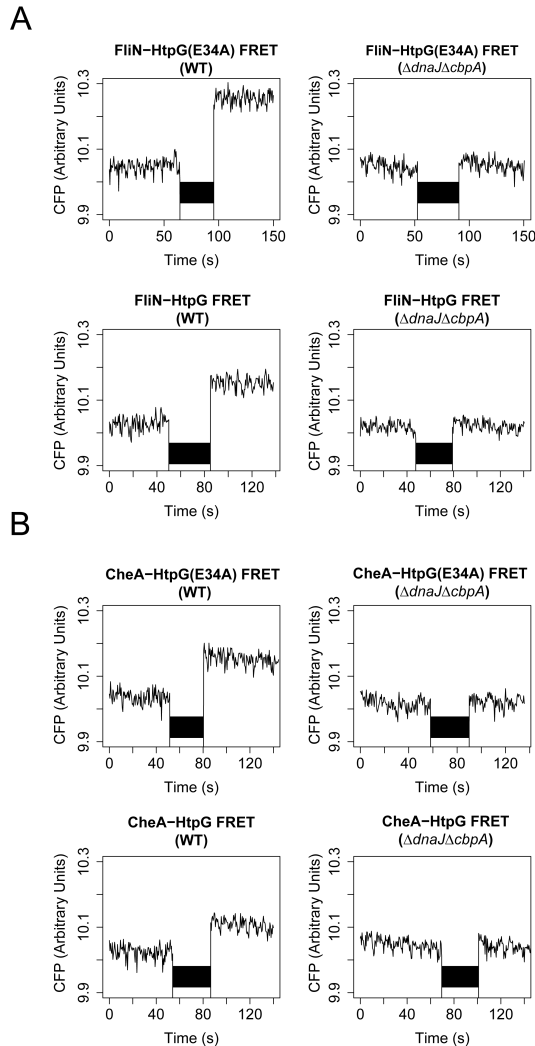
Figure F.6: HtpG interactions with FliN and CheA are dependent on the DnaJ/CbpA/DnaK chaperone system. Acceptor photobleaching FRET was measured between HtpG and FliN (A) or CheA (B). In each panel, HtpG(E 34 A) (top row) and wild-type HtpG (bottom row) were assayed, and experiments were performed in both WT (left column) and \Delta dnaJ \Delta cbpA (right column) backgrounds. Y-axes are normalized in each case to the mean CFP signal before bleaching (first 45 s). Photobleaching begins at 50 s and lasts for 20 s (indicated by black bar). FRET interaction is indicated by a post-photobleaching increase in CFP signal above pre-photobleaching CFP signal (as observed in all experiments in the WT background).
