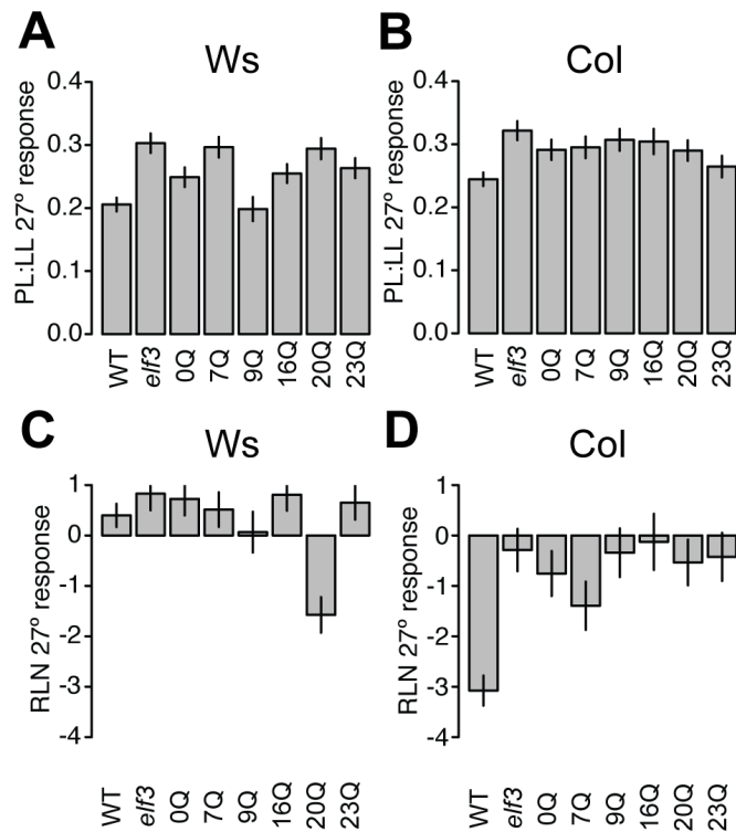
Figure 6.2: Adult plant responses to elevated temperature (27°, relative to 22°) in long days among transgenic lines expressing different ELF3-polyQ variants. (A) and (C): Response in the Ws (Wassilewskija) strain background. Lines are in an elf3-4 background. (B) and (D): Response in the Col (Columbia) strain background, lines are in an elf3-200 background. (A) and (B) display PL:LL temperature response, (C) and (D) display RLN temperature response. Average responses and errors were estimated in a regression model accounting for variation between experiments (Table E.2), based on two to three independently-generated transgenic lines for each genotype. n \geq 24 plants overall for each genotype in each condition. PL:LL = petiole to leaf length ratio at 25 days post germination, RLN = rosette leaf number at flowering, WT = wild type, elf3 = elf3 mutant+vector control, 0Q = elf3 mutant+ ELF3 transgene with entire polyglutamine removed, etc. Error bars indicate standard error.
