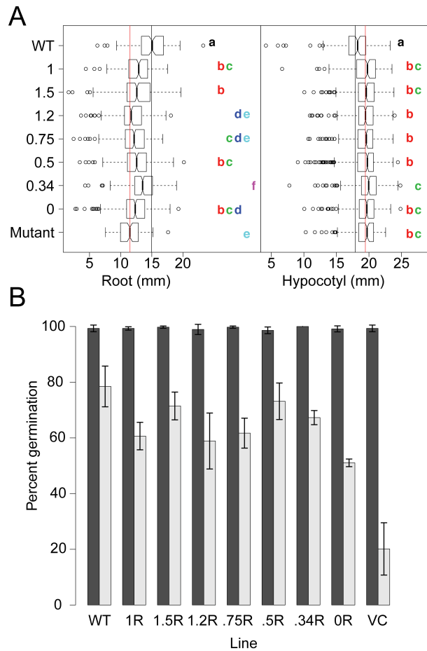
Figure 3.3: PFT1 STR alleles differ in their ability to rescue a pft1 loss-of-function mutant for early seedling phenotypes. A) Strains sharing letters are not significantly different by ANOVA with Tukey's HSD test. Black lines represent WT means, red lines represent pft1-2 means for each phenotype. Each allele is represented by at least two independent transgenic lines, N > 100 for all phenotypes for each allele, pooled across at least two experiments; \alpha = 0.05 . Hypocotyl length and root length were assayed in 7d seedlings grown in dark conditions. B) Dark and light bars represent mean germination across 3 biological replicates on 0 mM NaCl and 200 mM NaCl, respectively. N = 36 for each replicate experiment. Error bars represent standard error across these three replicates.
