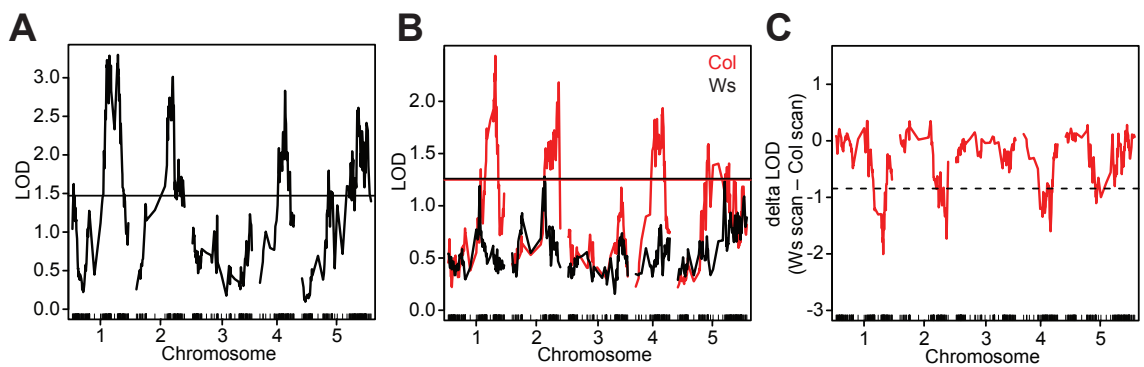
Figure 5.2: QTL analysis identifies interactions of ELF3 with multiple loci. (A): one-dimensional QTL scan including all F_2 s. Horizontal line indicates 99% significance threshold based on permutations. (B): QTL scan stratified by ELF3 genotype (all genotypes but those of indicated F_2 s masked in each analysis). Horizontal lines of each color indicate 99% significance threshold based on permutations for each scan. (C): A direct nonparametric test of epistasis between ELF3 and other loci, using the independent QTL scans shown in (B). ELF3 is located on chromosome 2. Dotted horizontal line indicates 99% significance threshold based on simulations.
