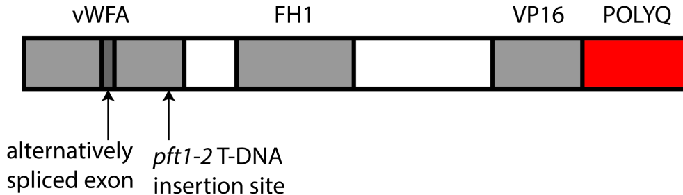
Figure B.1: Structure of the PFT 1 protein. Important features and domains are indicated. vWFA: van Willebrand Factor A domain, FH 1 : Formin homology 1 domain, VP16: VP16-like interaction domain, POLYQ: glutamine-rich domain including the polyglutamine encoded by the PFT1 STR. Also indicated is the difference between the two splice forms of PFT1 (minor splice form, PFT1.2 , lacks a small exon), and the site of the T-DNA insertion in the pft1-2 mutant.
