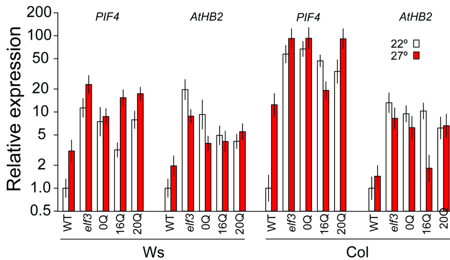
Figure E.1: Expression analysis of PIF4 and AtHB2 depends on temperature, genetic background, and ELF3 functionality. Error bars represent the standard error of the mean across 3 technical replicates. White bars represent 22° expression, red bars 27° expression for each line. Tissue was collected from 7d seedlings at ZT0. This experiment was repeated with similar results.
