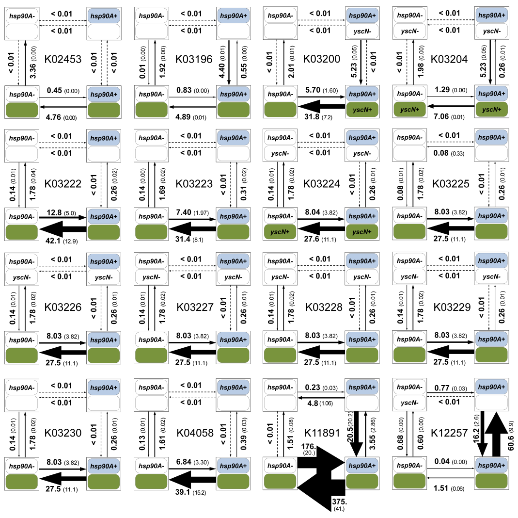
Figure F.3: Co-evolutionary gain and loss rates of all hsp90A - associated secretion genes. The layout of each diagram is similar to that used in Figure 7.2.
