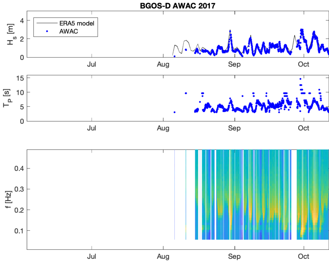
Figure 11: Significant wave heights, peak wave periods, and spectrograms (color is \log_{10} of wave energy density) of waves from BGOS-D in 2017.
