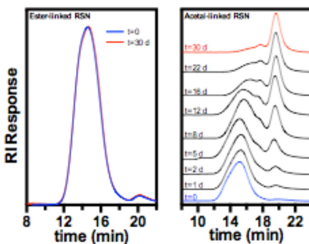
FIGURE 6.4. Molecular weight distributions for poly(DMA) polymerized from poly(hECT) and poly(aECT) transmer cores following incubation in pH 5.0 acetate buffer at 37 °C.
