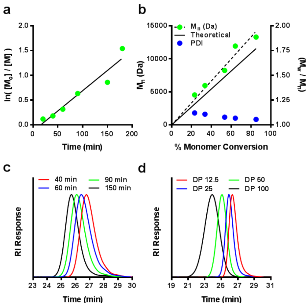
Figure 3.3. Kinetic analysis of the RAFT polymerization of HBC. (a) Pseudo first order rate plot, (b) M_n and \bar{M}_w/\bar{M}_n vs. conversion, and (c) RI traces showing the evolution of molar mass with time for [M]_0:[CTA]_0:[I]_0 equal to 25:1:0.2 at 70 °C with CTP and ABCVA as the chain transfer agent and initiator respectively. (d) Molecular weight distributions for the RAFT polymerization of HBC conducted at initial [M]_0/[CTA]_0 ratios of 12.5, 25, 50, and 100 at a fixed initial [M]_0 and [CTA]_0/[I]_0 ratio 20 wt% and 10 respectively. M_n (Da) and \bar{M}_w/\bar{M}_n values for the series were determined to be: DP 12.5 (7650/1.09), DP 25 (12000/1.07), DP 50 (26300/1.08), and DP 100 (52400/1.15). Absolute molecular weight values were determined by SEC equipped with inline laser light scattering detectors. Monomer conversion was determined by ^1\text{H} NMR by comparison of the vinyl resonances normalized to the total ester region relative prepolymerization values.
