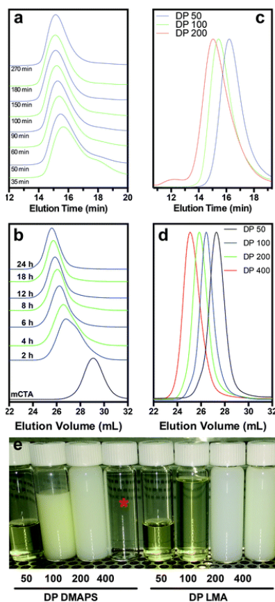
FIGURE 4.4. Overlay of SEC chromatograms traces (RI channel) showing the evolution of molar mass with time for (a) DMAPS and (b) LMA with [M]_0 : [mCTA]_0 : [I]_0 equal to 200 : 1 : 0.05 and 200 : 1 : 0.1, respectively. Molecular weight distributions for the PISA of (c) DMAPS and (d) LMA conducted at initial [M]_0/[mCTA]_0 ratios of 50, 100, 200, and 400. (e) Photographs of polymer solutions following the PISA of DMAPS or LMA from a poly(HEMA- co -O300) macro-CTA in acetic acid. Target DPs for both monomers were 50, 100, 200 and 400. * DMAPS samples targeting a DP of 400 were observed to phase separate, forming a white colloid oily phase and a clear acetic acid phase upon polymerization.
