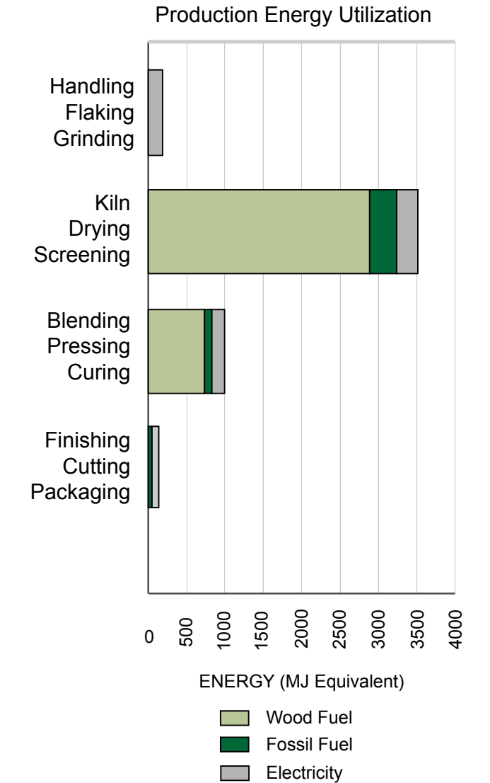
FIGURE 4: 80% of heat energy used in production of OSB is used in the drying of raw materials using biomass fuel. (Data from Kline.)
