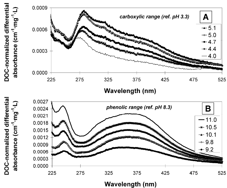
Figure 2.1 DAS profiles of the Suwannee River fulvic acid (SRFA) reflecting the engagement of carboxylic and phenolic groups at varying pHs (adopted from Dryer et al. 96 )
