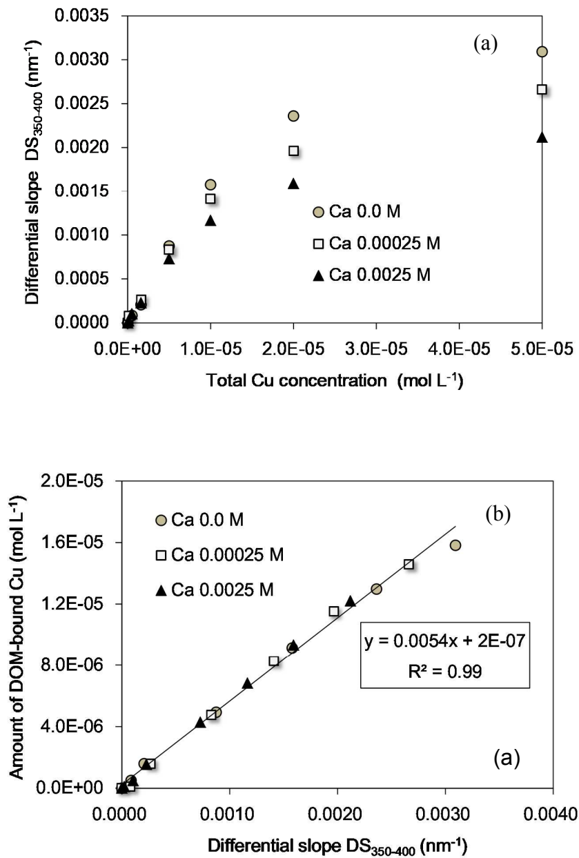
Figure 5.8 Correlation between changes of the spectral slope in the range of 350 to 400 nm and (a) total Cu concentration and (b) the amount of SRHA-bound copper ions predicted for varying background calcium concentrations.
