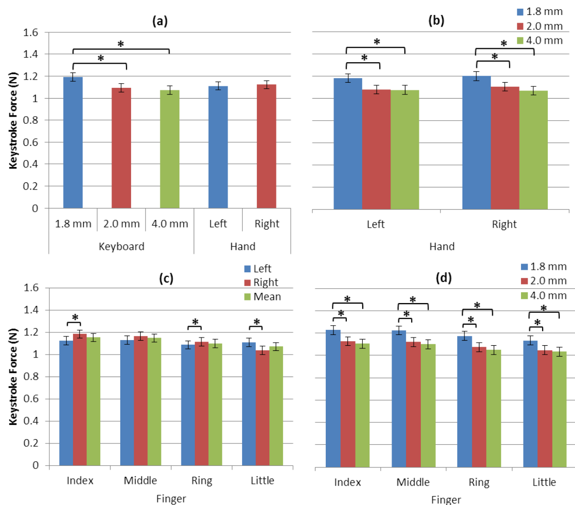
Figure 3.5 Comparisons of mean keystroke forces [n=13]: (a) by keyboard and by hand; (b) by hand and keyboard; (c) by finger and hand; (d) by finger and keyboard. Asterisks denote statistical significance ( p < 0.05 ).
