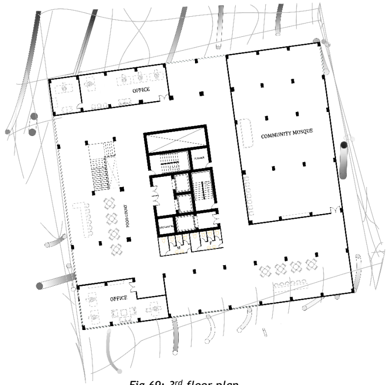
Fig 69: 3 rd floor plan
