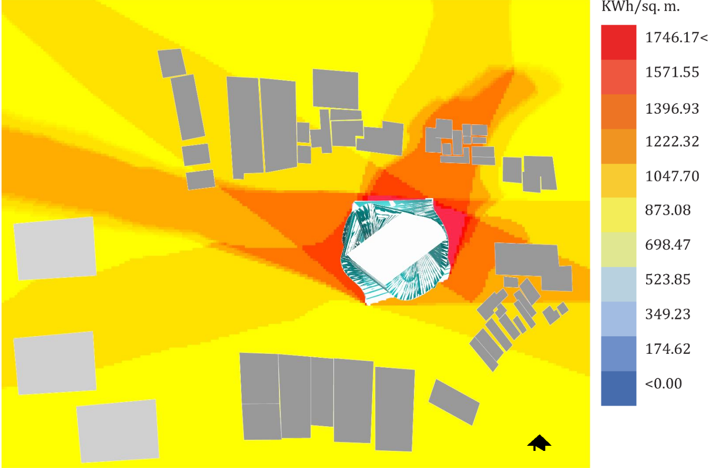
Fig 64: shadow range study for around the year solar gain on ground plane
