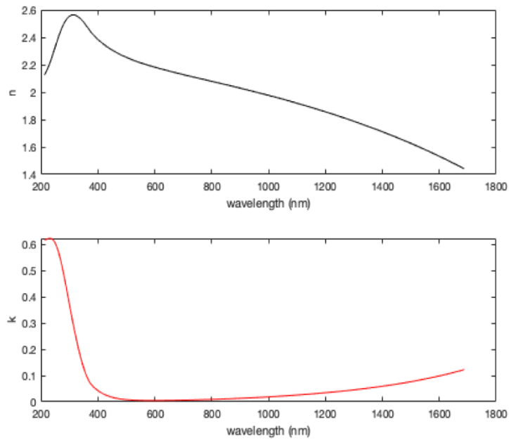
Figure 6.3. Averaged ITO refractive index. Real (top) and imaginary (bottom) versus wavelength. Measured using ellipsometry
