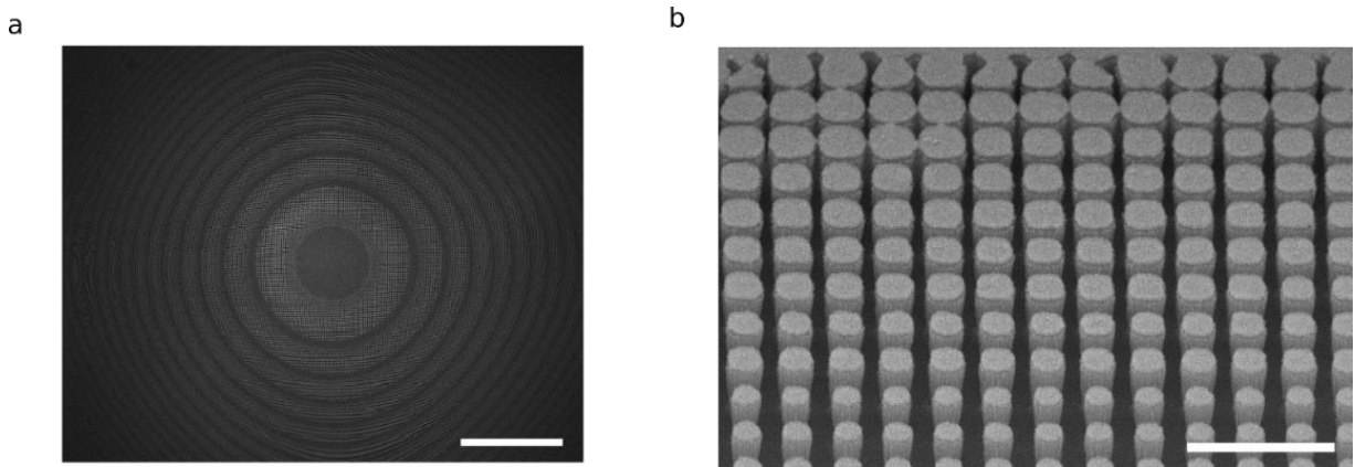
Fig. 2.2 - SEMs of the fabricated device structure. The metasurface was sputter coated with gold-palladium alloy for charge dissipation a) Scale bar is 100um. b) Scale bar of 1um taken at 45 degrees to normal. [22]
