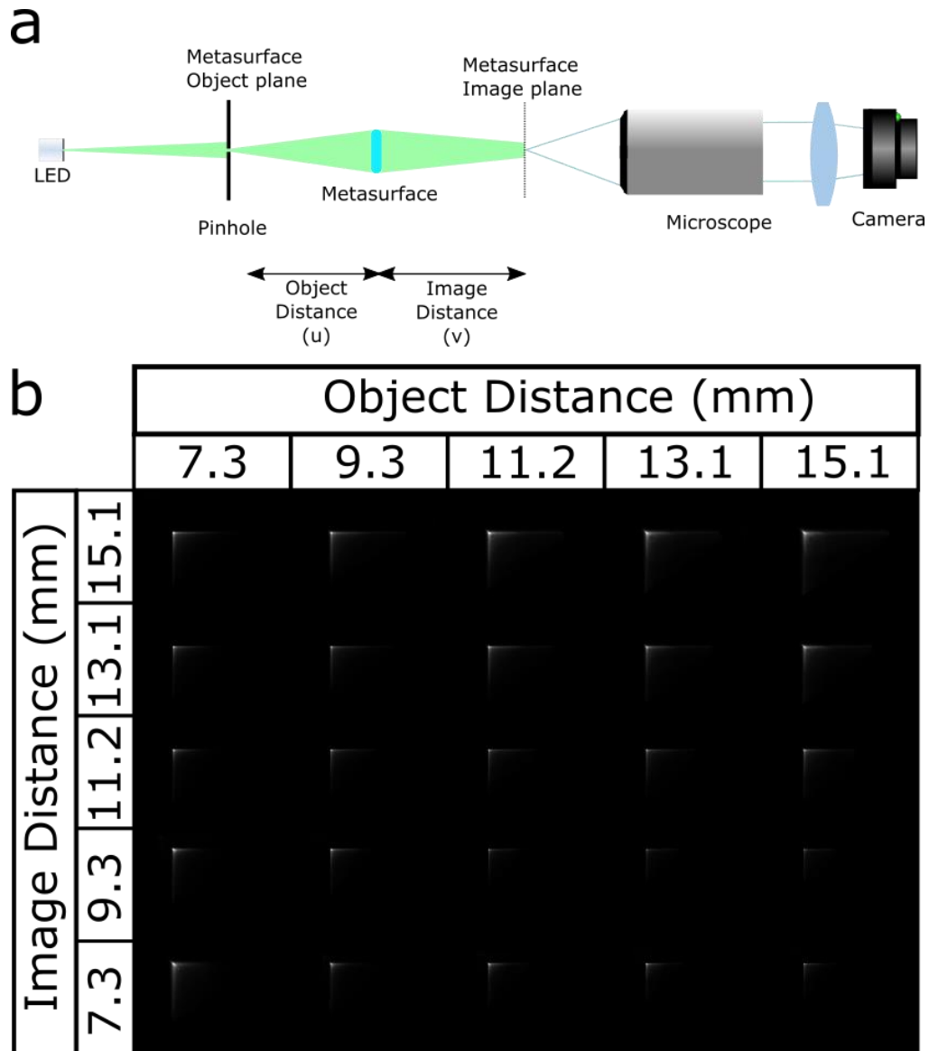
Fig 4.3. a) Setup for PSF measurement. b) Image of 25 \mu m pinhole. Image and object plane sweep. Illumination is using a 530nm LED with 33nm bandwidth.
