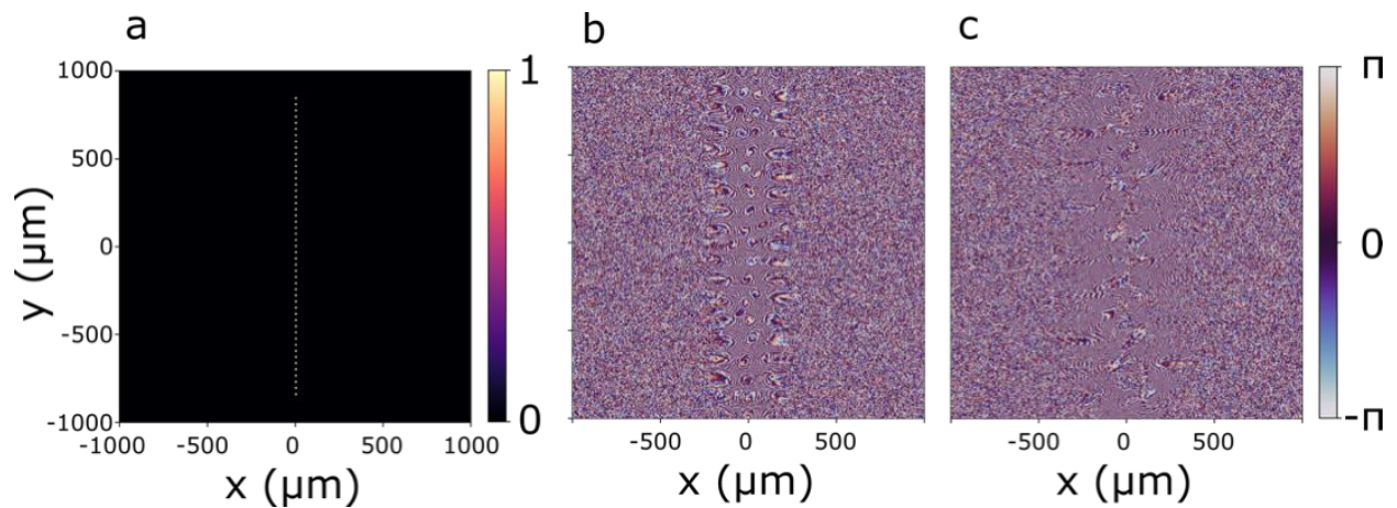
Figure 7.2. a) Input pixel intensity, optimized phase profiles for the a) first and b) second phase mask.
