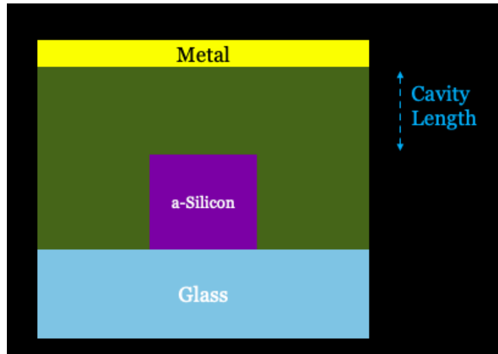
Figure 6.5 – Geometry cross section of a single grating
