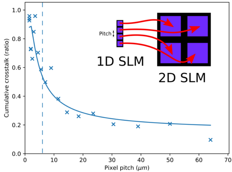
Figure 7.5. Cumulative crosstalk between output modes for a range of trained systems that map a 4-pixel 1D SLM to a 2 \times 2 output SLM. The simulation region was shrunk by a factor of 10 to clearly observe the breakdown of our proposed method. All other simulation parameters are identical to the featured model except for the input pixel pitch. The solid curve serves as a guide to the eye.
