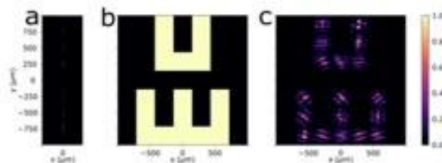
Figure 7.4. a) 1D SLM input field b) Target output field c) Simulated output field using 1D-to-2D mapping
