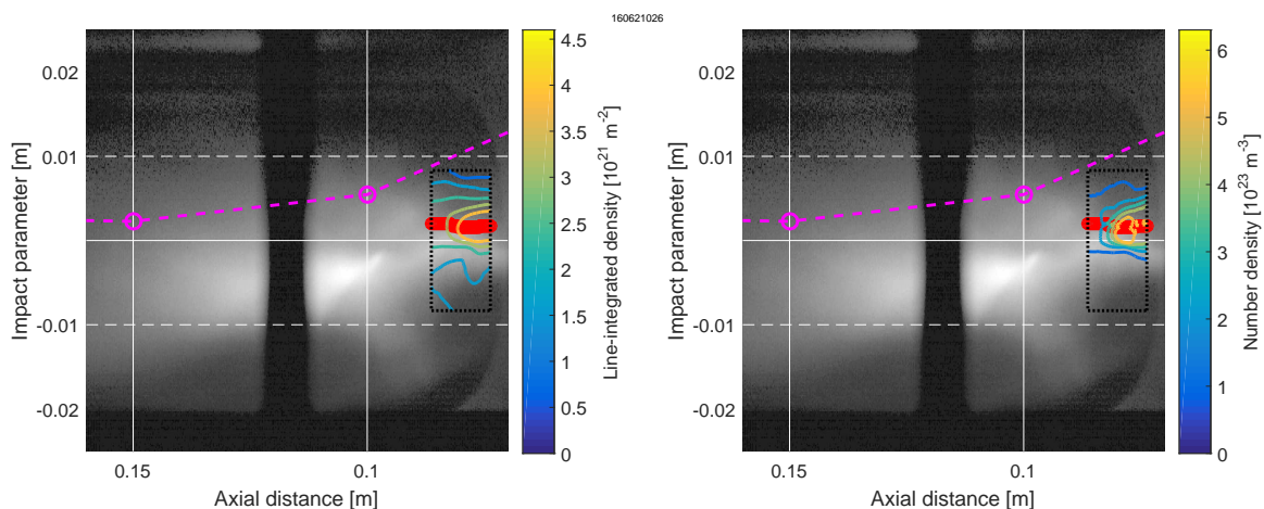
Figure 5.9: Contours of (left) line-integrated density and (right) number density are plotted over an optical image taken during pulse 160621026 at 50 \mu\text{s} , the time of the DHI pulse. The magenta circles are the current centroid locations projected into the plane of the image, and the red markers indicate the density centroids computed during Abel inversion. This image shows fair agreement between the image, density data, and centroid position. The vertical shadow at 0.12 m is part of a 3D printed hanger holding a laser beam guide. The shadow of the beam guide is visible at the right edge of the image.
