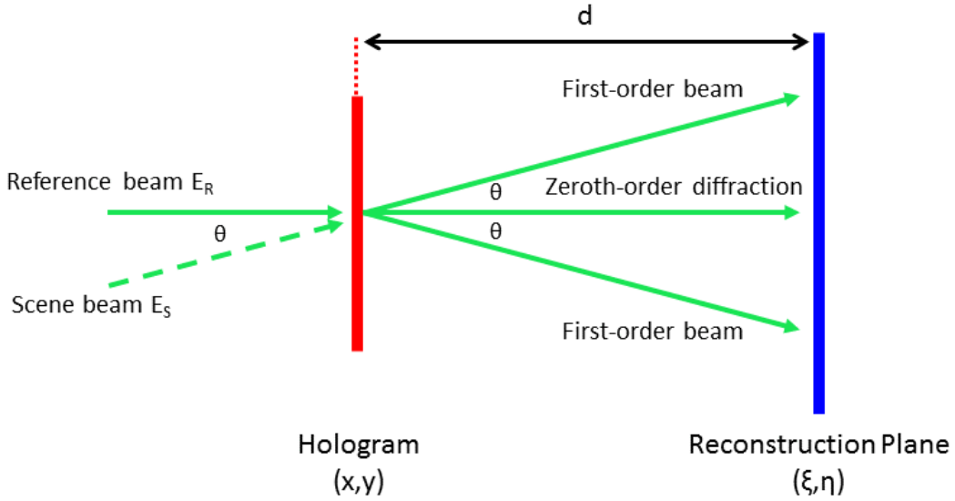
Figure 3.2: If the reference beam is incident normal to the hologram, both first-order beams propagate at the incident angle of the original scene beam, \theta . Reconstruction distance, d , spans from the hologram to the reconstruction plane. In the case of a planar reference beam, the phase distributions of the two first-order diffraction beams are identical except for being 180-degrees shifted. Therefore, the reconstructed phase maps resulting from the first-order diffraction beams are commonly called twin images. Zeroth-order diffraction is the portion of the reference beam that does not diffract; it contains no useful information.
