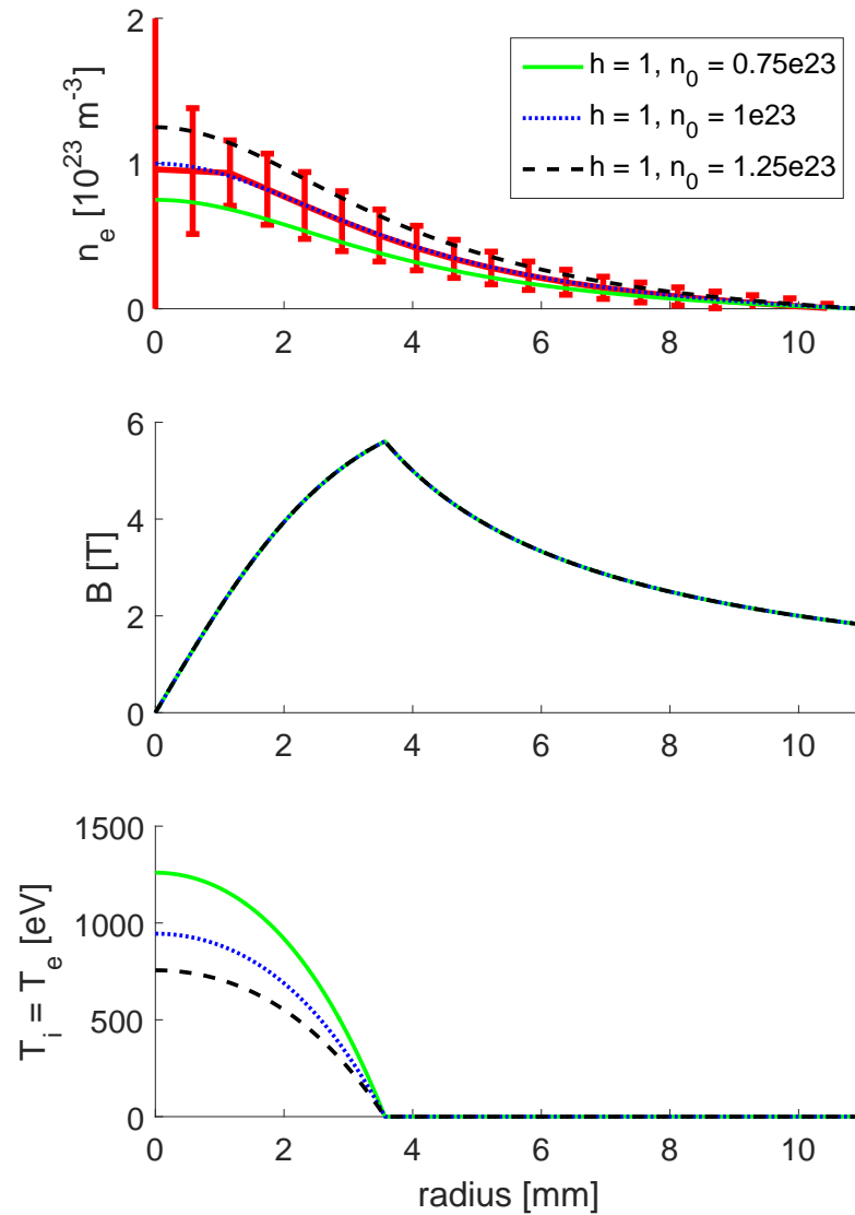
Figure 4.2: Results of equilibrium analysis of three Lorentzian density profiles with different peak densities and identical shape parameter, h = 1 . Changing the peak density does not affect the magnetic field, but it does change the temperature profile. Changing only the peak density does not affect the radius a .
