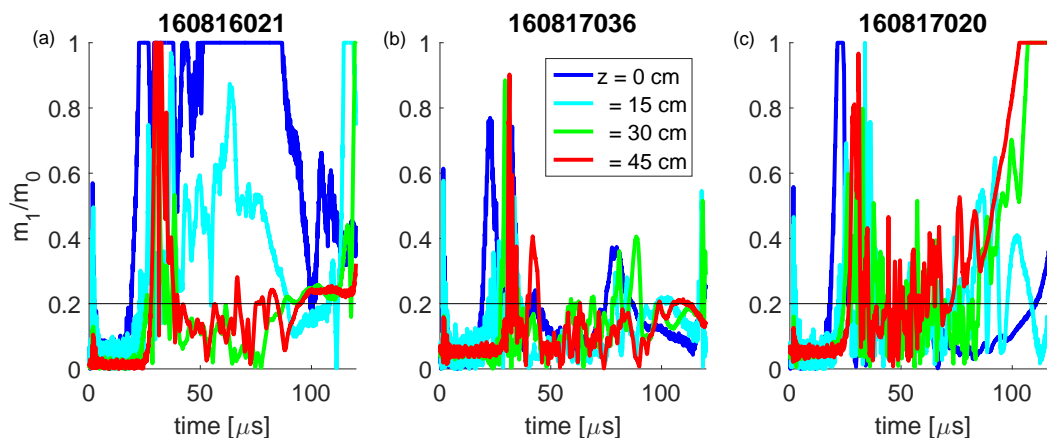
Figure 5.2: Normalized magnetic mode data, m_1/m_0 , showing stability initially improves with increased compression bank voltage and then degrades at high voltages. Compression bank voltages of (a) 0 kV, (b) 2 kV, and (c) 8 kV are shown for pulses with otherwise identical run settings. Horizontal black lines indicate a current centroid displacement of 1 cm.
