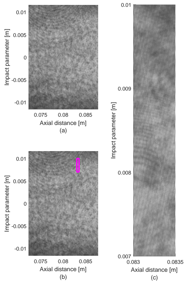
Figure 3.7: Raw experimental (a) vacuum (pulse 160524020) and (b) plasma (pulse 160524021) holograms. The horizontal axes measure the distance downstream from the ZaP-HD nose cone, and the vertical axes indicate the impact parameter relative to the geometric axis of the outer electrode. The full holograms exhibit aliasing at this size, so the subsection of the plasma hologram identified by the magenta box has been magnified in (c) to resolve the approximately vertical d_f \approx 20 \mu\text{m} fringes. The small fringe size and gradual density gradient make it difficult to see the phase shift in the raw data, but Fresnel transform reconstruction reveals shifts of approximately one fringe.
