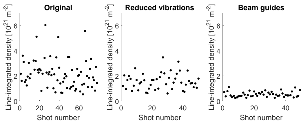
Figure 5.19: Comparison of the baseline variability during the original DHI set up, a reduced vibration set up, and the reduced vibration set up including beam guides. The beam guides significantly reduced baseline variability.
