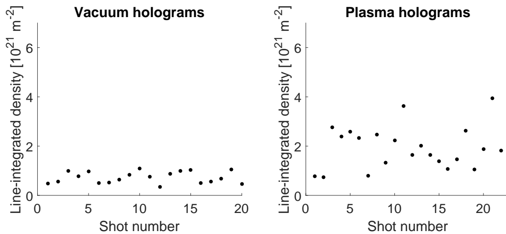
Figure 5.20: Line-integrated density from many vacuum and plasma holograms after DHI beam guide installation showing the noise level on baselines is below the line-integrated density seen on plasma pulses.
