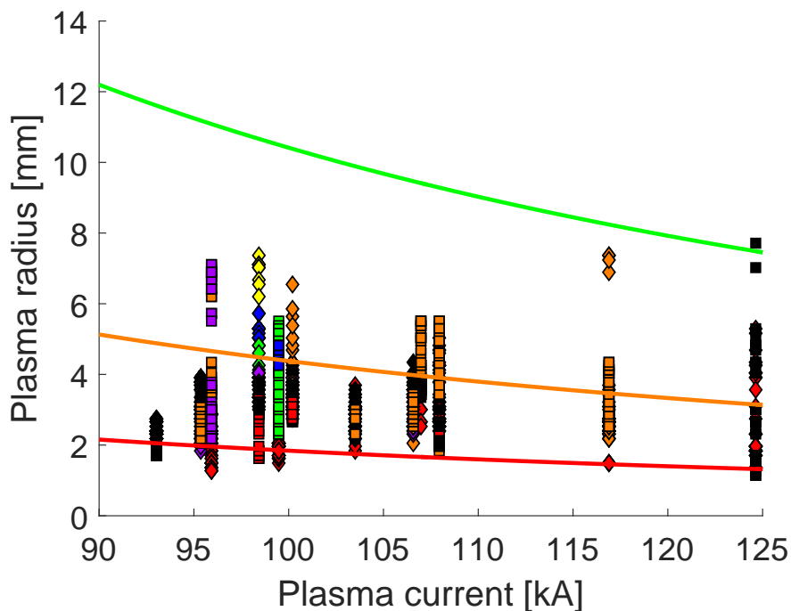
Figure 4.20: Plasma radius plotted versus plasma current for profiles from many plasma pulses with similar run settings. Markers are colored according to the linear density ranges in Fig. 4.15. The orange curve represents the adiabatic scaling of Eq. (1.9) for the orange linear density bin. The curve is drawn from Eq. (1.9) with N_2/N_1 = 1 and an initial state chosen to maximize the proximity of the curve to the orange markers. The green and red curves indicate the adiabatic scaling for values of N_2/N_1 of 2 and 1/2 respectively, which correspond to the green and red linear density ranges. The insensitivity of the observed plasma radius over this range of currents matches the adiabatic prediction. The dependence of the radius on the linear density appears to follow the trend of adiabatic theory with lower linear density markers generally located towards the bottom of the plot.
