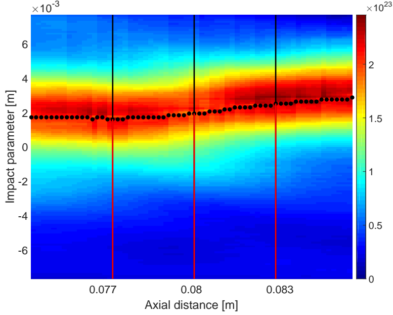
Figure 3.10: The n_e from Abel inversion of the N_e in Fig. 3.9(a) using the centroids plotted as black dots. The vertical lines correspond to the profiles plotted in Fig. 3.11.
