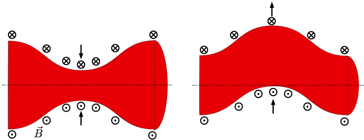
Figure 1.1: Sausage and kink mode instabilities are shown at left and right respectively. The magnetic fields induced by current flow from right to left are shown. The sausage mode results in azimuthally symmetric \vec{B} concentration that causes the pinch to further constrict. The kink mode causes an asymmetric \vec{B} concentration that drives the pinch further off axis.
