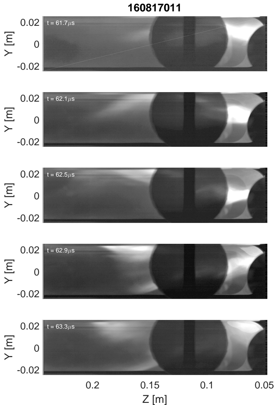
Figure 5.8: High speed camera images contrasting unfiltered and filtered plasma light emission. The circular bremsstrahlung filter is visible between z = 10 and 15 cm. Structures originating in the unfiltered region upstream are visible moving through the filtered region and then out into the unfiltered region downstream. Observations consistently see strong correlation between unfiltered and filtered structures. The vertical shadow at 0.12 m is part of a 3D printed hanger holding a laser beam guide. The shadow of the beam guide is visible at the right edge of the image.
