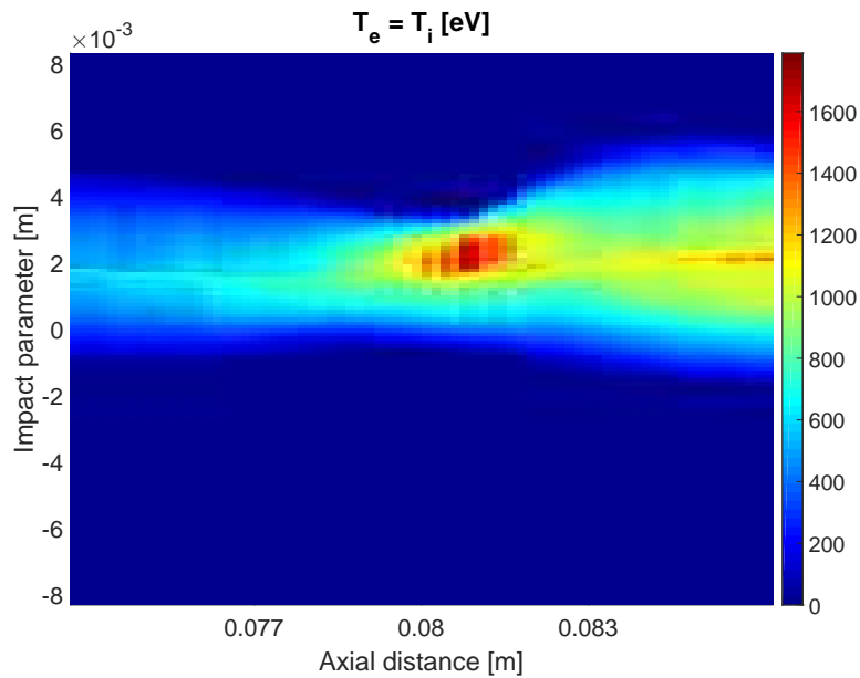
Figure 4.14: Contours of temperature for pulse 160621026 analyzed in Fig. 4.11. This pulse exhibits significant axial variation in temperature with the hottest temperatures in cross-sections with the smallest pinch radii.
