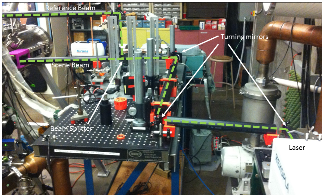
Figure B.5: The DHI's optical set up on the upstream optics table. The dashed green line shows the laser's path through black beam guides meant to block air currents. Three turning mirrors raise the Nd:YAG laser beam to the height of the ZaP-HD mid-plane.
