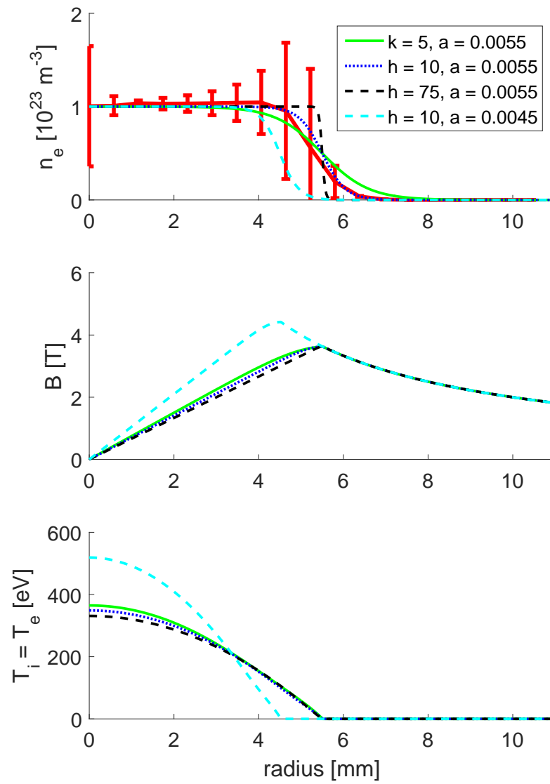
Figure 4.4: Results of equilibrium analysis of four hyperbolic tangent profiles with varying steepness and size. The field and temperature are insensitive to profile steepness, while changing the specified radius makes a greater difference in the analysis.
