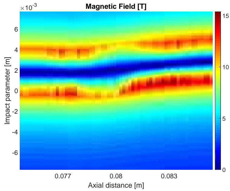
Figure 4.8: Contour plot of magnetic field strength computed from uniform drift velocity equilibrium analysis for pulse 160524021. The density contour for this relatively axially uniform pulse is Fig. 4.7.
