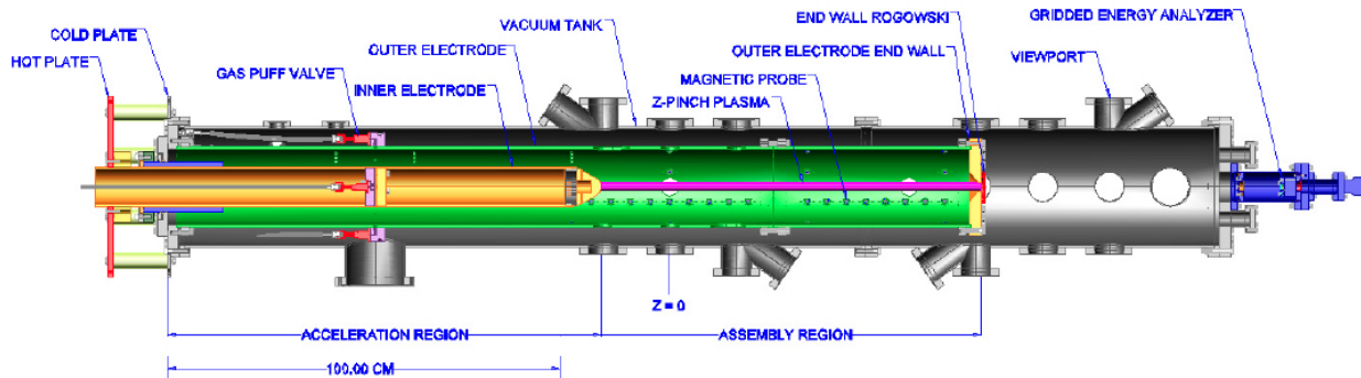
Figure 1.4: A cross-section of the ZaP experiment shows its internal design. The inner and outer electrodes are colored yellow and green respectively, the vacuum chamber is shown in gray, and the Z-pinch is in pink. The coaxial accelerator ionizes plasma and pushes it into the assembly region. The z = 0 location for ZaP’s axial coordinate system is shown. The z -coordinate increases to the right in units of cm; locations left of z = 0 are negative.
