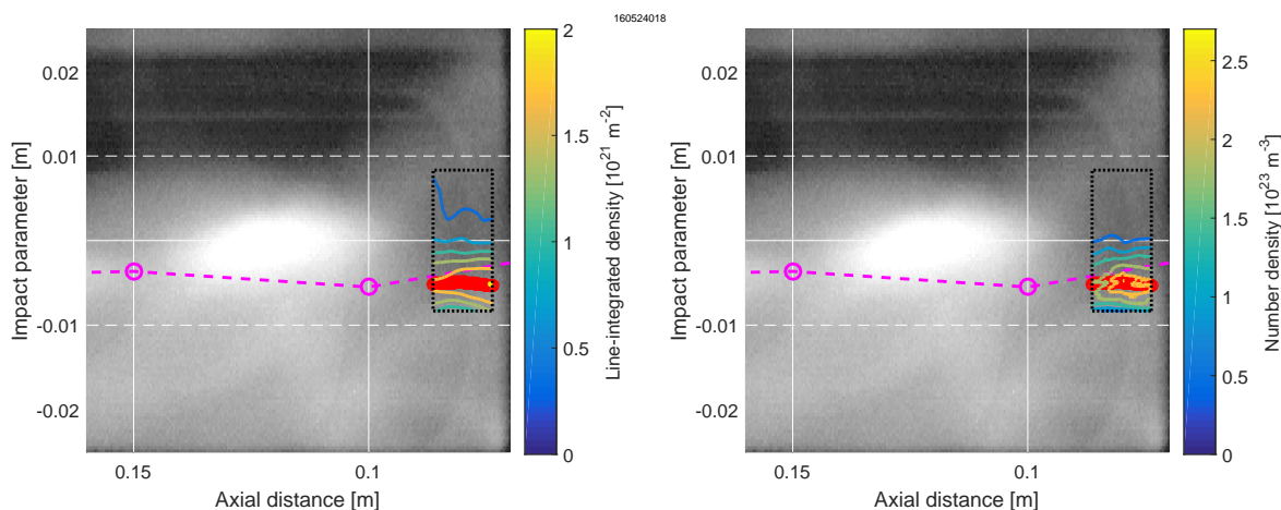
Figure 5.10: Contours of (left) line-integrated density and (right) number density are plotted over an optical image taken during pulse 160524018 at 50 \mu\text{s} , the time of the DHI pulse. The magenta circles are the current centroid locations projected into the plane of the image, and the red markers indicate the density centroid computed during Abel inversion. This image shows good agreement between the image, density data, and centroid position. The downstream scene beam guide was removed on this pulse, but testing showed this section of beam guide made little difference to the DHI's signal to noise.
