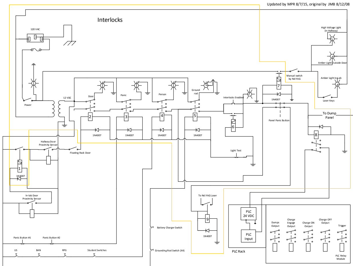
Figure B.1: Electronic schematic of the ZaP-HD interlocks system. Items within the orange box are inside the 19 inch rack mount panel while all other items are external. The Nd:YAG laser needs to see a short circuit connection to allow itself to enter run mode. Relay number 9 inside the panel will short the laser interlock circuit provided all interlock conditions are met except the grounding rod condition. A manual switch in the lab next to the laser allows the user to toggle the high voltage warning lights even when no interlocks are met. This allows users to discourage unauthorized lab entry during DHI alignment.
