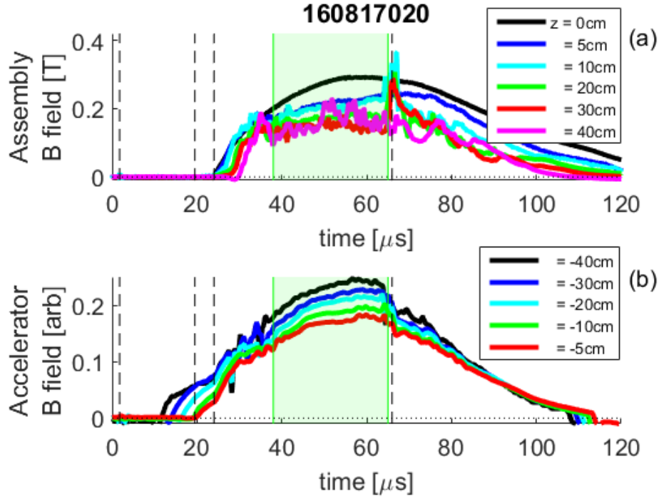
Figure 2.8: In a typical ZaP-HD plasma pulse, (a) the average magnetic fields from assembly azimuthal probe arrays rise one after another starting with the z = 0 array at the time of the compression bank discharge. During the quiescent period denoted by shaded green, the radial current distribution in the assembly region remains more or less constant in time. Radial currents exist between z = 0 cm and 20 cm, although current further downstream is more purely axial. (b) The relative magnitudes of the magnetic fields in the accelerator linear probe array initially rise one after another as the initial plasma front moves down the gun. The time this plasma front exits the accelerator matches the time V_M goes to zero in Fig. 2.7. During the quiescent period, radial current exists in the accelerator, while an abrupt decrease in the radial current marks the end of the quiescent period. The first, second, third, and fourth dashed vertical lines correspond to the acceleration bank discharge, plasma exiting the accelerator, the compression bank discharge, and the high peak in the assembly magnetic field respectively.
