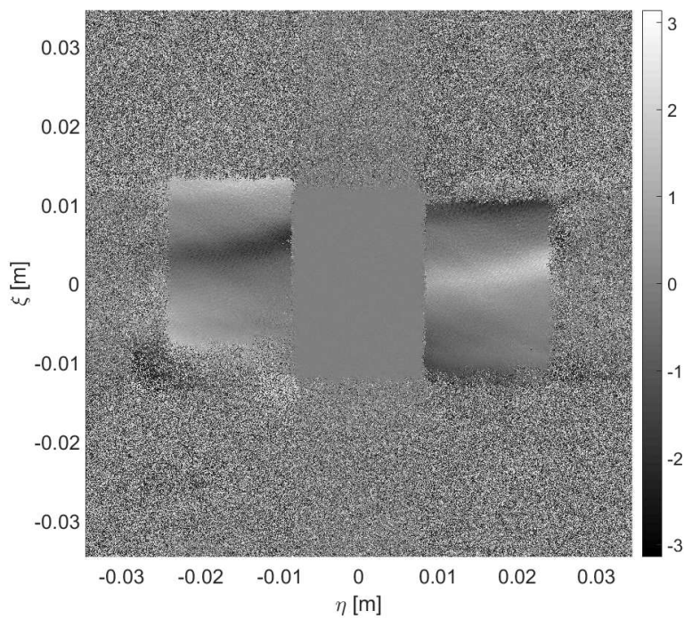
Figure 3.8: The reconstructed phase difference (between pulses 160524021 and 160524020) at a reconstruction distance d = 0.5 m. This figure shows the equivalent of the reconstructed phase difference shown in Fig. 3.6 for experimental plasma data. The choice of reconstruction distance here maximizes the size of the twin images and therefore the resolution obtained for the reconstruction. A smaller reconstruction distance would lead to the zeroth-order image obscuring the twin images.
