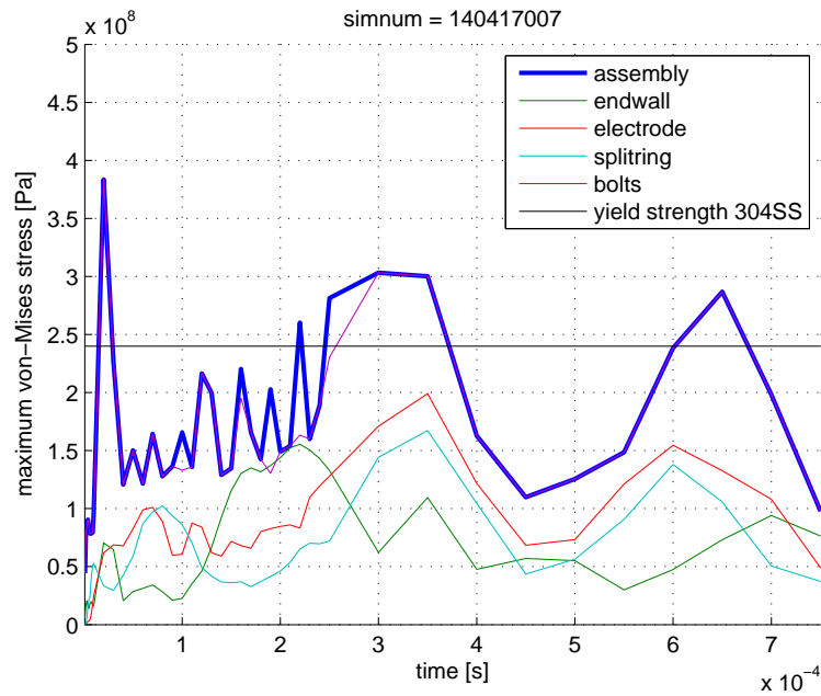
Figure D.9: The max von Mises stresses in each component of the spoked endwall assembly exhibit damped oscillations in time.
