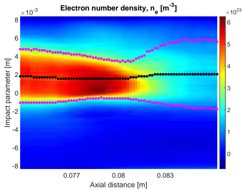
Figure 4.12: Contours of density for pulse 160621026 analyzed in Fig. 4.11. The black dots indicate the centroids used in Abel inversion, and the magenta dots indicate the radius a for each profile where the density drops to half its peak value. This pulse exhibits significant axial variation in density.
