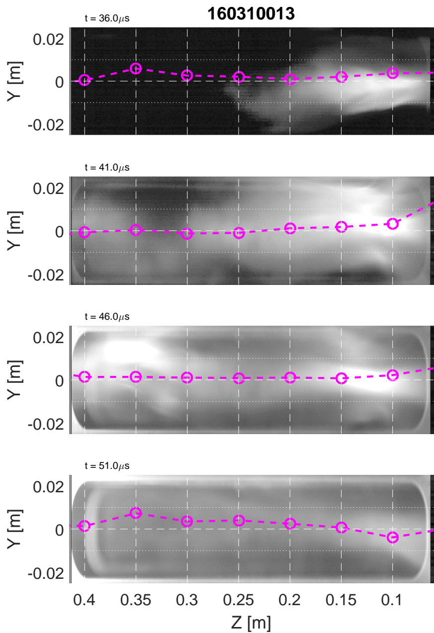
Figure 5.3: High speed camera images showing the typical appearance of a stable Z-pinch during a 14 \mu\text{s} quiescent period from 36 to 51 \mu\text{s} during pulse 160310013. The frame at 41 \mu\text{s} shows the distinct necking behavior localized at z = 10 - 15 \text{ cm} typical of stable Z-pinchs. The intensity is shown on a logarithmic scale.
