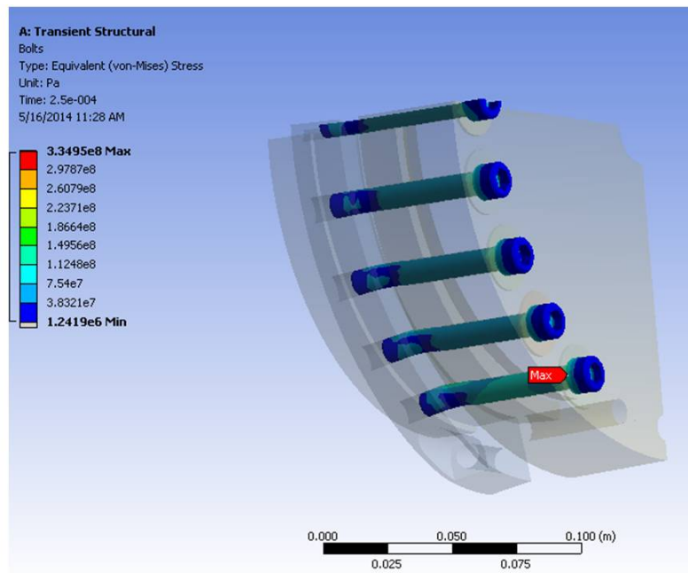
Figure D.13: For the single hole endwall, the von Mises stresses in the bolts at the instant of maximum stress.
