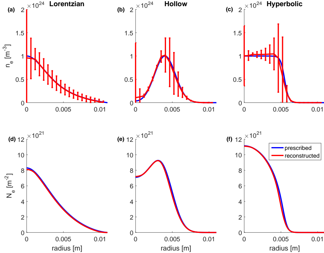
Figure 3.5: Prescribed number density profiles and their corresponding line-integrated profiles are shown in blue in (a) and (d) for the Lorentzian profile of Eq. (3.27), (b) and (e) for the hollow profile of Eq. (3.28), and (c) and (f) for the hyperbolic tangent profile of Eq. (3.29). The red curves are the profiles reconstructed from synthetic holograms. The differences between the assumed and reconstructed line-integrated density profiles are propagated through an Abel inversion to compute the uncertainties in the number densities, which are plotted as red error bars.
