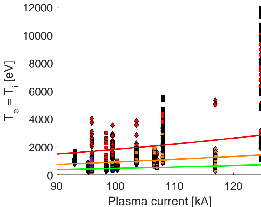
Figure 4.21: Temperature plotted versus plasma current for profiles from many plasma pulses with similar run settings. Markers are colored according to the linear density ranges in Fig. 4.15. The orange curve represents the adiabatic scaling of Eq. (1.7) for the orange linear density bin. The curve is drawn from Eq. (1.7) with N_2/N_1 = 1 and an initial state chosen to maximize the proximity of the curve to the orange markers. The green and red curves indicate the adiabatic scaling for values of N_2/N_1 of 2 and 1/2 respectively, which correspond to the green and red linear density ranges. The insensitivity of the observed temperature over this range of currents matches the adiabatic prediction. The dependence of the temperature on the linear density appears to follow the trend of adiabatic theory with lower linear density markers generally located towards the top of the plot.
