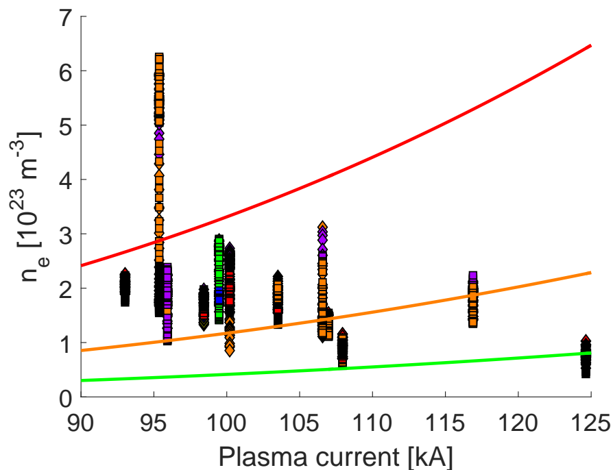
Figure 4.19: Electron density plotted versus plasma current for profiles from many plasma pulses with similar run settings. Markers are colored according to the linear density ranges in Fig. 4.15. The orange curve represents the adiabatic scaling of Eq. (4.19) for the orange linear density bin. The curve is drawn from Eq. (4.19) with N_2/N_1 = 1 and an initial state chosen to maximize the proximity of the curve to the orange markers. The green and red curves indicate the adiabatic scaling for values of N_2/N_1 of 2 and 1/2 respectively, which correspond to the green and red linear density ranges. The dependence of the measured density on the linear density does not appear to follow the adiabatic theory. The empirical density does not scale up as effectively as adiabatic theory predicts.
