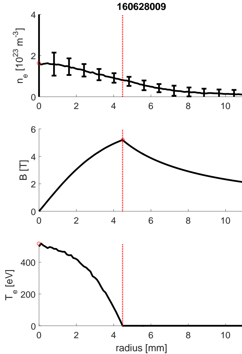
Figure 4.6: Cross-sections of measured density and computed field and temperature from the uniform drift velocity equilibrium model for pulse 160628009. This pulse exhibits relatively wide profiles. The vertical red lines indicate the pinch radius, a , and the red circles indicate the peak density, edge field, and peak temperature values taken as characteristic property values.
