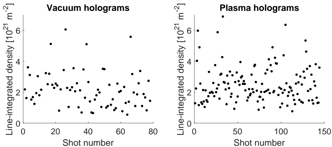
Figure 5.18: Line-integrated density from many vacuum and plasma holograms prior to DHI beam guide installation showing the noise level on baselines is similar to the line-integrated density seen on plasma pulses.
