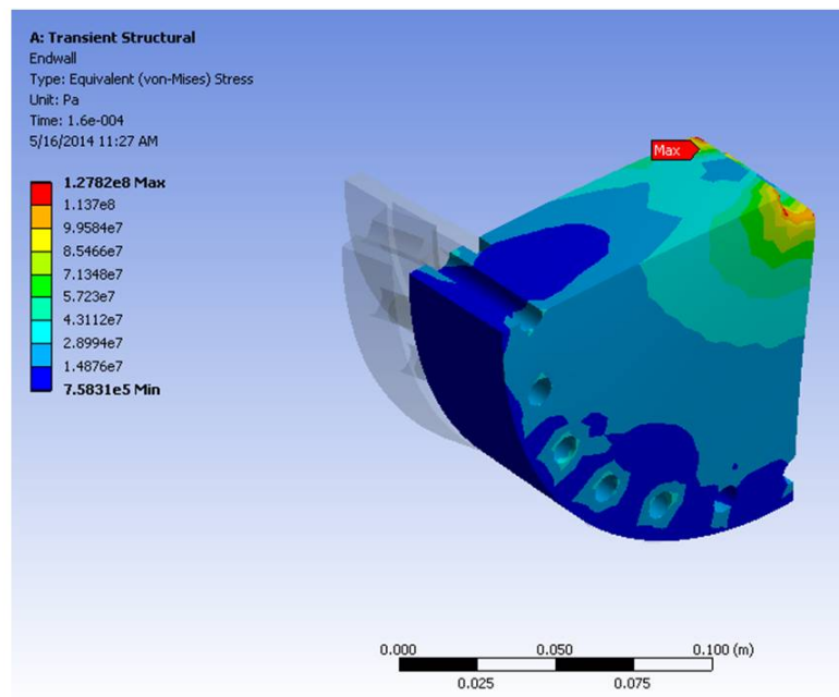
Figure D.12: For the single hole endwall, the von Mises stresses in the endwall at the instant of maximum stress.
