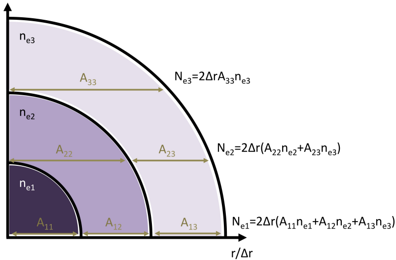
Figure 3.3: The Abel transform breaks up an axisymmetric plasma into concentric annular areas. Assuming uniform n_e in each annulus makes computation of N_e a matter of multiplying the discrete n_e by a matrix \mathbf{A} containing the relative lengths of chord lengths in the geometry. The elements of \mathbf{A} for a coarse discretization are shown here. \mathbf{A} can be expanded to arbitrary size to transform arbitrarily large n_e profiles.
