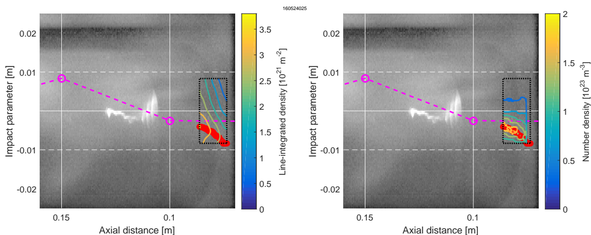
Figure 5.13: Contours of (left) line-integrated density and (right) number density are plotted over an optical image taken during pulse 160524025 at 50 \mu\text{s} , the time of the DHI pulse. The magenta circles are the current centroid locations projected into the plane of the image, and the red markers indicate the density centroid computed during Abel inversion. Excellent correlation exists between density and current centroid, but the light emission is too diffuse to make a meaningful comparison of its position to the other diagnostics. In the upstream portion of the DHI data, the density centroid reaches the edge of the imaged area. At every cross-section where this happens, the number density is set to zero across the cross-section.
