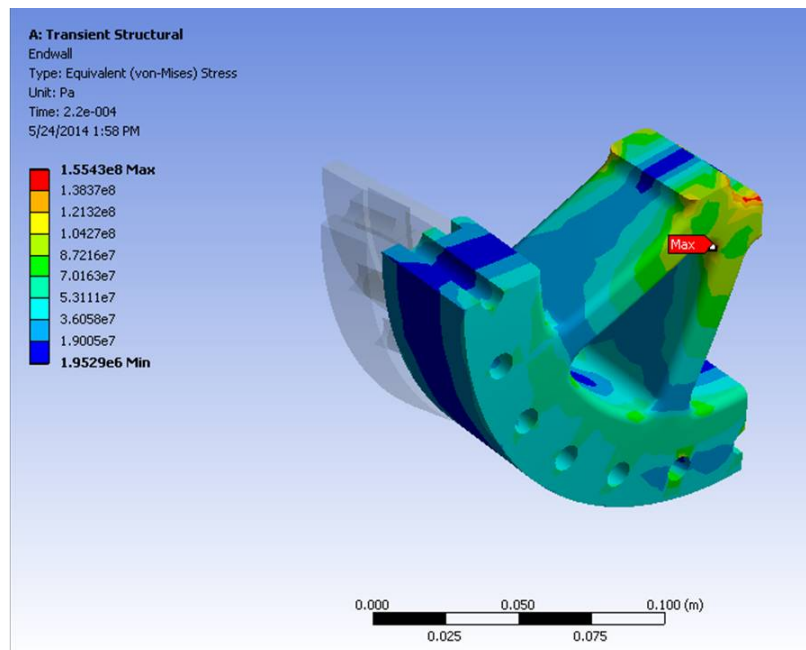
Figure D.16: For the spoked endwall, the von Mises stresses in the endwall at the instant of maximum stress.
