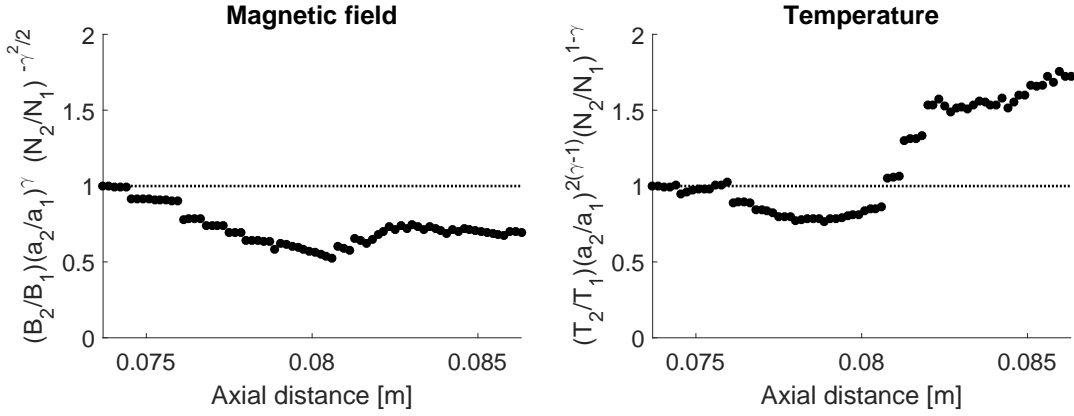
Figure 4.11: Examining relations between pinch size and field and temperature to determine if an axially non-uniform Z-pinch behaves adiabatically. The two plots compare the left and right-hand-sides of Eqs. (4.20, 4.21) for pulse 160621026. The profiles below the density centroids in Fig. 4.12 are used in this analysis, and each black marker corresponds to a profile at a different axial location. Upstream of 0.076 m, the markers near a value of 1 on the ordinate indicate states reached in agreement with the adiabatic scaling laws. Abrupt changes in the ratios of Eqs. (4.23, 4.24) at 0.076 m and 0.081 m suggest non-adiabatic processes dictate the difference between the plasma states at adjacent cross-sections in these locations. The more abrupt change at 0.081 m corresponds to the plasma radius change.
