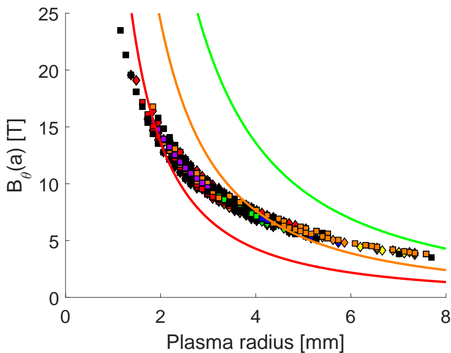
Figure 4.17: Magnetic field plotted versus plasma radius for profiles from many plasma pulses with similar run settings. Markers are colored according to the linear density ranges in Fig. 4.15. The orange curve represents the adiabatic scaling of Eq. (4.21) for the orange linear density bin. The curve is drawn from Eq. (4.21) with N_2/N_1 = 1 and an initial state chosen to maximize the proximity of the curve to the orange markers. The green and red curves indicate the adiabatic scaling for values of N_2/N_1 of 2 and 1/2 respectively, which correspond to the green and red linear density ranges. The empirical B(a) relation appears insensitive to linear density, which does not match the adiabatic prediction. Also, the empirical trend is more gradual than the prediction.
