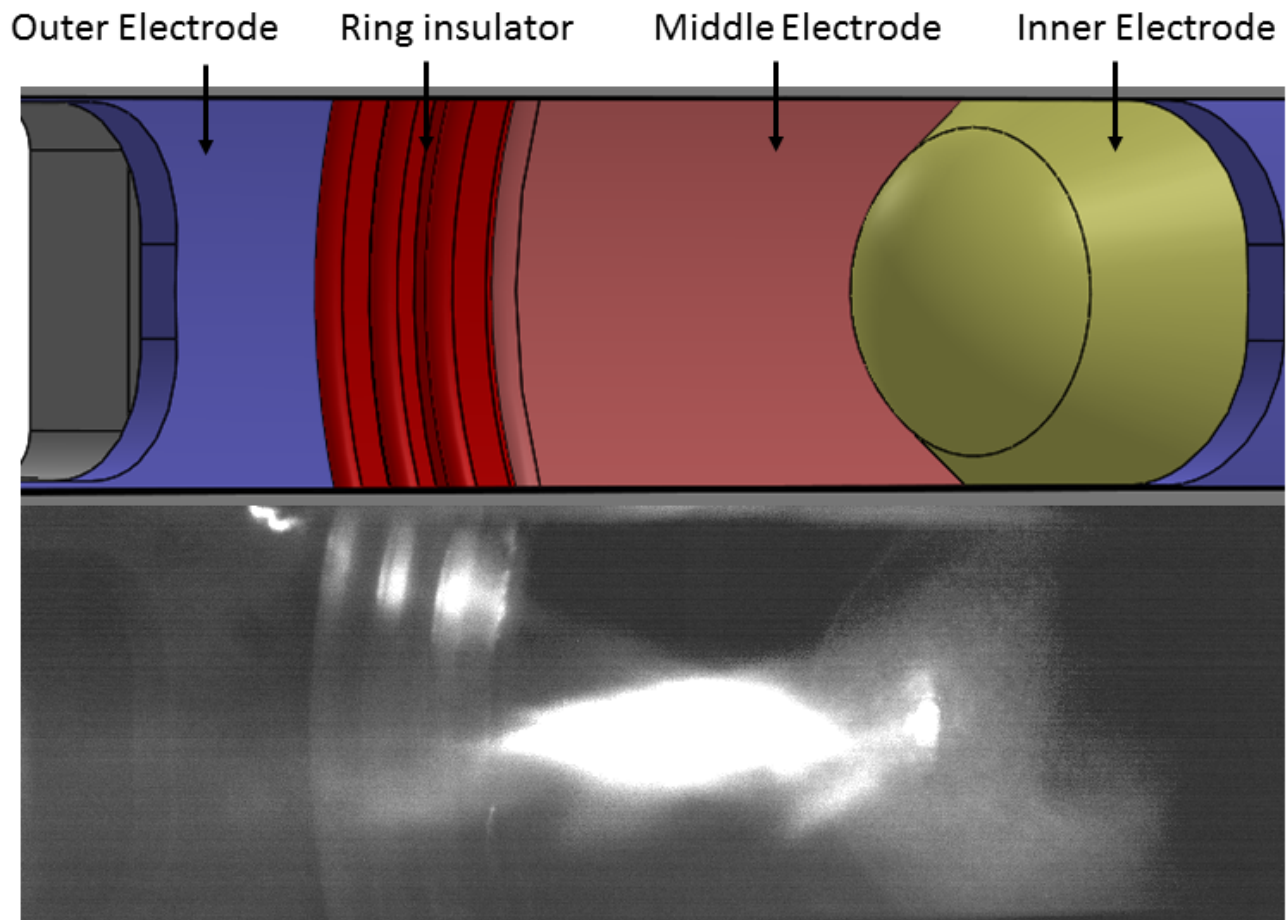
Figure 2.15: (top) A CAD image indicates the positions of the electrodes and ring insulator. (bottom) An optical camera image taken with a bremsstrahlung filter, f stop of 5.6, and exposure time of 200 ns (pulse 160427024). Localized plasma contact between the middle and outer electrodes across the ring insulator correlates with current centroid position data at z = 0 and suggests current flow directly between the outer and middle electrodes. The plasma appears to jump across each of the three ridges in the ring insulator.
