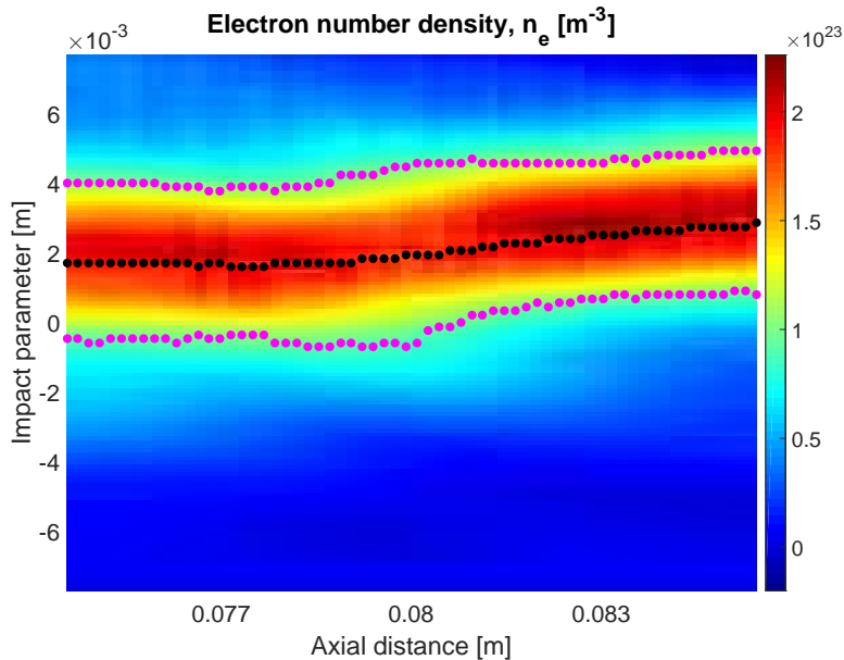
Figure 4.7: Contour plot of electron density measured on pulse 160524021 with markers indicating density centroid and pinch size. The black markers indicate the density centroids identified during Abel inversion, and the magenta markers show the radius a for each profile defined as the location where the density drops to half the max value in the cross-section. The plasma radius bulges slightly near 0.081 m but otherwise remains largely uniform axially.
