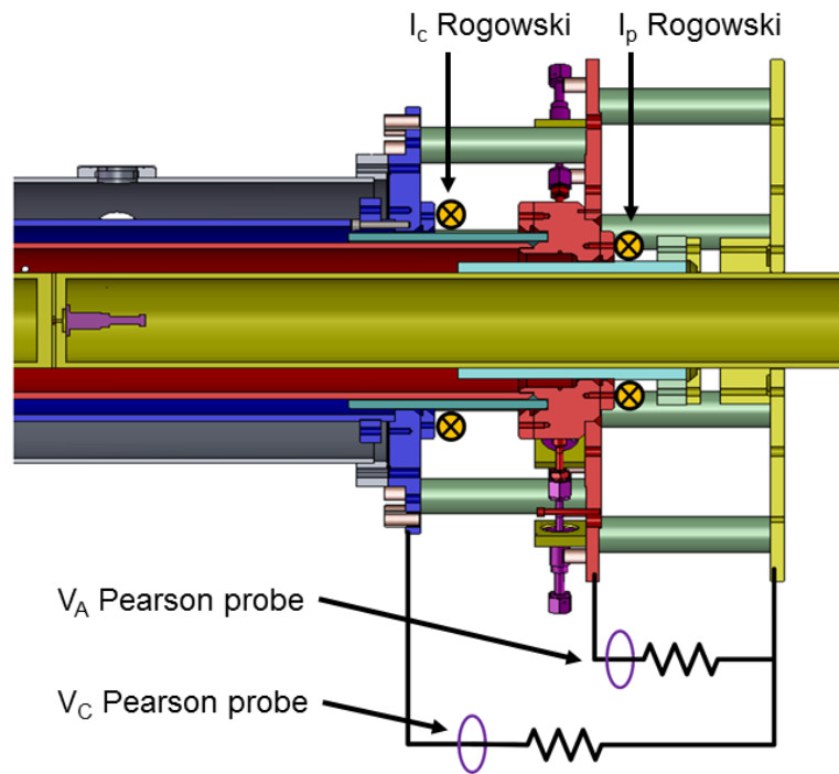
Figure 2.2: A view of the upstream portion of the ZaP-HD electrodes shows the location of the experiment's current and voltage measurements. The orange dots with black crosses indicate the positions of the I_c and I_p Rogowski coils, and the circuit diagram at the bottom illustrates the design of the voltage measurement, which uses Pearson probes to measure the current across high power, non-inductive resistors.
