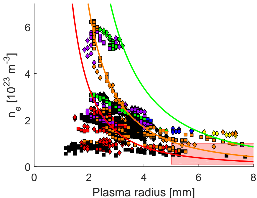
Figure 4.16: Peak density versus plasma radius for profiles from many plasma pulses with similar run settings. Markers are colored according to the linear density ranges in Fig. 4.15. The orange curve represents the adiabatic scaling of Eq. (4.22) for the orange linear density bin. The curve is drawn from Eq. (4.22) with N_2/N_1 = 1 and an initial state chosen to maximize the proximity of the curve to the orange markers. The green and red curves indicate the adiabatic scaling for values of N_2/N_1 of 2 and 1/2 respectively, which correspond to the green and red linear density ranges. The red-shaded box indicates the region of ZaP operations, and extends off the plot to radii of 0.015 m. The empirical data exhibits the same trends as the adiabatic predictions: density increases as pinch size decreases, and markers of higher linear density generally appear towards the upper-right of the plot. The empirical relation between density and radius is more gradual than the adiabatic prediction.
