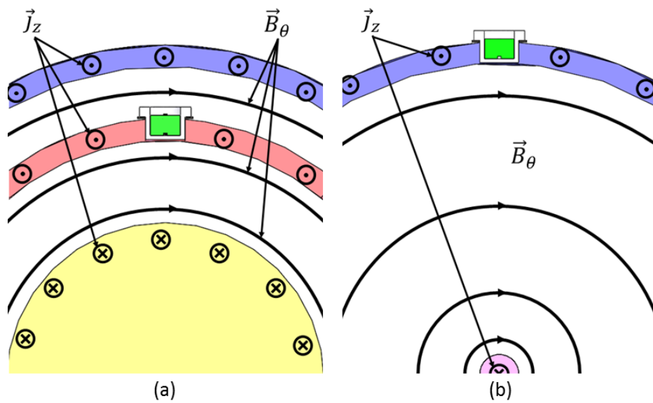
Figure 2.4: Axial cross-sections show the magnetic fields near wall-embedded magnetic field probes for (a) an accelerator probe and (b) an assembly region probe. The inner, middle, and outer electrodes are shown in yellow, red, and blue respectively in (a). In (b), the outer electrode is blue and the Z-pinch plasma is pink. Directions of current flow are shown by vectors into and out of the page, and magnetic field lines are also drawn. Boron nitride probe shields are shown in white, and Kel-F plastic forms are green.
