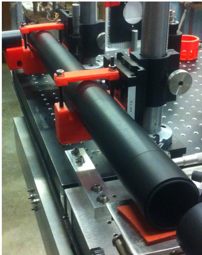
Figure B.4: The DHI beam expander is held by orange 3D-printed clamps. The clamps mount to 1.5" vertical posts and linear translators, which give the user independent control of the position of the two lenses in the expander.
