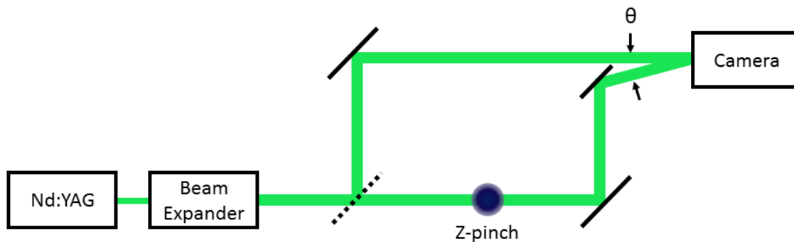
Figure 3.1: A Mach-Zehnder interferometer splits a laser beam into two identical beams. One beam passes through the plasma while the other bypasses the experiment. Then, the beams are recombined with a beamsplitter and recorded on a camera or other sensor. The phase shift between the two beams is proportional to the plasma’s line-integrated electron density.
