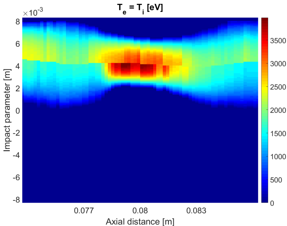
Figure 5.17: Temperature contour plot showing high temperature at the constriction of a sausage mode instability. Temperature values are computed with the analysis of Ch. 4 from the density in Fig. 5.15.
