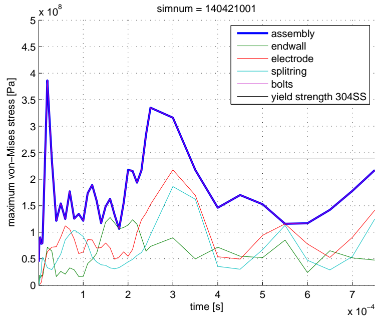
Figure D.8: The max von Mises stresses in each component of the single hole endwall assembly exhibit damped oscillations in time. Stresses before 100 \mu\text{s} are caused by bolt pre-tension.
