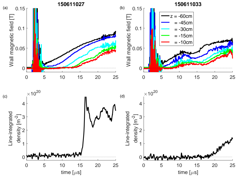
Figure 2.10: (a) Accelerator probe data shows a slower-moving current front when the outer gas is given more time to expand. (c) An interferometry chords at z = 7 cm and y = 0 cm shows an abrupt arrival of density in the assembly region. These characteristics are indicative of snowplow operation where plasma is entrained by the current front and pushed downstream. Pulse 150611027 had inner/outer gas timings of -0.6/-1.0 ms. (b) Accelerator probe data shows a faster-moving current front when the outer gas is given less time to expand. (d) Interferometry shows a more gradual density arrival. Both these characteristics are indicative of a deflagration mode of operation. Pulse 150611033 had inner/outer gas timings of -0.6/-0.8 ms.
