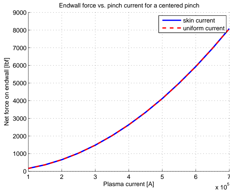
Figure D.6: For on-axis pinches (the best case loading scenario), the current profile does not affect the scaling between load and current. This lack of sensitivity is expected because the pressure profiles for the current profiles are identical beyond the radius of the pinch.
