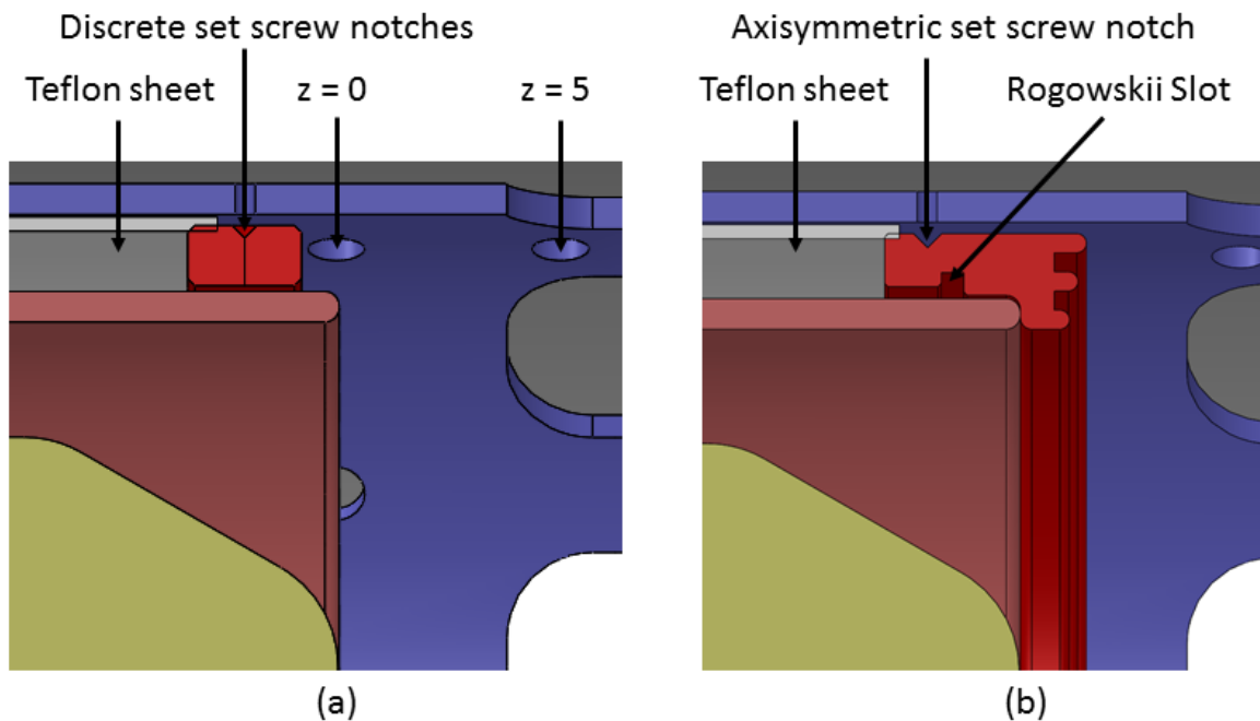
Figure 2.11: (a) In ZaP-HD's original design, a simple ring of electrically insulating alumina was intended to block plasma flow into the gap between the middle and outer electrodes upstream of the accelerator exit. Plasma arcing across the insulator surface may have contributed to large radial currents just downstream of the accelerator. (b) A modified ring insulator extends further downstream with machined grooves meant to baffle surface tracking arcs.
