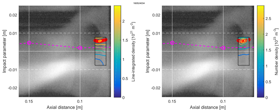
Figure 5.14: Contours of (left) line-integrated density and (right) number density are plotted over an optical image taken during pulse 160524034 at 50 \mu\text{s} , the time of the DHI pulse. The magenta circles are the current centroid locations projected into the plane of the image, and the red markers indicate the density centroid computed during Abel inversion. Excellent correlation exists between density and current centroid, but the light emission is too diffuse to make a meaningful comparison of its position to the other diagnostics.
