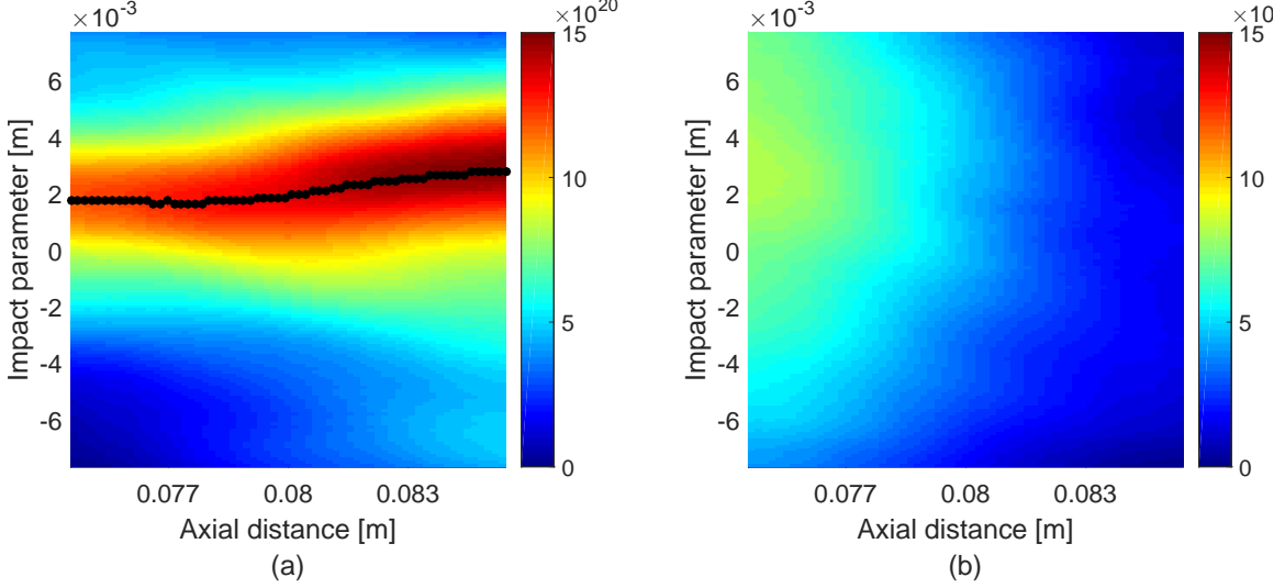
Figure 3.9: (a) A subsection of one of the twin images of Fig. 3.8 smoothed and converted to N_e . The horizontal axis measures the distance downstream from the ZaP-HD nose cone, and the vertical axis indicates the impact parameter relative to the geometric axis of the outer electrode. The black dots indicate centroid locations identified by the Abel inversion process. (b) A twin image of N_e obtained from computing the phase difference between two vacuum holograms (pulses 160524020 and 160524017), one of which was used to find the phase difference with the plasma hologram leading to Fig. 3.9(a). The N_e variation of 1.5 \times 10^{21} \text{ m}^{-2} observed across axial cross-sections of (a) is much larger than the 3 \times 10^{20} \text{ m}^{-2} variation seen across (b).
