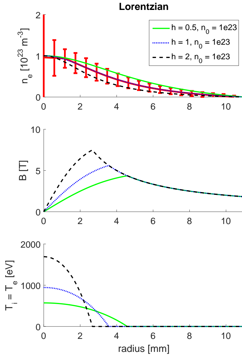
Figure 4.3: Results of equilibrium analysis of three Lorentzian-like density profiles with identical peak densities and different shape parameters. Changing the density profile shape affects both the field and the temperature. Note that changing the profile shape affects radius a .
