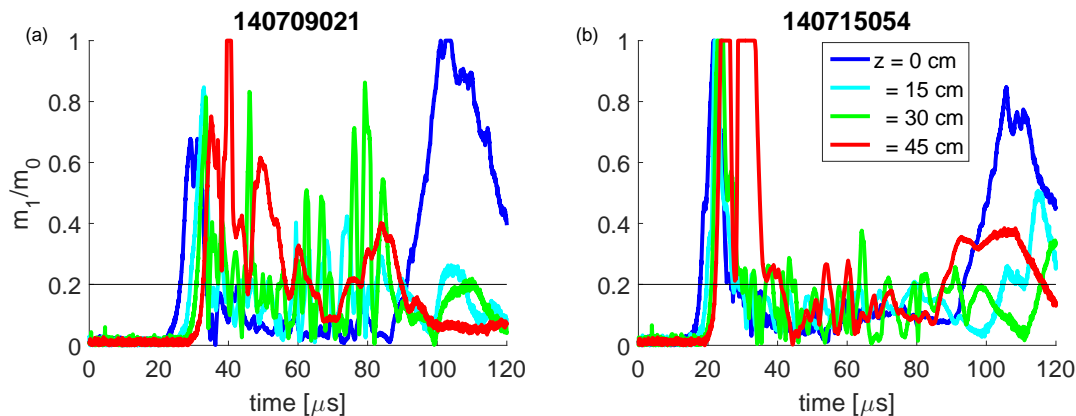
Figure 5.1: Normalized magnetic mode data, m_1/m_0 , showing stability improves with increased acceleration bank voltage. The middle electrode was grounded to the outer electrode for the pulses shown during testing of the accelerator. Acceleration bank voltages of (a) 3.5 kV and (b) 6 kV are shown for pulses with otherwise identical run settings. Horizontal black lines indicate a current centroid displacement of 1 cm.
