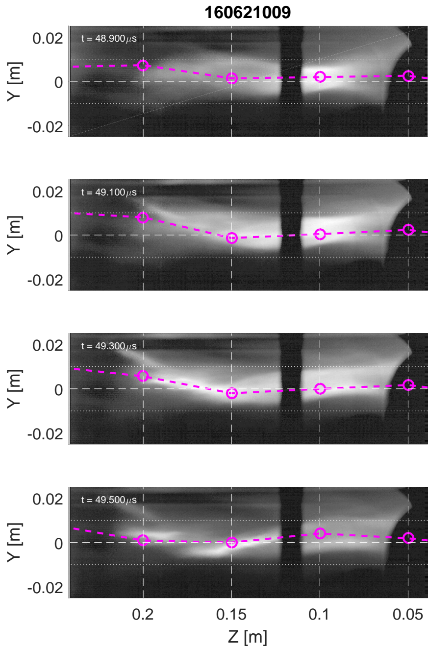
Figure 5.5: High speed camera images showing relatively large scale, slow moving structure correlates well with current centroid locations. The intensity is shown on a logarithmic scale. The vertical shadow at 0.12 m is part of a 3D printed hanger holding a laser beam guide. The shadow of the beam guide is visible at the right edge of the image.
