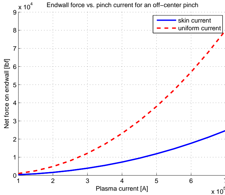
Figure D.5: For off-axis pinches (the worst case loading scenario), the choice of current profile significantly alters the scaling relation between load and current. The uniform current profile scales to much higher endwall loads for a given current than does the skin current profile.
