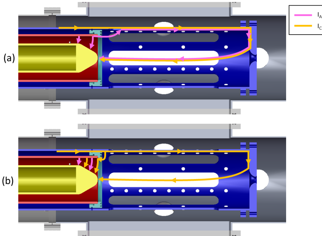
Figure 2.17: Illustration of the flow of I_A and I_C in ZaP-HD for (a) the case of low compression bank charge voltage relative to acceleration bank charge voltage. Acceleration current flows from the middle electrode to the outer electrode. This topology applies for 0 kV compression bank charge except in that case I_C = 0 . (b) The case of high compression bank charge voltage relative to acceleration bank charge voltage. Compression current flows from the outer electrode to the middle and inner electrodes.
