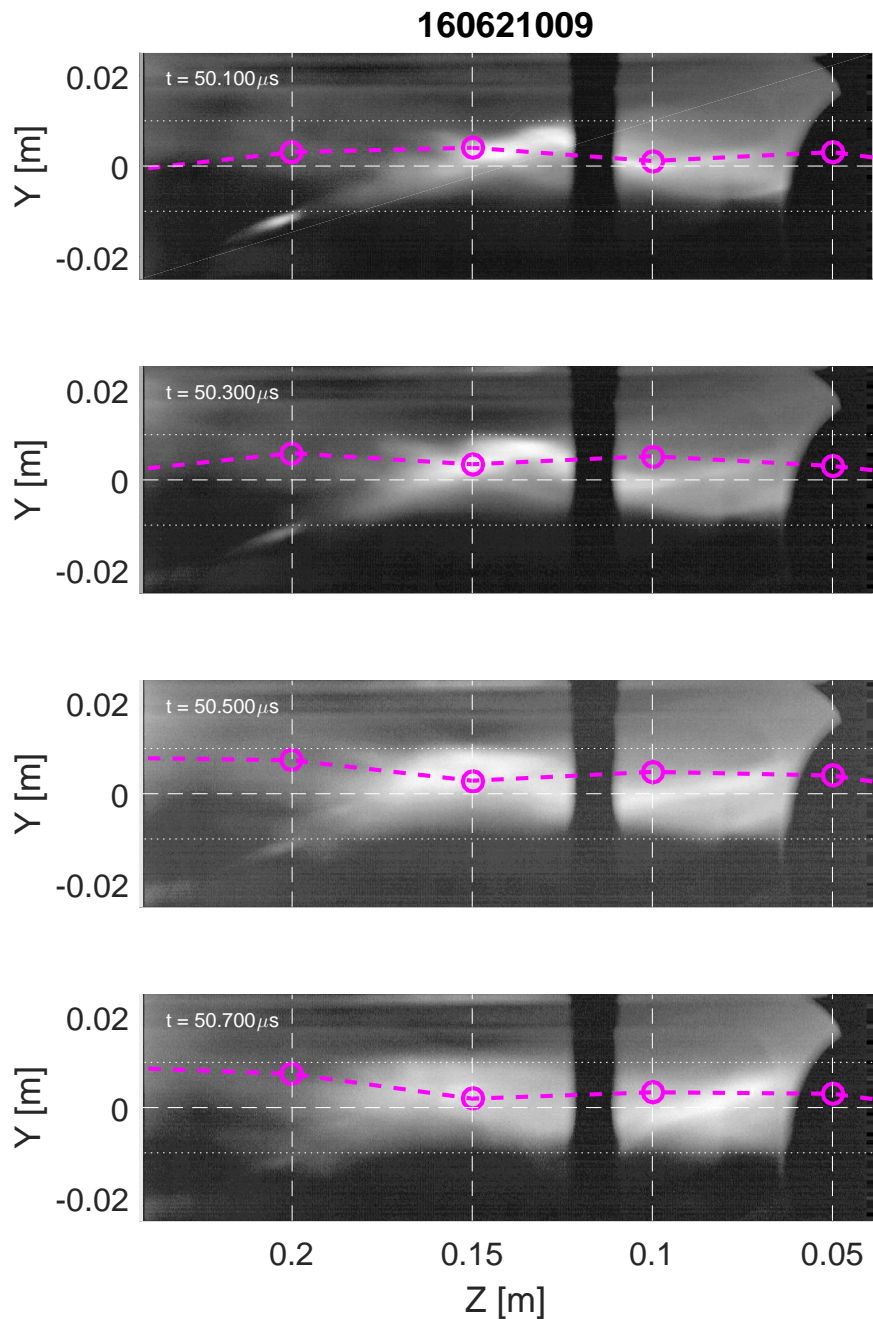
Figure 5.4: High speed camera images showing a saturated kink instability move past the z = 15 azimuthal probe array without affecting the current centroid. The intensity is shown on a logarithmic scale. The size ( \lambda \approx 3 cm) and velocity ( \approx 5 cm/ \mu\text{s} ) are consistent with instabilities seen on ZaP. The vertical shadow at 0.12 m is part of a 3D printed hanger holding a laser beam guide. The shadow of the beam guide is visible at the right edge of the image.
