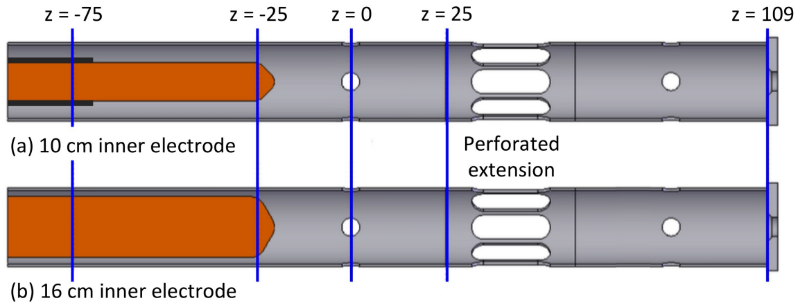
Figure 1.6: The 10 cm and 16 cm inner electrode configurations of the ZaP experiment are shown along with the outer electrode with the perforated section installed. Axial locations are referenced in units of cm. Gas injection from outer and inner valves occurs at z = -75 cm. The insulator extension shown in black extends downstream from these valves by 5 cm.
