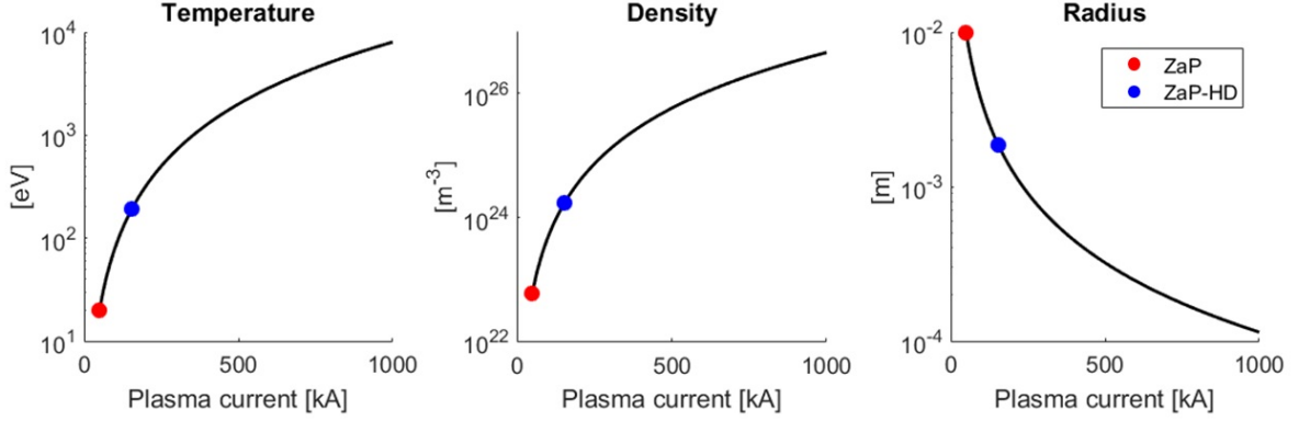
Figure 1.2: The ideal scaling of temperature, density, and radius with plasma current for an adiabatically compressed Z-pinch with constant linear density. The red and blue dots indicate the nominal run conditions for ZaP and ZaP-HD respectively.
