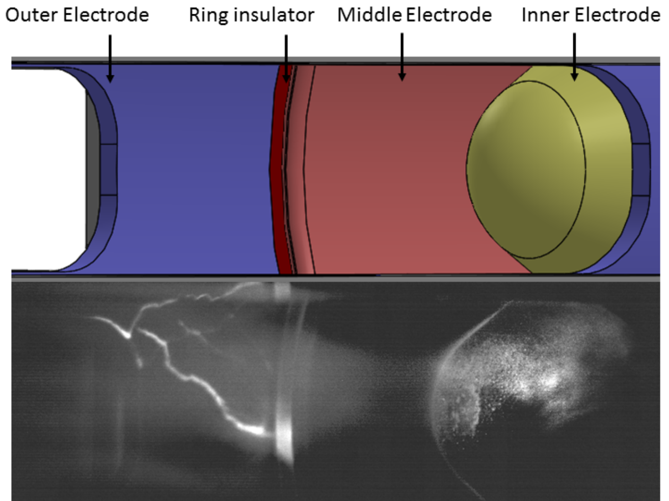
Figure 2.14: (top) A CAD image indicates the positions of the electrodes and ring insulator. (bottom) An optical camera image taken with a bremsstrahlung filter, f stop of 5.6, and exposure time of 200 ns (pulse 160224046). Localized plasma contact between the middle and outer electrodes across the ring insulator correlates with current centroid position data at z = 0 and suggests current flow directly between the outer and middle electrodes.
