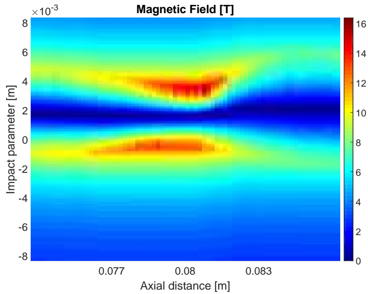
Figure 4.13: Contours of magnetic field for pulse 160621026 analyzed in Fig. 4.11. This pulse exhibits significant axial variation in field with the highest fields in cross-sections with the smallest pinch radii.
