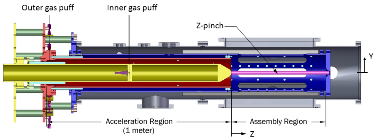
Figure 2.1: A cross section of the ZaP-HD experiment reveals its triaxial electrode design. A coaxial accelerator ionizes and accelerates plasma into the assembly region where the plasma is compressed on axis as a Z-pinch. The inner, middle, and outer electrodes are colored yellow, red, and blue respectively. The vacuum chamber is shown in gray, and the Z-pinch is in pink. The ZaP-HD coordinate system is also shown; unlike in ZaP, z = 0 is located at the inner electrode nosecone. Neutral gas injection into the accelerator between the middle and inner electrodes occurs at the two labeled axial locations. The inner gas injection puffs from a single valve through a manifold with eight outlets spaced evenly on the circumference of the inner electrode. The outer gas injection puffs inward from the exterior of the middle electrode through eight valves at the farthest upstream location in the accelerator.
