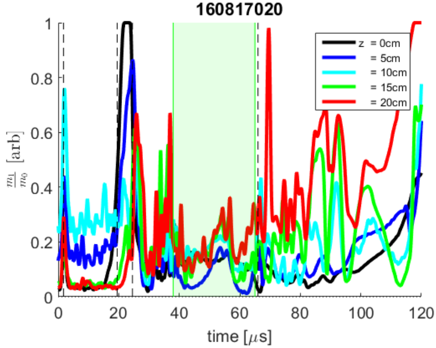
Figure 2.9: In a typical ZaP-HD plasma pulse, a quiescent period of relatively low mode activity occurs, which corresponds to optical camera images showing stable, slowly varying plasma behavior. The normalized mode data, \frac{m_1}{m_0} , remains relatively low during this period denoted in shaded green. On ZaP, \frac{m_1}{m_0} would remain below 0.2 for the quiescent period. On ZaP-HD, \frac{m_1}{m_0} often takes higher values than 0.2 during the quiescent period, but \frac{m_1}{m_0} between z = 0 cm and 20 cm changes slowly during this time, which indicates the current centroid moves gradually. Optical images corroborate that the plasma moves slowly as a coherent structure during the quiescent period. The \frac{m_1}{m_0} further downstream in the assembly region exhibits more rapid oscillations than the data from z = 0 cm to 20 cm. Optical images also suggest less coherent plasma structure and less stable dynamics further downstream. The first, second, third, and fourth dashed vertical lines correspond to the acceleration bank discharge, plasma exiting the accelerator, the compression bank discharge, and the high peak in the assembly magnetic field respectively.
