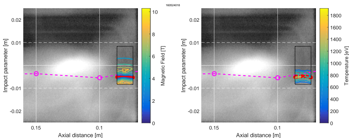
Figure 5.11: Contours of (left) magnetic field and (right) temperature are plotted over an optical image taken during pulse 160524018 at 50 \mu\text{s} , the time of the DHI pulse. The field and temperature are computed from the density in Fig. 5.10. The field and temperature are computed from the density in Fig. 5.10. The magenta circles are the current centroid locations projected into the plane of the image. Excellent correlation exists between the field, temperature, and current centroid.
