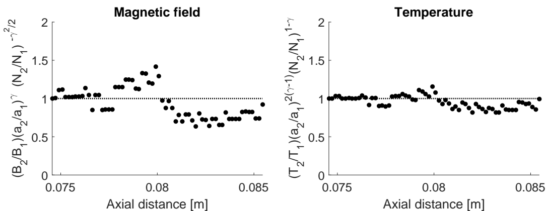
Figure 4.10: Examining relations between pinch size and density and field and temperature to determine if an axially uniform Z-pinch behaves adiabatically. The two plots compare the left and right-hand-sides of Eqs. (4.20, 4.21) for pulse 160524021. The profiles below the density centroids in Fig. 4.7 are used in this analysis, and each black marker corresponds to a profile at a different axial location. Upstream of 0.077 m, the markers near a value of 1 on the ordinate indicate states reached in agreement with the adiabatic scaling laws. Between 0.077 and 0.081 m, non-constant deviations of the markers from 1 suggest non-adiabatic processes are responsible for the difference of the plasma state in this region compared to the upstream region. The flat region in the markers downstream of 0.081 m indicates differences in the plasma state within this region are explained by adiabatic processes.
