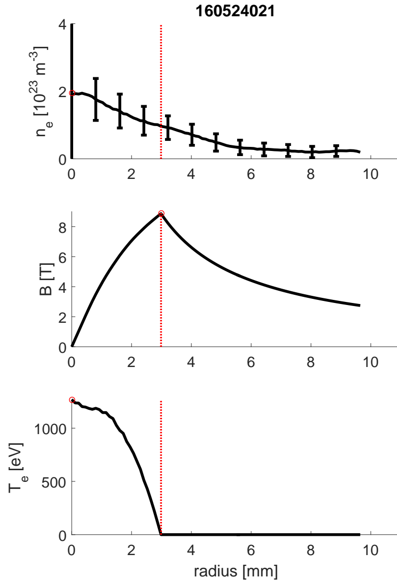
Figure 4.5: Cross-sections of measured density and computed field and temperature from the uniform drift velocity equilibrium model for pulse 160524021. This pulse exhibits relatively narrow profiles. The vertical red lines indicate the pinch radius, a , and the red circles indicate the peak density, edge field, and peak temperature values taken as characteristic property values.
