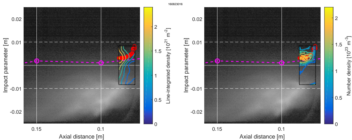
Figure 5.12: Contours of (left) line-integrated density and (right) number density are plotted over an optical image taken during pulse 160823016 at 60 \mu\text{s} , the time of the DHI pulse. The magenta circles are the current centroid locations projected into the plane of the image, and the red markers indicate the density centroid computed during Abel inversion. Here, excellent correlation exists between density and current centroid, but the light emission position is significantly different. In the upstream portion of the DHI data, the density centroid reaches the edge of the imaged area. At every cross-section where this happens, the number density is set to zero across the cross-section.
