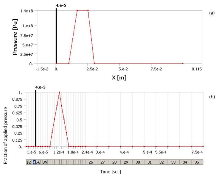
Figure D.7: (a) shows the spatial distribution of applied axial pressure on the plasma-facing endwall surface. The pressure and annular area to which it is applied are selected to match the expected cumulative applied load. Here, X is the radial component of a coordinate system centered on machine axis. (b) shows the time evolution of the applied pressure. The simulation is instructed to apply the specified fractions of the profile in (a) at each time point. The linear ramp up starts well after the simulation's start to ensure the transient behavior of the bolt pre-tension does not affect the results.
