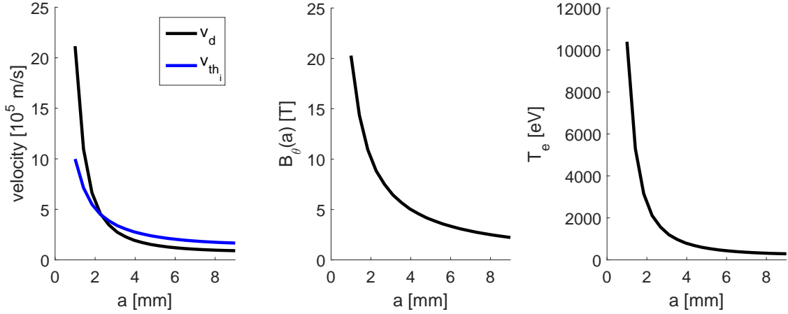
Figure 4.1: The sensitivity of plasma parameters to chosen plasma radius a . Conditions where v_d > v_{th_i} are non physical. The magnetic field at the plasma radius B_\theta(a) is less sensitive at larger radii as is the maximum T_e .
