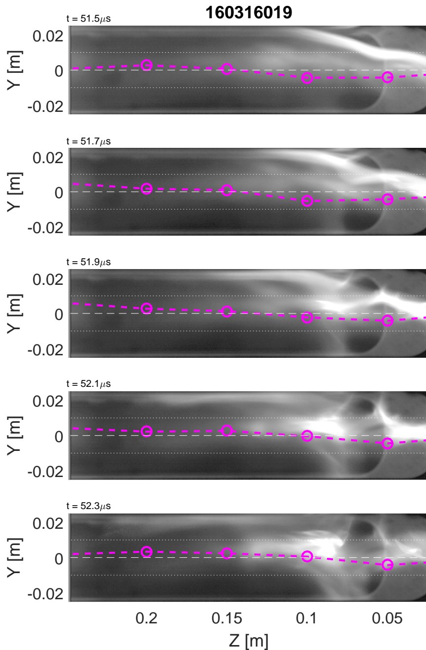
Figure 5.6: High speed camera images showing plasma translation and instability behavior not captured by magnetic mode data. In the first frame, a large structure has already deviated far from the current centroid. The subsequent frames show a kink instability grow and break apart. Throughout the instability breakup, the mode data remains well within the ZaP stability criterion. The mode data only register unstable conditions 4 \mu\text{s} after the final frame shown here.
