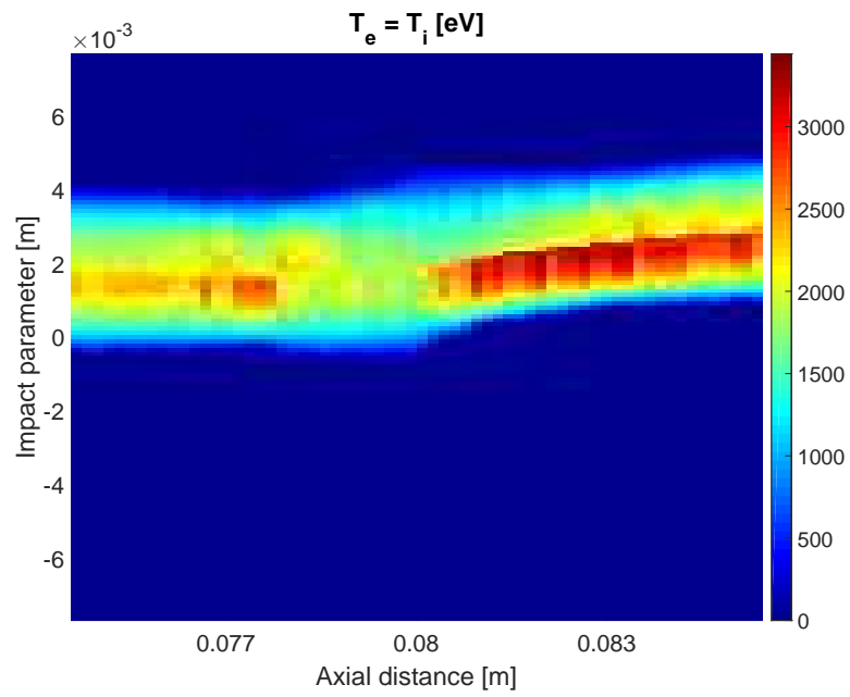
Figure 4.9: Contour plot of temperature, T_e = T_i , computed from uniform drift velocity equilibrium analysis for pulse 160524021. The density contour for this relatively axially uniform pulse is Fig. 4.7.
