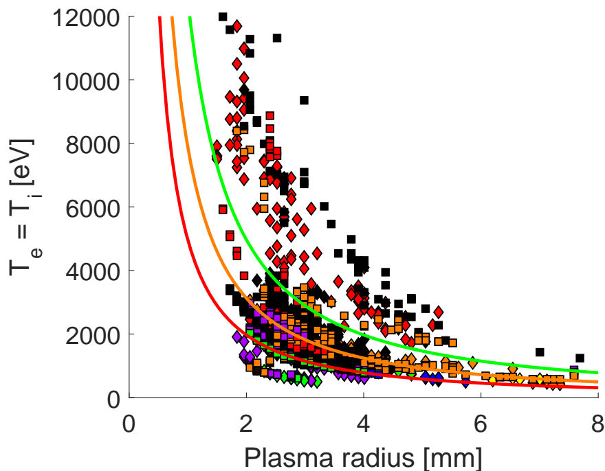
Figure 4.18: Temperature plotted versus plasma radius for profiles from many plasma pulses with similar run settings. Markers are colored according to the linear density ranges in Fig. 4.15. The orange curve represents the adiabatic scaling of Eq. (4.20) for the orange linear density bin. The curve is drawn from Eq. (4.20) with N_2/N_1 = 1 and an initial state chosen to maximize the proximity of the curve to the orange markers. The green and red curves indicate the adiabatic scaling for values of N_2/N_1 of 2 and 1/2 respectively, which correspond to the green and red linear density ranges. The observed temperature follows the predicted trend of increased temperature at smaller pinch sizes. The dependence of the empirical data on linear density appears inverted from the adiabatic predictions with markers of higher linear density generally shifted towards the lower-left corner of the plot.
