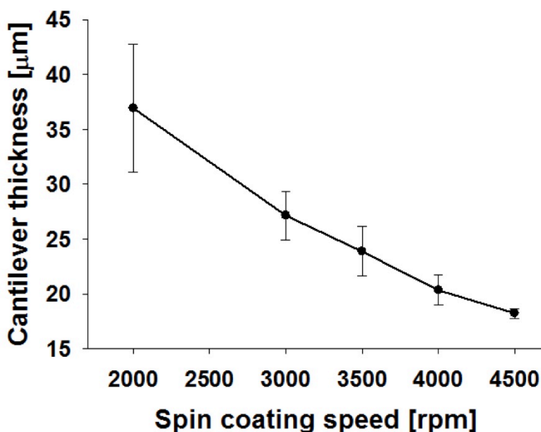
Figure 7. Cantilever thickness measured using optical microscope. The thickness of PDMS cantilevers over a range of spin coating speed was plotted. The thickness decreased as the spin coating speed increased. (Error bars: \pm SEM)
