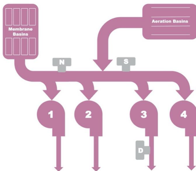
Figure A7. Brightwater treatment plant odor control system. Gaseous analyzer sample locations are labeled as “N” (North), “S” (South), and “D” (Downstream). The four odor control blowers are labeled 1-4.
