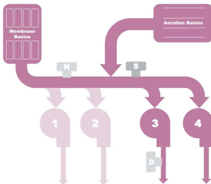
Figure A8. Configuration 0011S. Blowers 1 and 2 are off, and blowers 3 and 4 are on. The gaseous analyzer is located at the South sampling port.
