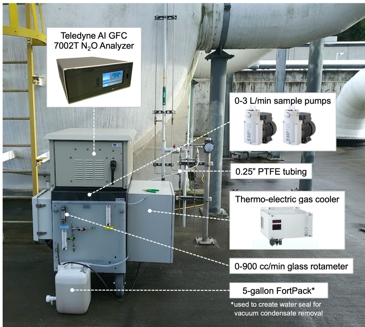
Figure A5. Gaseous N 2 O field sampling unit.
