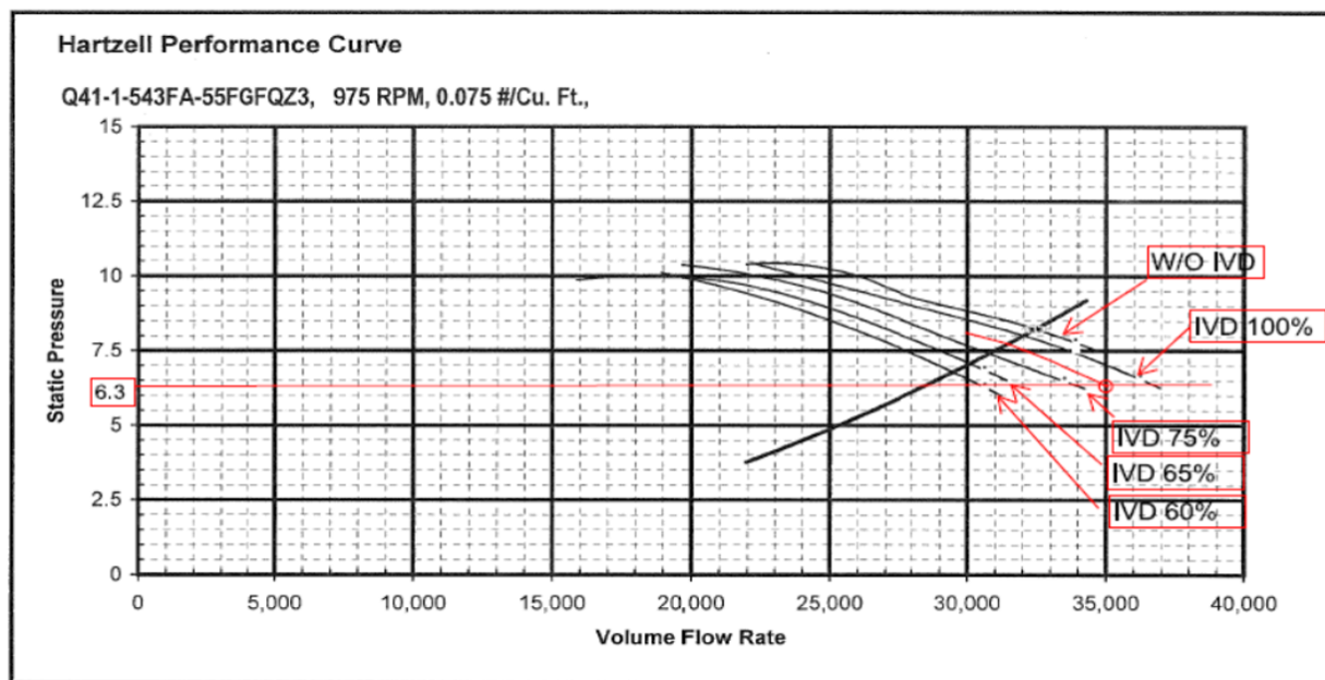
Figure A6. Performance curves for Brightwater odor control blowers. Static pressure is reported in inches water column (in wc). Volume flow rate is reported in standard cubic feet per minute (SCFM). IVD stands for Inlet Vane Damper and is reported as percent open.
