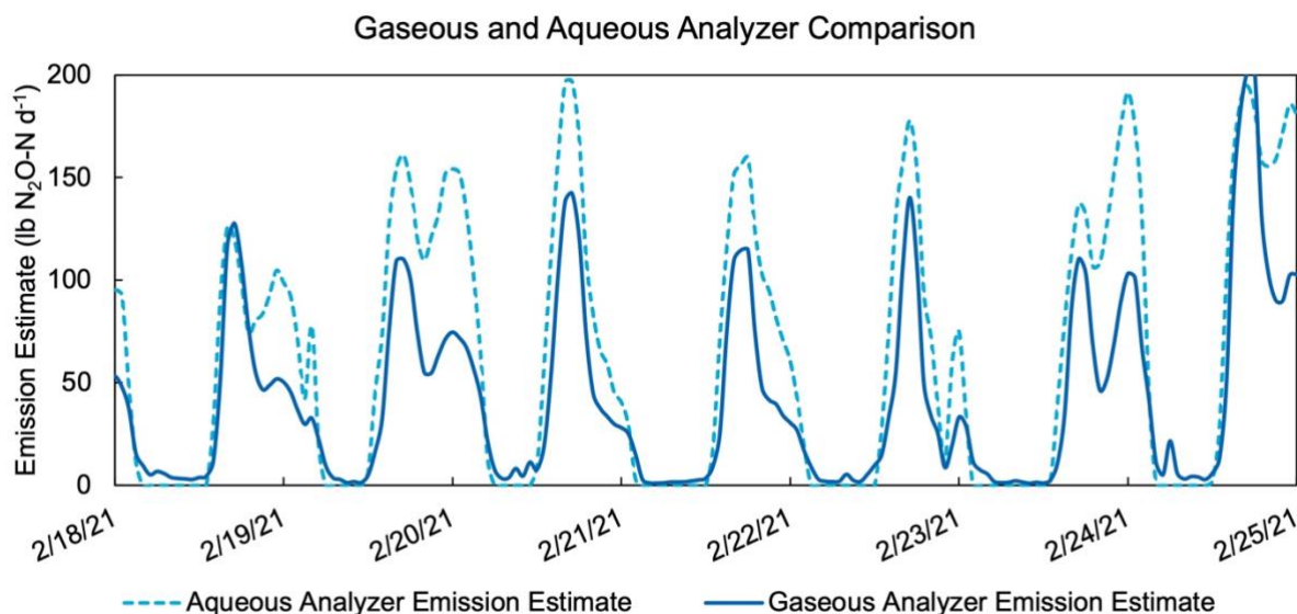
Figure 3-5. Discrepancy between aqueous and gaseous emission estimates while the gaseous analyzer sample was fully representative of both aeration and membrane basin emissions.
