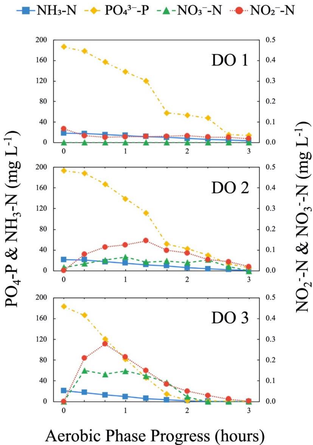
Figure 4-1. Aerobic phase nutrient concentration profiles at varied dissolved oxygen concentrations.
