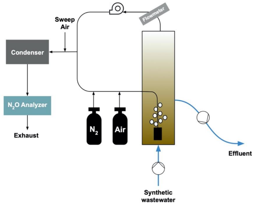
Figure B1. Lab-scale sequencing batch reactor with gaseous \text{N}_2\text{O} analyzer
