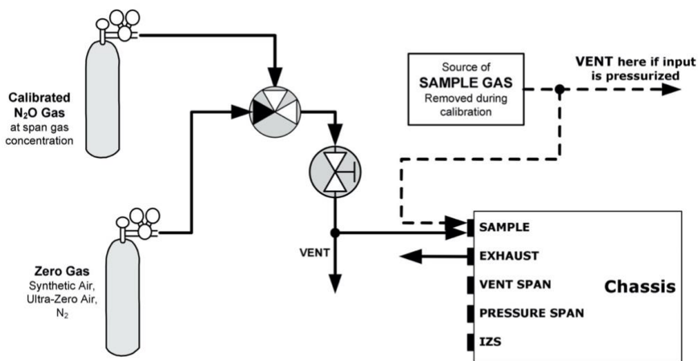
Figure A1. Pneumatic connections using bottled span gas
