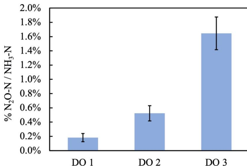
Figure 4-2. Percent of oxidized NH 3 -N emitted as N 2 O-N at dissolved oxygen concentrations of 1, 2, and 3 mg O 2 L -1 .
