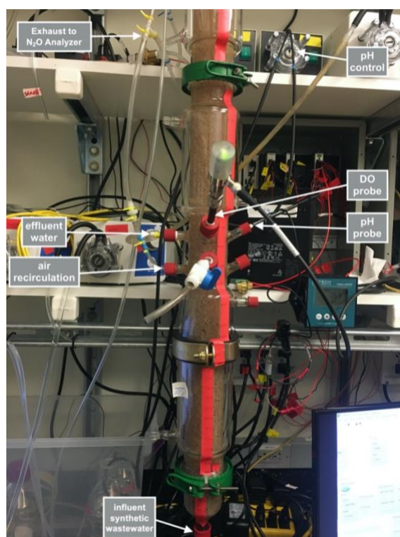
Figure B2. Image of lab reactor (some reactor components are not shown)
