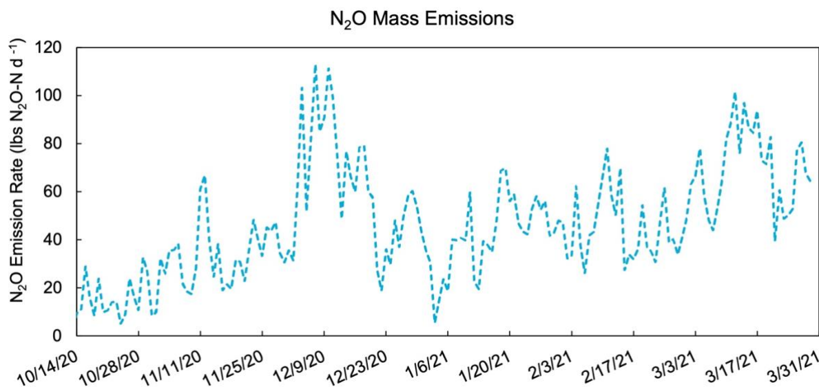
Figure 3-7. N 2 O mass emissions over the course of the monitoring period.
