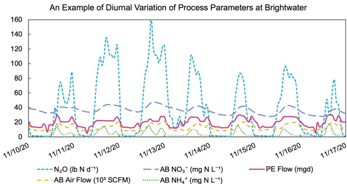
Figure 3-4. Process parameters demonstrating diurnal variation with \text{N}_2\text{O} . A representative 7-day period (November 10-17) was chosen to display data at high temporal resolution (hourly) to demonstrate diurnal variability.
