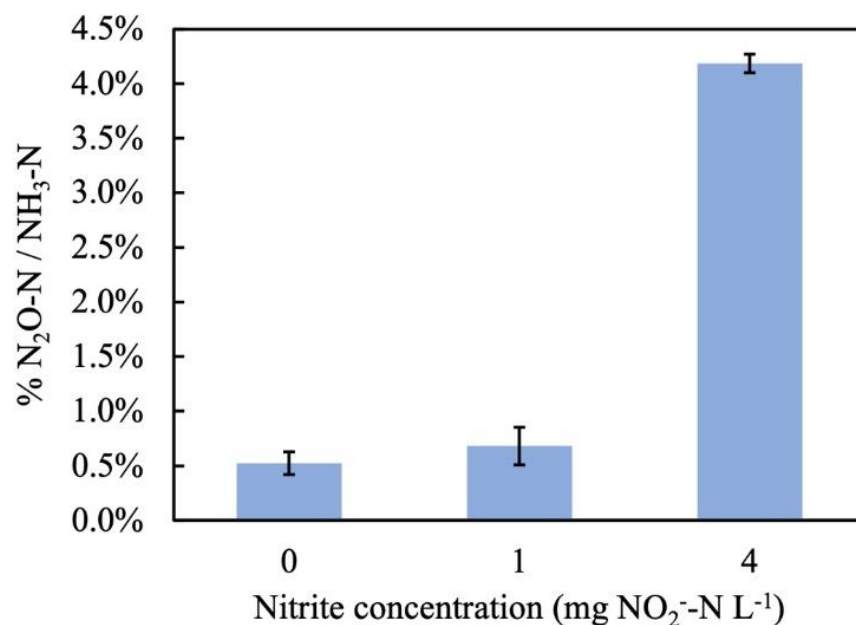
Figure 4-4. Percent of oxidized NH 3 -N emitted as N 2 O-N at differing NO 2 - concentrations at the beginning of the aerobic phase, with DO controlled at 2 mg O 2 L -1 .
