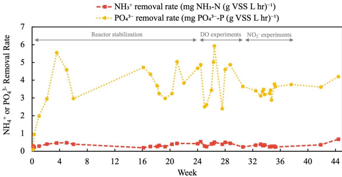
Figure B6. Reactor performance; ammonia and phosphate removal rates over reactor lifetime
