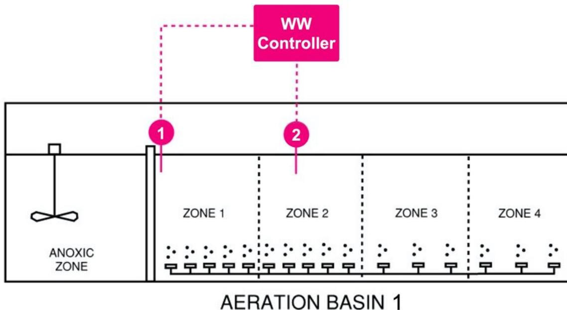
Figure 3-3. Aqueous N_2O measurement setup. N_2O sensors are labeled 1 and 2.
