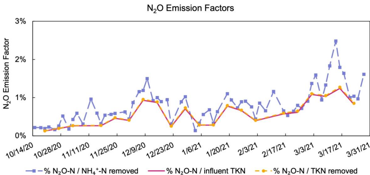
Figure 3-6. N 2 O emission factors over the course of the monitoring period.
