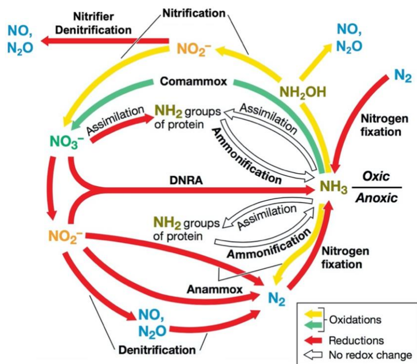
Figure 2-3. Biological nitrogen cycling with relevant \text{N}_2\text{O} emission pathways. (Adapted from Brock Biology of Microorganisms 28 ).
