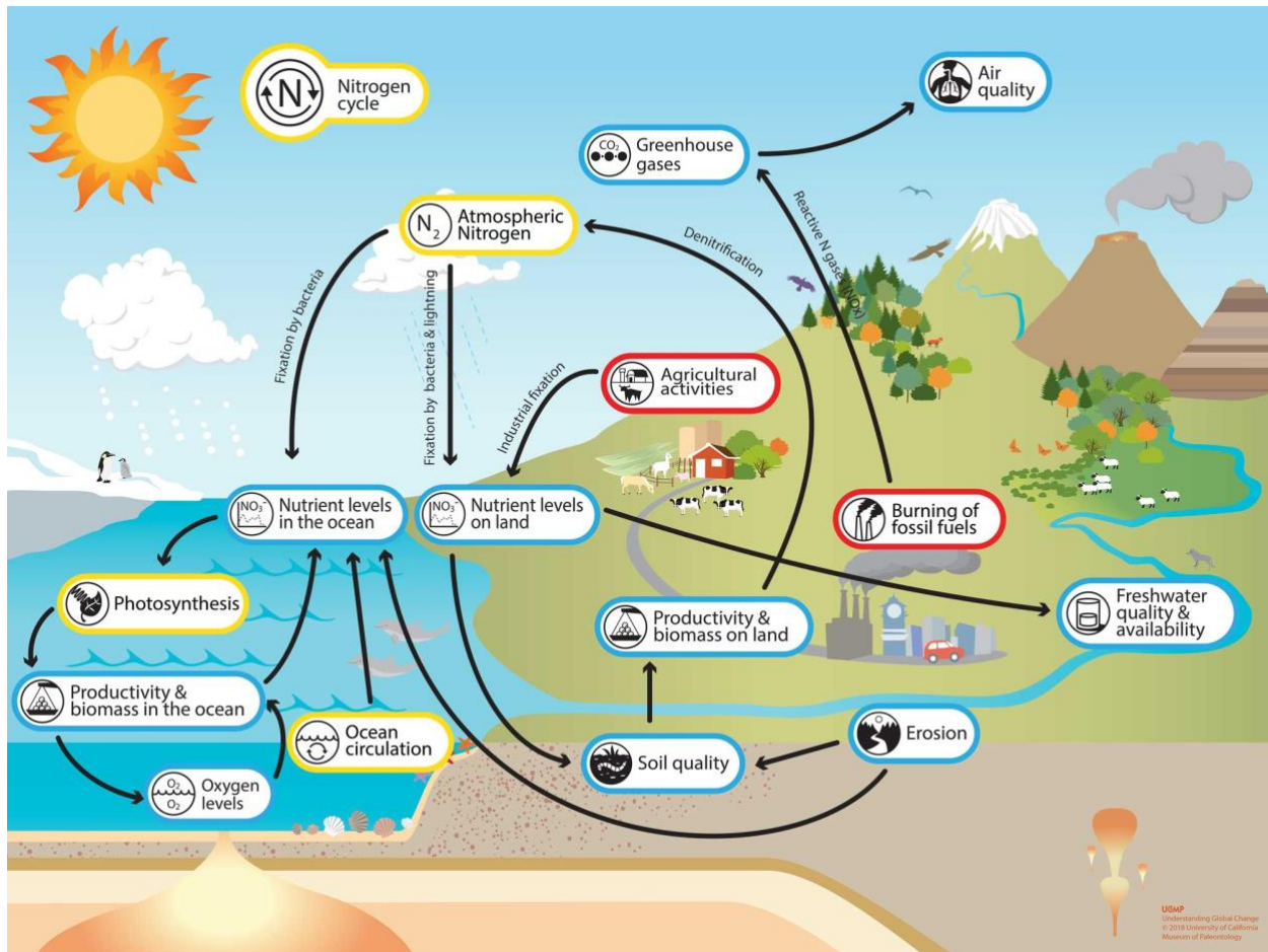
Figure 2-1. Earth system model of the nitrogen cycle (University of California Museum of Paleontology) 13 .
