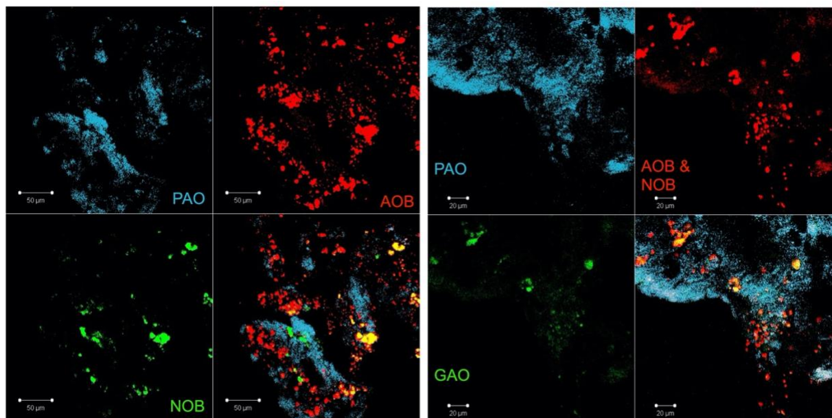
Figure B5. Color separated FISH images
