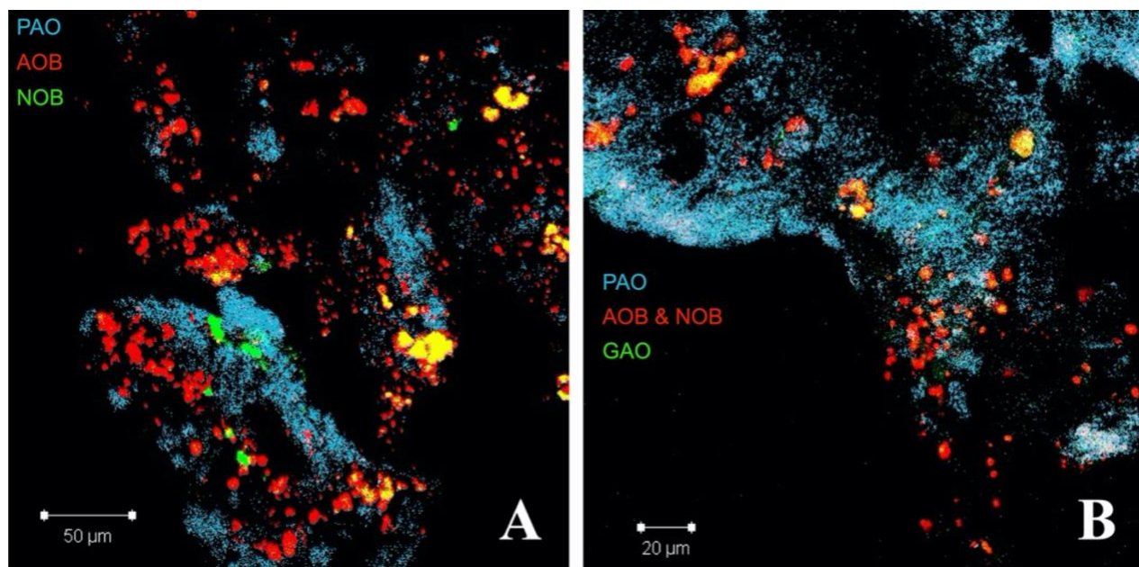
Figure 4-6. FISH imagery with PAO, AOB, and NOB displayed in A and PAO, AOB+NOB, and GAO in B.
