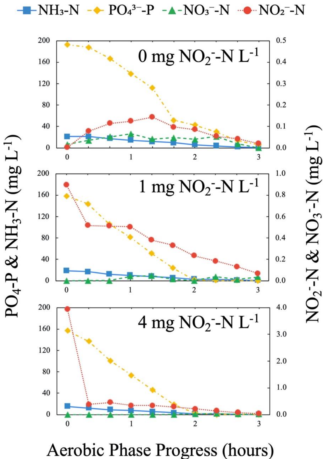
Figure 4-3. Aerobic phase nutrient concentration profiles for varied \text{NO}_2^- concentration spikes with DO controlled at 2 \text{ mg O}_2 \text{ L}^{-1} .
