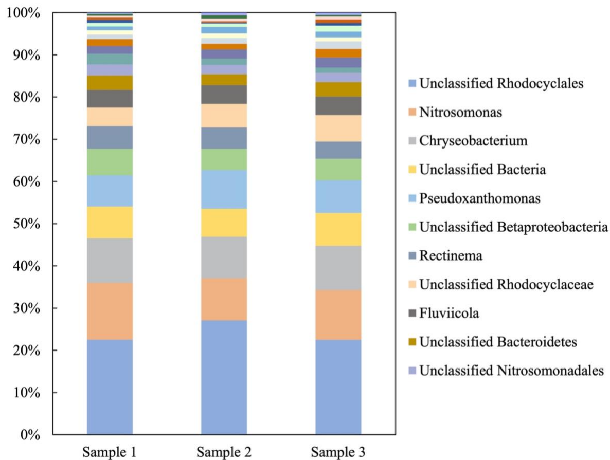
Figure B4. 16S rRNA sequencing data from AGS under baseline conditions
