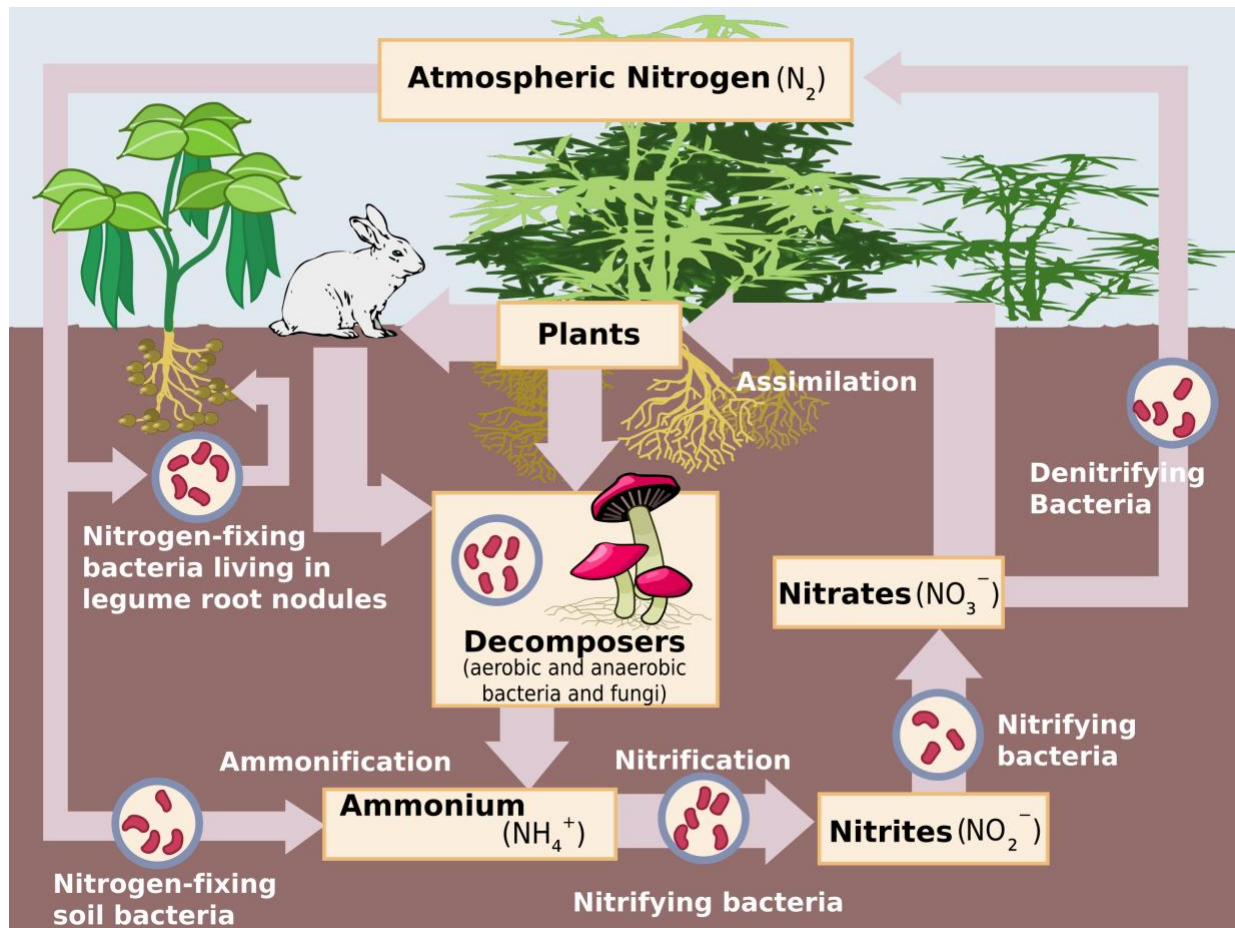
Figure 2-2. Major biological processes in the nitrogen cycle (USEPA, 2003) 14
