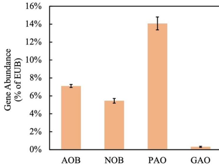
Figure 4-5. qPCR results for AGS under baseline conditions.
