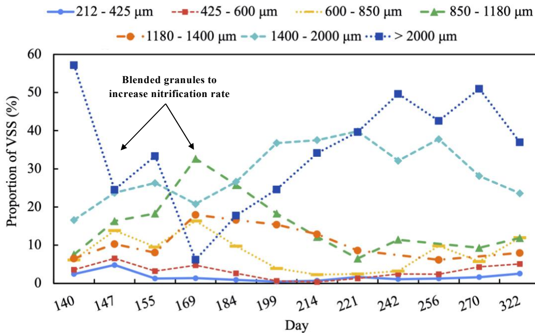
Figure B7. Granule size distribution over time
