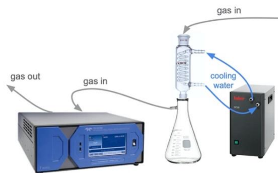
Figure B3. \text{N}_2\text{O} analyzer and condenser setup
