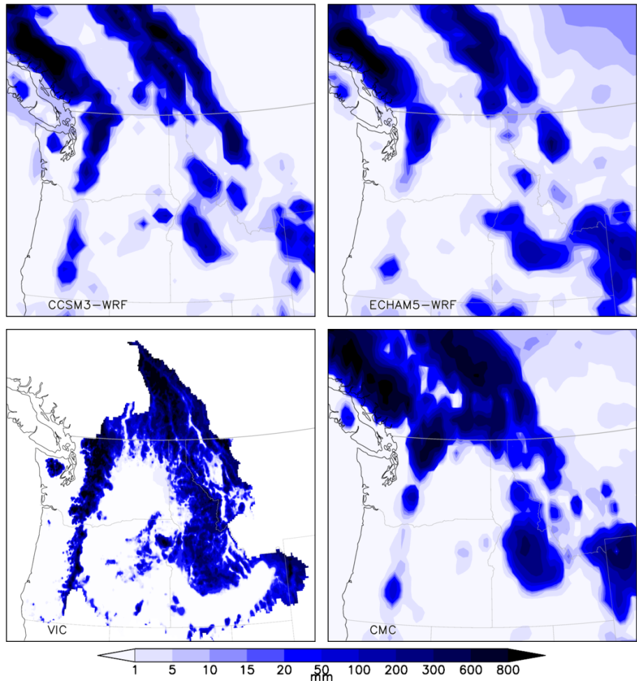
Figure 3. 1970-1999 simulated April 1 snow water equivalent (mm) from CCSM3-WRF (top left), ECHAM5-WRF (top right), the VIC model forced by the gridded observations in Figs 1 and 2 (bottom left). 1979-1997 average April SWE from the Canadian Meteorological Centre snow analysis (bottom right).
