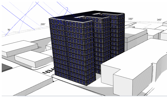
Fig.16:Shadow diagram of March 21st at Noon
