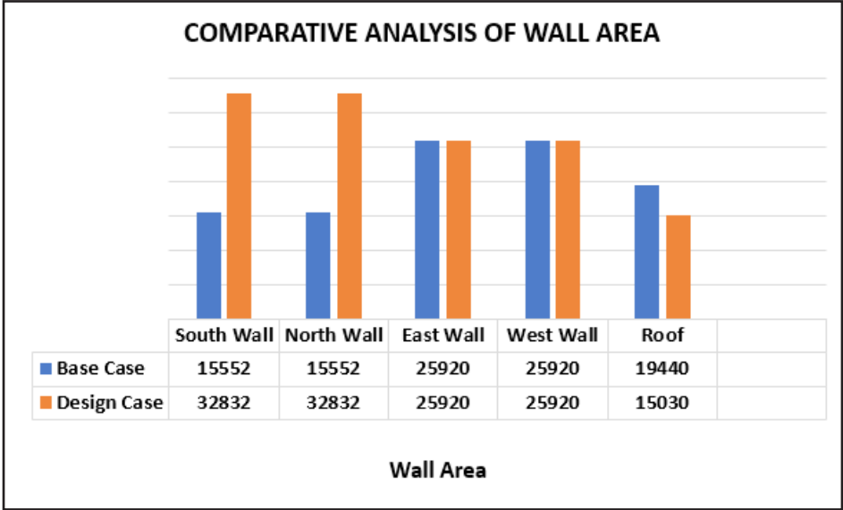
Fig.53: Comparative Analysis of wall surface area
