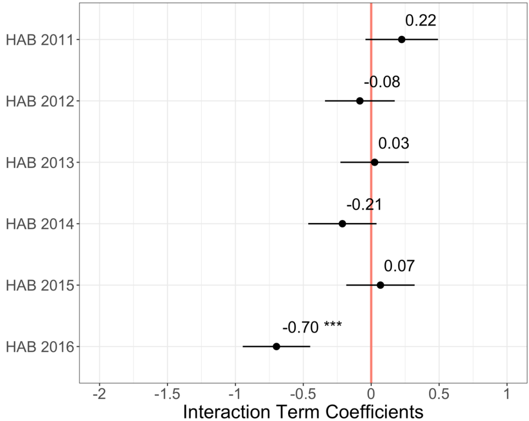
Figure 4: Placebo test interaction term coefficients and 95% confidence intervals, using robust standard errors.
