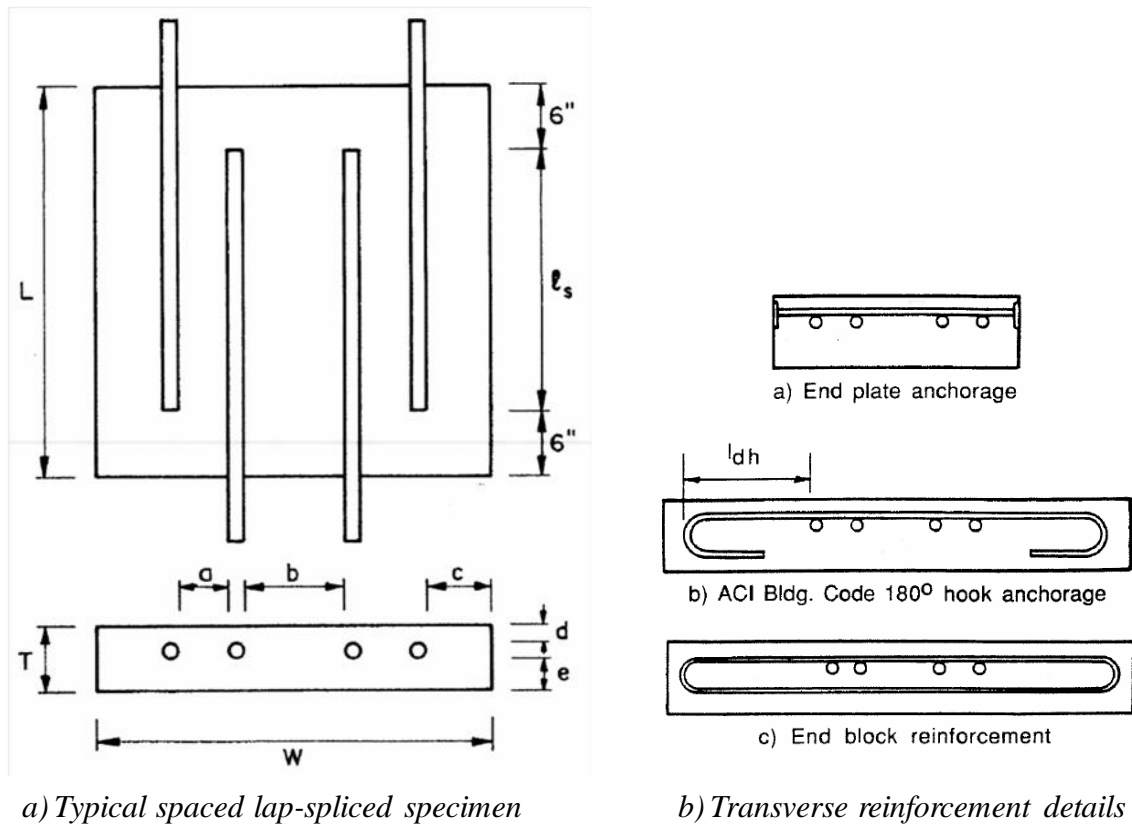
Figure 2-2. Noncontact lap splice flat-plate specimens (Sagan et al. 1991)
