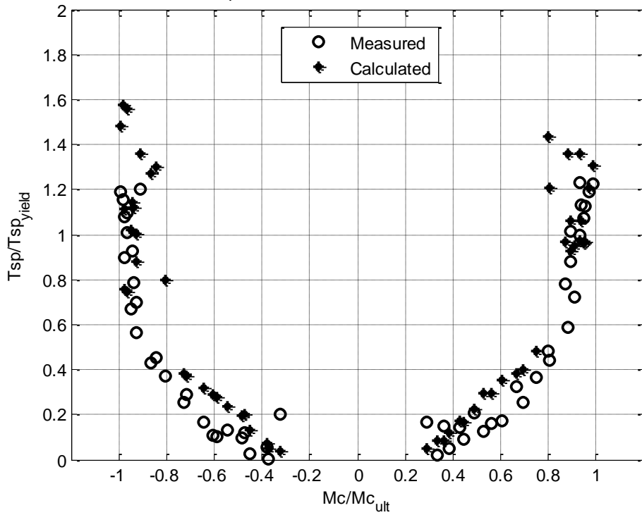
Figure 6-38. Spiral resultant force vs. column moment – DS-3
