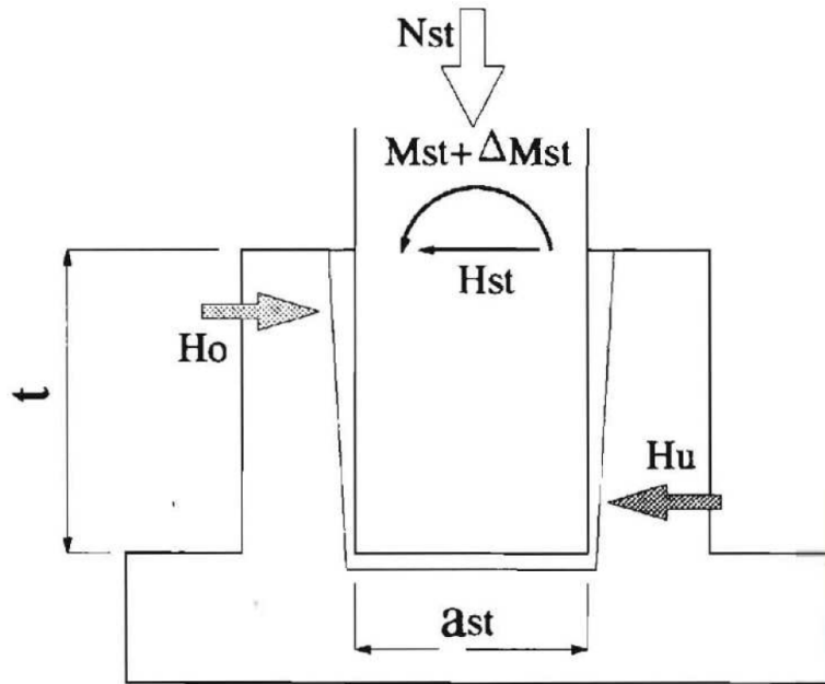
Figure 2-13. Concept of DIN-1045 (Osanaï et al. 1996)
