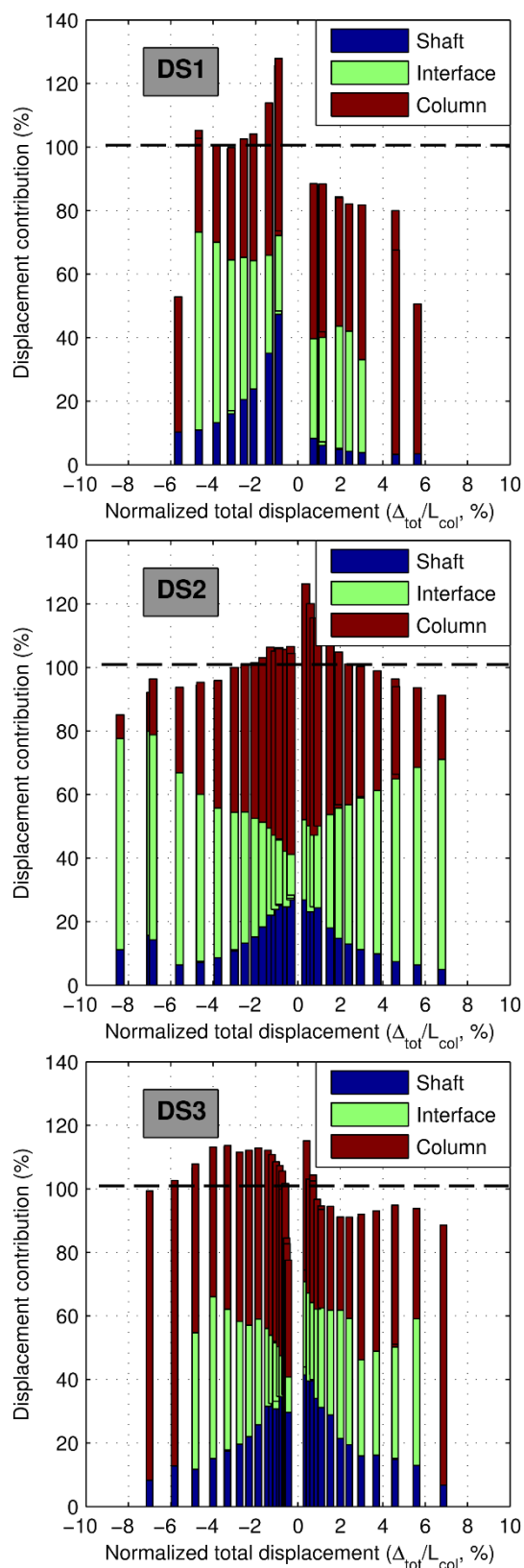
Figure 5-7. Displacement contribution
