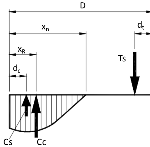
Figure 2-15. Stress distribution on the column section (Osanai et al. 1996)
