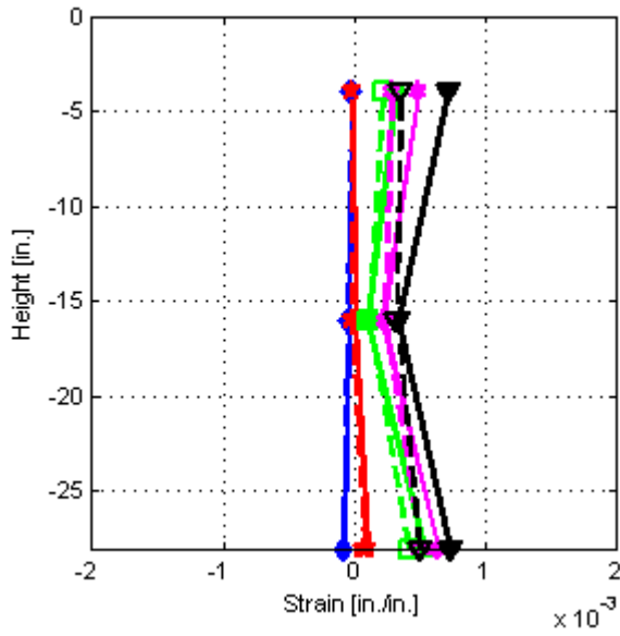
c). DS-1 - East reinforcing bar of shaft.
