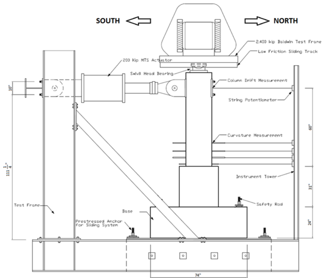
Figure 4-1. Test setup
