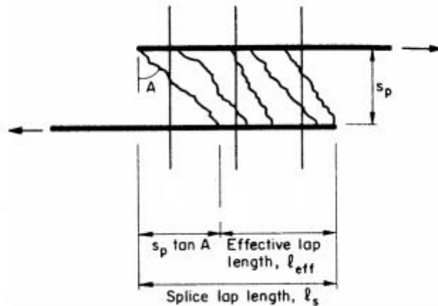
Figure 2-4. Effective lap length (Sagan et al. 1991)
