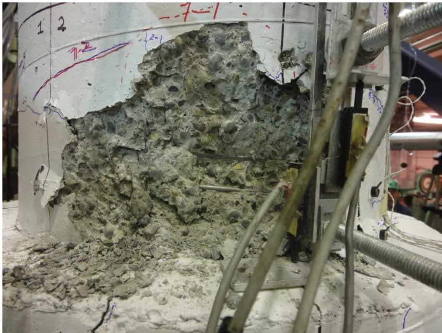
Figure C-0-16. DS-3 – Plastic hinge formed in the column at 4.57/-4.84 percent drift
