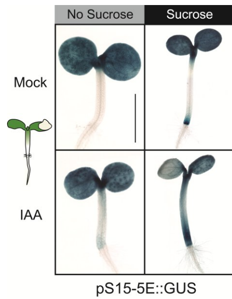
Figure S1
