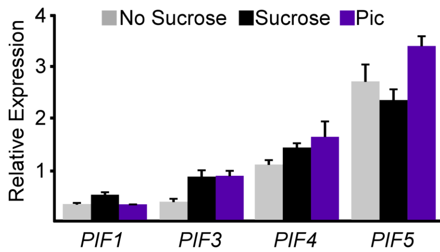
Figure S3
