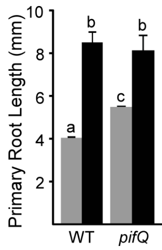
Figure S2
