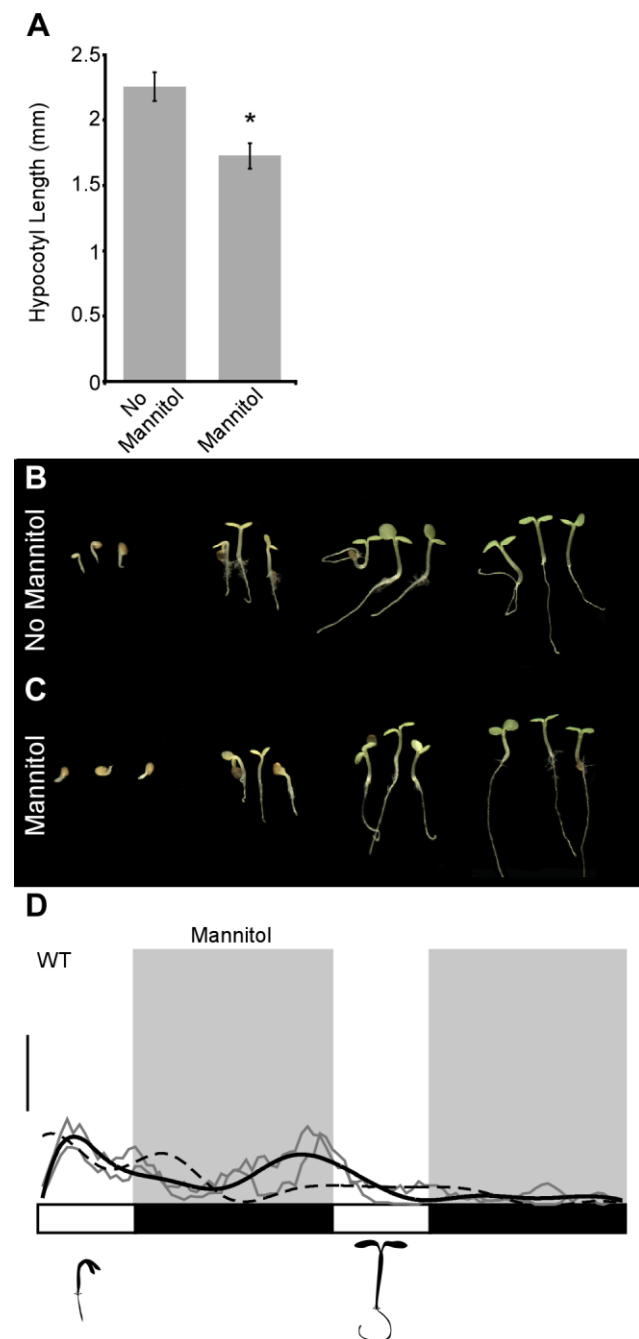
Figure S1
