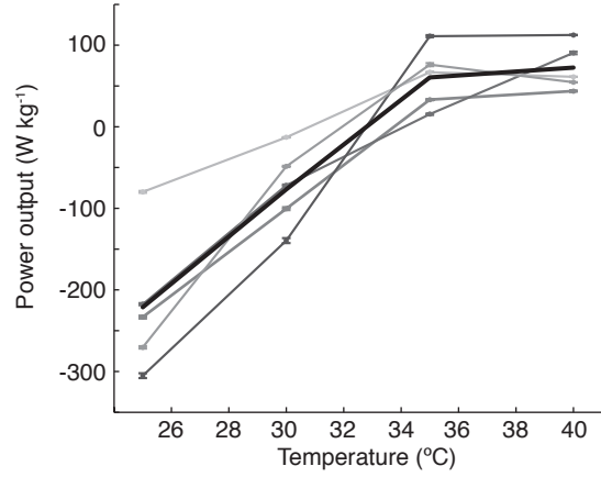
Figure 3.3: Temperature significantly affected power output in intact DLM I . Mass specific power output is plotted as a function of temperature at the approximately in vivo phase of activation (0.46) for intact DLM I . Each individual of the intact DLM I preparation is represented as a separate gray line. There were statistically significant differences in power output between each temperature point, except for one individual between 35-40°C (Tukey–Kramer HSD, P < 0.0001 ). The thick black line superimposed over the individual data represents the mean power output of all moths. Power output was positive between 40 and 35°C and negative between 30 and 25°C. Values are reported as means \pm s.e.m. ( N=5 moths, 20 cycles per trial).
