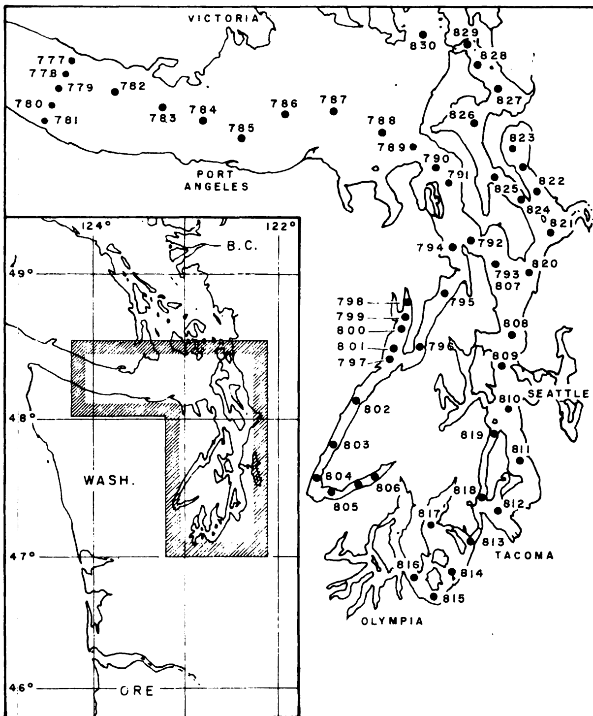
Oceanographic Station Locations Brown Bear Cruise 30 18-22 July 1953
