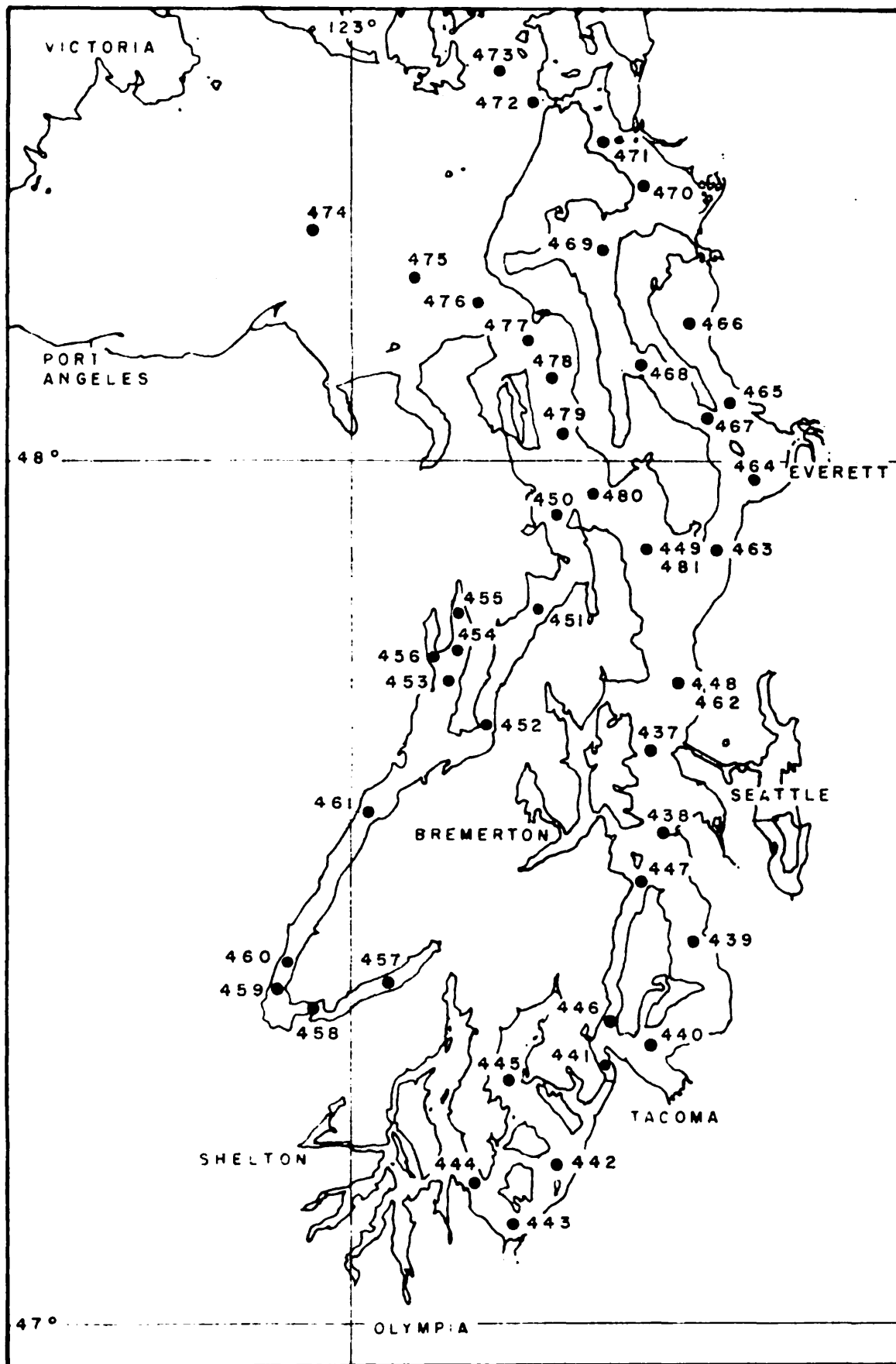
Oceanographic Station Locations Brown Bear Cruise 20 21-27 January 1953
