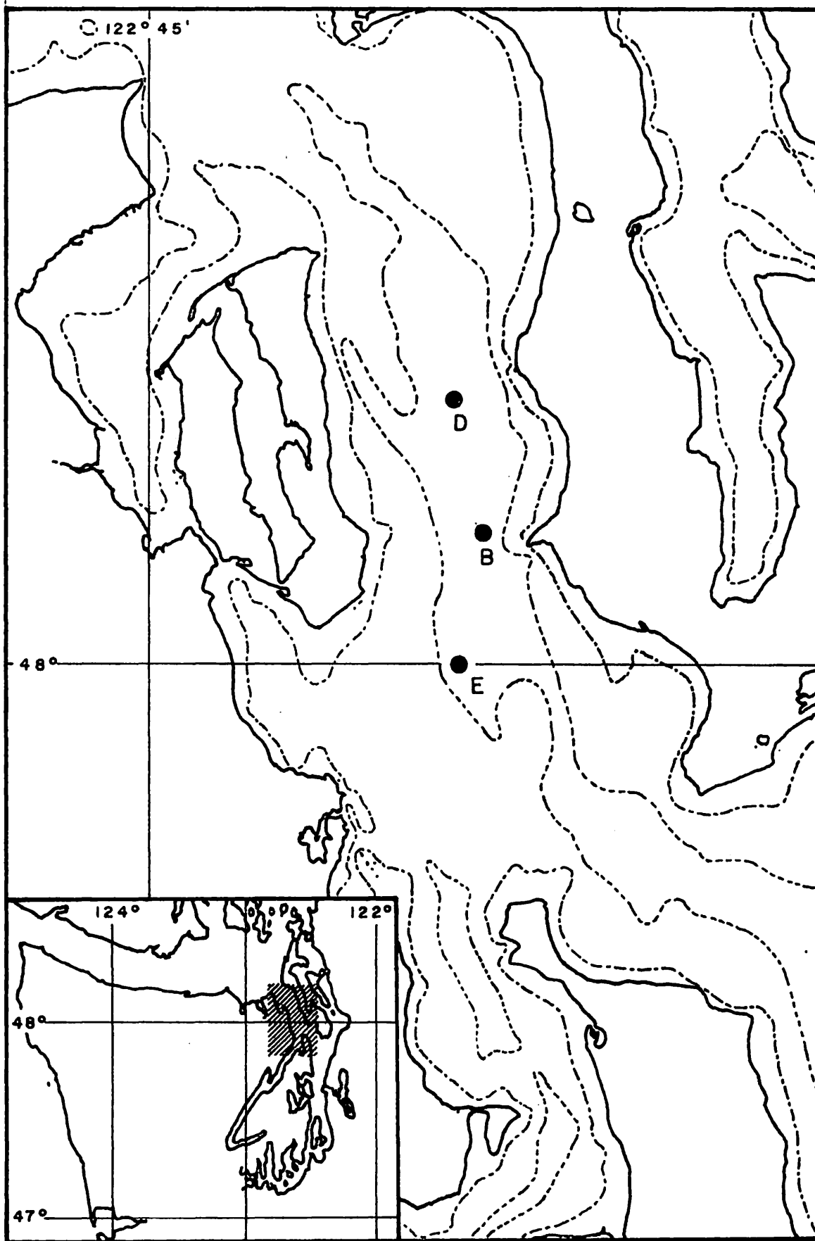
Oceanographic Station Locations Brown Bear Cruise 44 21 - 23 December 1953
