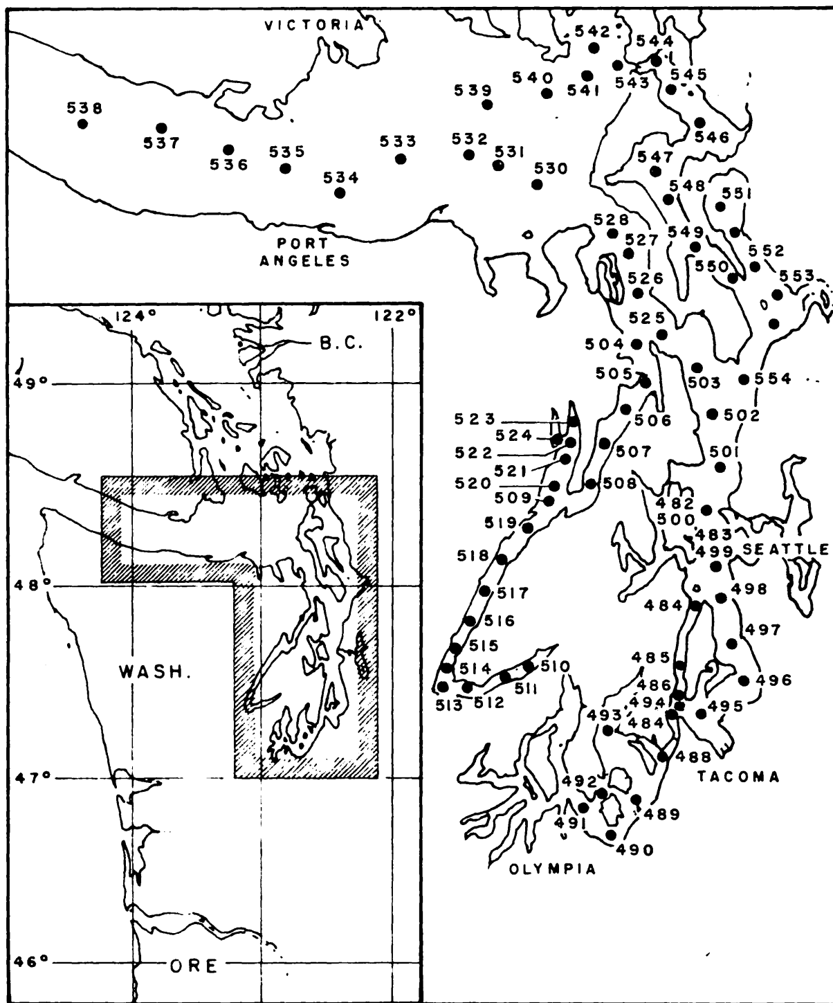
Oceanographic Station Locations Brown Bear Cruise 21 16-20 February 1953
