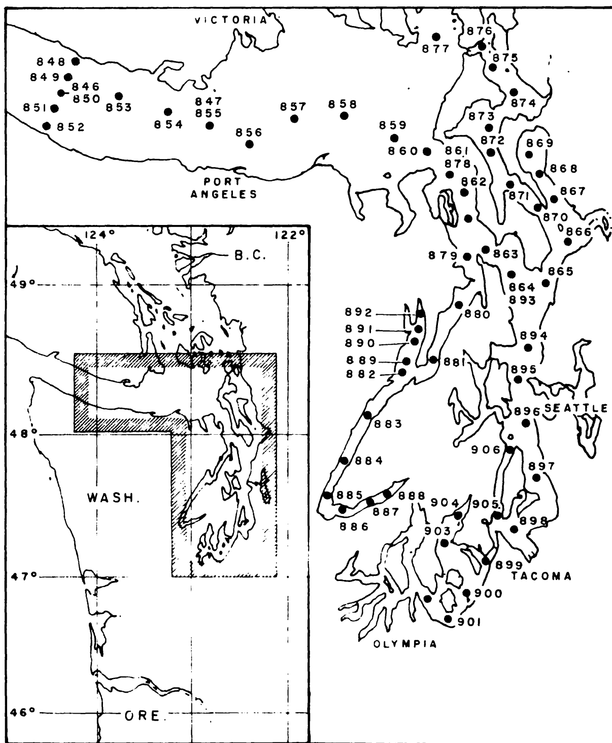
Oceanographic Station Locations Brown Bear Cruise 32 19-22 August 1953
