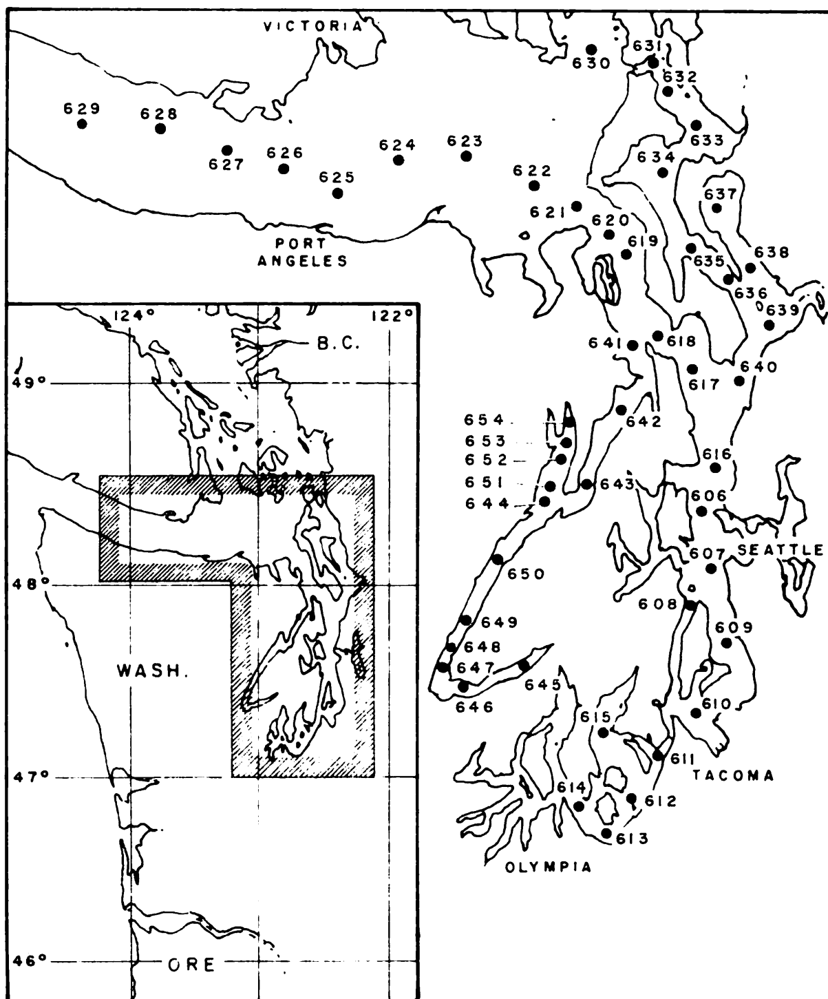
Oceanographic Station Locations Brown Bear Cruise 24 14-18 April 1943
