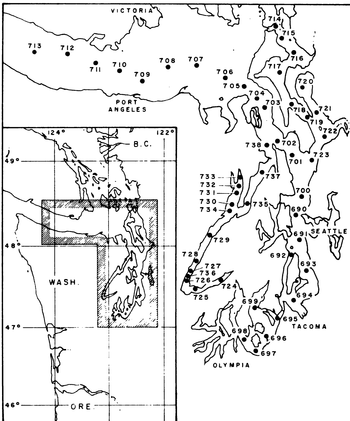
Oceanographic Station Locations Brown Bear Cruise 27 18-22 May 1953
