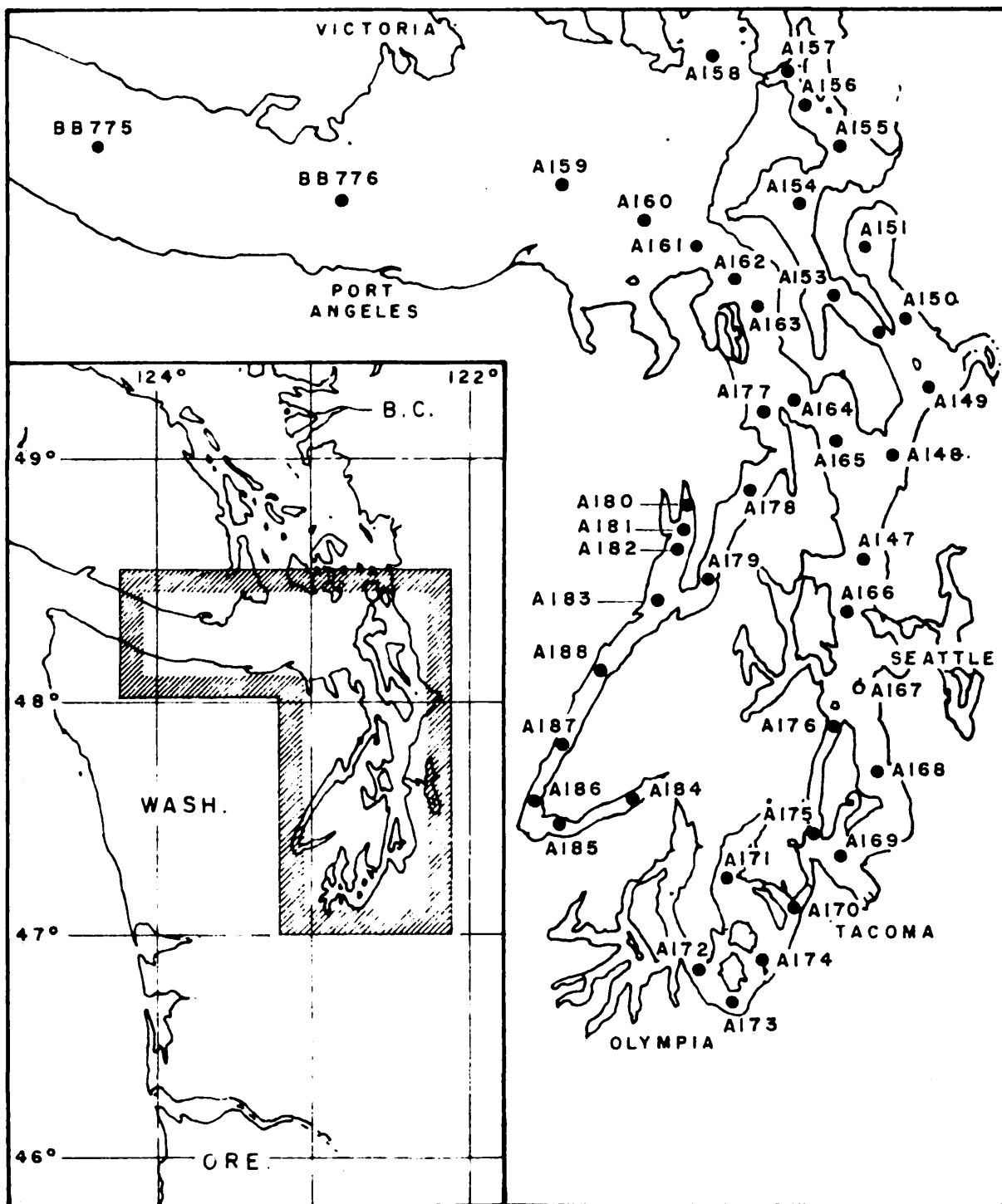
Oceanographic Station Locations Onchorhynchus Cruise PSS-10 17-25 June 1953
