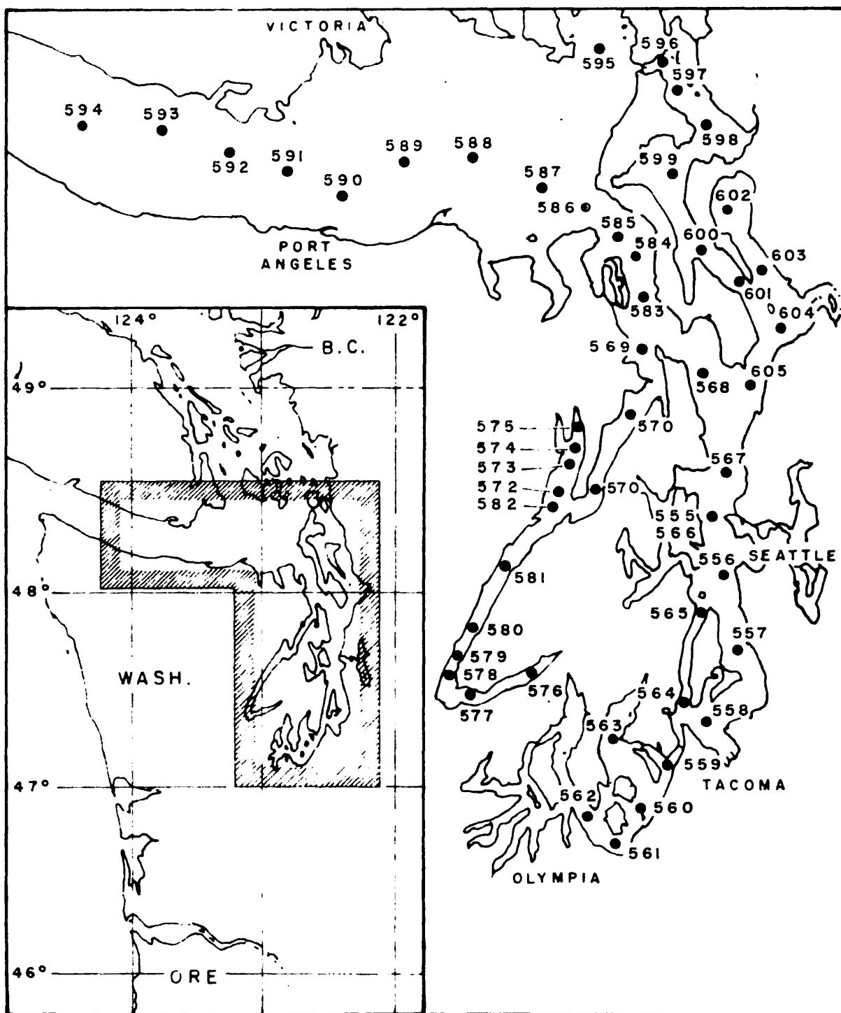
Oceanographic Station Locations Brown Bear Cruise 23 16-20 March 1953
