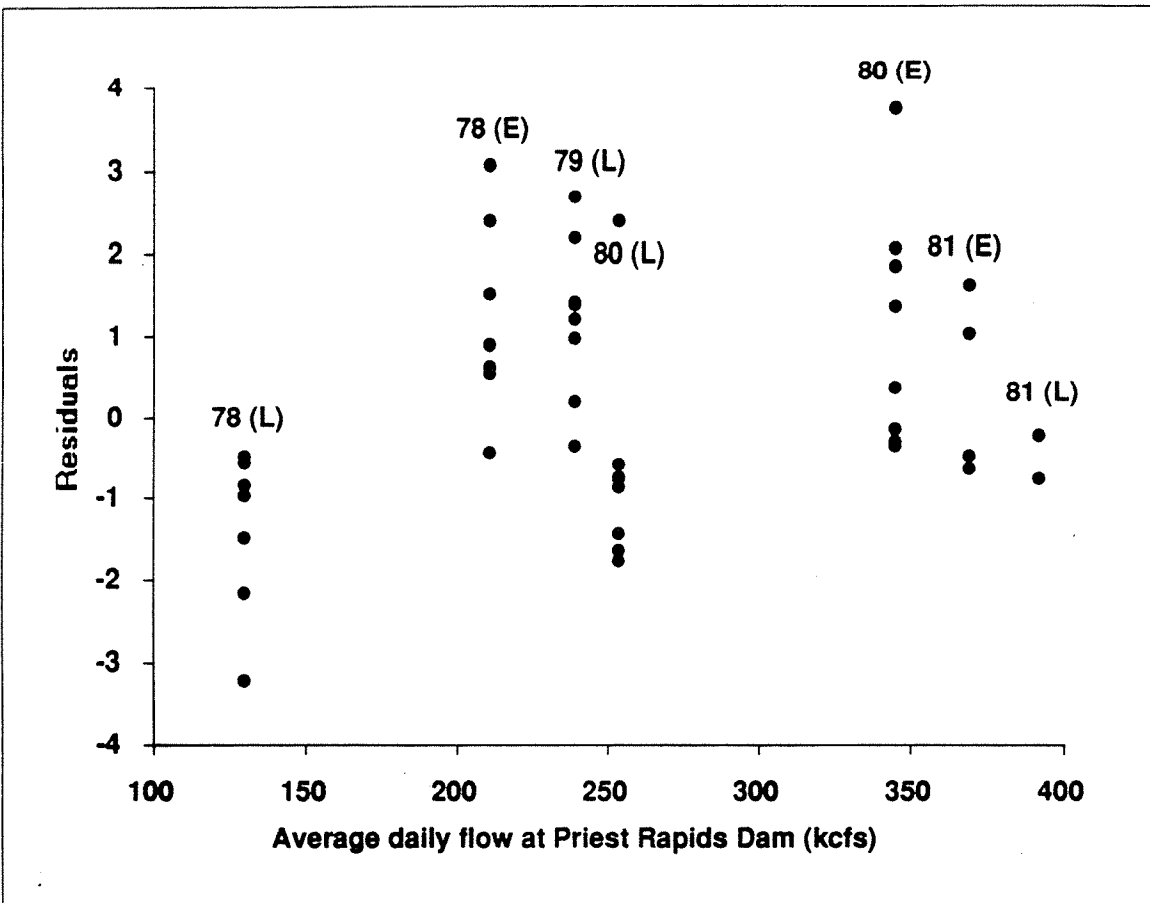
Figure 5.2. Residuals from fitting a log-linear model to Priest Rapids fall chinook recovery data plotted against daily average flow at Priest Rapids Dam at the time of outmigration. Numbers indicate brood year; E and L indicate early and late releases. Each residual is generated from the model fit for each space-time recovery component of each CWT group. Therefore, the number of residuals depends on the number of areas and ages of each CWT group at recapture.
