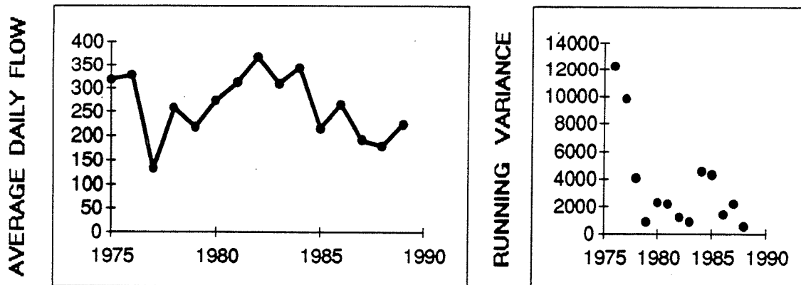
Figure 2.1. Time series of average daily flow during June and July and corresponding running variance at Priest Rapids Dam and John Day Dam.
