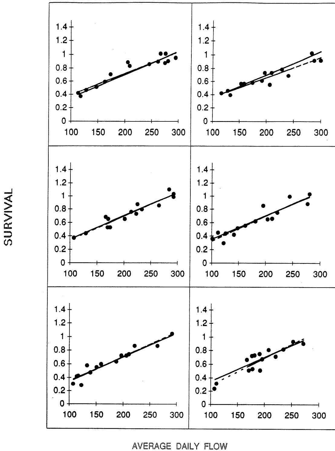
Figure 6.1. Six data sets of flow/survival data, randomly simulated with a low variance (coefficient of variation [(MSE^{1/2})/\text{mean flow}] = 0.1 ) and steep slope (survival at 100 kcfs = 0.5%, survival at 300 kcfs = 1%). Solid line represents expected flow/survival relationship and dotted line represents the estimated flow/survival relationship.
